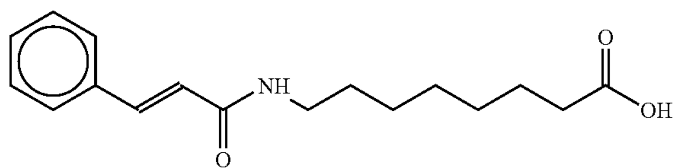
8-cinnamoylaminocaprylic acid
