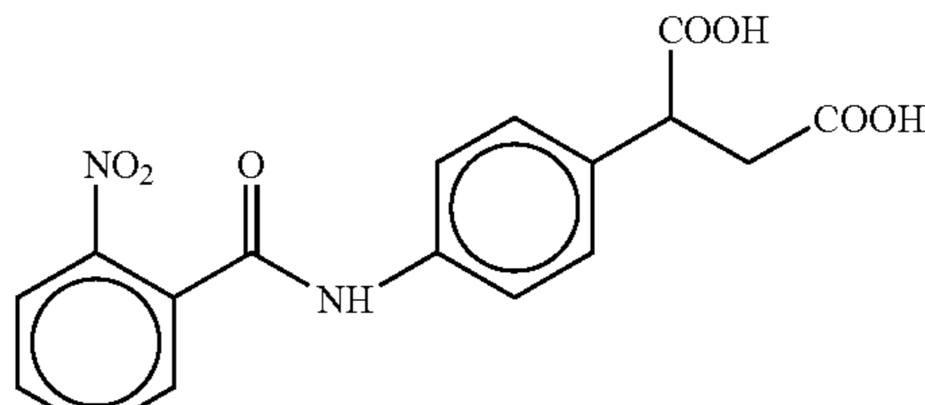
4-(2-Nitrobenzoyl)aminophenylsuccinic acid
