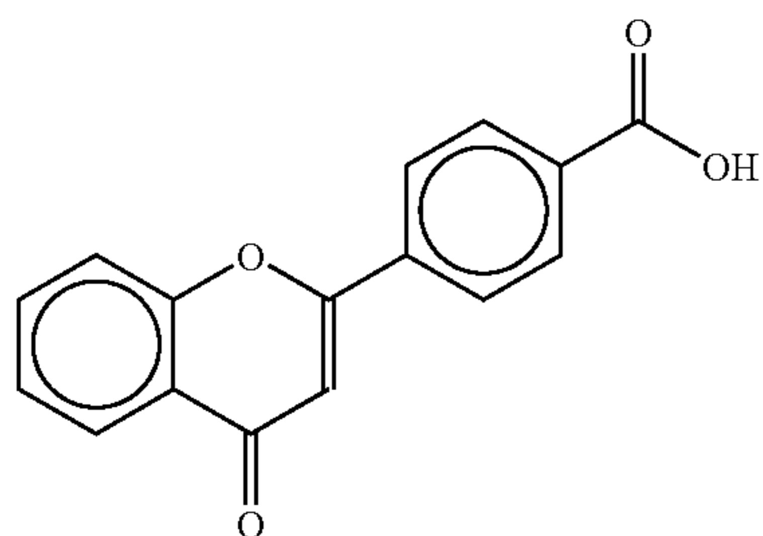
4'-flavonic acid
