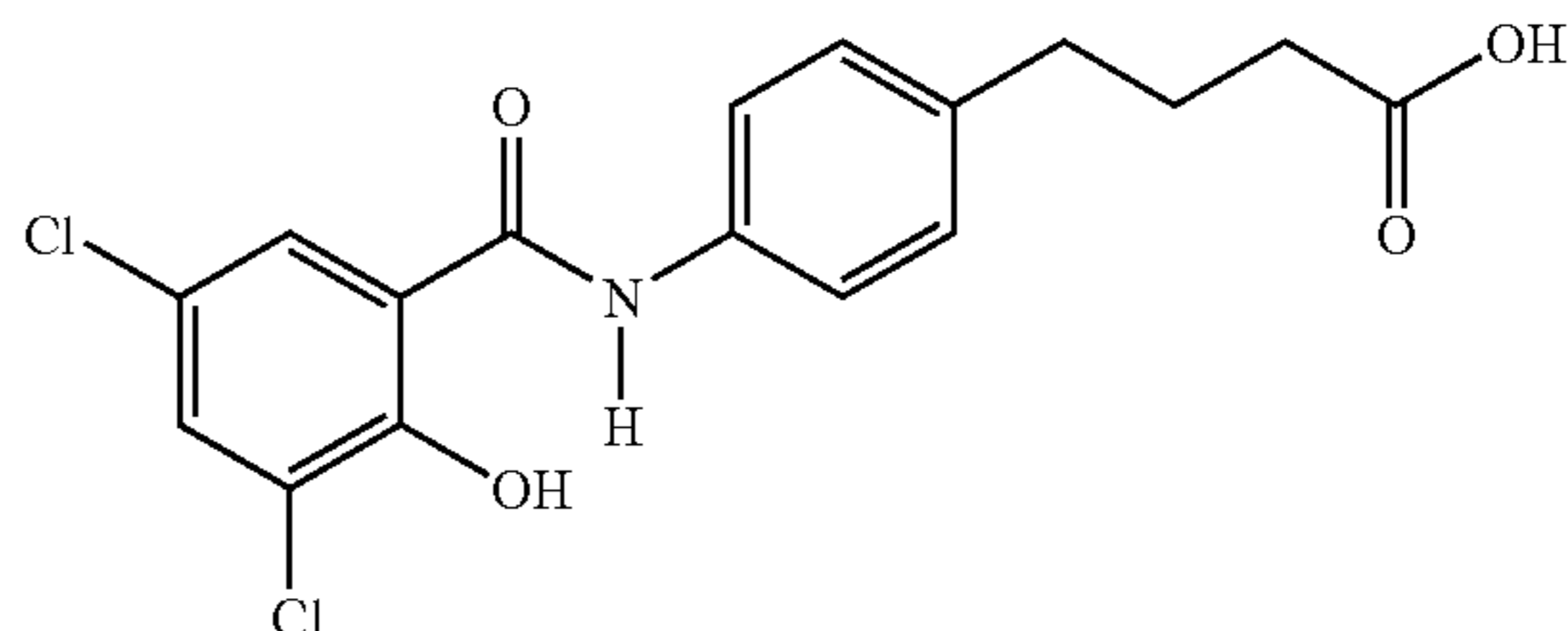
N-[3,5-dichloro-2-hydroxybenzoyl-4-(4-aminophenyl)]butyric acid
