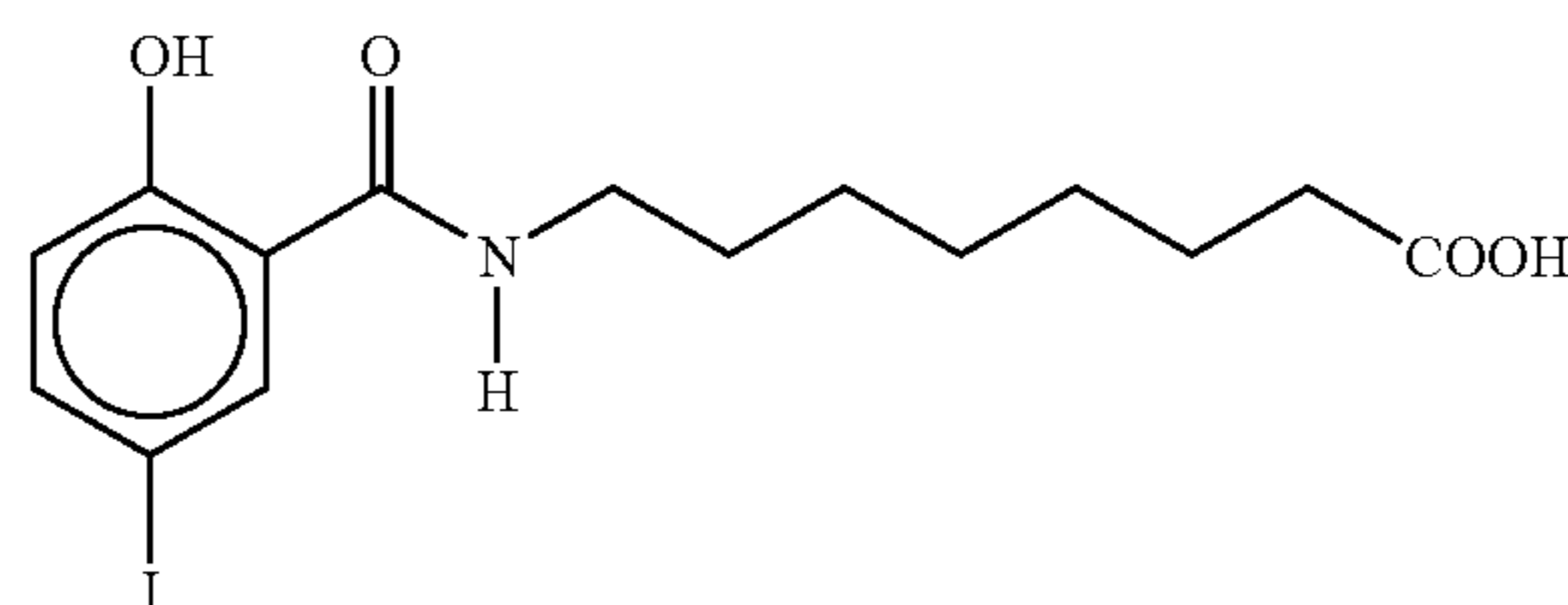
8-(N-(2-hydroxy-5-iodobenzoyl)aminocaprylic acid
