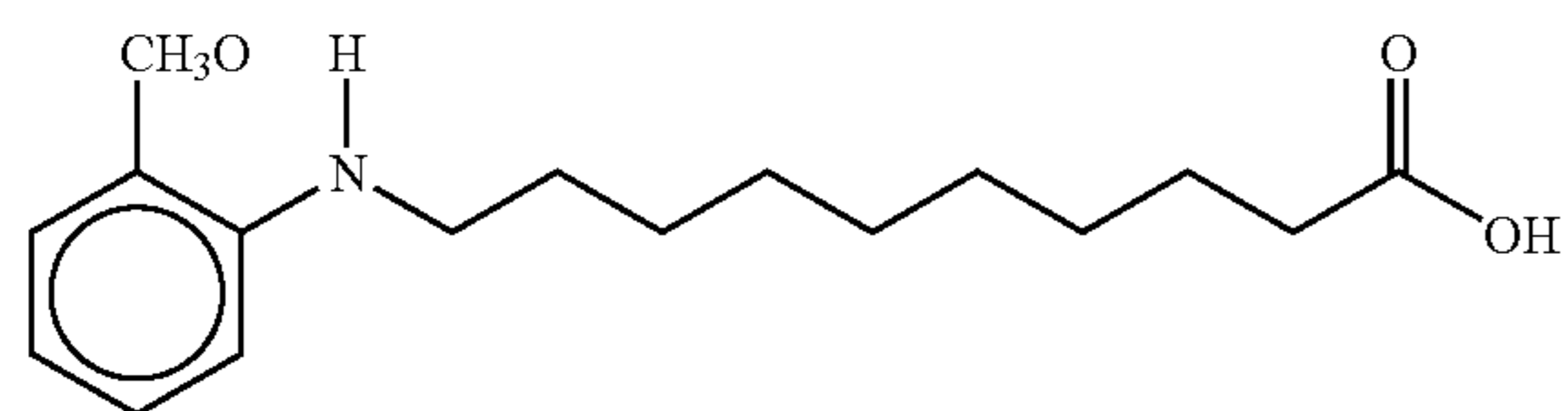
2-Methoxybenzenaminodecanoic acid
