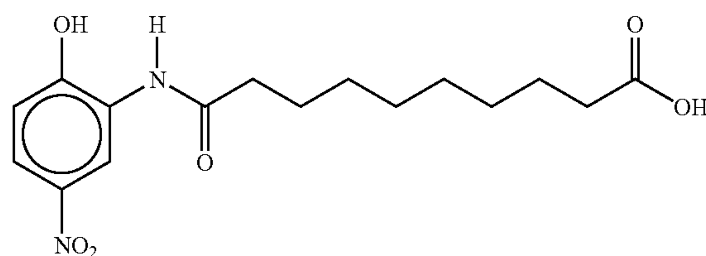
N-10-(2-hydroxy-5-nitroanilino)decanoic acid
