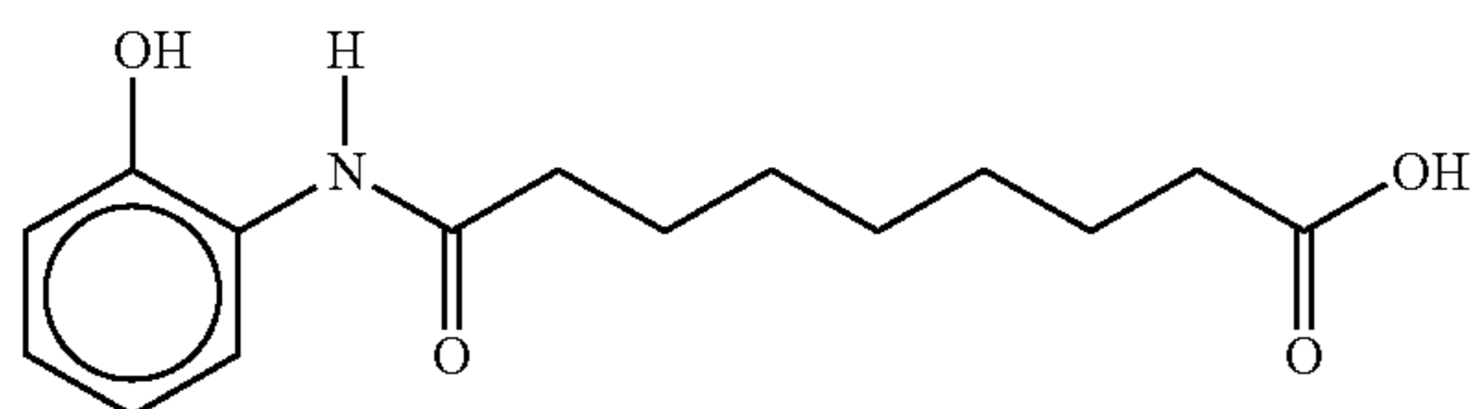
9-(2-hydroxybenzamido)nonanoic acid
