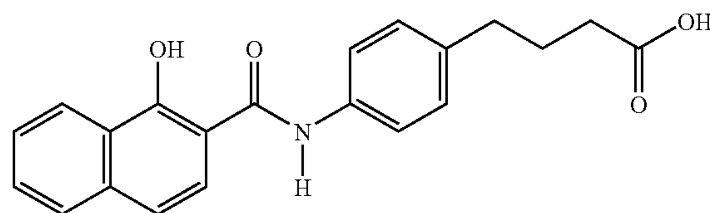
4-{4-[N-(1-hydroxy-2-naphthoyl)]aminophenyl}butyric acid
