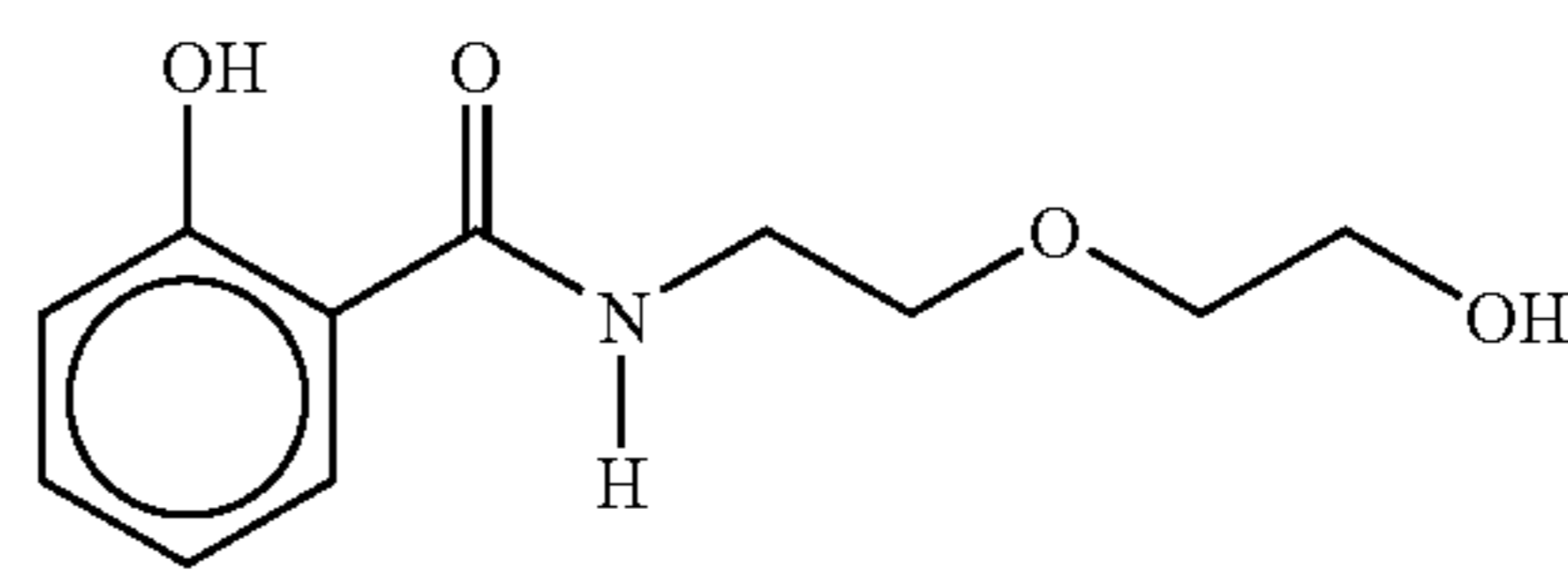
2-[N-(2-hydroxybenzoylamino)ethoxy]ethanol
