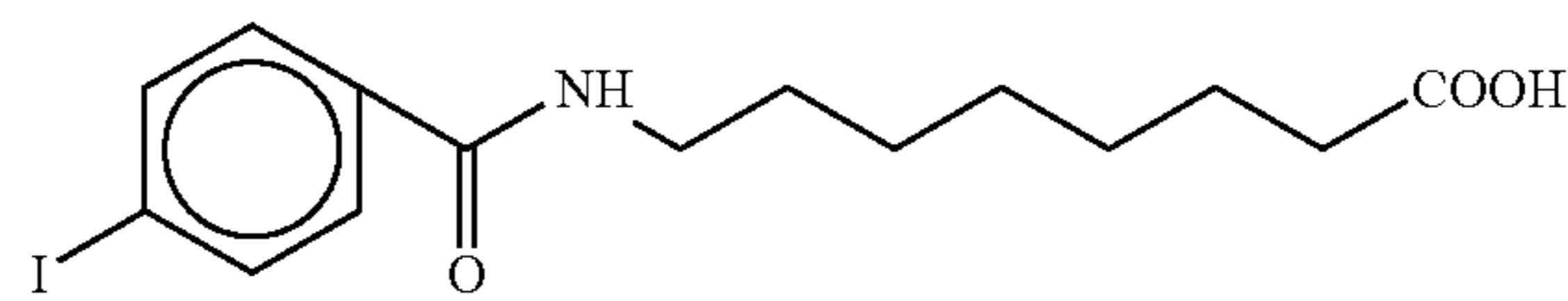
8-[N-(4-iodobenzoyl)]aminocaprylic acid
