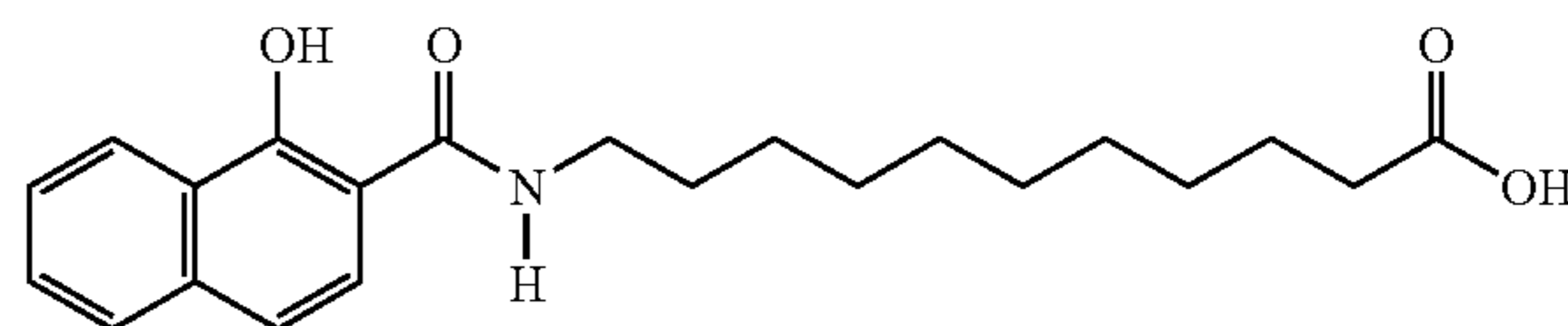
11-N-(1-hydroxy-2-naphthoyl)aminoundecanoic acid
