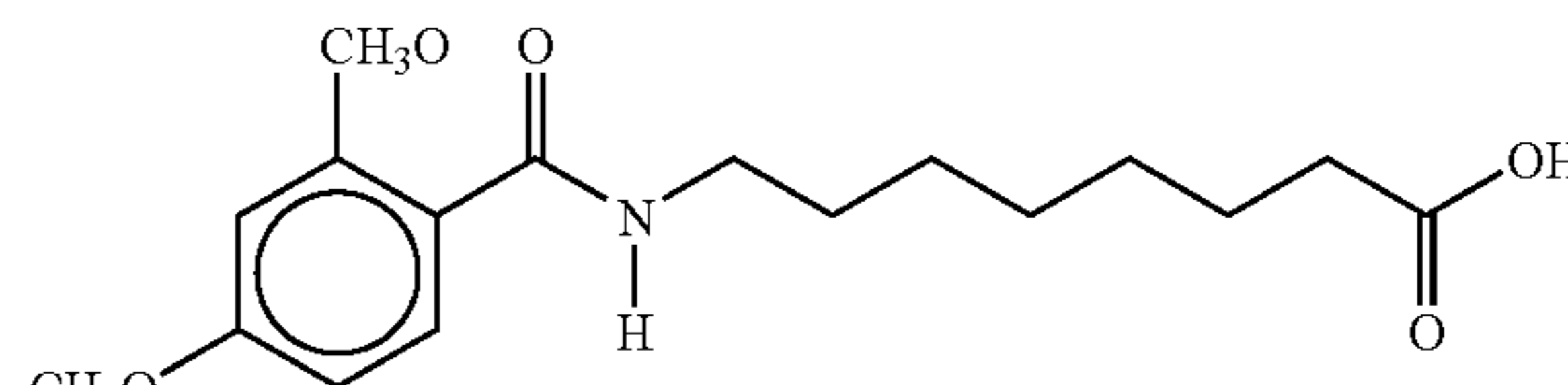
8-(N-(2,4-Dihydroxybenzoyl))aminocaprylic acid
