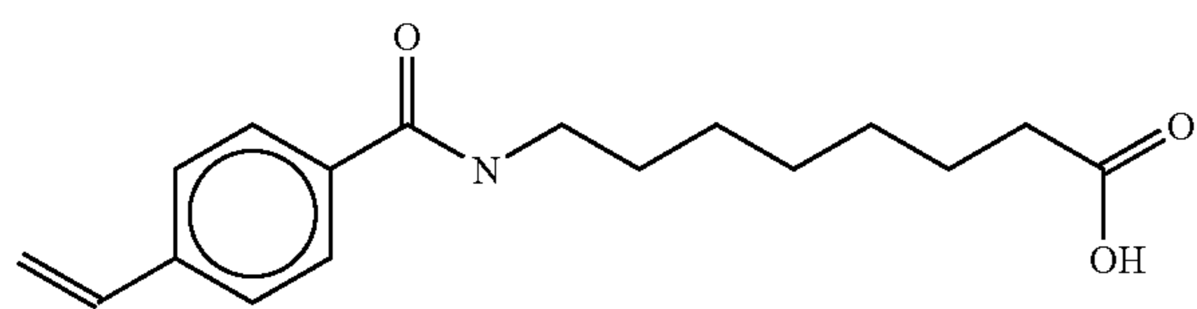
8-(vinylbenzoyl)aminocaprylic acid
