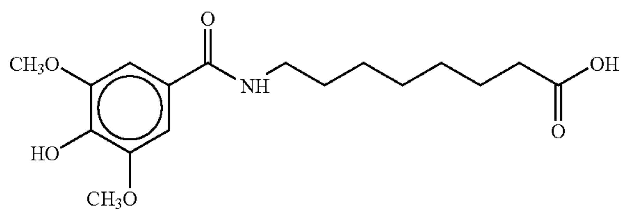
8-(N-3,5-Dimethoxy 4-hydroxybenzoyl)aminocaprylic acid
