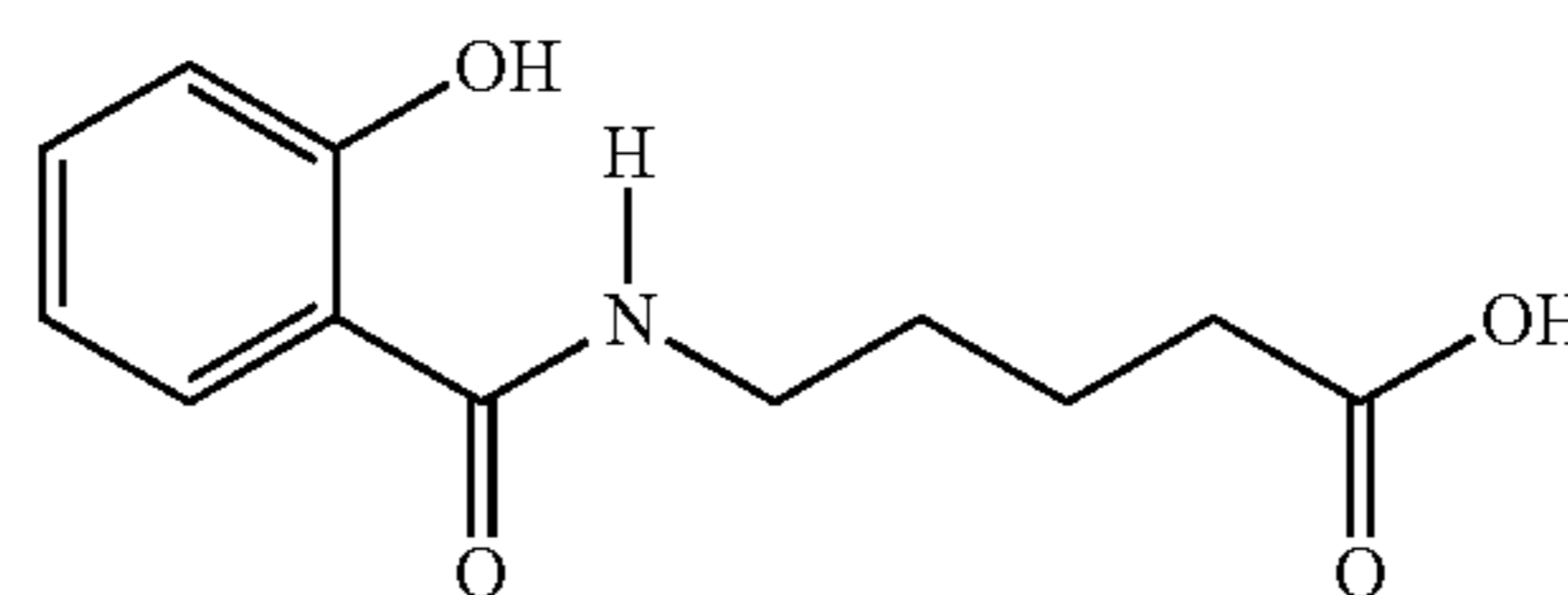
5-(N-salicyloylamino)valeric acid
