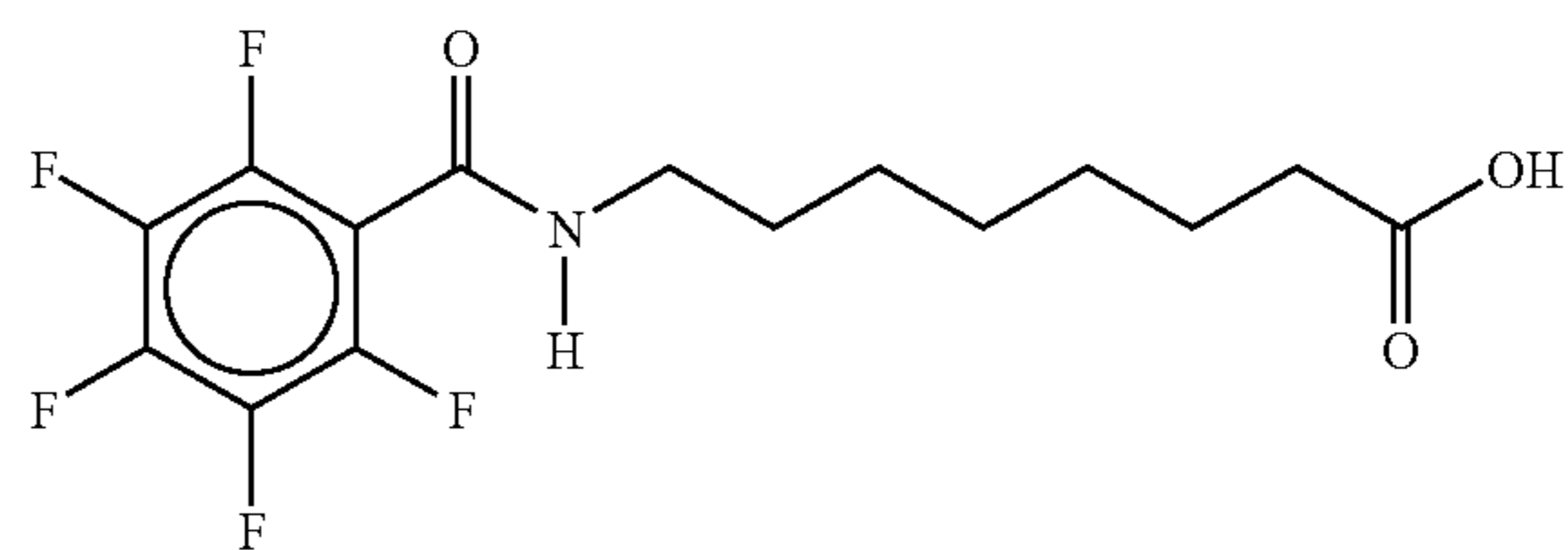
8-(pentafluorobenzoyl)aminocaproic acid
