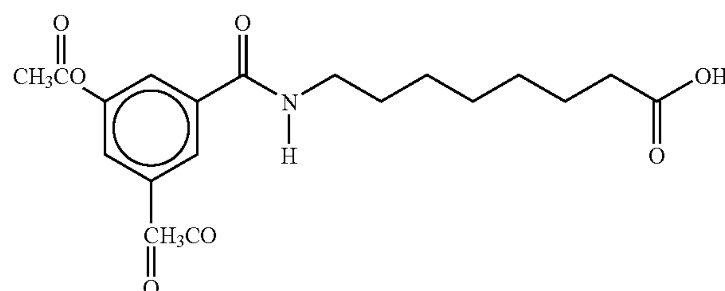
8-(N-(3,5-Diacetyloxybenzoyl))aminocaprylic acid
