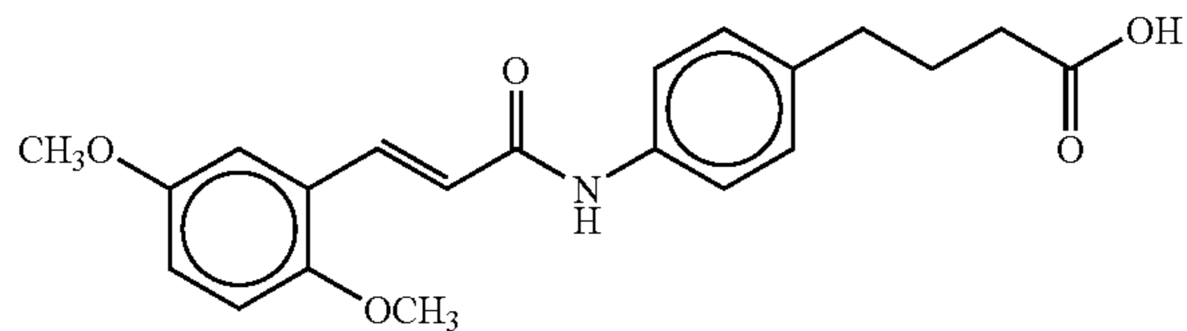
4-(4-(2,5-dimethoxycinnamoyl)aminophenyl)butyric acid
