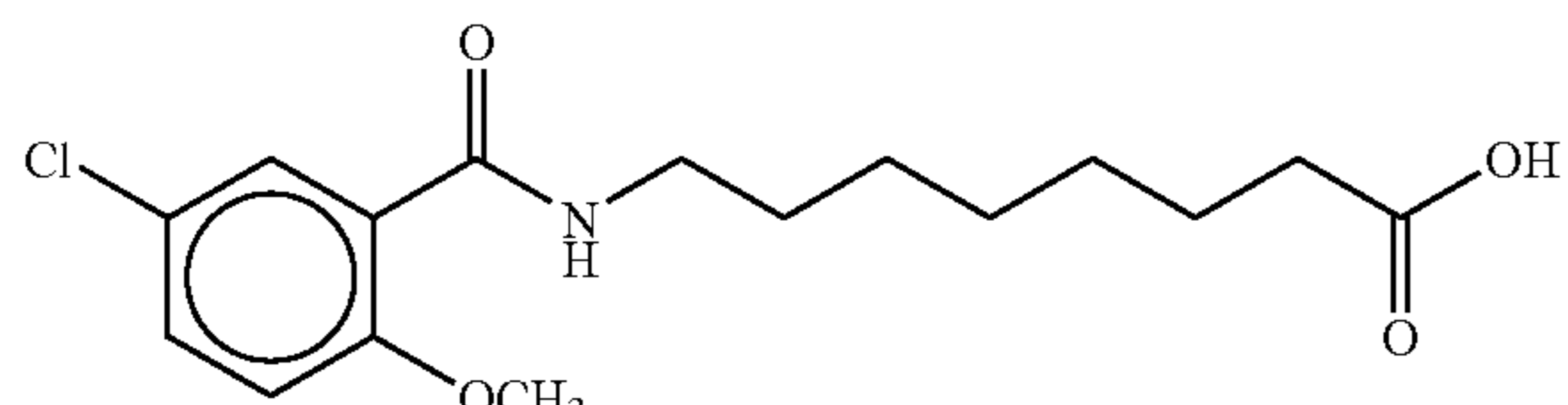
8-(5-chloro-o-anisoyl)aminocaprylic acid
