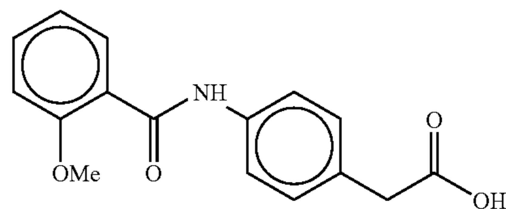
4-(o-anisoyl)aminophenylacetic acid
