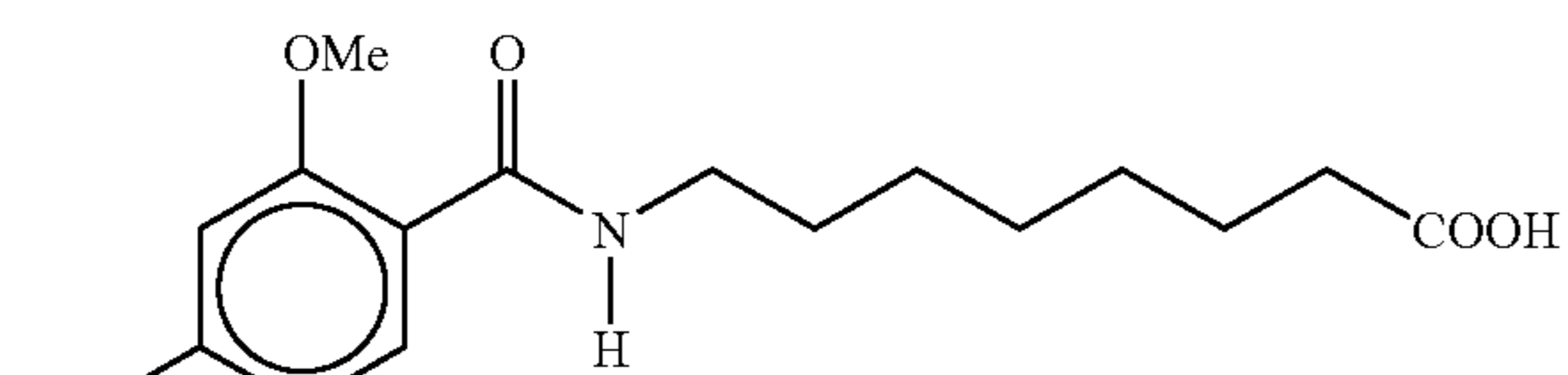
8-N-(2-methoxy-4-nitrobenzoyl)aminocaprylic acid
