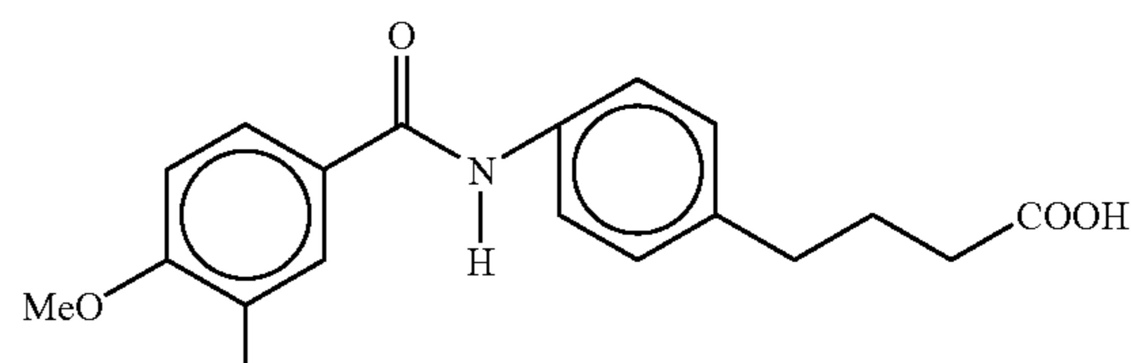
4-[4-N-(4-methoxy-3-nitrobenzoyl)aminophenyl]butyric acid
