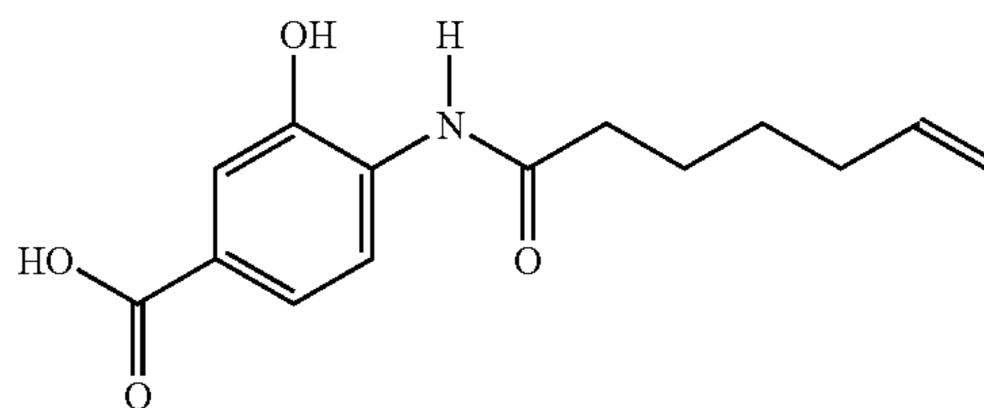
N-(2-hydroxy-4-carboxy)-6-heptenamide
