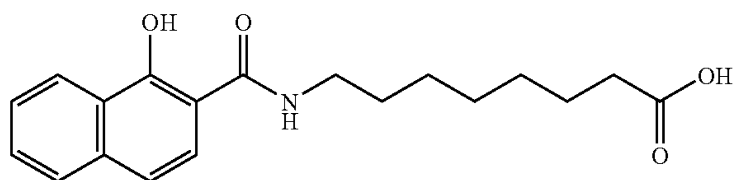
8-(N-(1-hydroxy-2-naphthoyl)aminocaprylic acid
