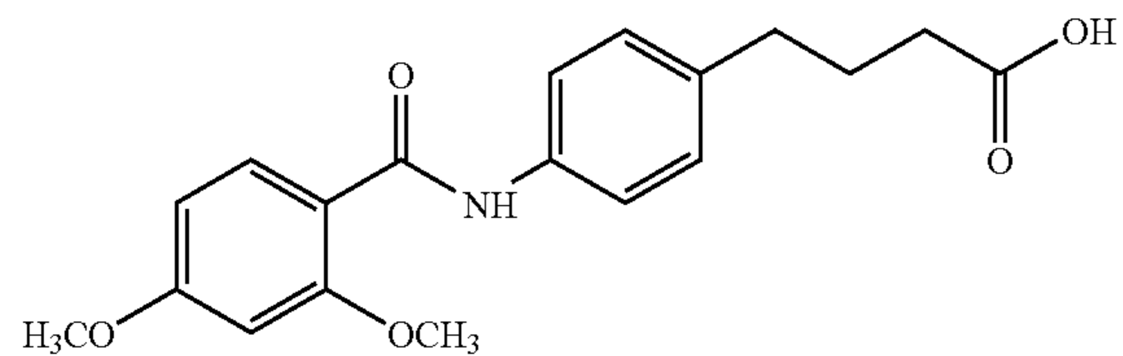
4-(4-(2,4-dimethoxybenzoyl)aminophenyl)butyric acid
