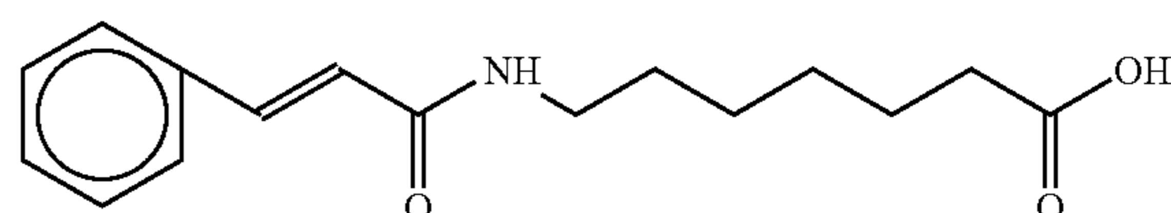
7-cinnamoylaminoheptanoic acid
