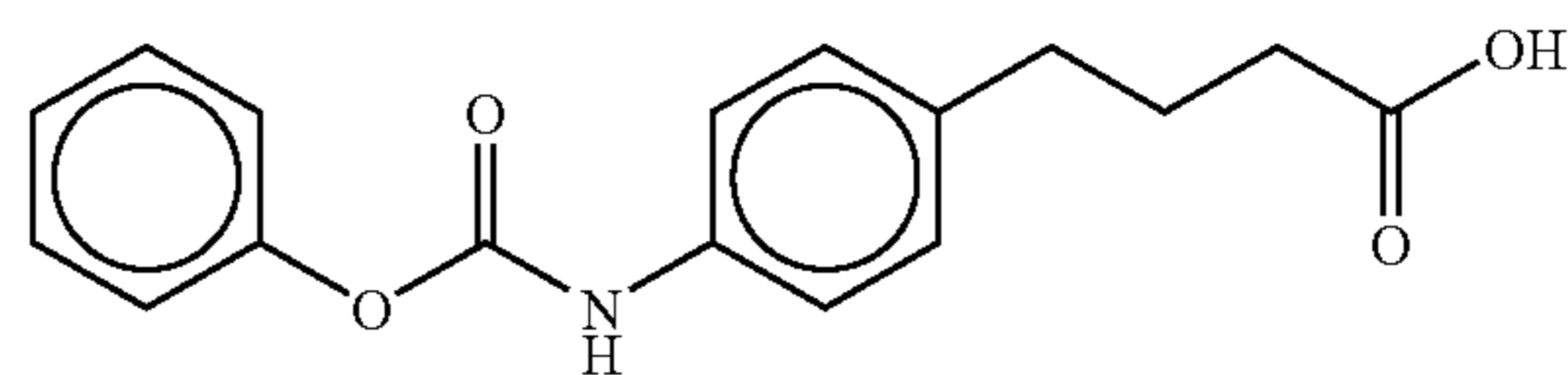
4-(4-phenyloxycarbonylamino)phenylbutyric acid
