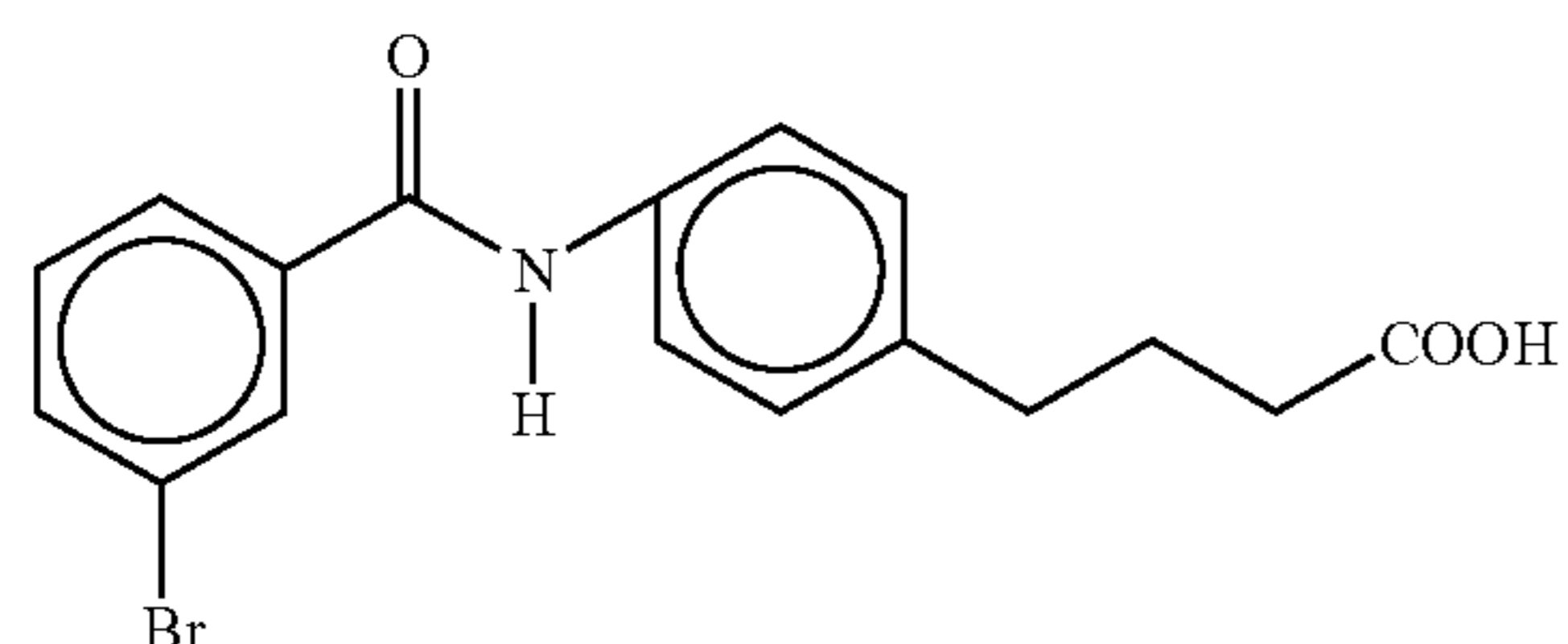
4-{4-[N-(3-bromobenzoyl)aminophenyl]}butyric acid
