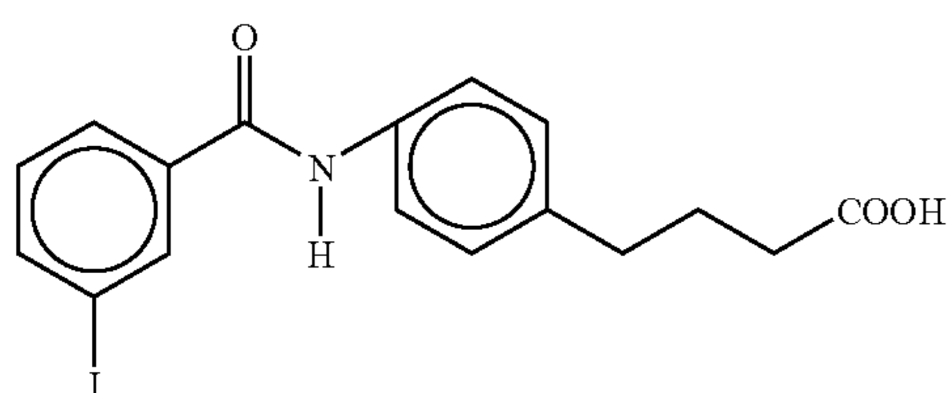
4-(N-[4-(3-iodobenzoyl)aminophenyl])butyric acid
