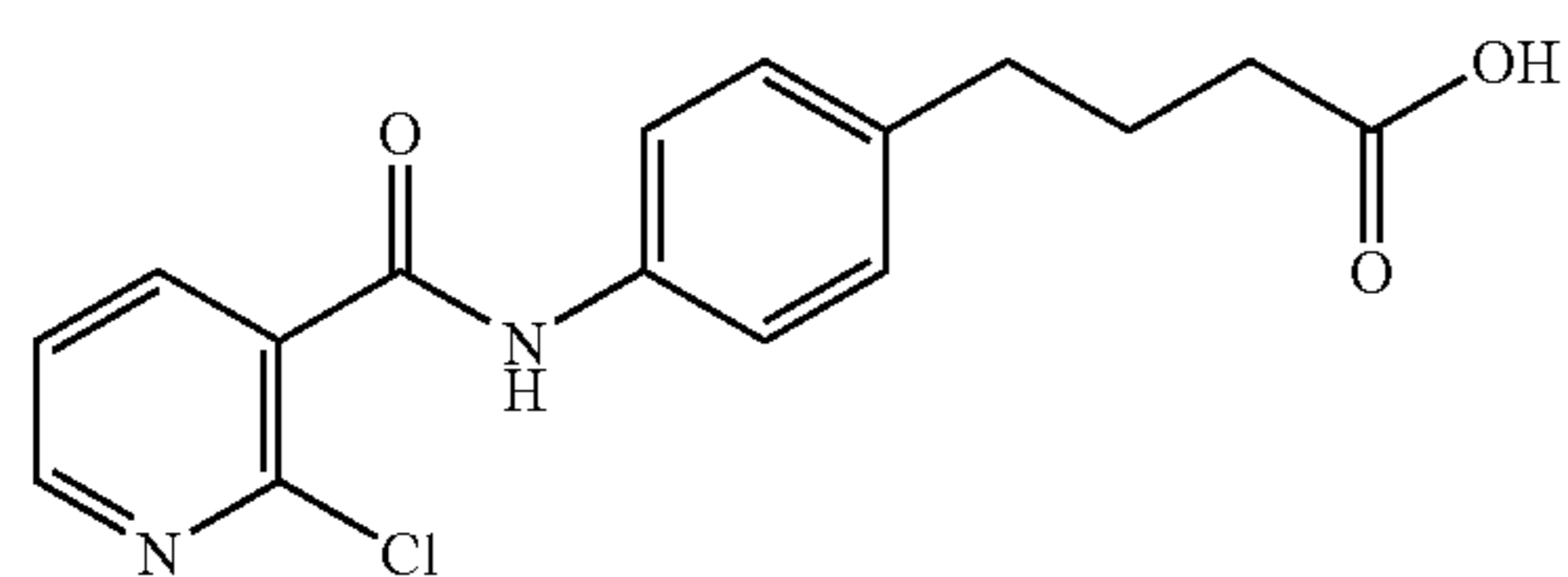
4-(4-(2-chloronicotinoyl)aminophenyl)butyric acid
