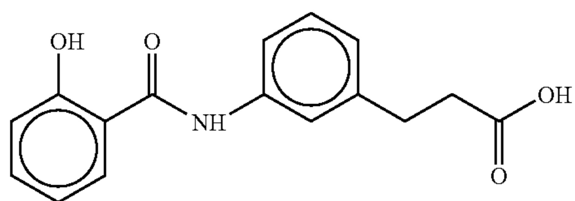
3-(3-(salicyloyl)aminophenyl)propionic acid
