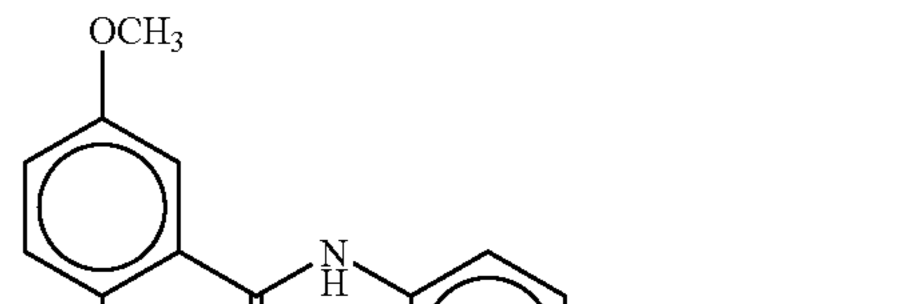
4-(4-(4-chloro-o-anisoyl)aminophenyl)butyric acid
