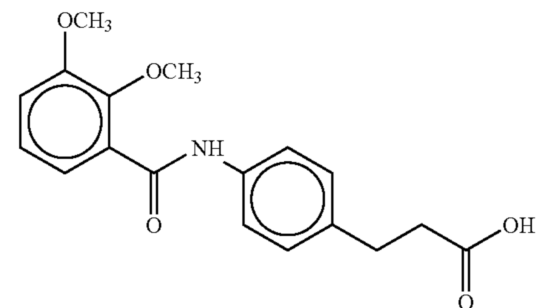
3-[4-(2,3-dimethoxybenzoyl)aminophenyl]propionic acid
