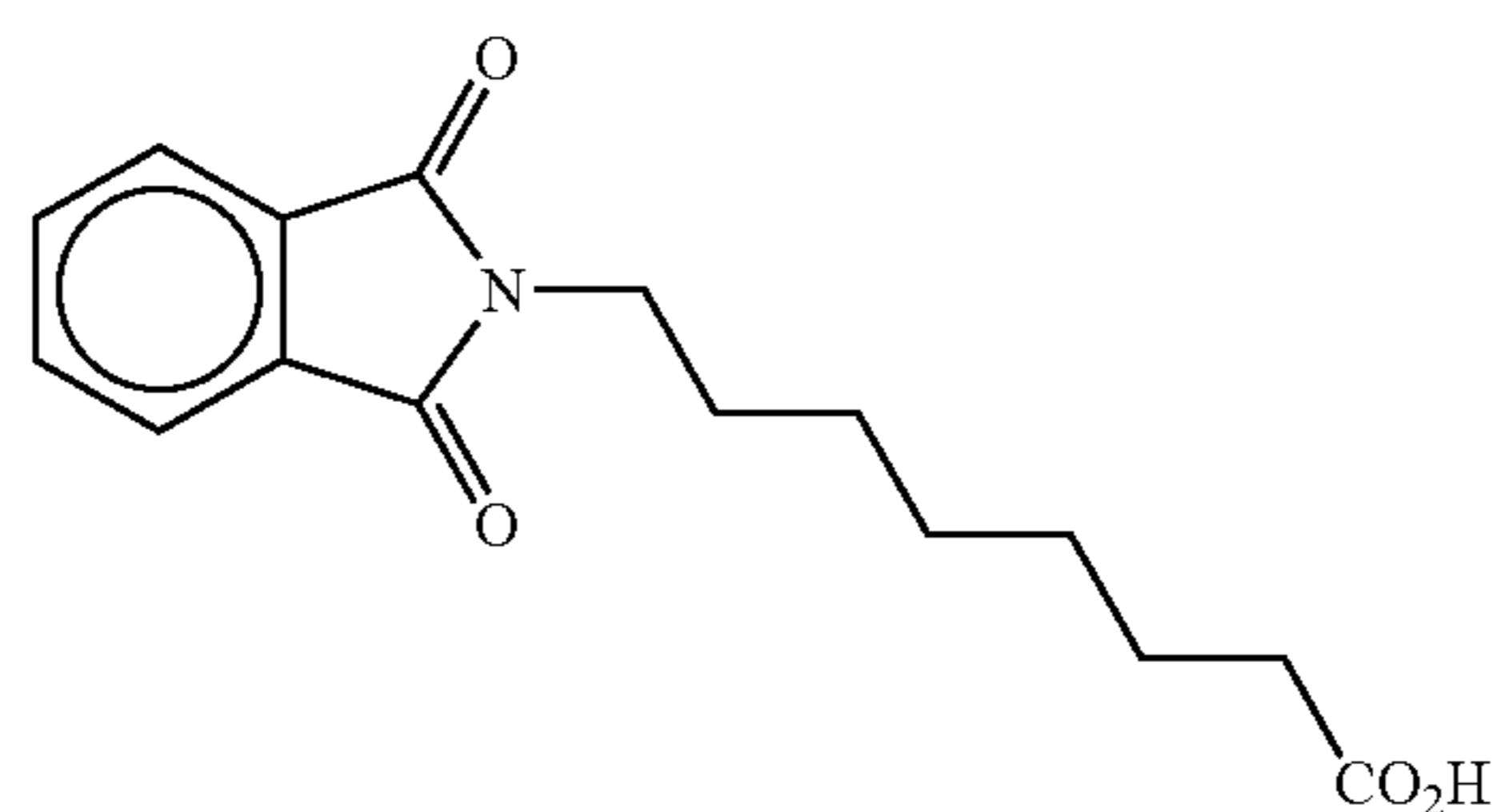
8-(phthalimido)caprylic acid
