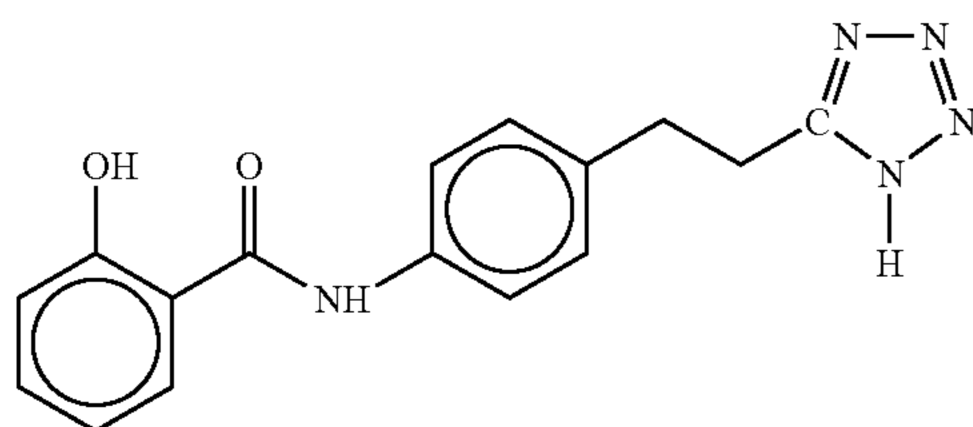
4-(Salicyloyl)aminophenylethyltetrazole
