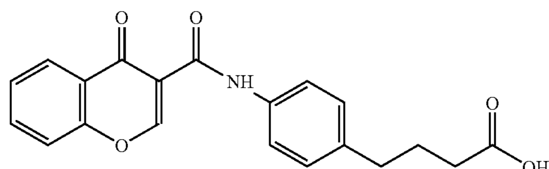
4-(4-(chromone-3-carbonyl)aminophenyl)butyric acid
