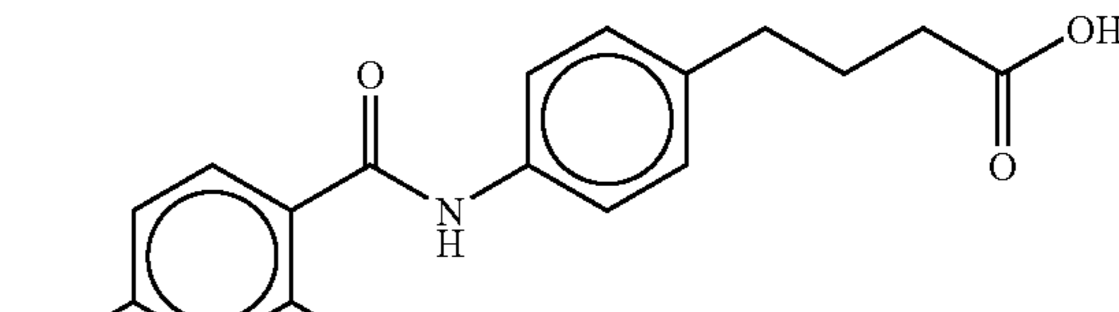
4-(4-(4-chloro-o-anisoyl)aminophenyl)butyric acid
