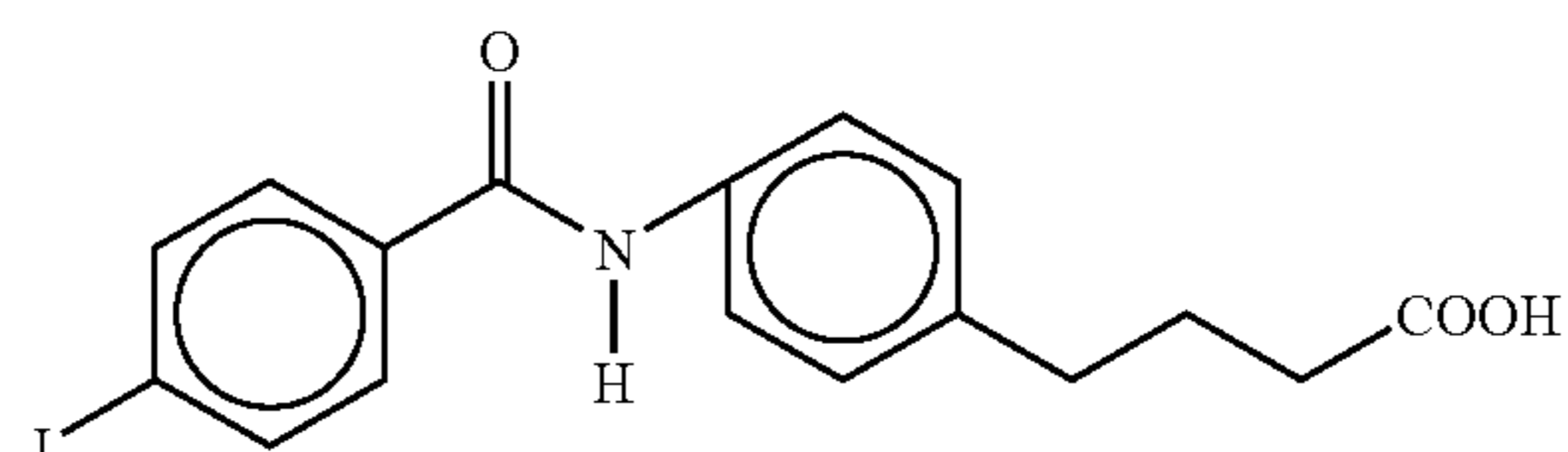
4-{4-[N-(4-iodobenzoyl)]aminophenyl}butyric acid
