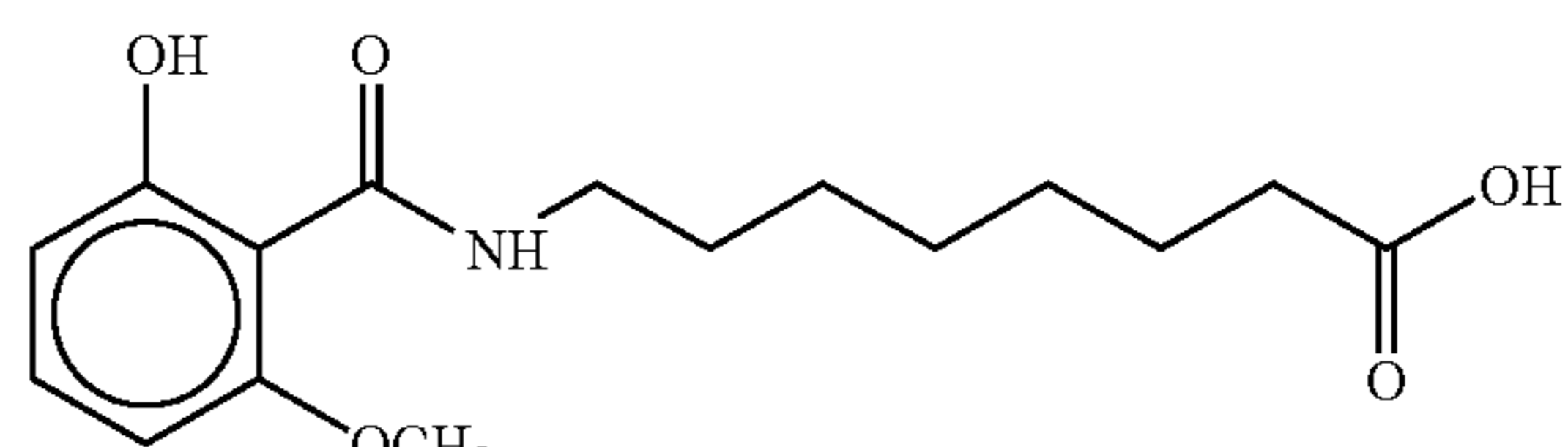
8-(N-2-Hydroxy-6-methoxybenzoyl)aminocaprylic acid
