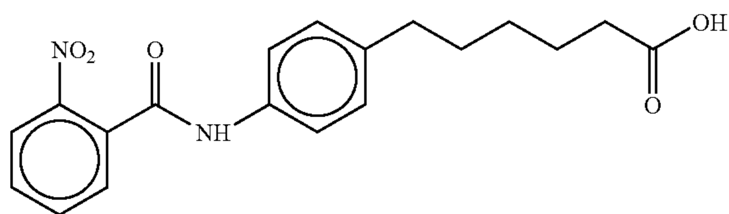
6-(4-(N-2-Nitrobenzoyl)aminophenyl)hexanoic acid
