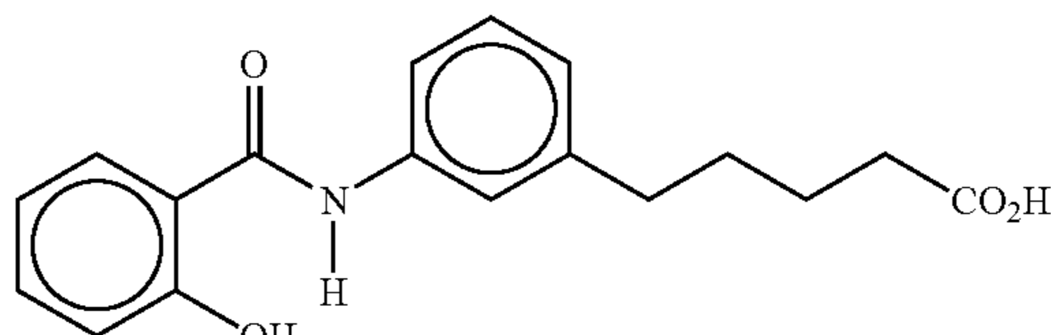
N-Salicyloyl-5-(3-aminophenyl)valeric acid
