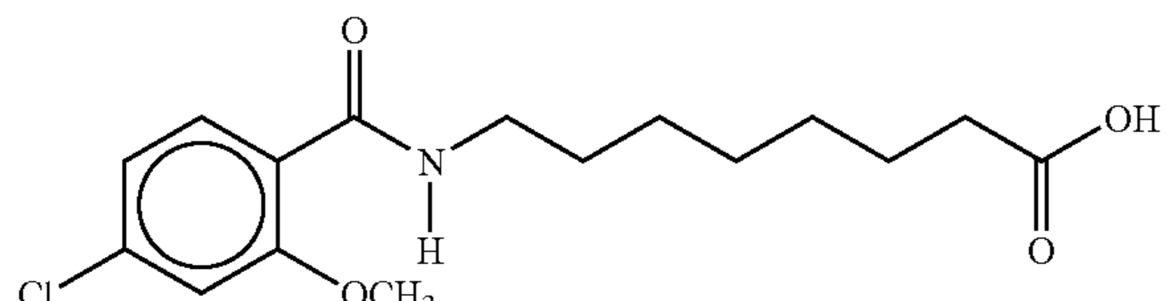
8-(4-chloro-o-anisoyl)aminocaprylic acid
