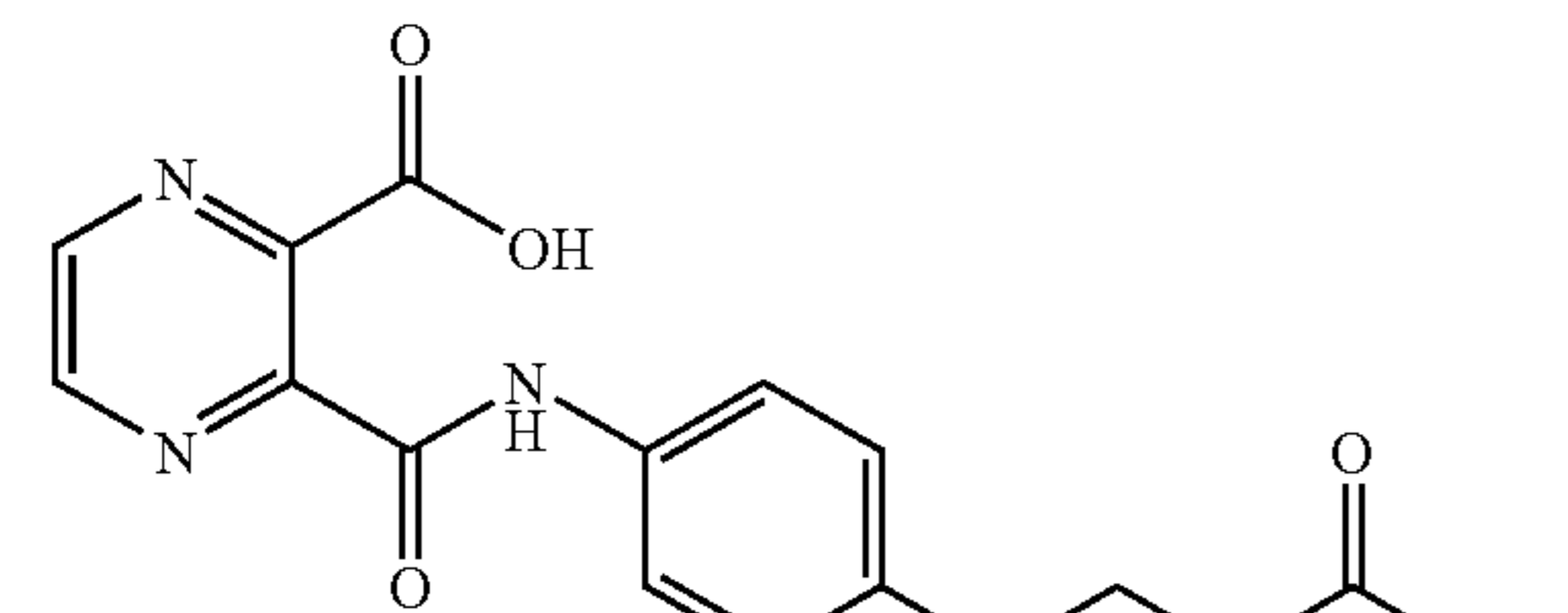
4-(4-(2-(3-carboxyl)pyrazinecarbonyl)aminophenyl)butyric acid
