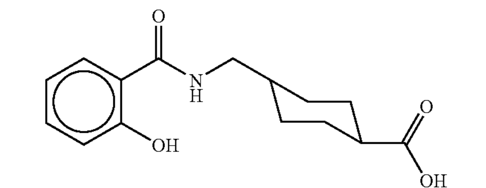
trans-4-(N-salicyloylaminomethyl)cyclohexane carboxylic acid
