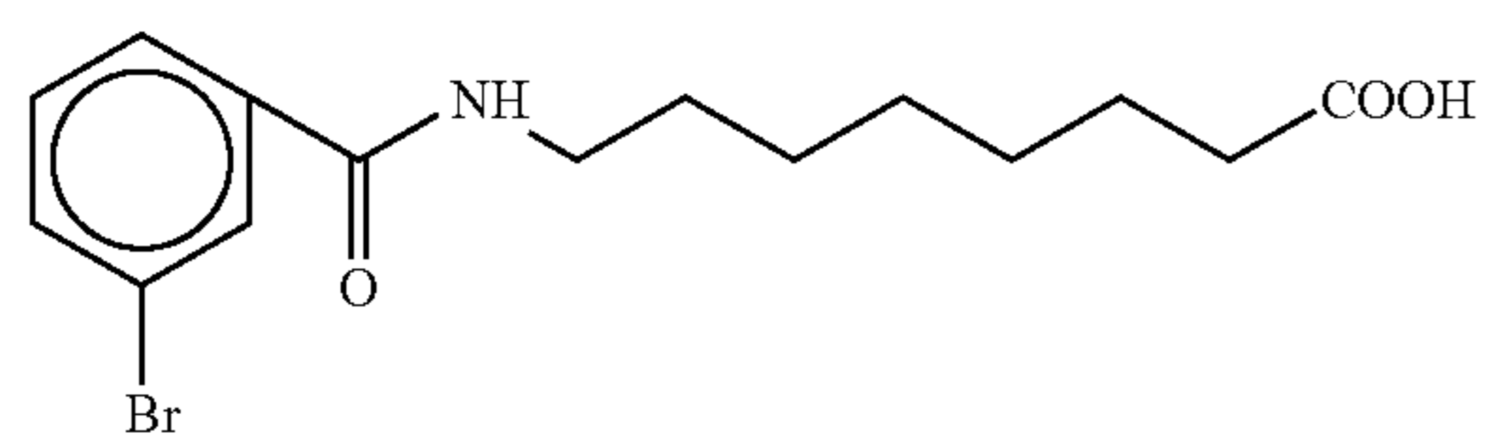
8-[N-(3-bromobenzoyl)]aminocaprylic acid
