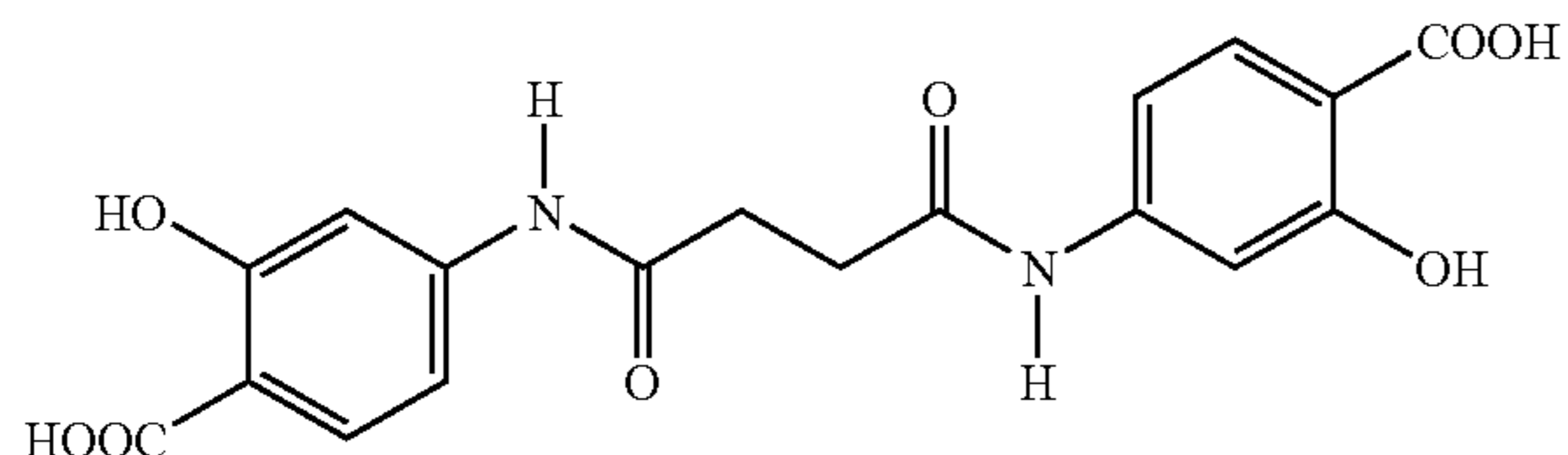
Succinyl-4-aminosalicylic acid
