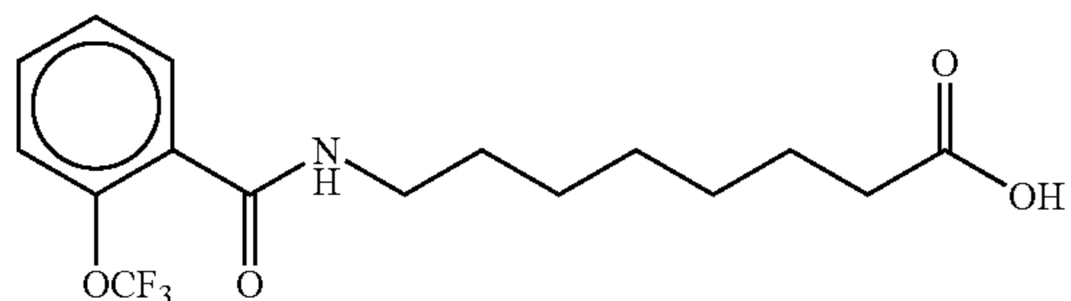
8-(2-(trifluoromethoxy)benzoyl)aminocaprylic acid
