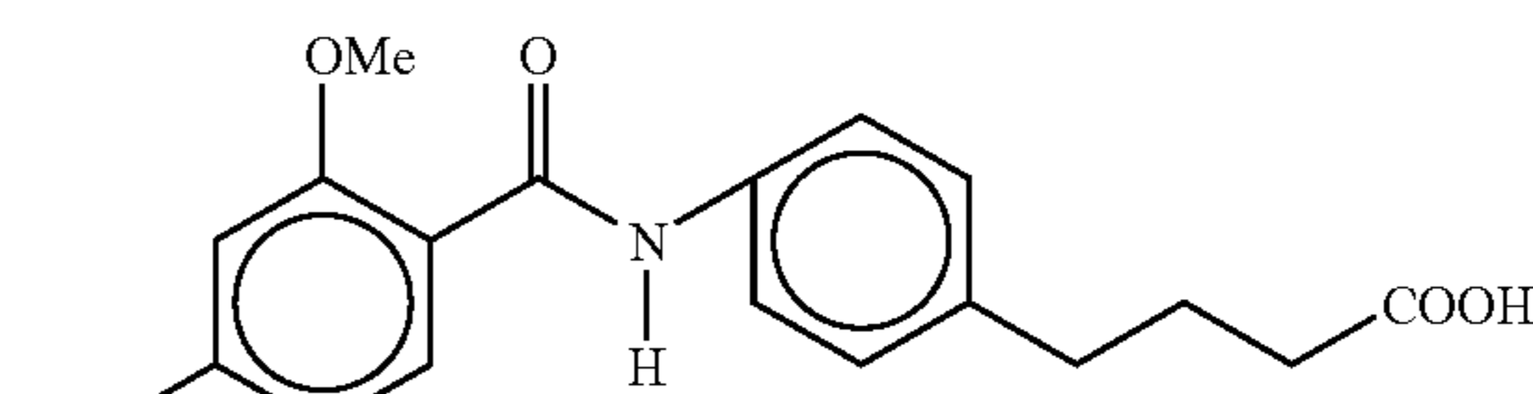
4-{N-[4-(2-methoxy-4-nitrobenzoyl)aminophenyl]}butyric acid
