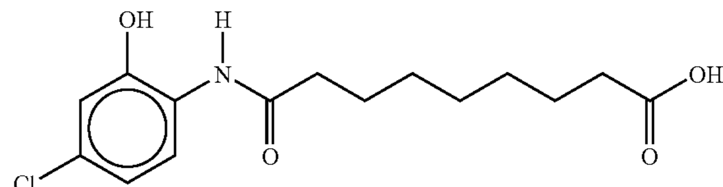
8-(2-hydroxy-5-chloroanilino)octanoic acid
