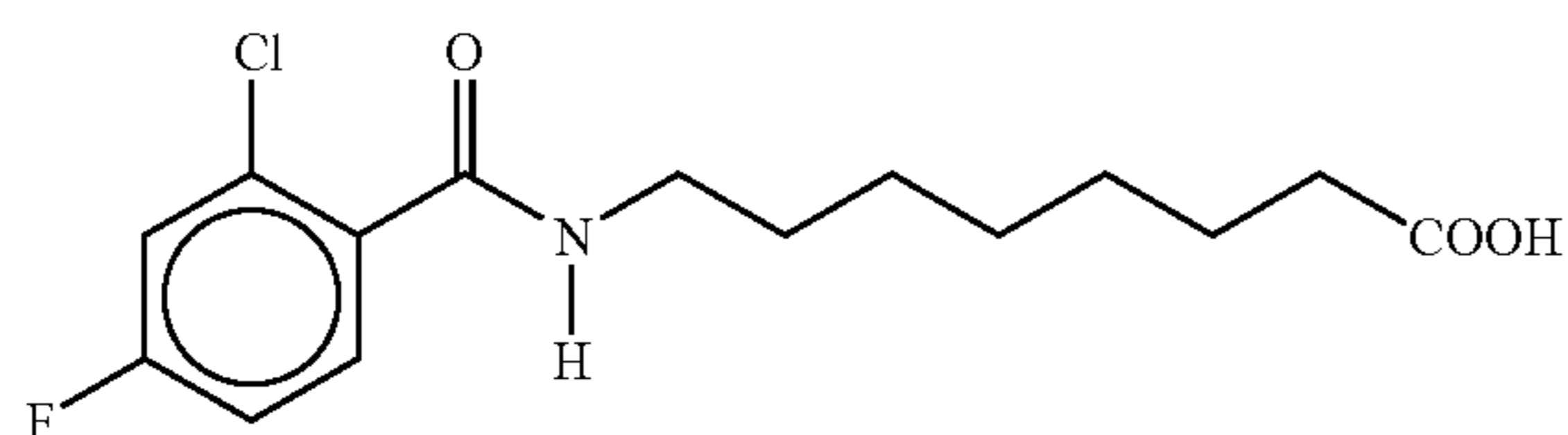
8-(N-(2-chloro-4-fluorobenzoyl)aminocaprylic acid
