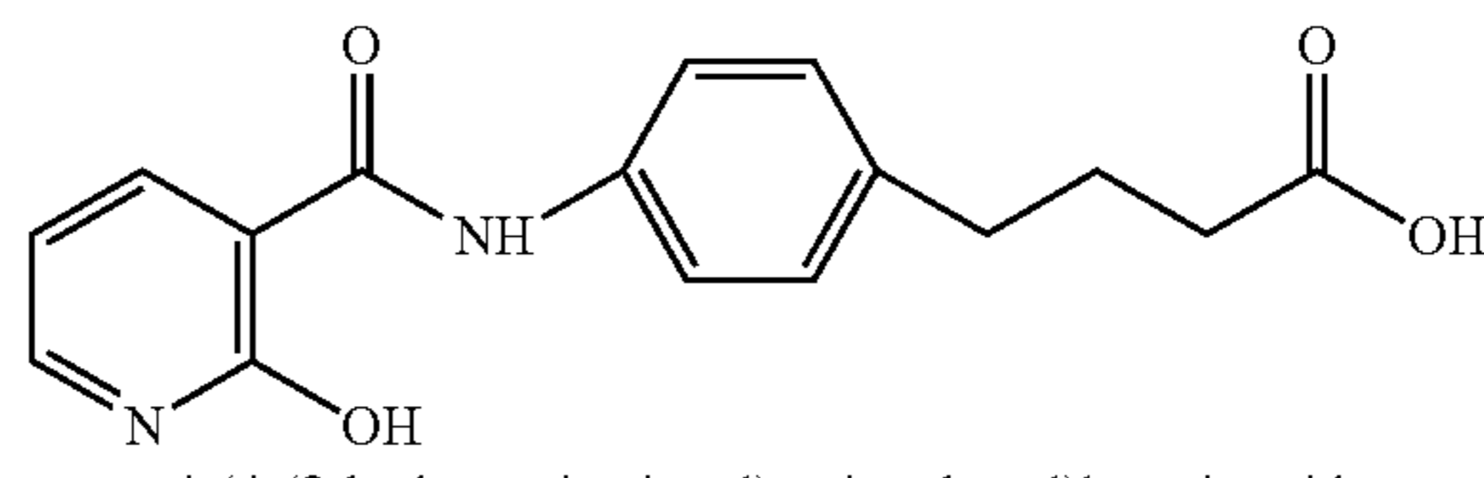
4-(4-(2-hydroxynicotinoyl)aminophenyl)butyric acid
