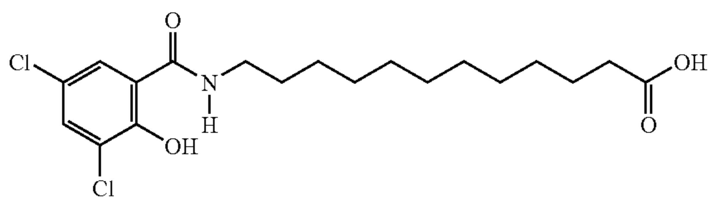
12-N-(3,5-dichloro-2-hydroxybenzoyl)aminododecanoic acid
