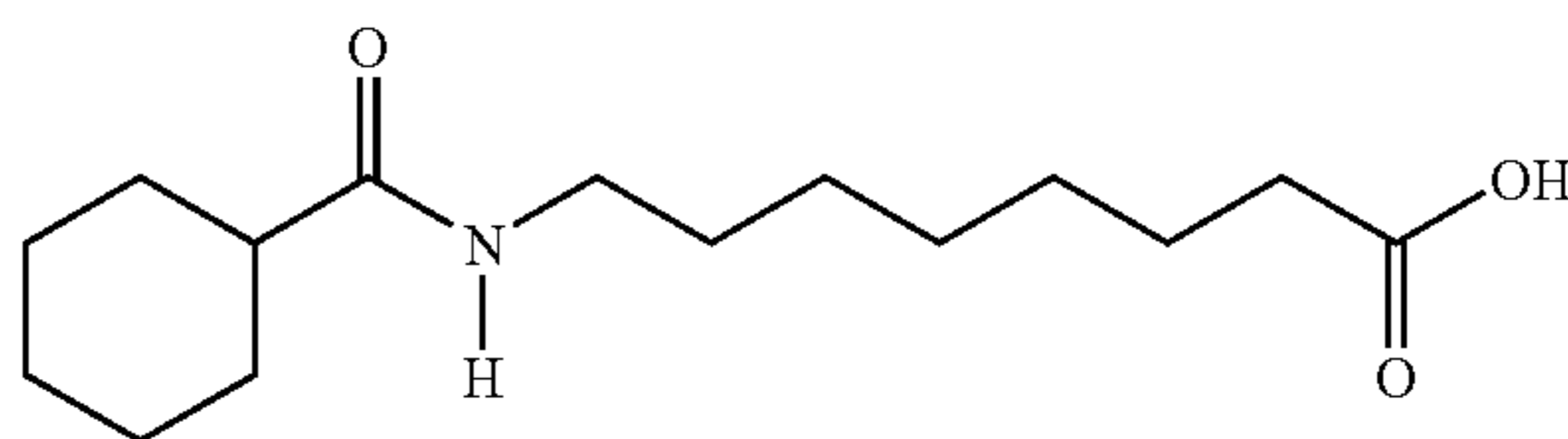
8-N-cyclohexanoylaminocaprylic acid
