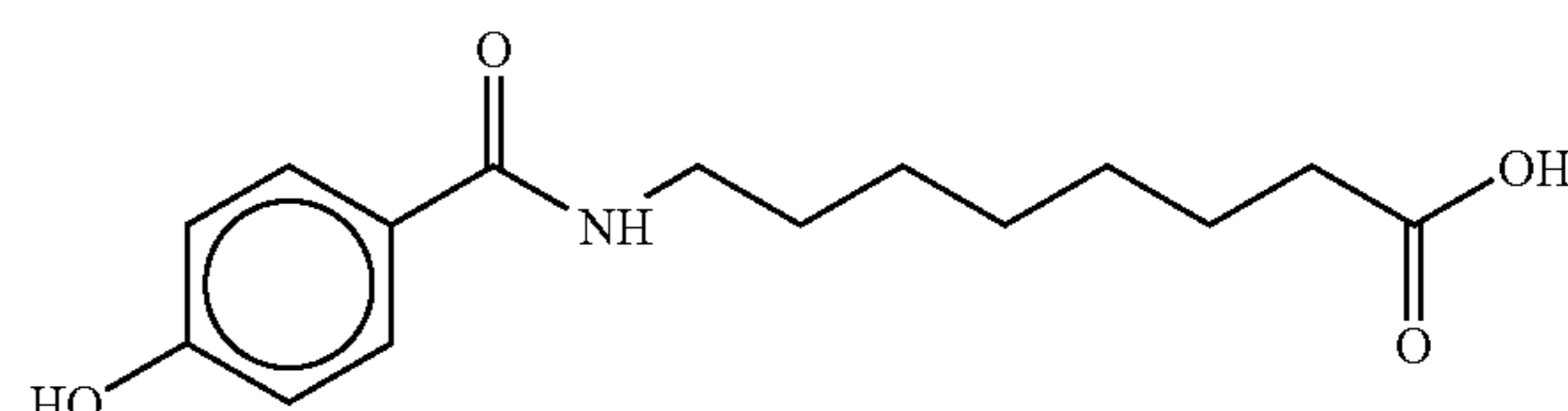
8-(4-Hydroxybenzoyl)aminocaprylic acid
