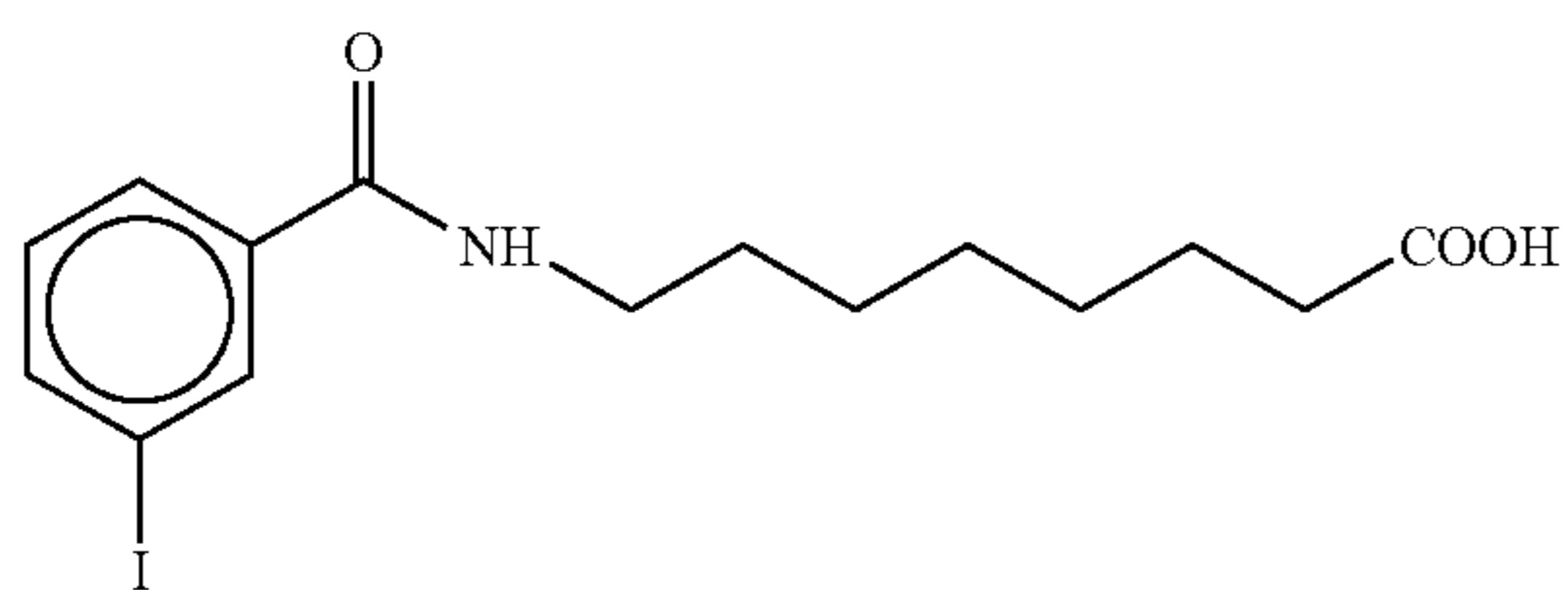
8-N-(3-iodobenzoyl)aminocaprylic acid
