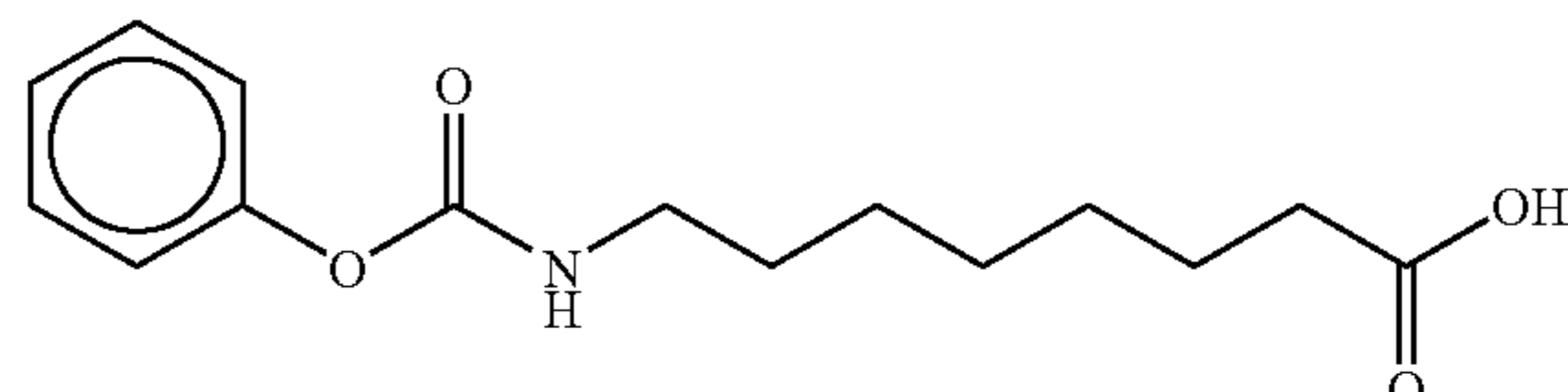
8-(phenylcarbonylamino)caprylic acid
