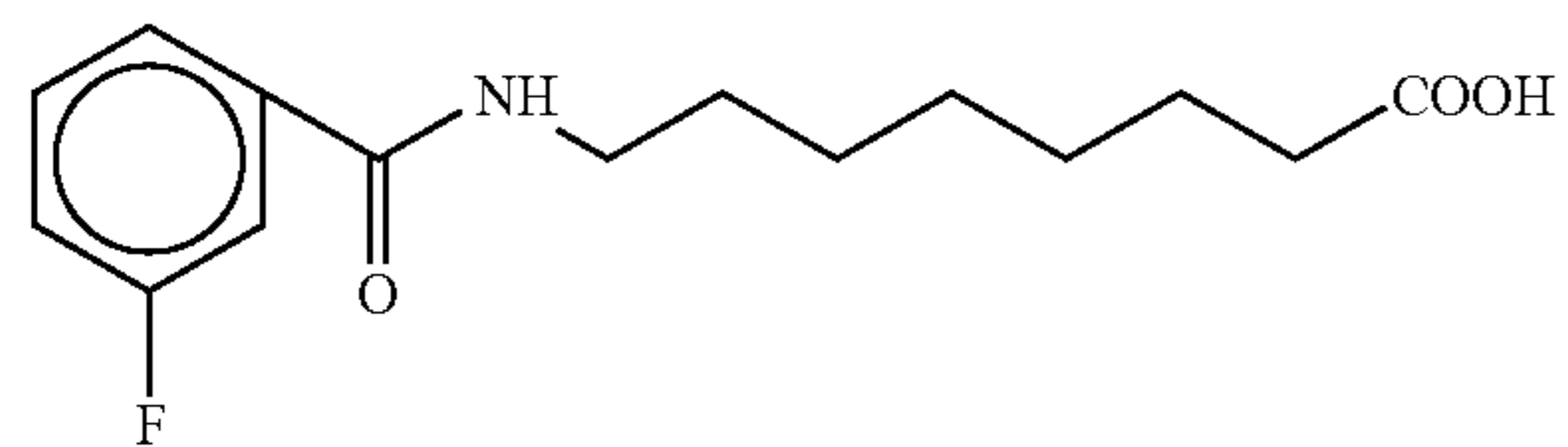
8-[N-(3-fluorobenzoyl)]aminocaprylic acid
