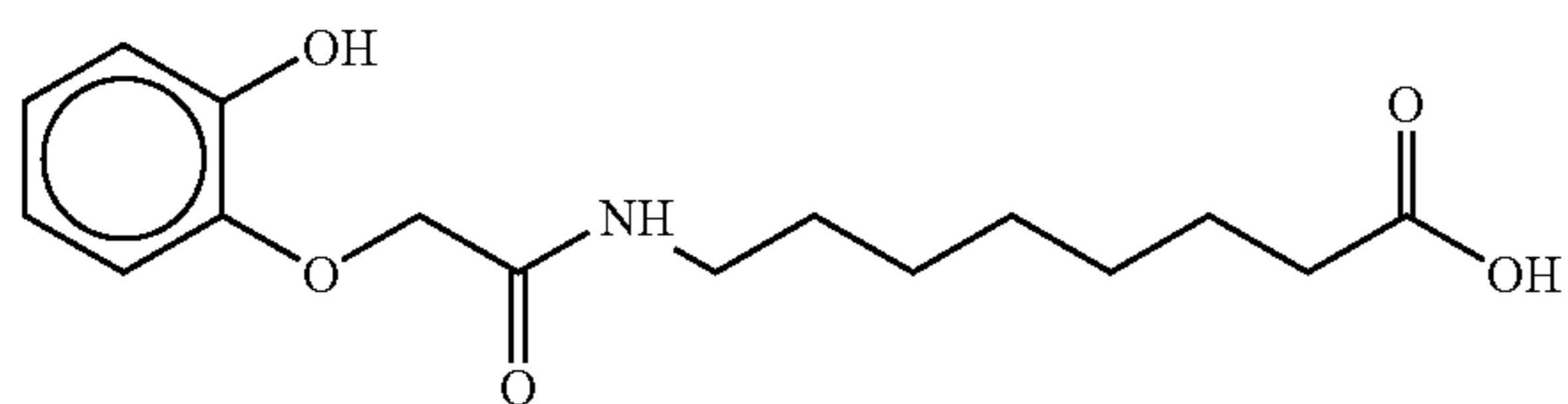
7-(2-hydroxyphenoxyacetyl)aminocaproic acid
