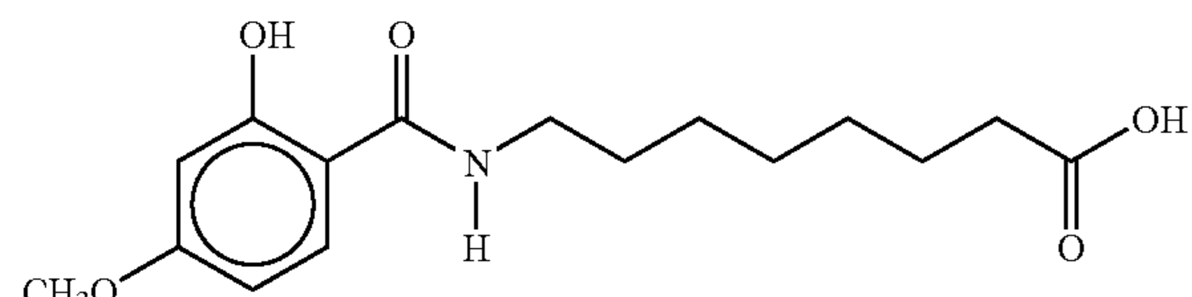
8-(N-(2-Hydroxy-4-methoxybenzoyl))aminocaprylic acid
