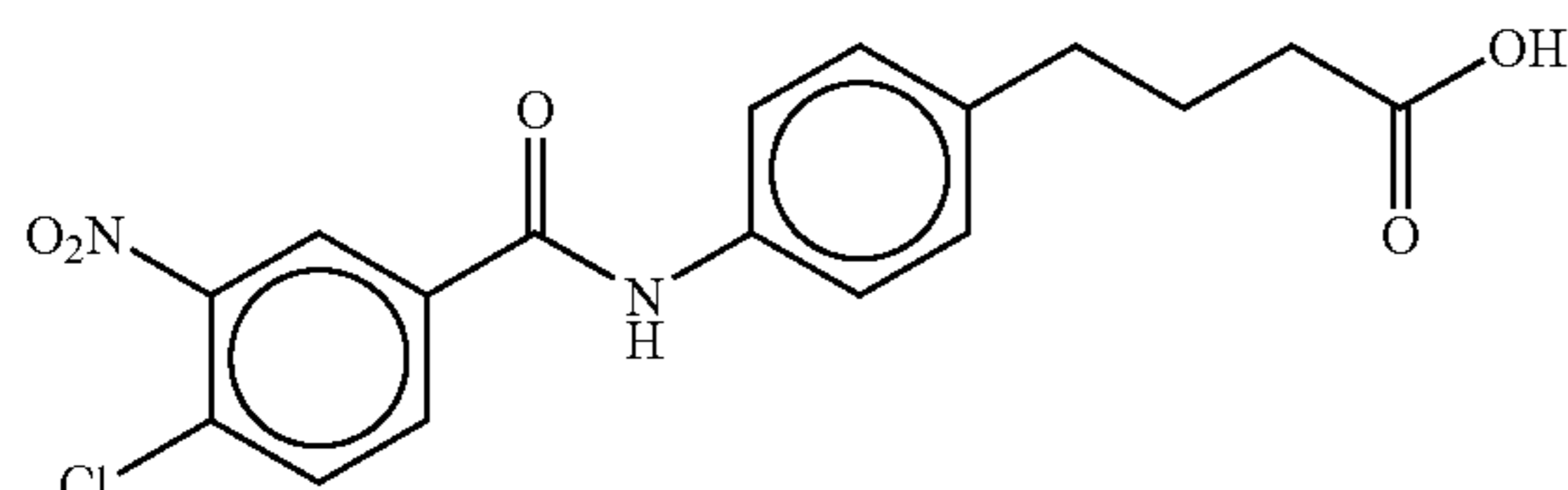
4-(4-(4-chloro-3-nitrobenzoyl)aminophenyl)butyric acid
