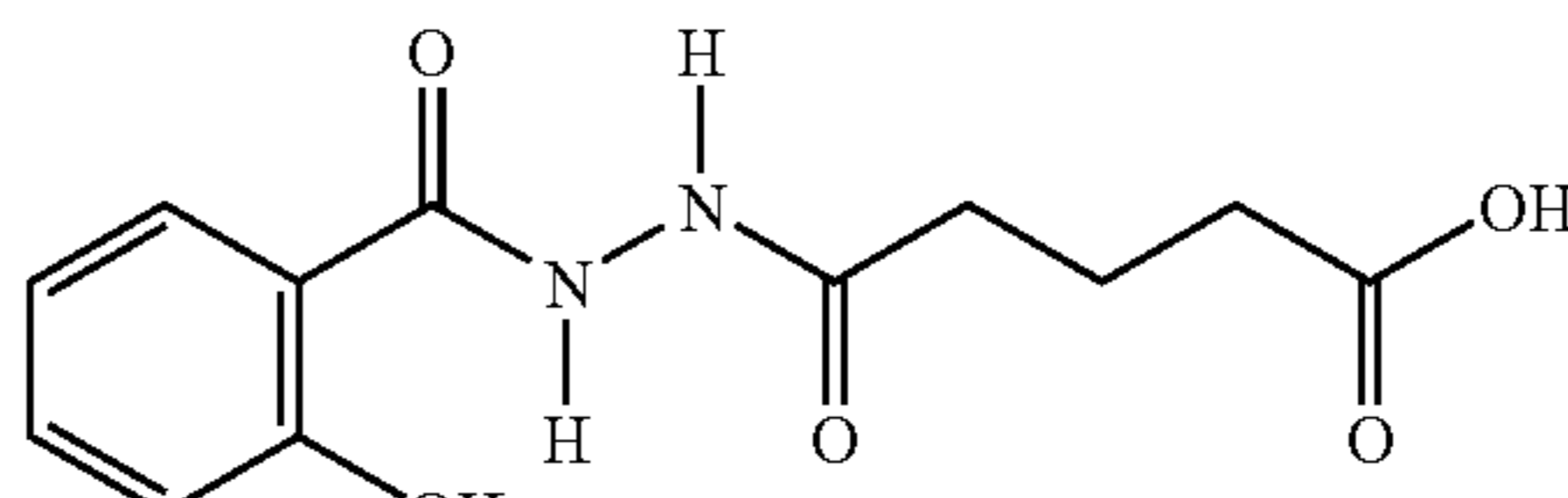
1-salicyloyl-2-glutaryl hydrazide
