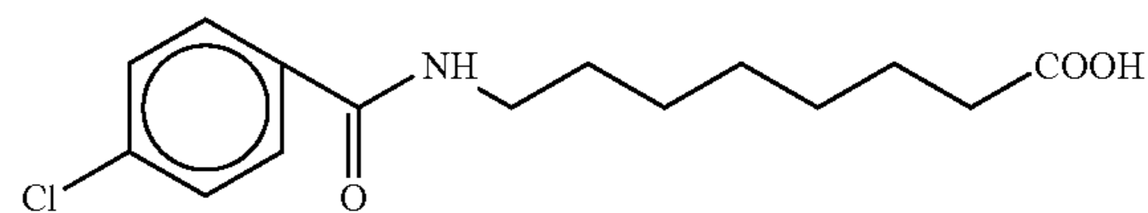
8-[N-(4-chlorobenzoyl)]aminocaprylic acid
