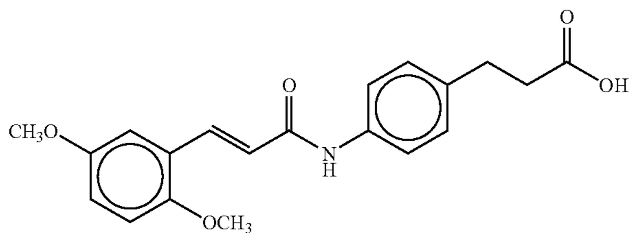
3-(4-(2,5-dimethoxycinnamoyl)aminophenyl)propionic acid
