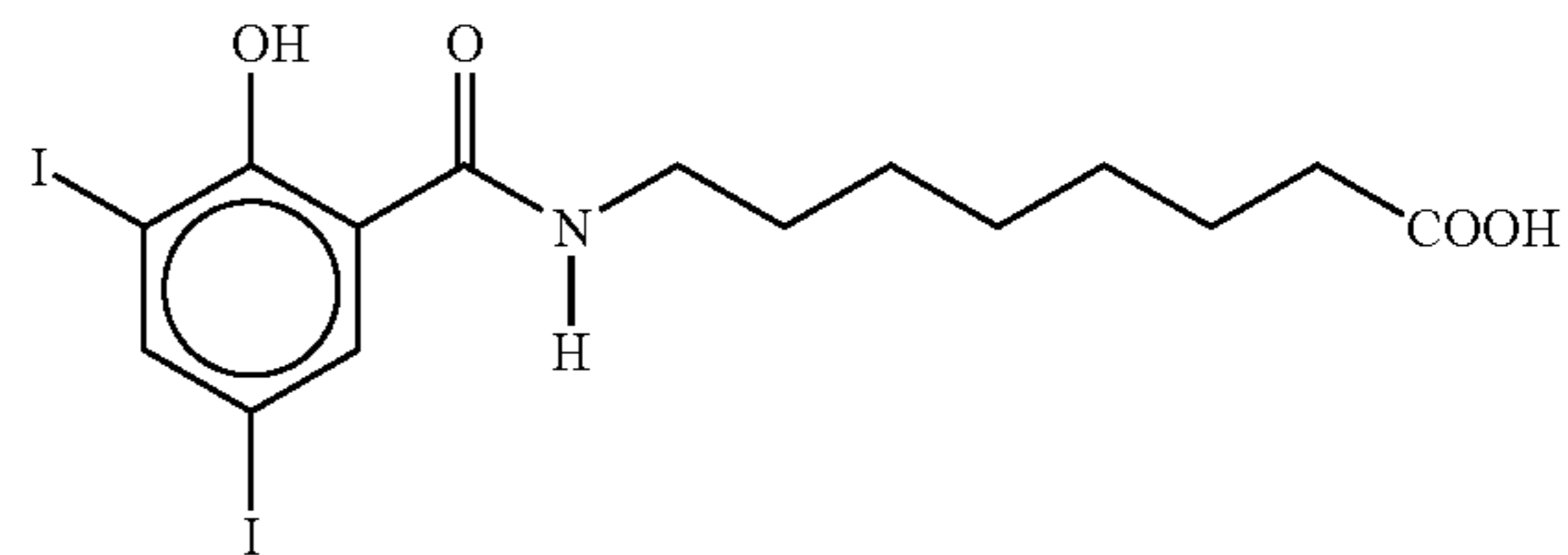
8-(N-(2-hydroxy-3,5-diiodobenzoyl)aminocaprylic acid
