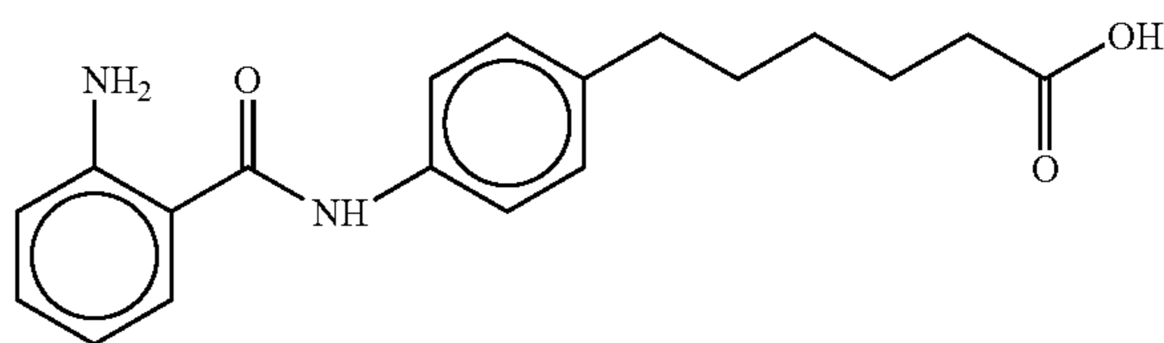
6-(4-(N-2-aminobenzoyl)aminophenyl)hexanoic acid
