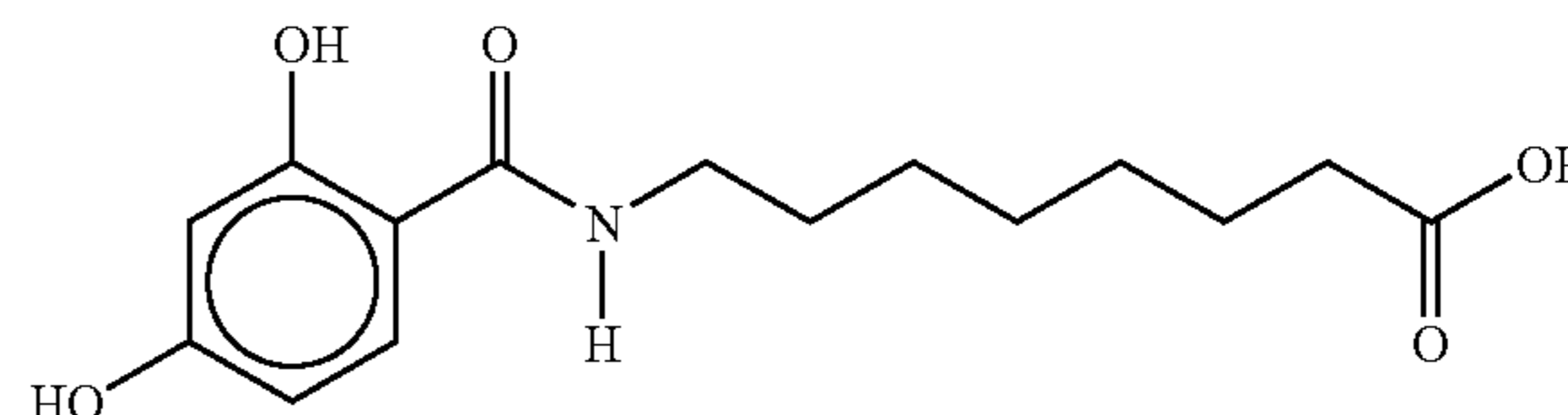
8-(N-(2,4-Dihydroxybenzoyl))aminocaprylic acid
