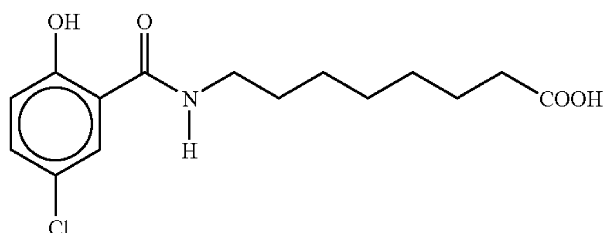
8-(N-(2-hydroxy-5-chlorobenzoyl)aminocaprylic acid
