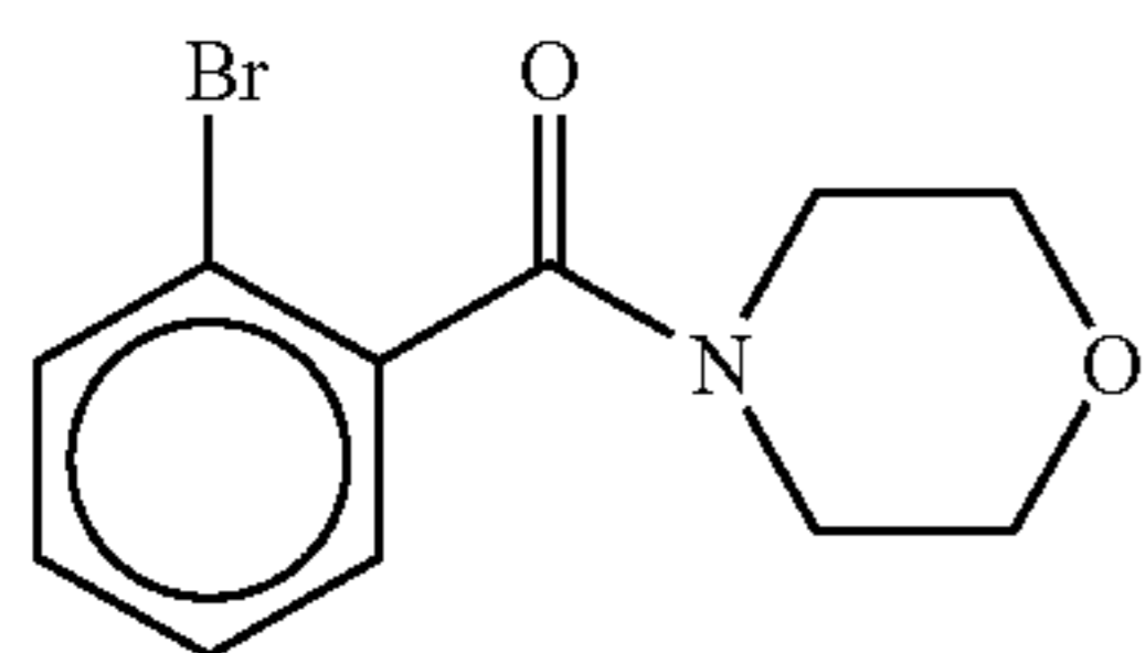
N-(2-bromobenzoyl)morpholine
