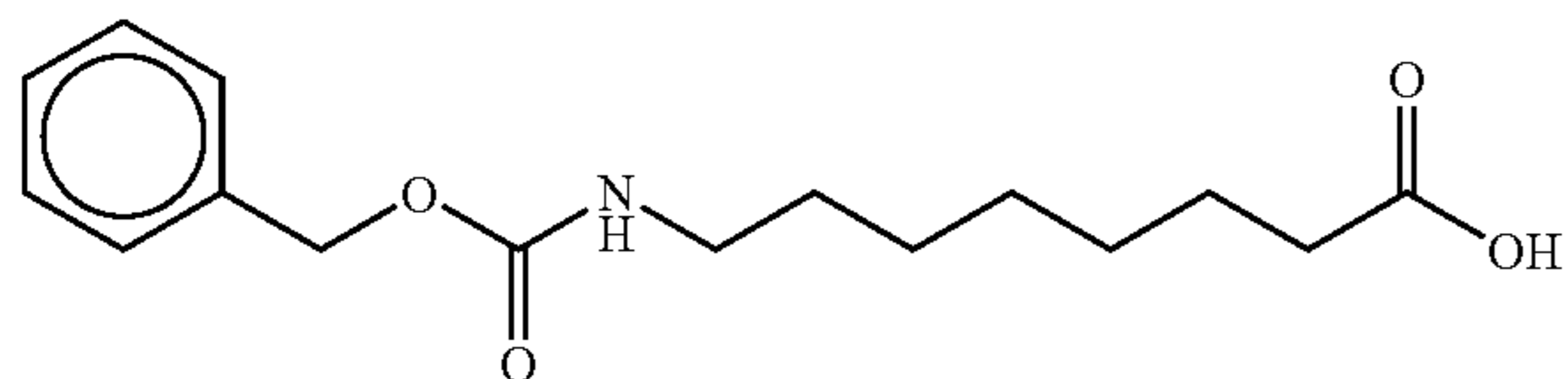
8-(Benzylcarbonylamino)caprylic acid
