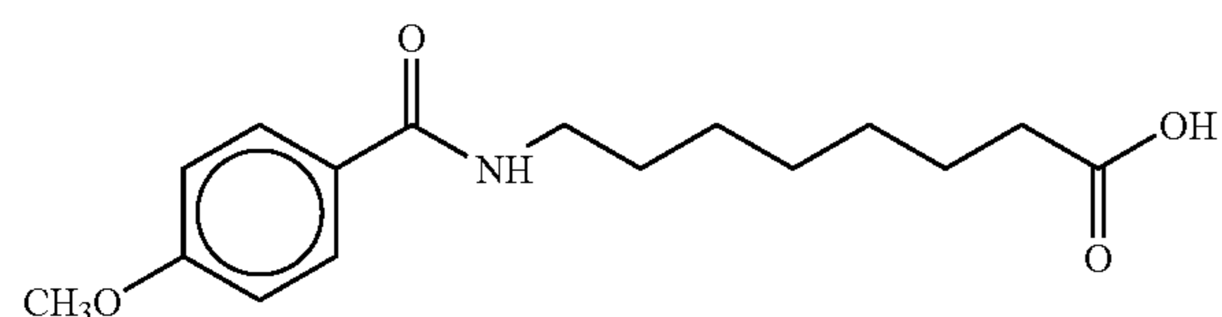
8-(p-anisoyl)aminocaprylic acid
