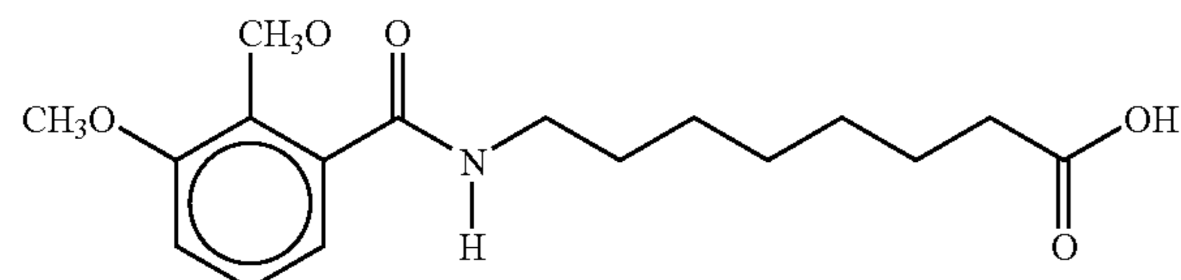
8-(N-(2,3-Dimethoxybenzoyl))aminocaprylic acid
