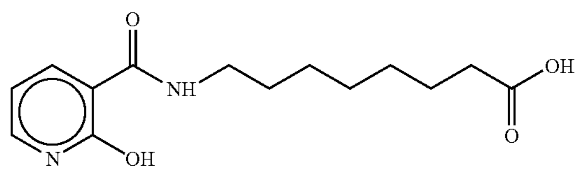
8-(2-Hydroxynicotinoyl)aminocaprylic acid
