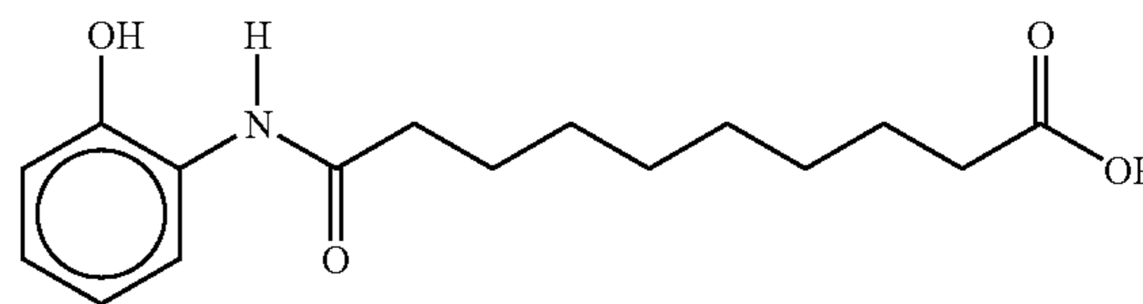
10-(N-(2-Methoxyanilino))sebacic acid
