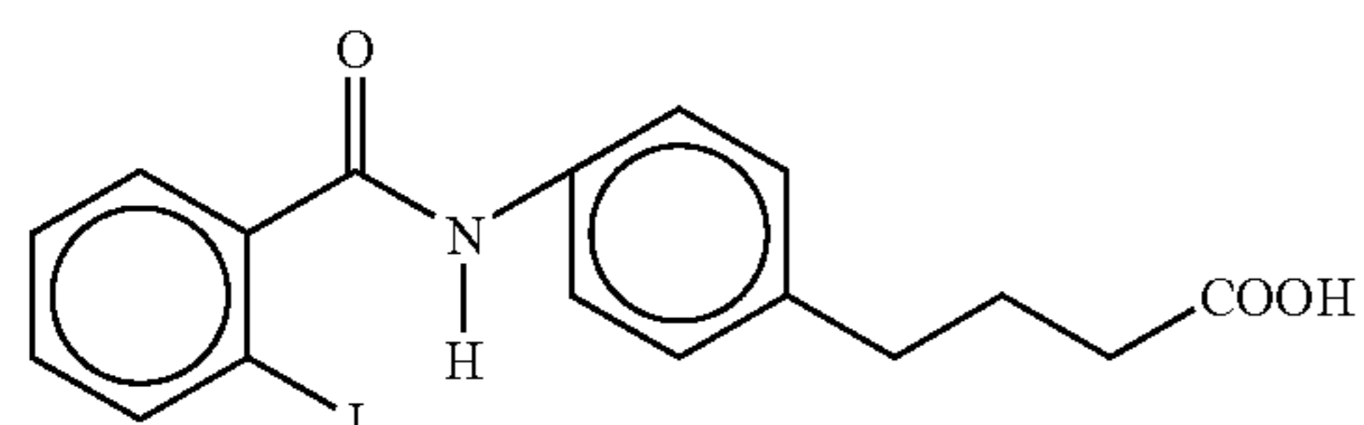
4-{4-[N-(2-iodobenzoyl)]aminophenyl}butyric acid
