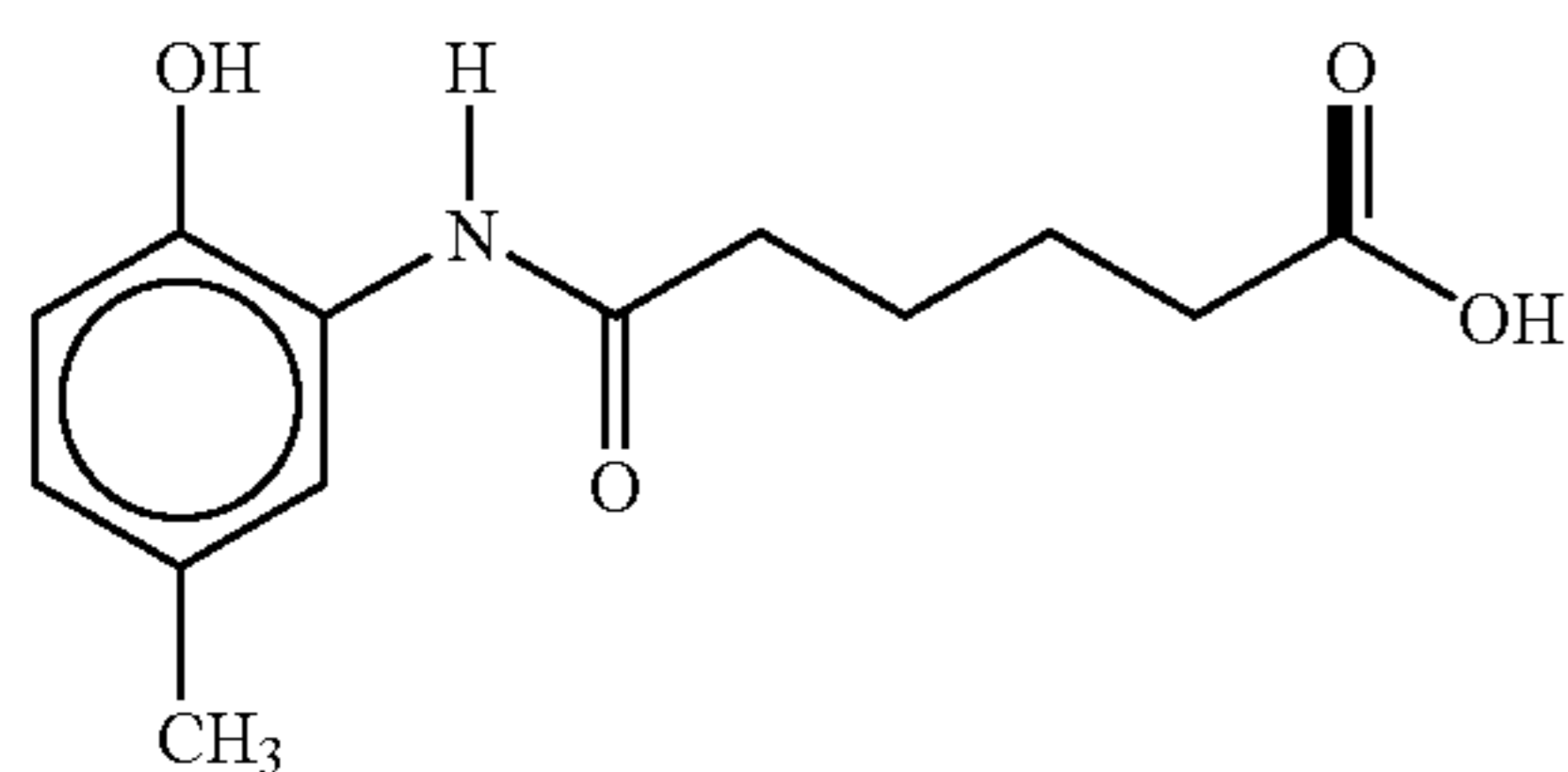
5-(2-hydroxy-5-methylanilino)valeric acid
