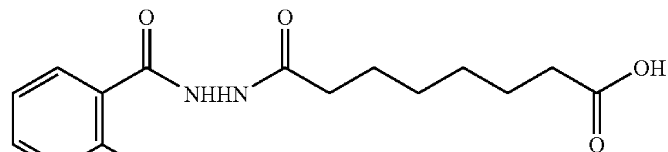
1-salicyloyl-2-suberyl hydrazide
