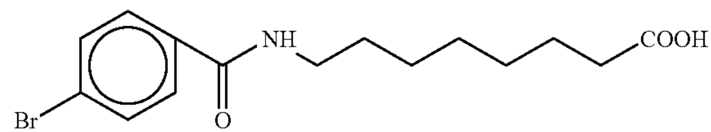
8-[N-(4-bromobenzoyl)]aminocaprylic acid
