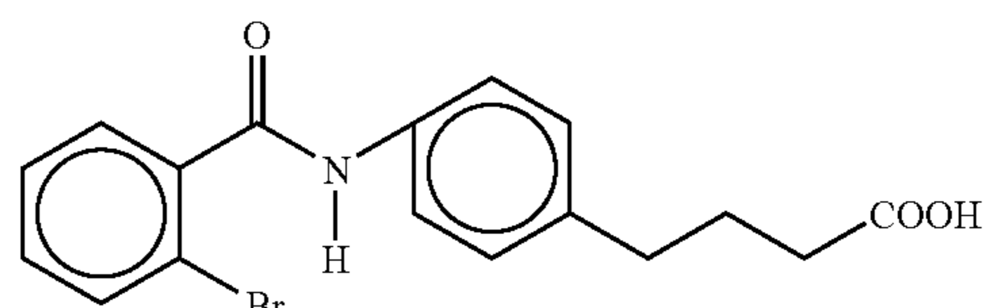
4-{4-[N-(2-bromobenzoyl)]aminophenyl}butyric acid
