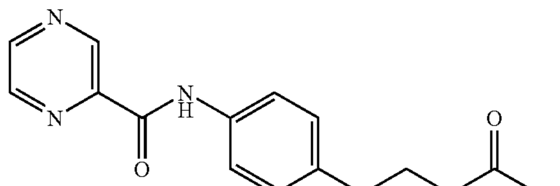
4-(4-(2-pyrazinecarbonyl)aminophenyl)butyric acid
