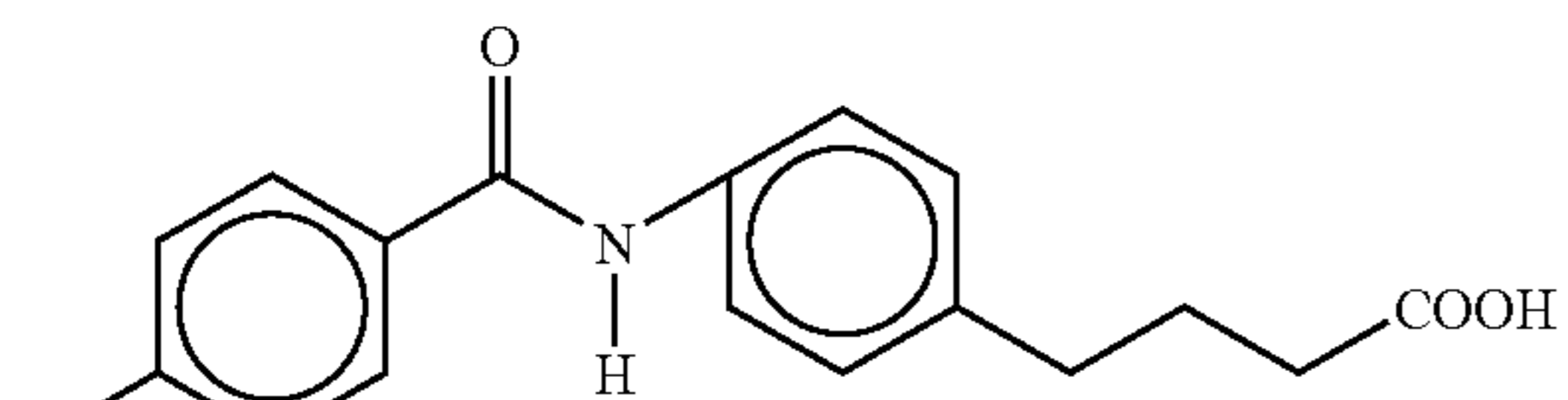
4-(4-[N-(4-bromobenzoyl)aminophenyl])butyric acid
