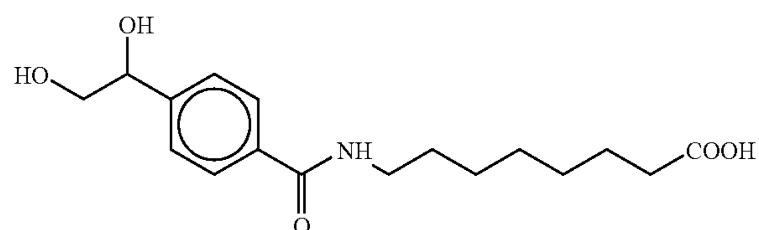
8-(4-(1,2-dihydroxyethyl)benzoyl)aminocaprylic acid
