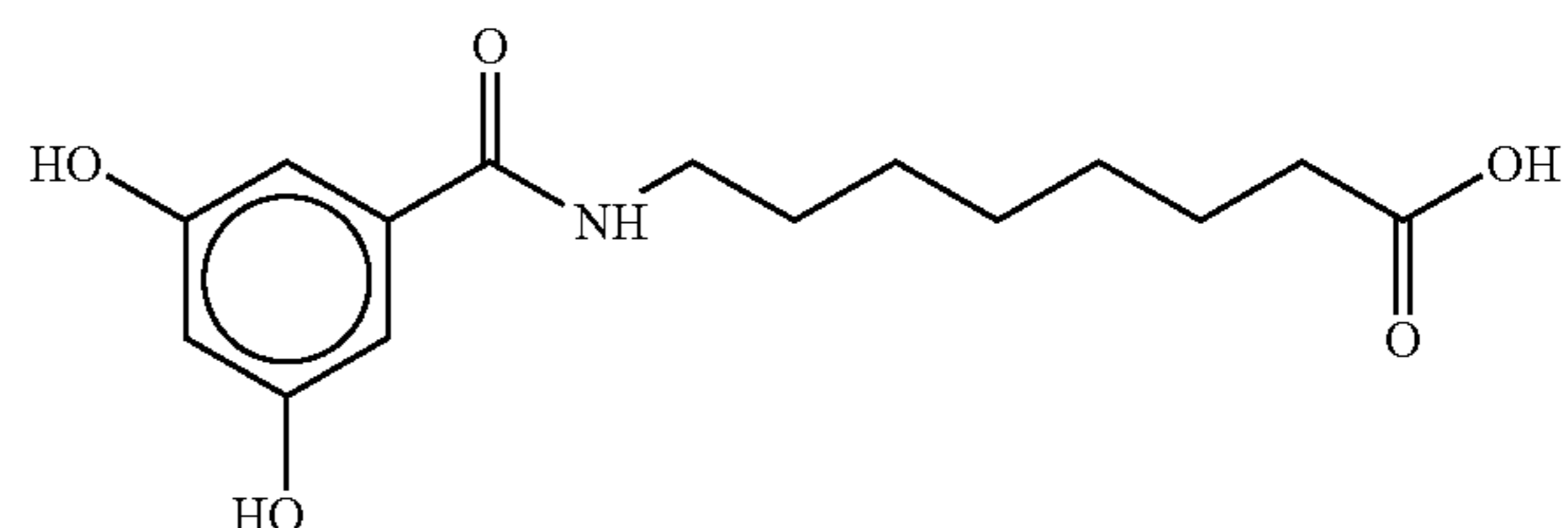
8-(N-3,5-Dihydroxybenzoyl)aminocaprylic acid
