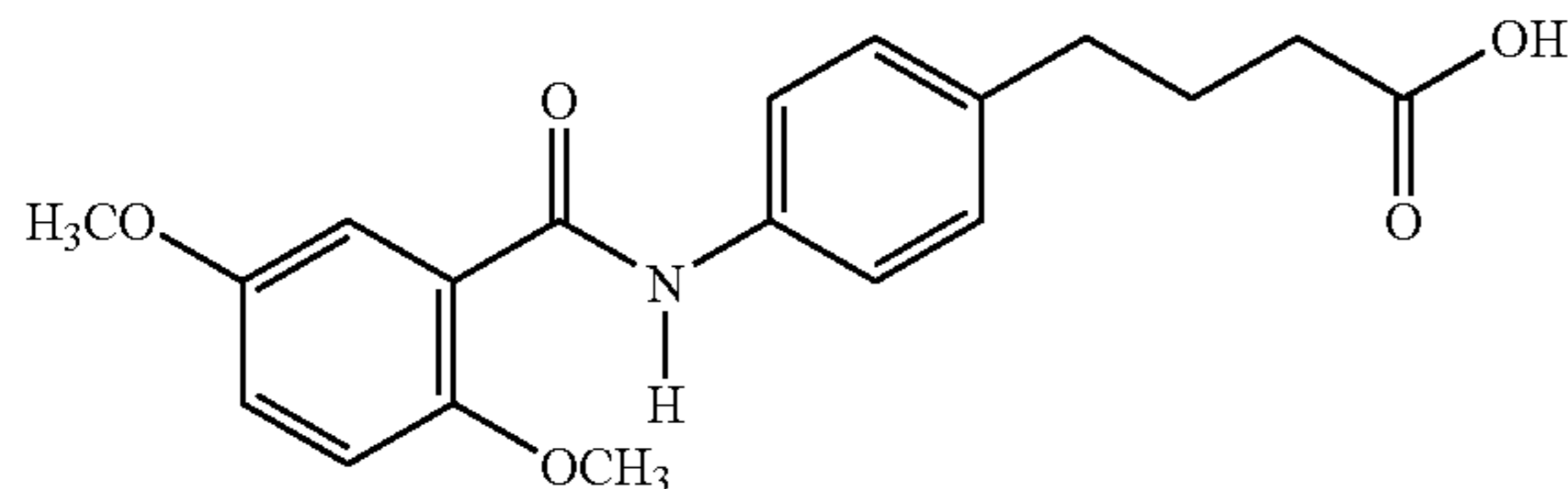
4-(4-(2,5-dimethoxybenzoyl)aminophenyl)butyric acid
