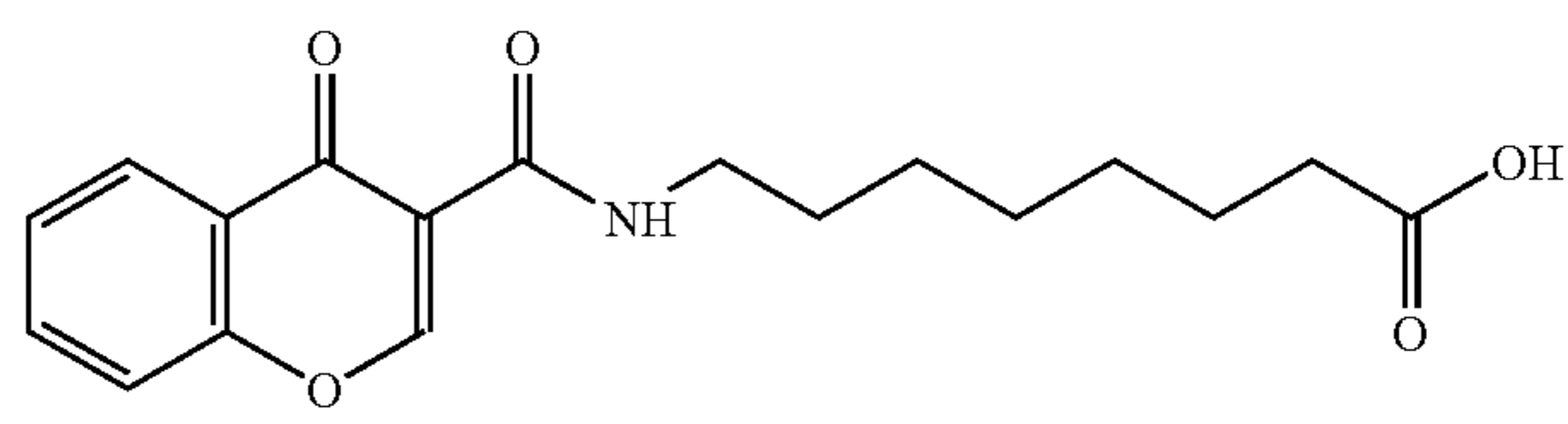
8-(chromone-3-carbonyl)aminocaprylic acid
