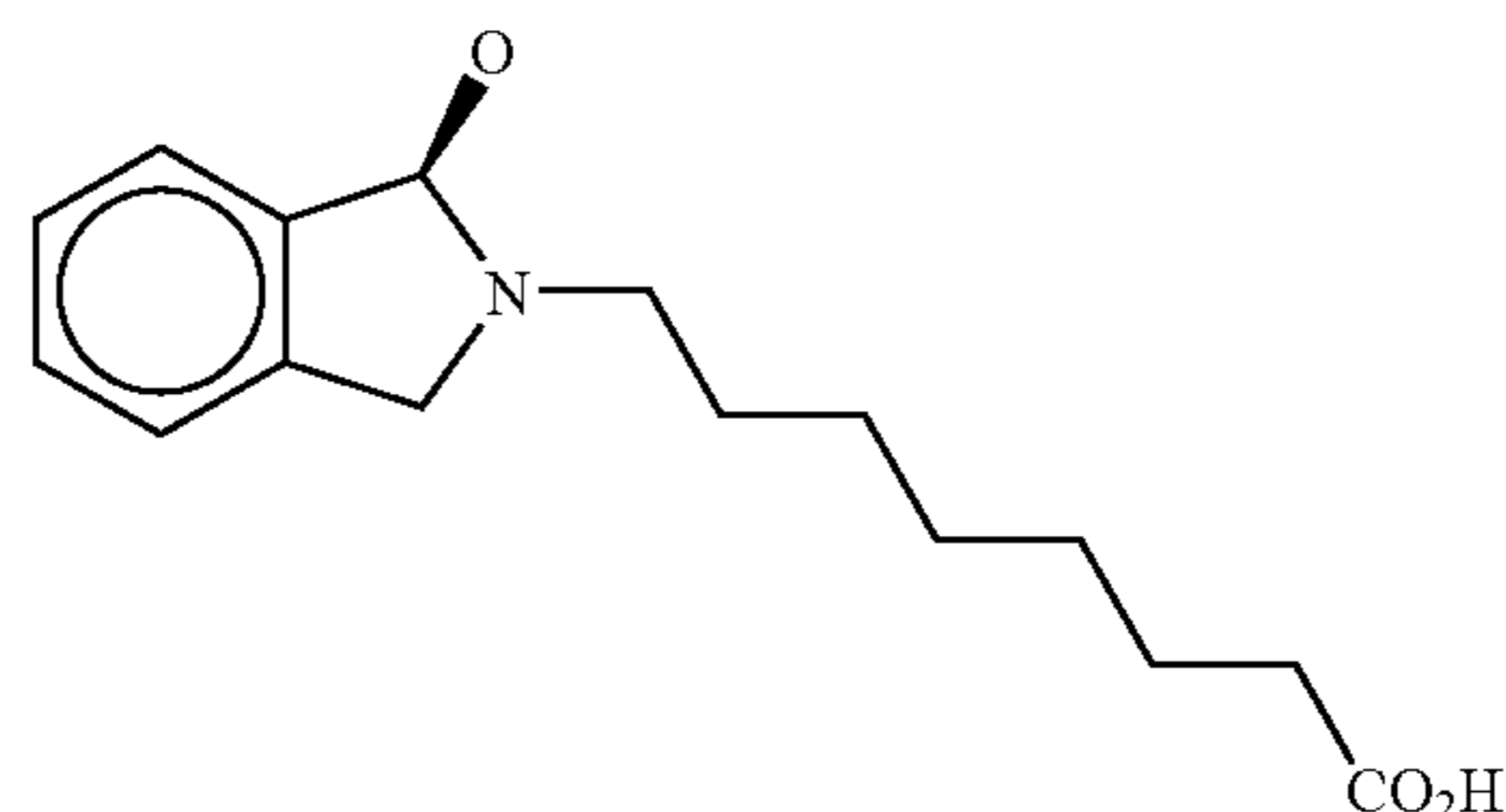
8-(2-(1,2-dihydroisoindole-1-one))octanoic acid
