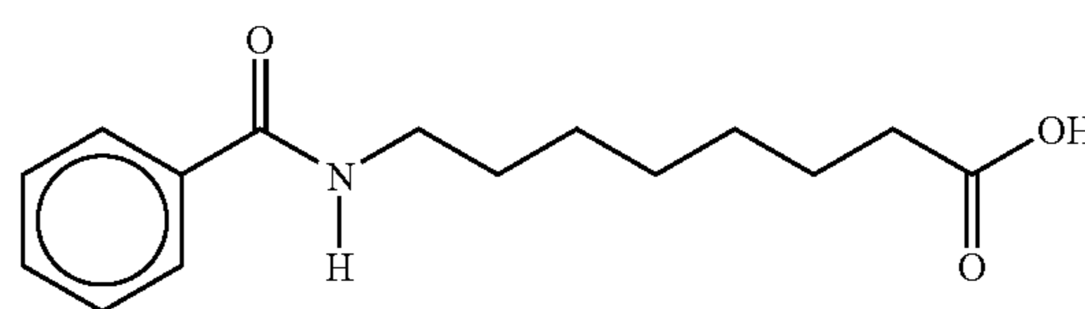
8-(N-benzoyl)aminocaprylic acid
