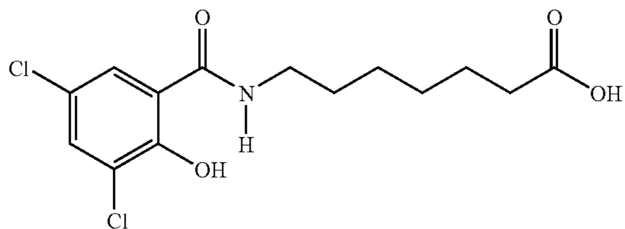
7-N-(3,5-dichloro-2-hydroxybenzoyl)aminoheptanoic acid
