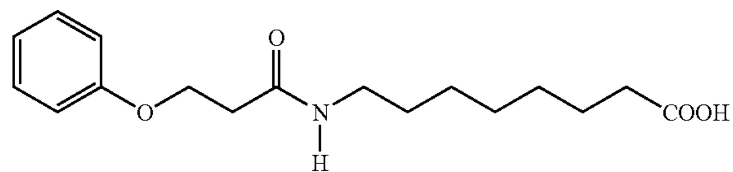
8-(3-Phenoxypropionylamino)caprylic acid
