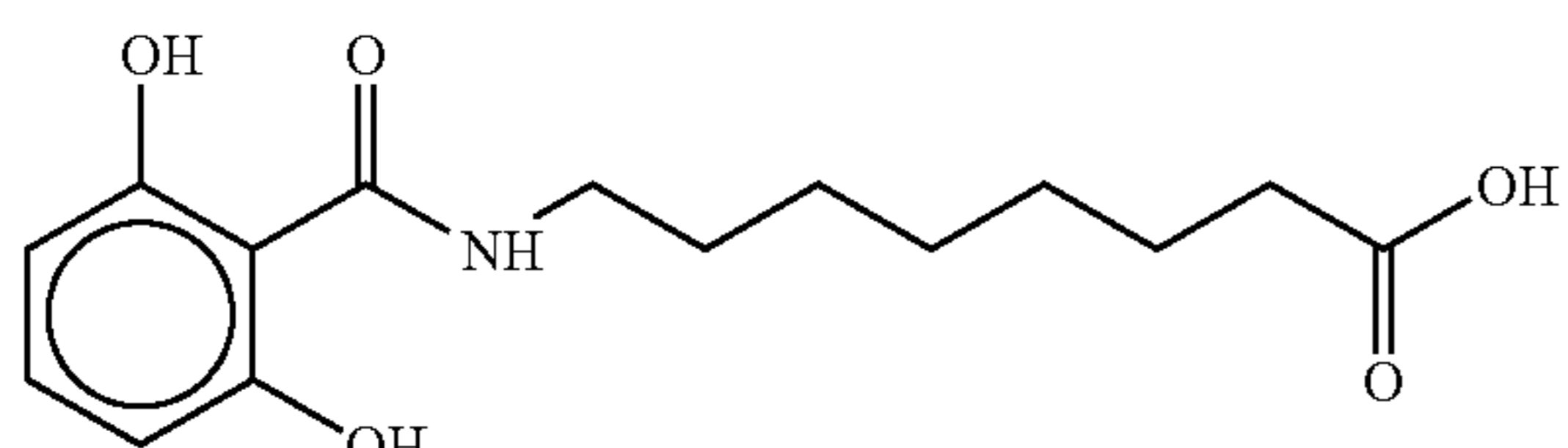
8-(N-2,6-Dihydroxybenzoyl)aminocaprylic acid
