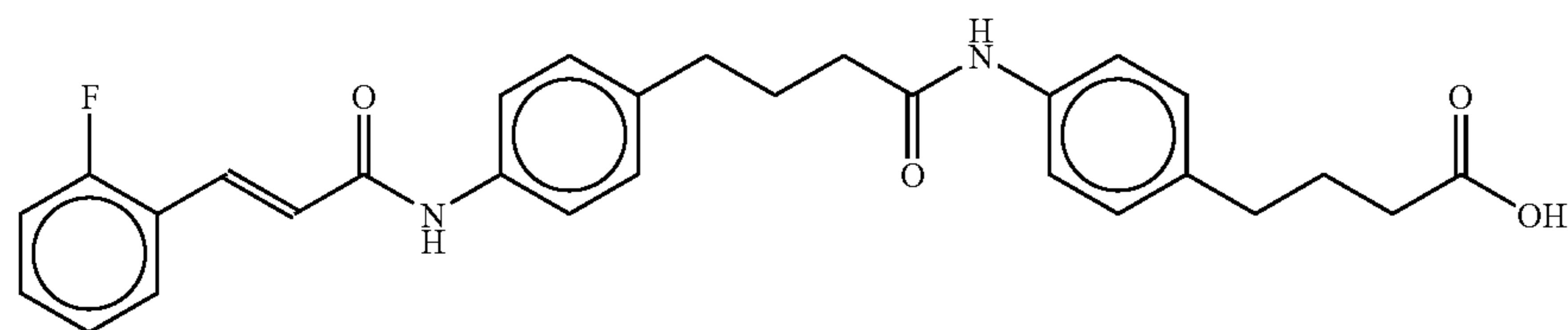
4-(4-(N-(2-Fluorocinnamoyl)aminophenyl)butyric
