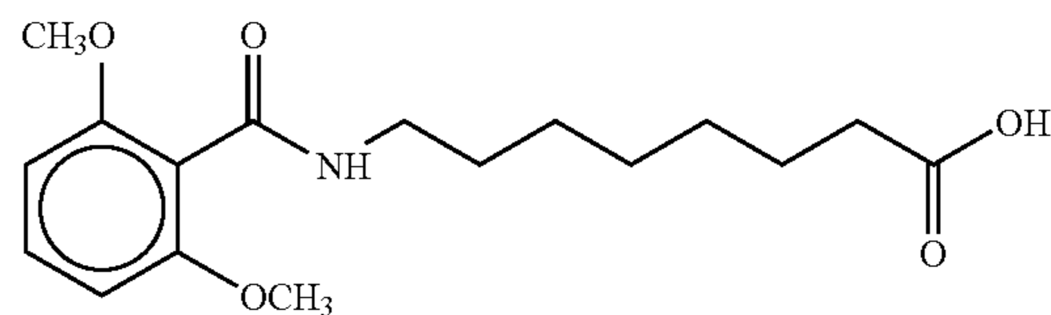
8-(N-2-6-Dimethoxybenzoyl)aminocaprylic acid
