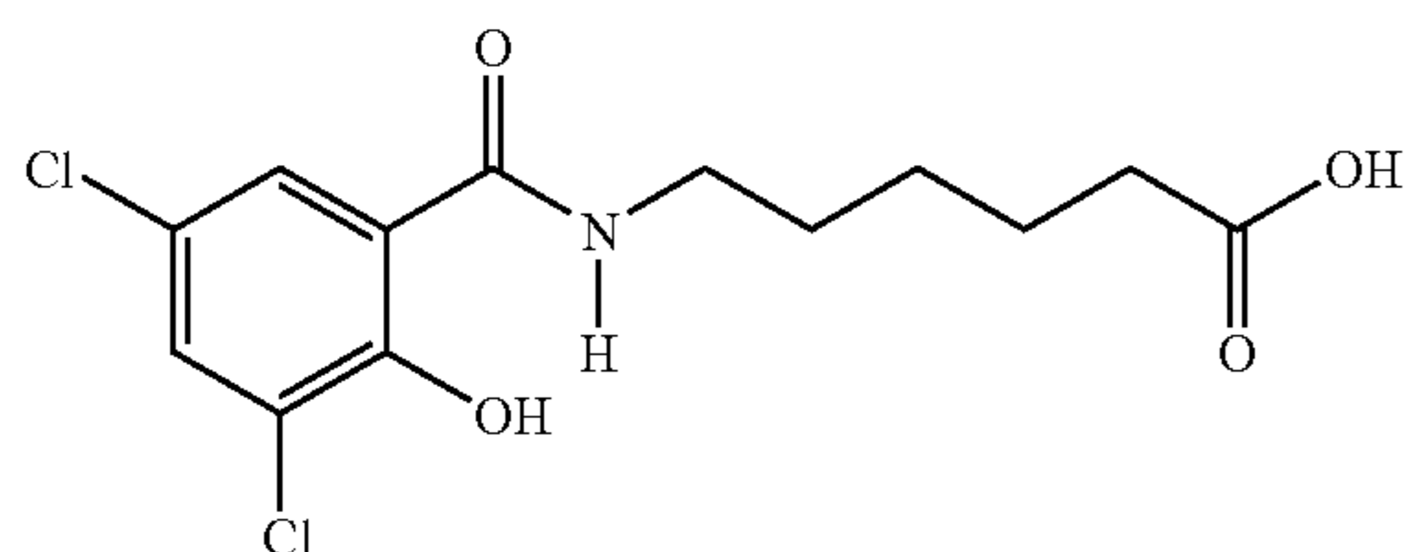
6-N-(3,5-dichloro-2-hydroxybenzoyl)aminocaproic acid
