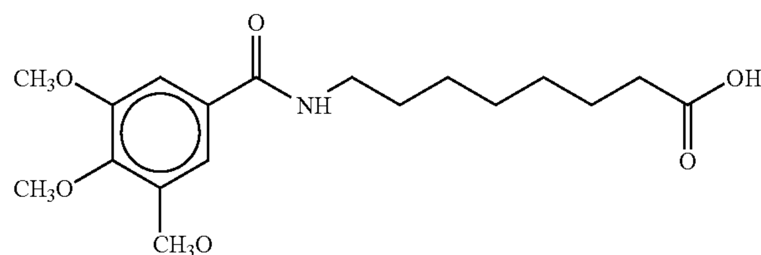
8-(3,4,5-Trimethoxybenzoyl)aminocaprylic acid
