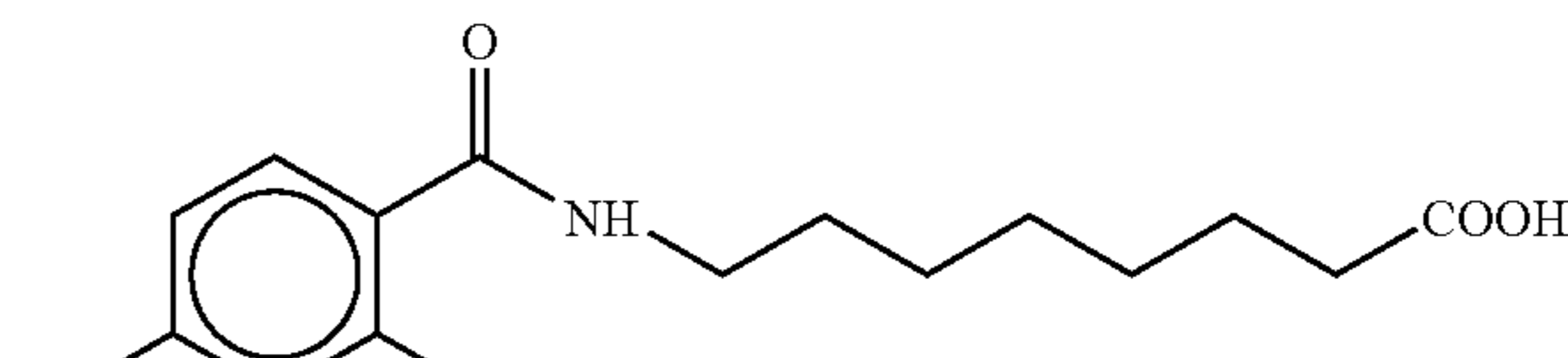
8-(2-hydroxy-4-chlorobenzoyl)aminocaprylic acid
