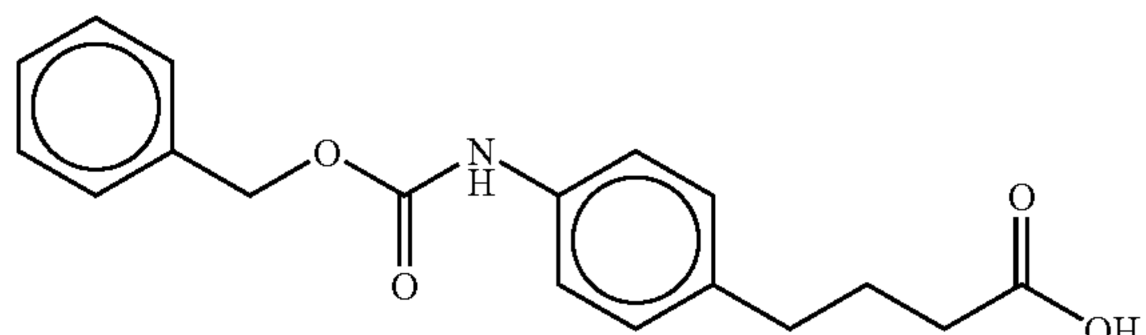
4-(4-benzyloxycarbonylamino)phenylbutyric acid
