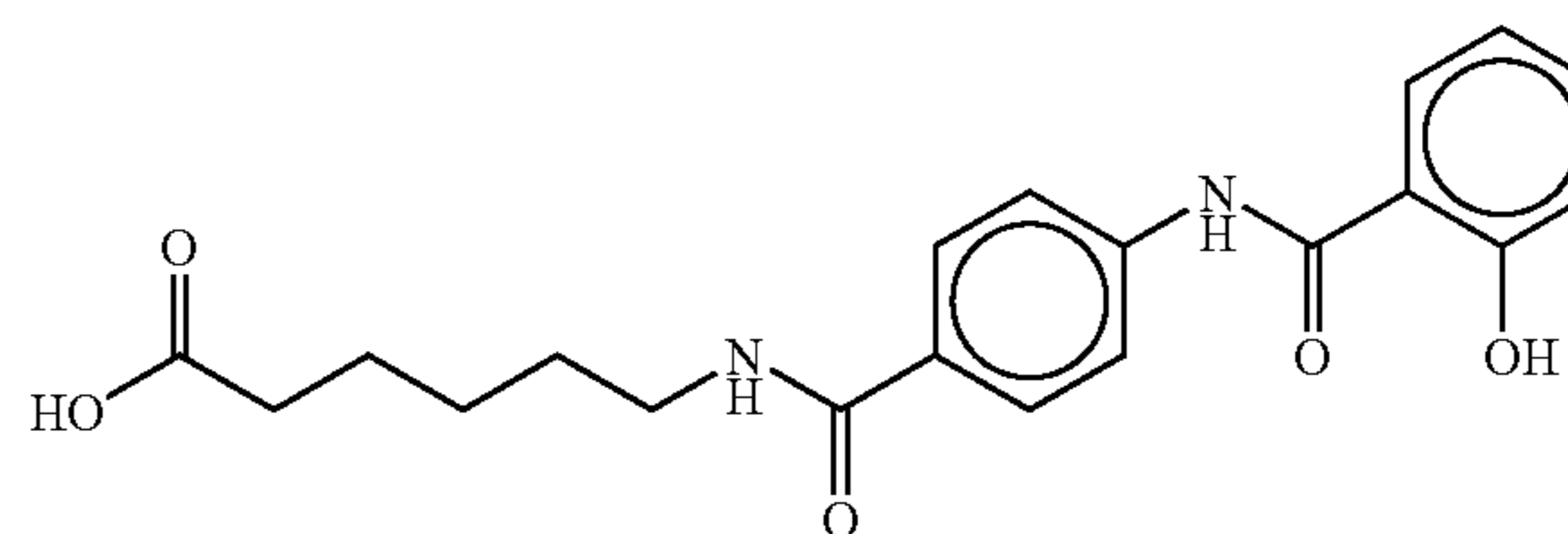
N-(4-salicyloylamino)-6-caproic acid
