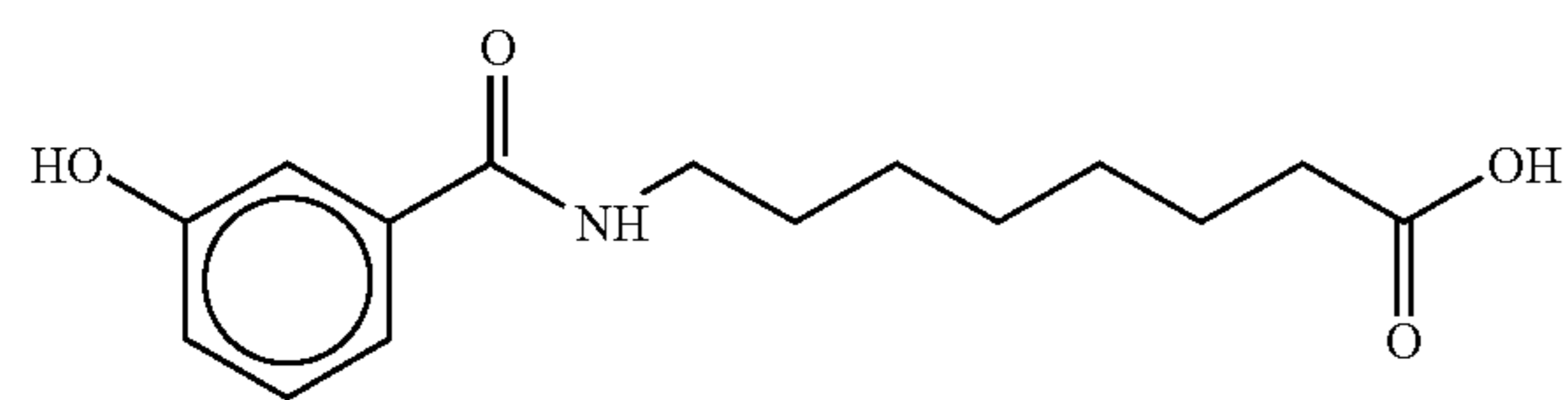
8-(3-Hydroxybenzoyl)aminocaprylic acid
