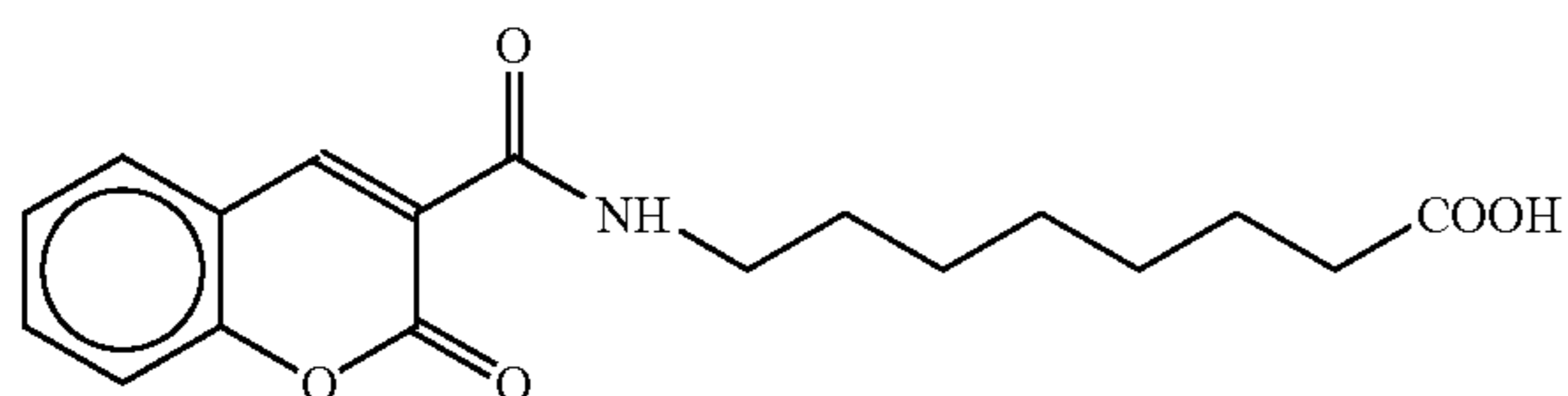
8-[N-(3-coumarincarboxyl)]aminocaprylic acid
