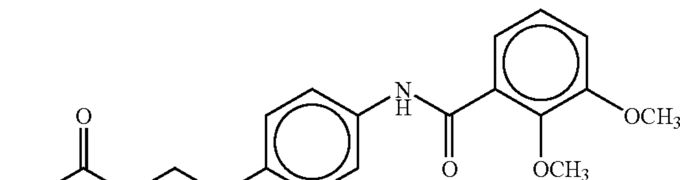
4-(4-(2,3-dimethoxybenzoyl)aminophenyl)butyric acid
