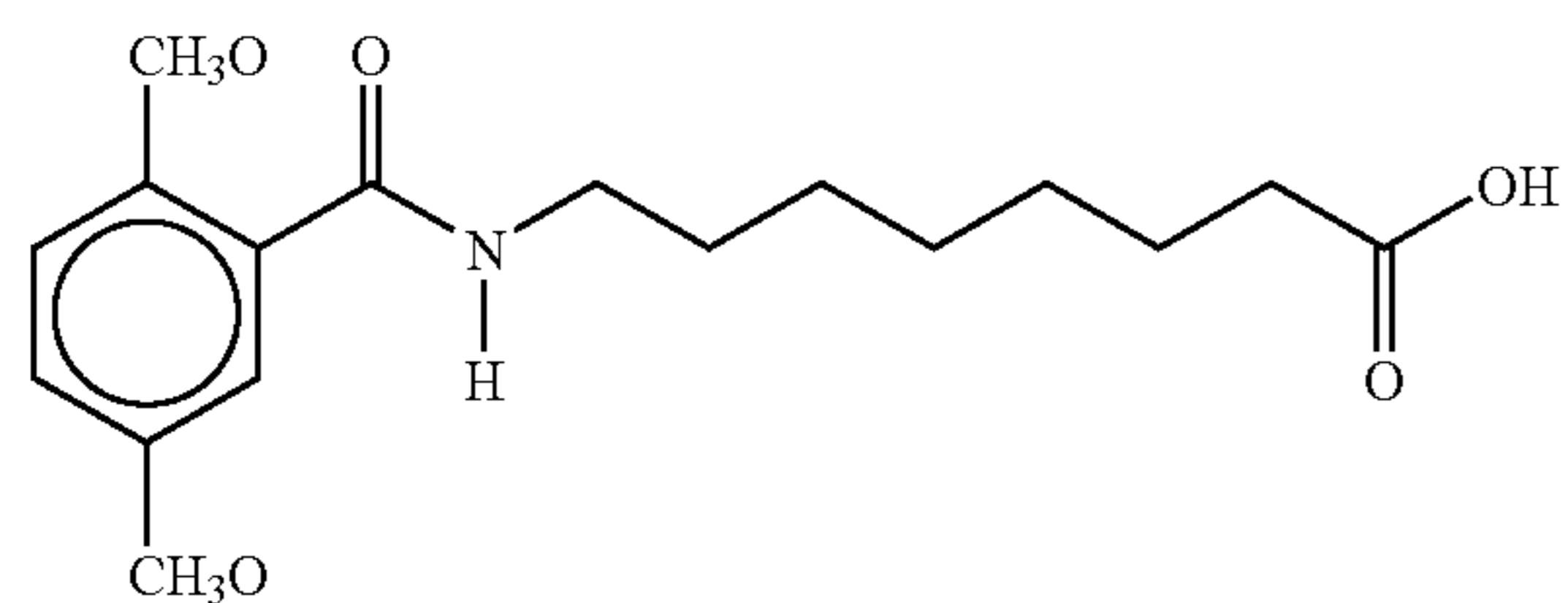
8-(N-(2,5-Dimethoxybenzoyl))aminocaprylic acid
