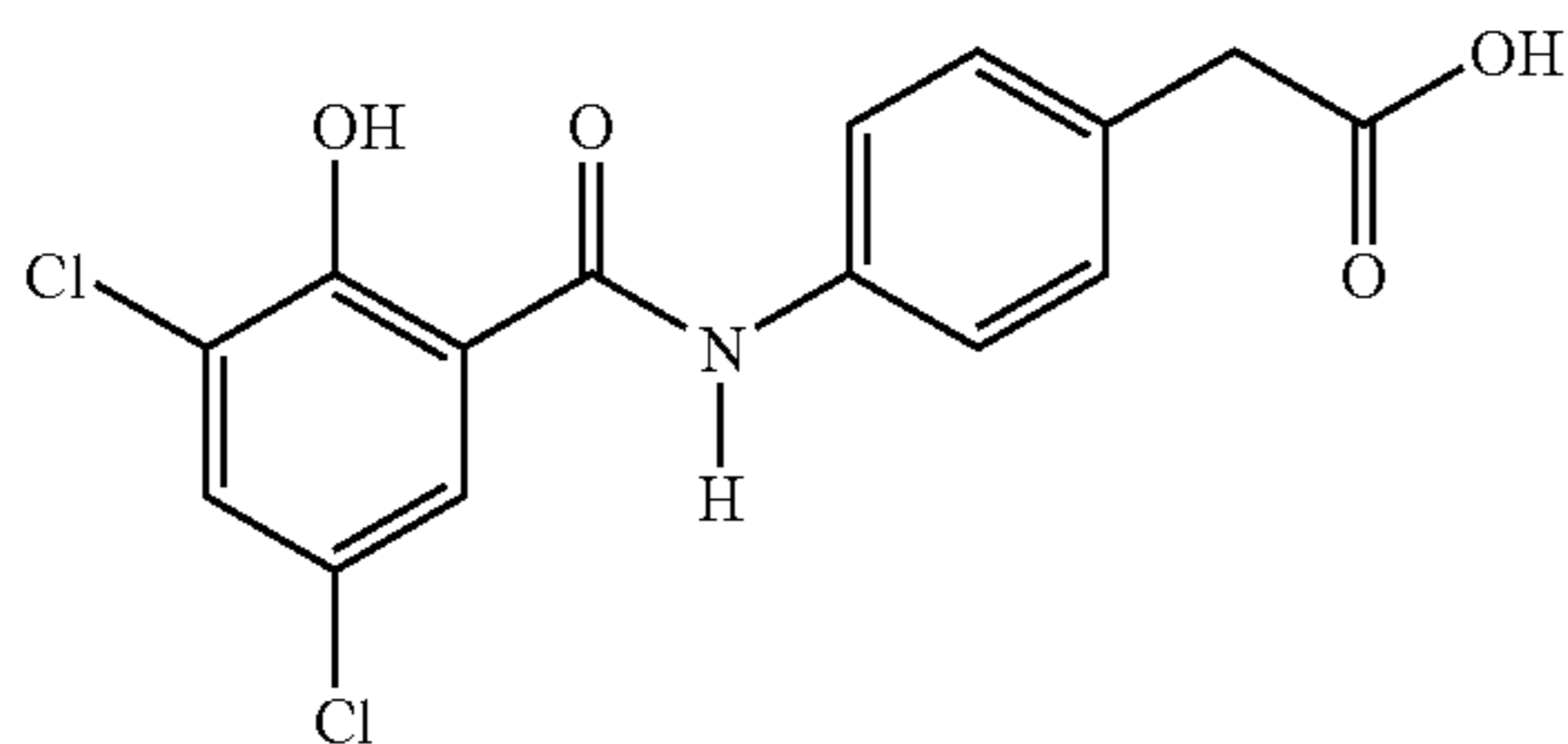
4-[N-(3,5-dichloro-2-hydroxybenzoyl)]aminophenylacetic acid
