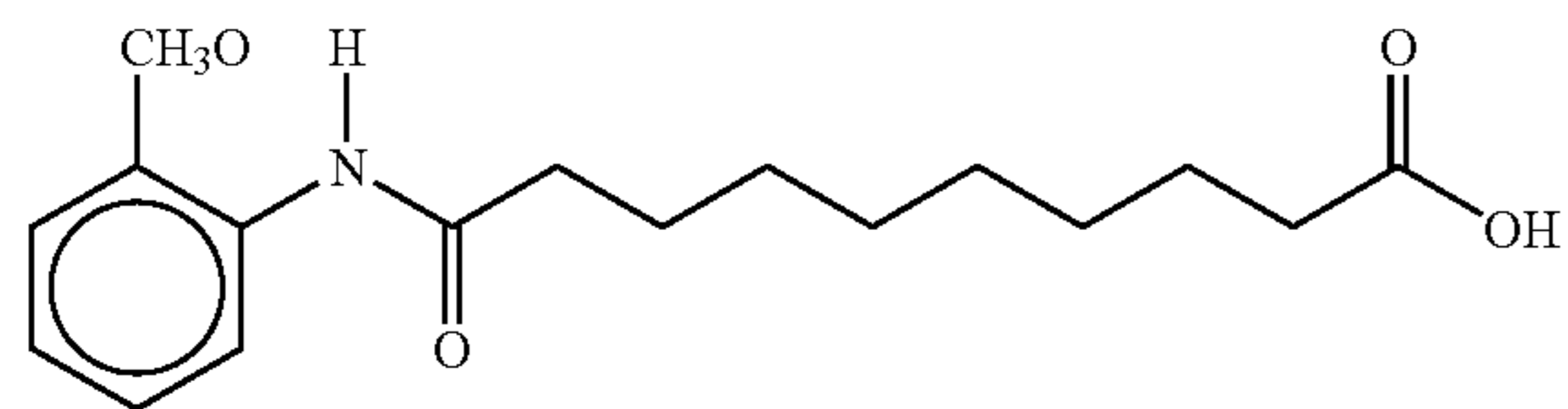
10-(N-(2-Methoxyanilino))sebacic acid
