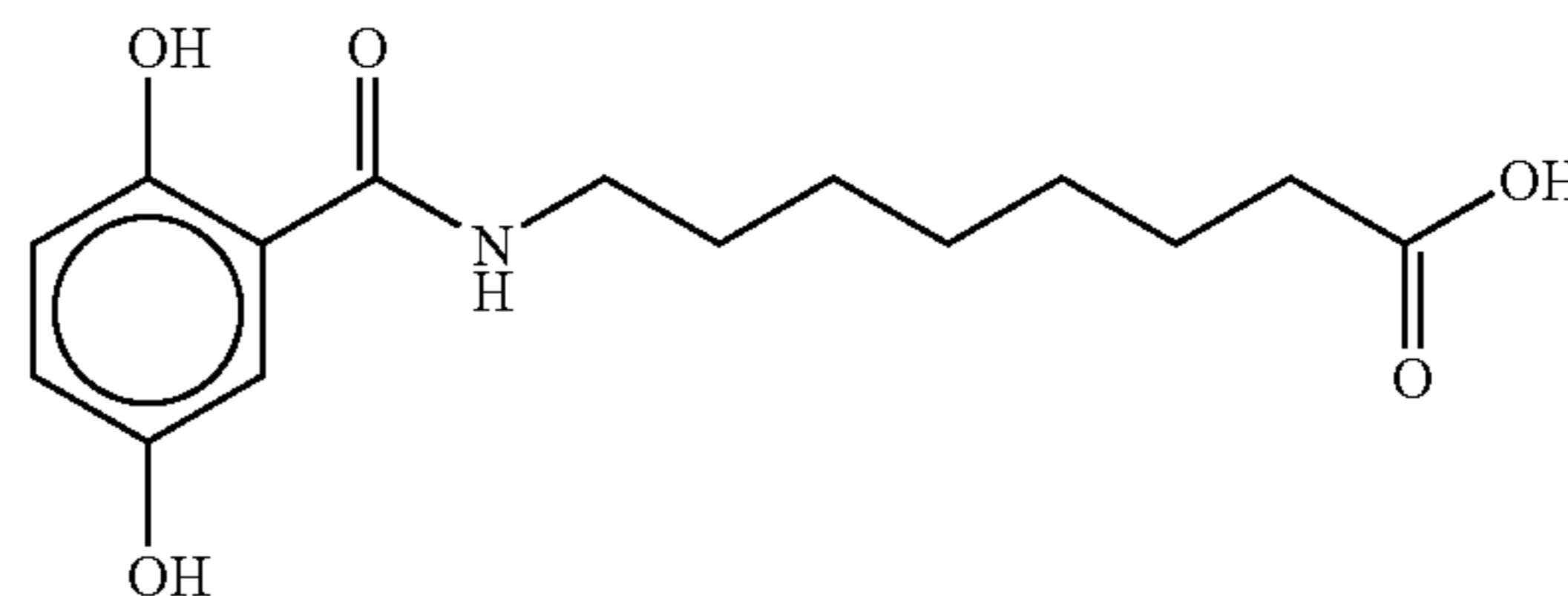
8-(N-(2,5-Dihydroxybenzoyl))aminocaprylic acid
