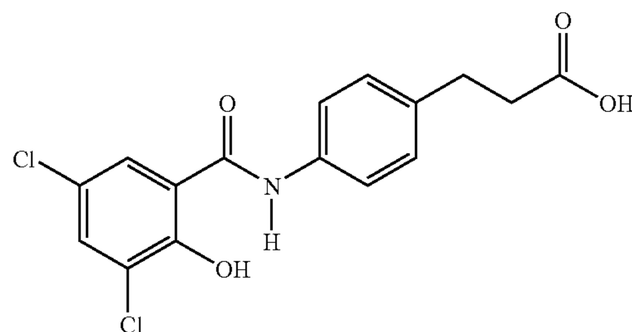
N-[3,5-dichloro-2-hydroxybenzoyl-3-(4-aminophenyl)]propionic acid
