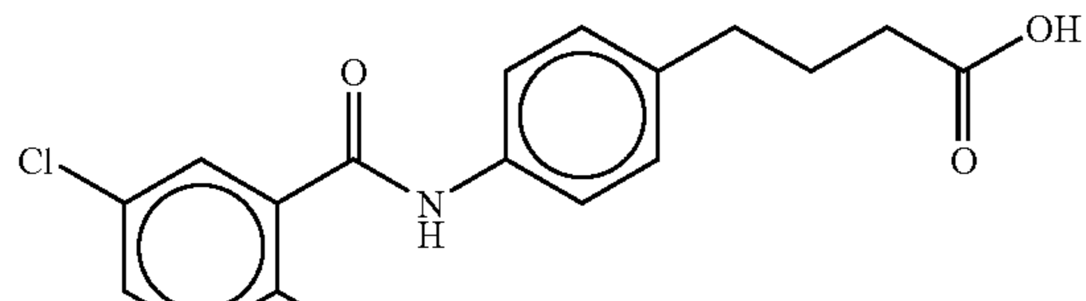
4-(4-(5-chloro-o-anisoyl)aminophenyl)butyric acid
