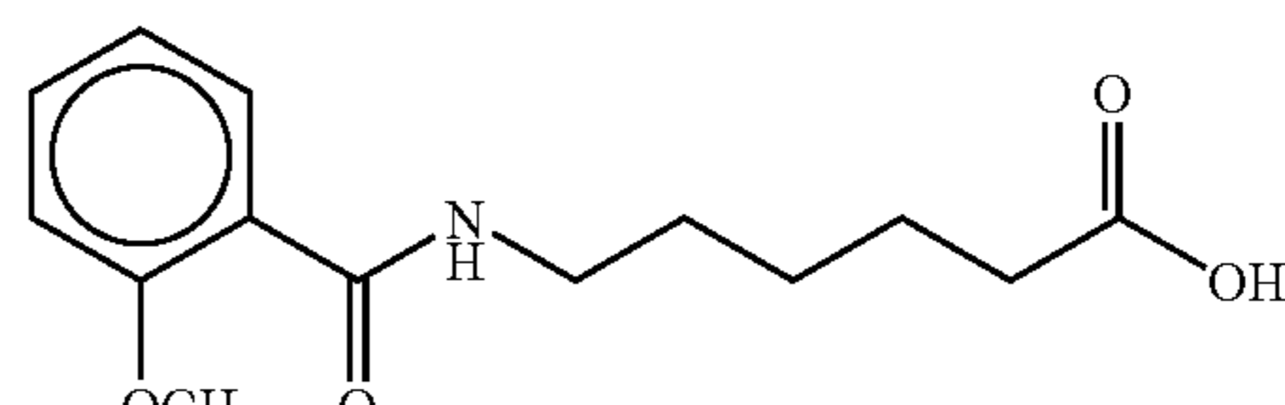
6-(anisoyl)aminocaproic acid
