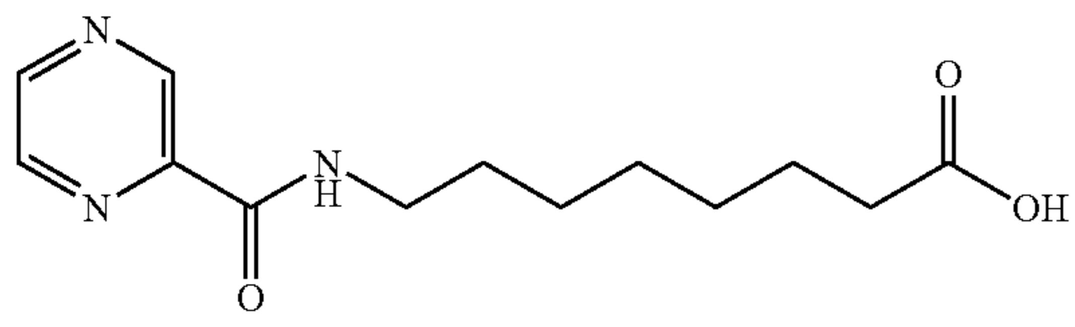
8-(2-pyrazinecarbonyl)aminocaprylic acid
