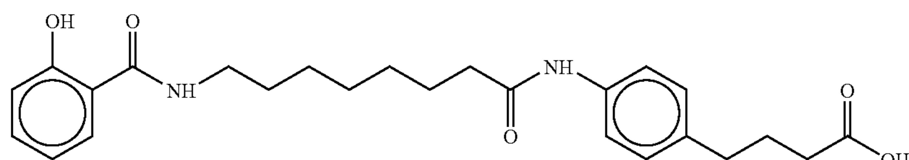
4-(4-(N-8(N-Salicyloyl)aminocaprylic)aminophenyl)butyric acid
