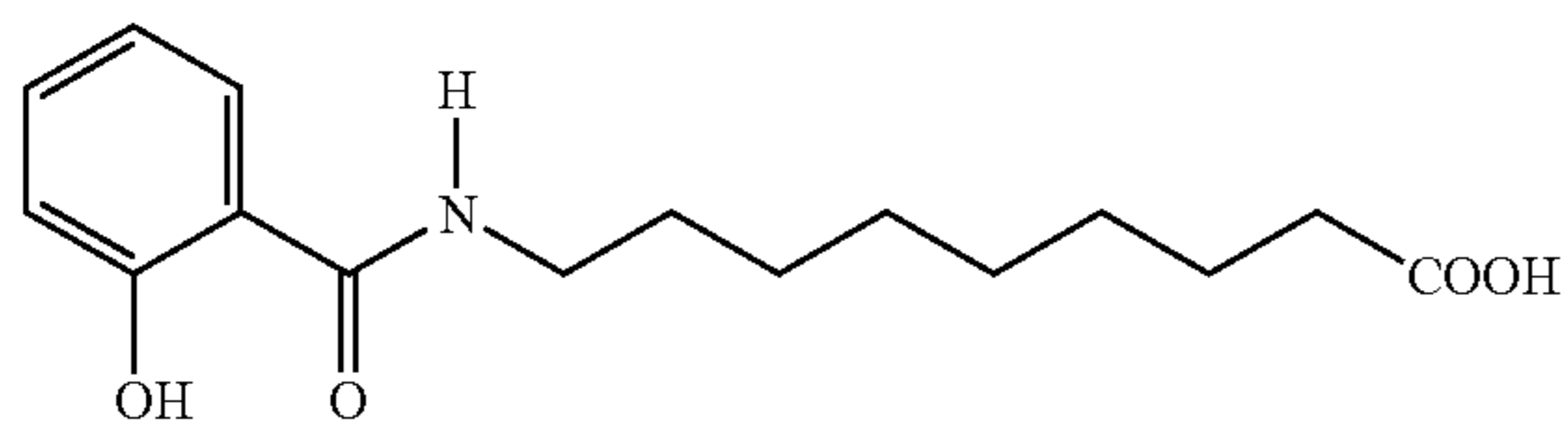
9-Salicyloylaminononanoic acid
