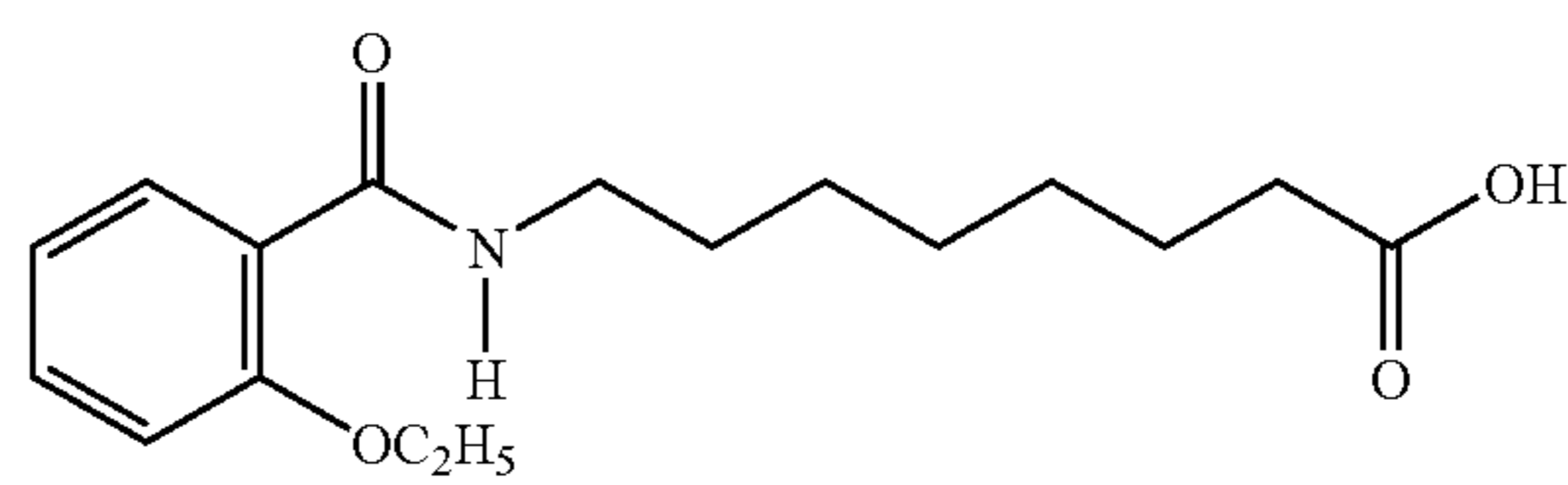
8-(2-ethoxybenzoyl)aminocaproic acid
