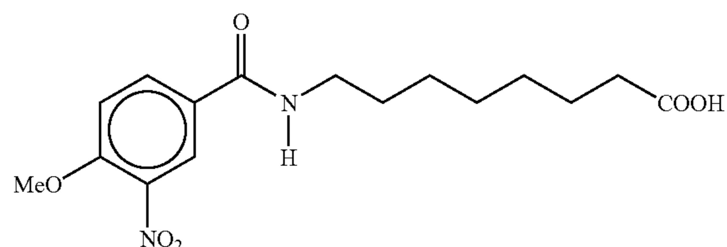
8-N-(4-methoxy-3-nitrobenzoyl)aminocaprylic acid
