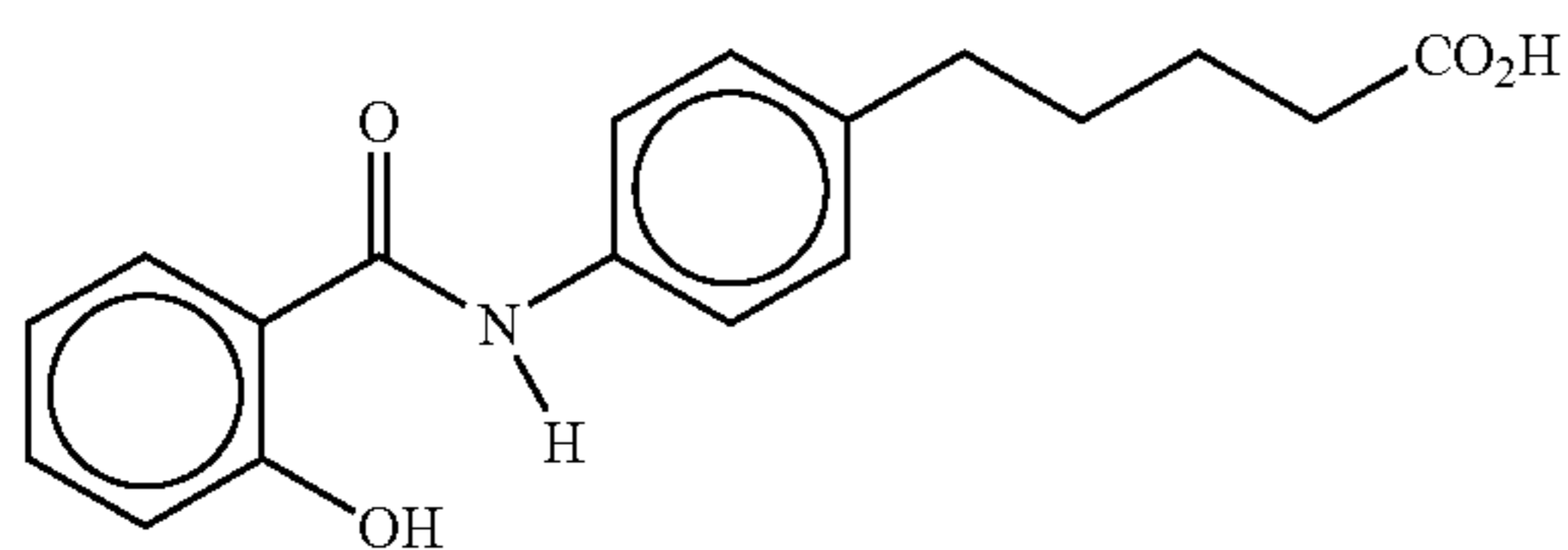
N-salicyl-5-(4-aminophenyl)valeric acid
