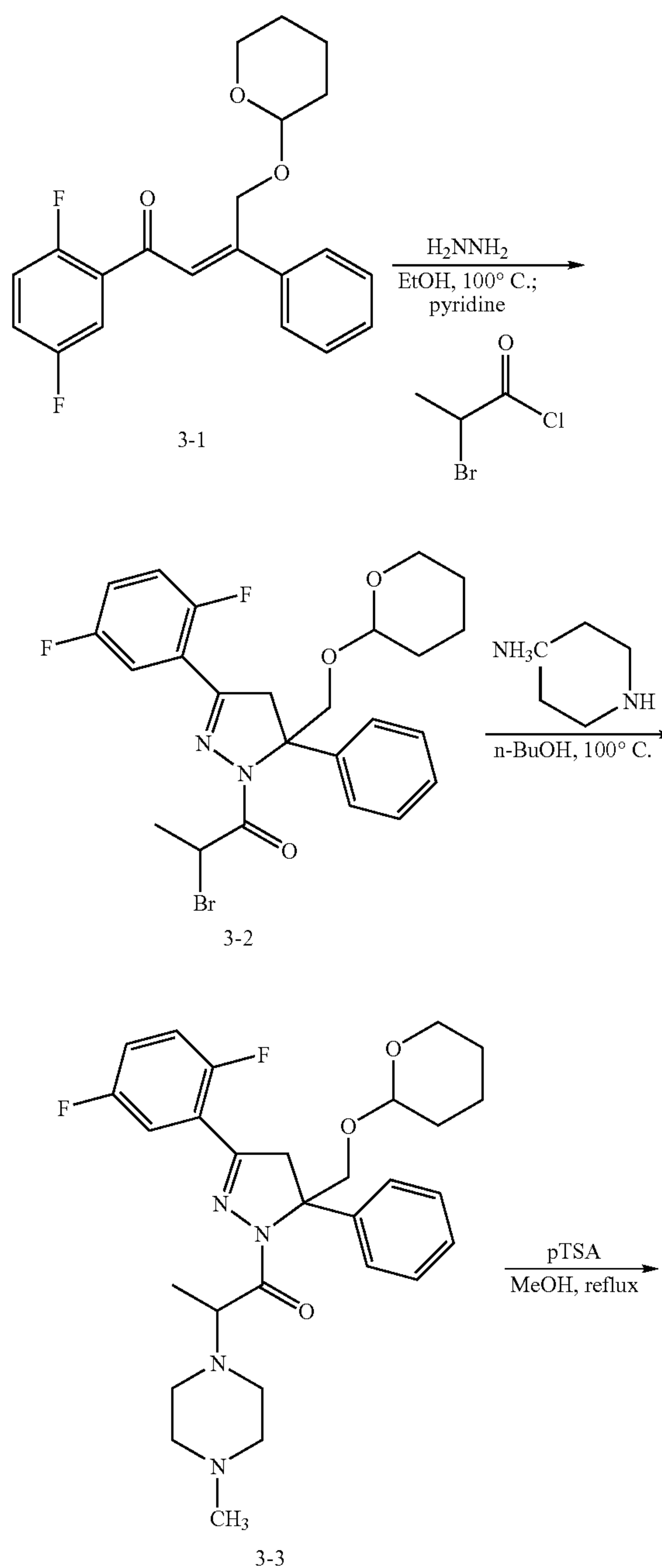
SCHEME 3
