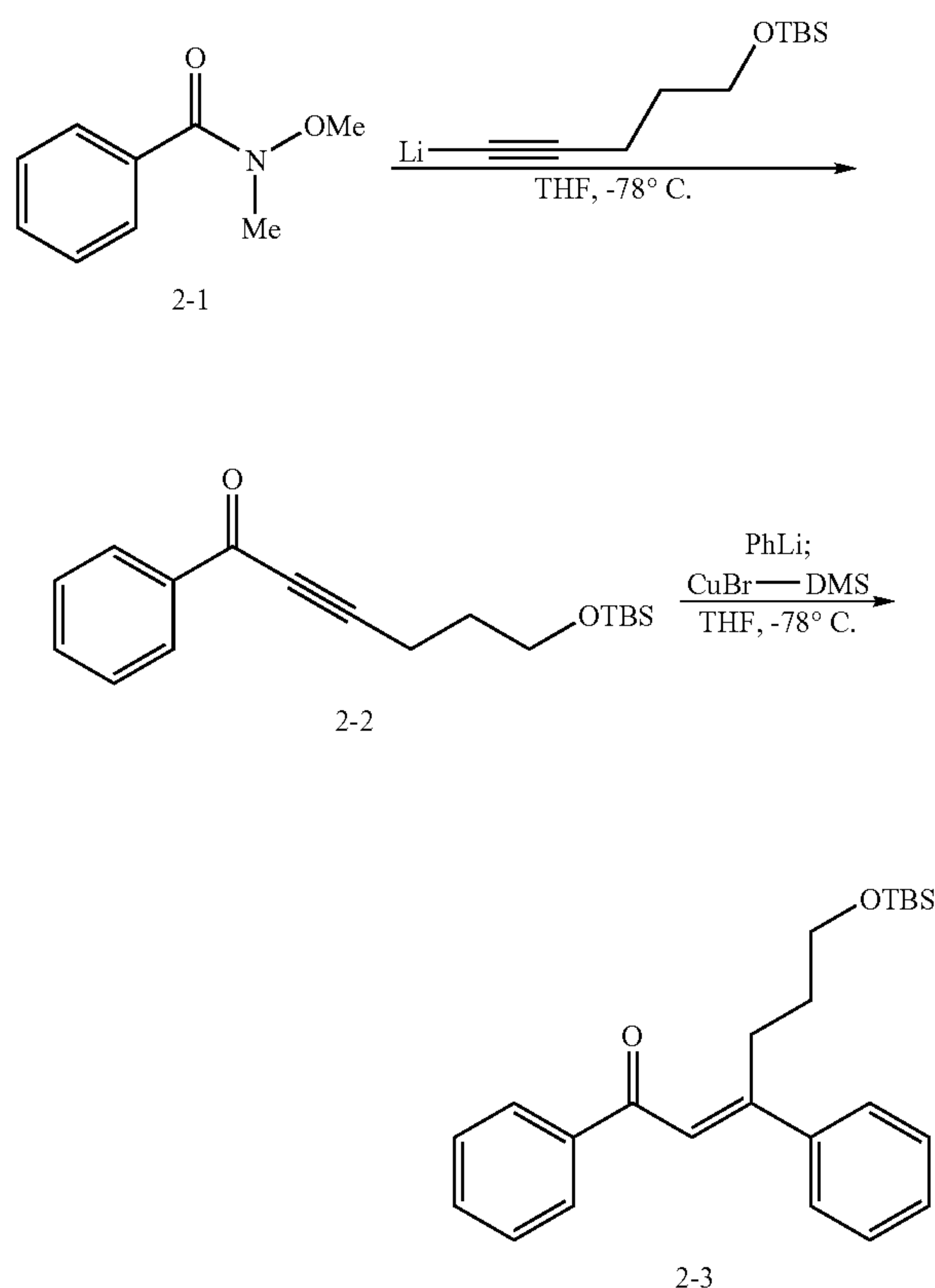
SCHEME 2
