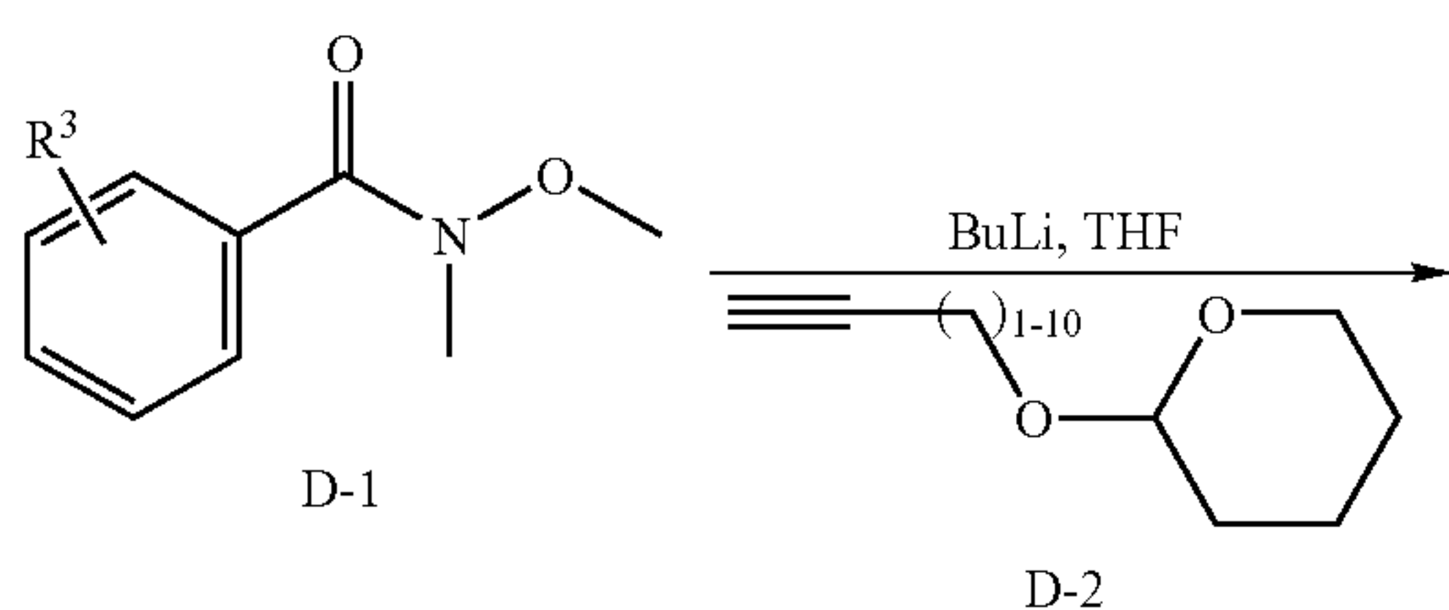
SCHEME D
