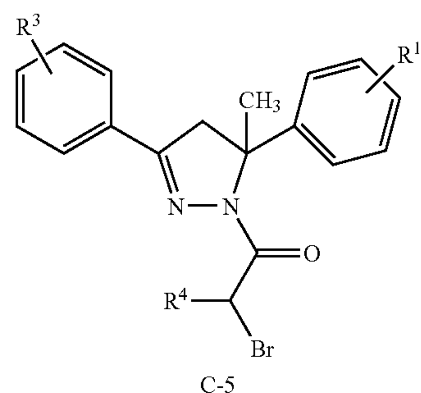
SCHEME D
