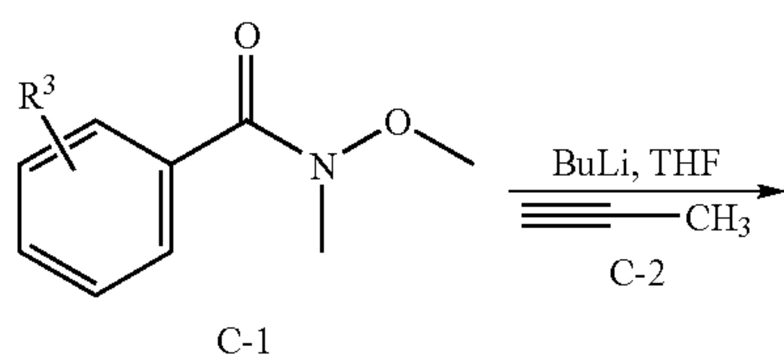
SCHEME C
