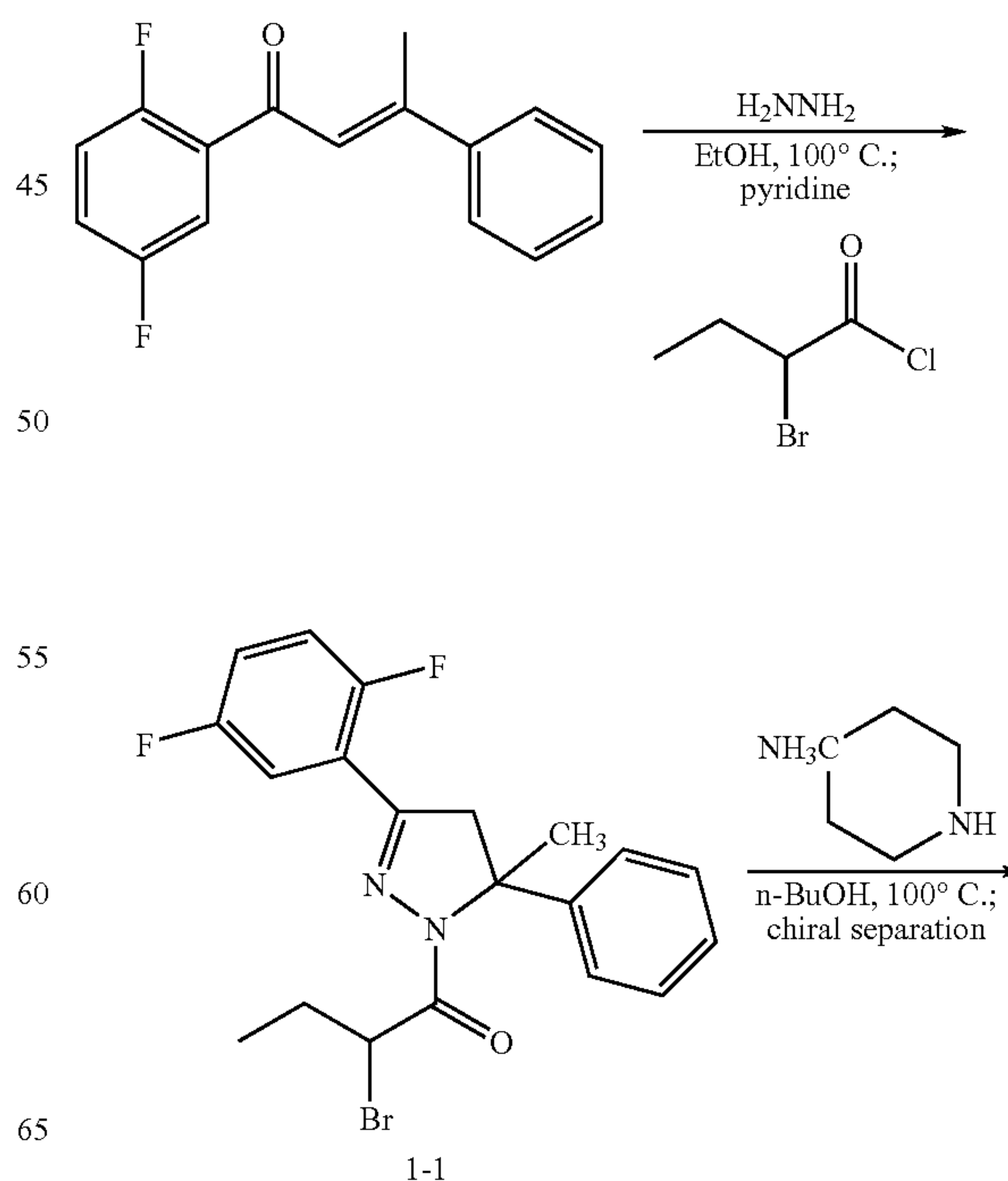
SCHEME 1
