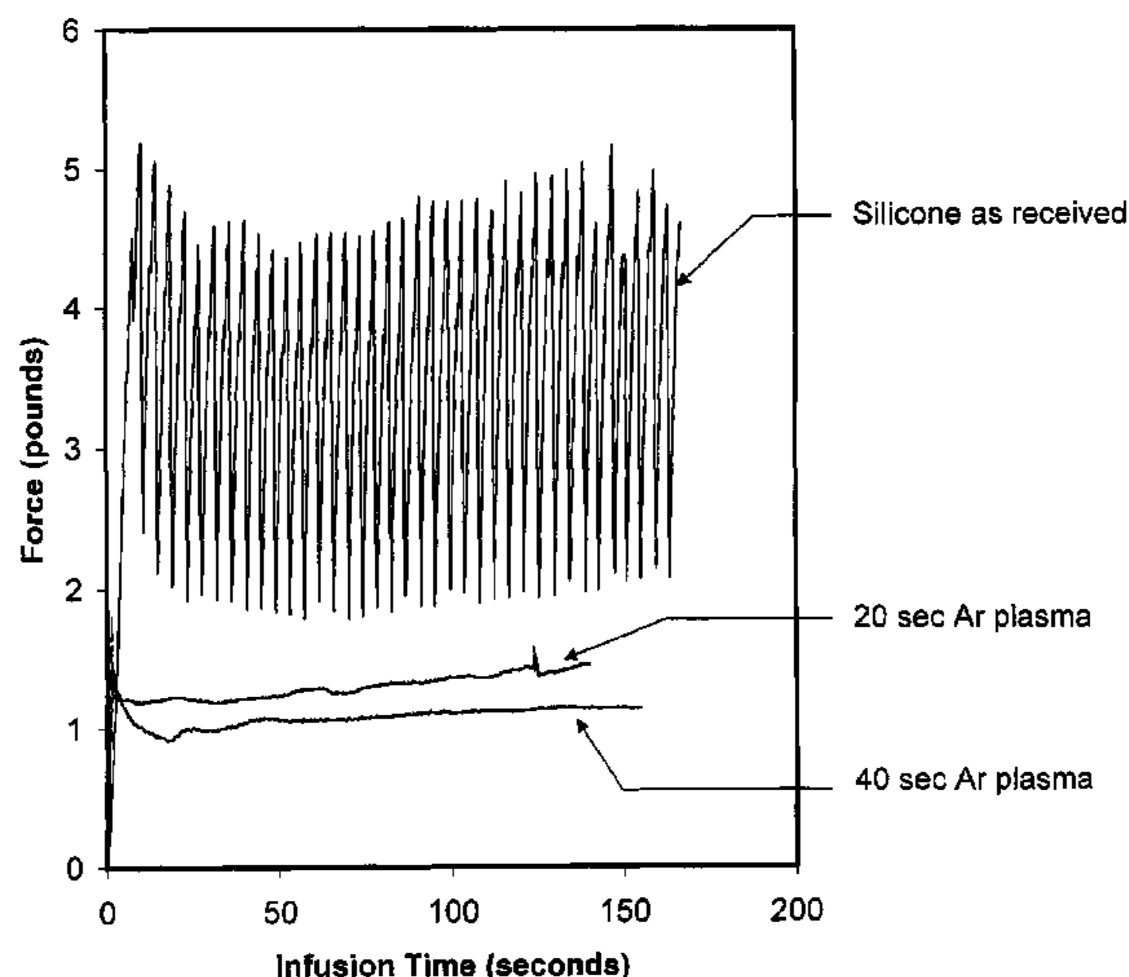
10 cc Plastic Syringes, Silicone Oil Infusion Rate 3 cc/min
