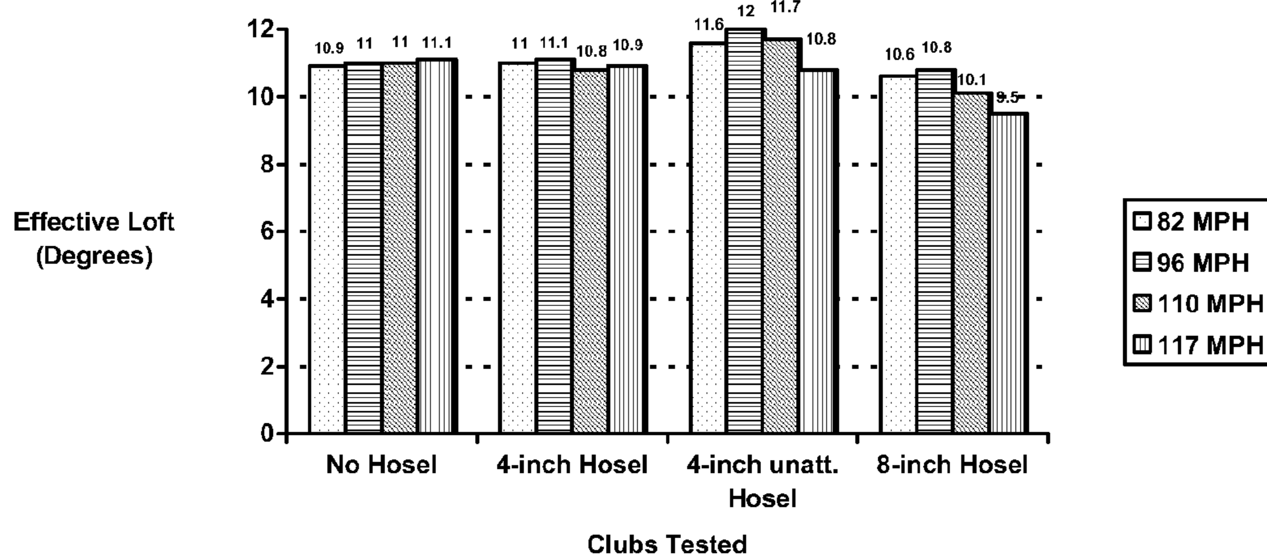
Effective Loft
