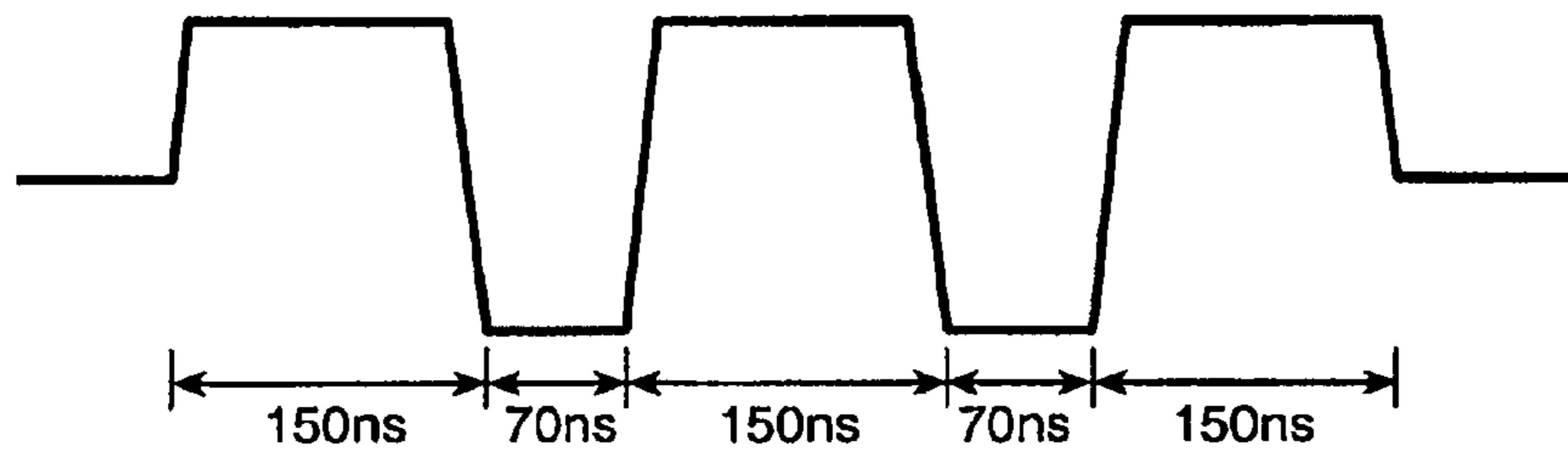
Transmitted Pulse
