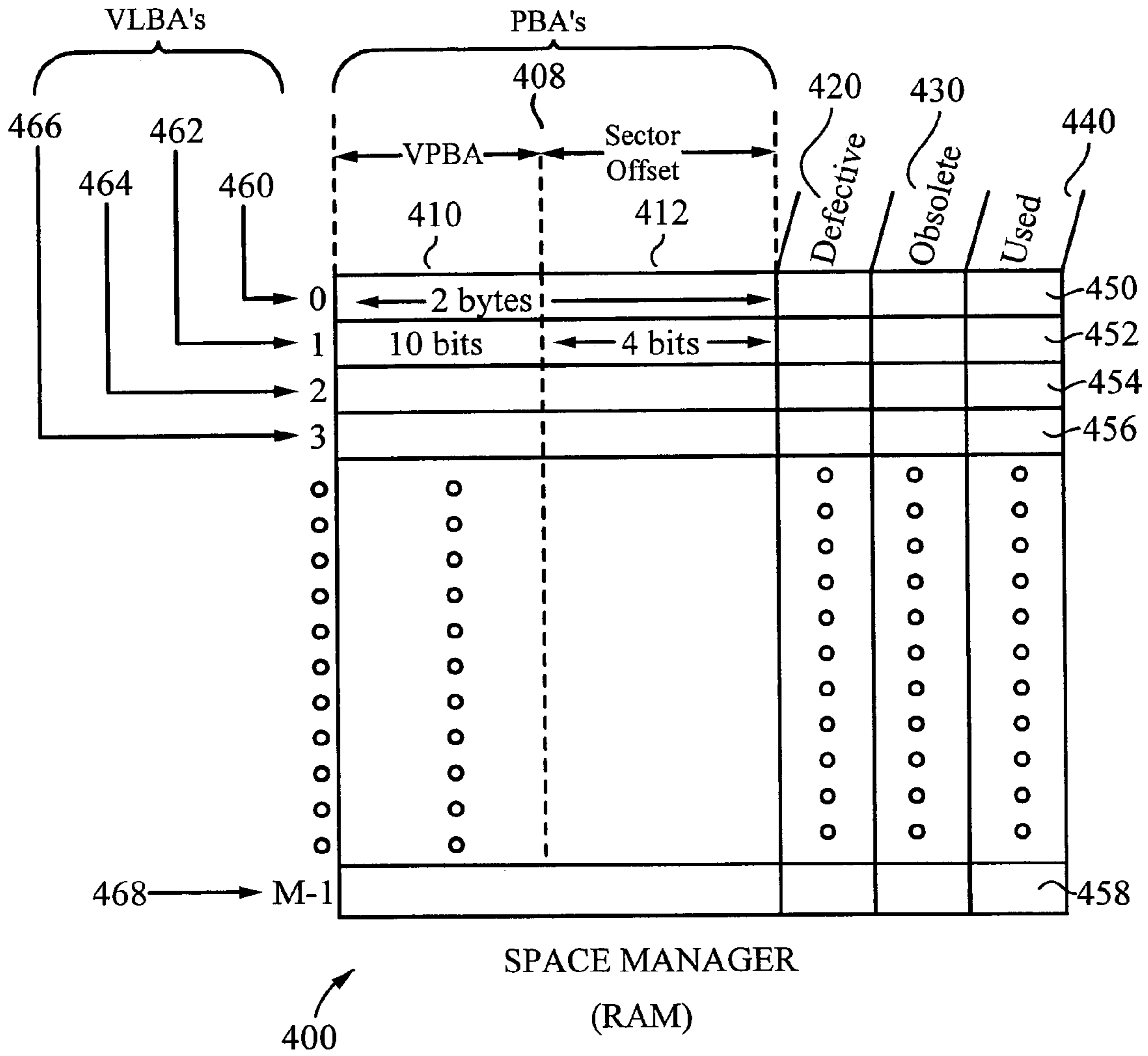
Fig. 4 (PRIOR ART)
