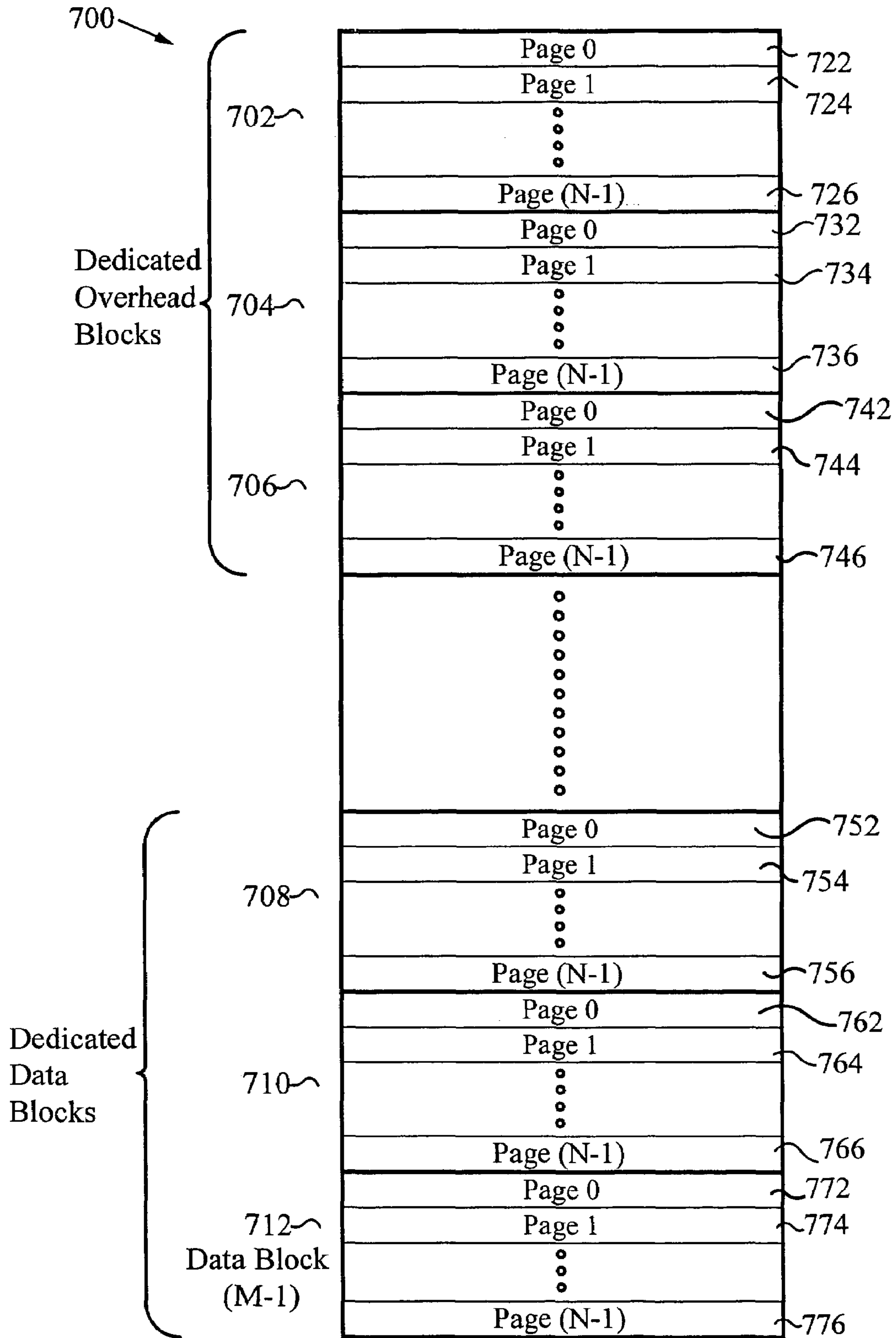
Flash Memory Array
