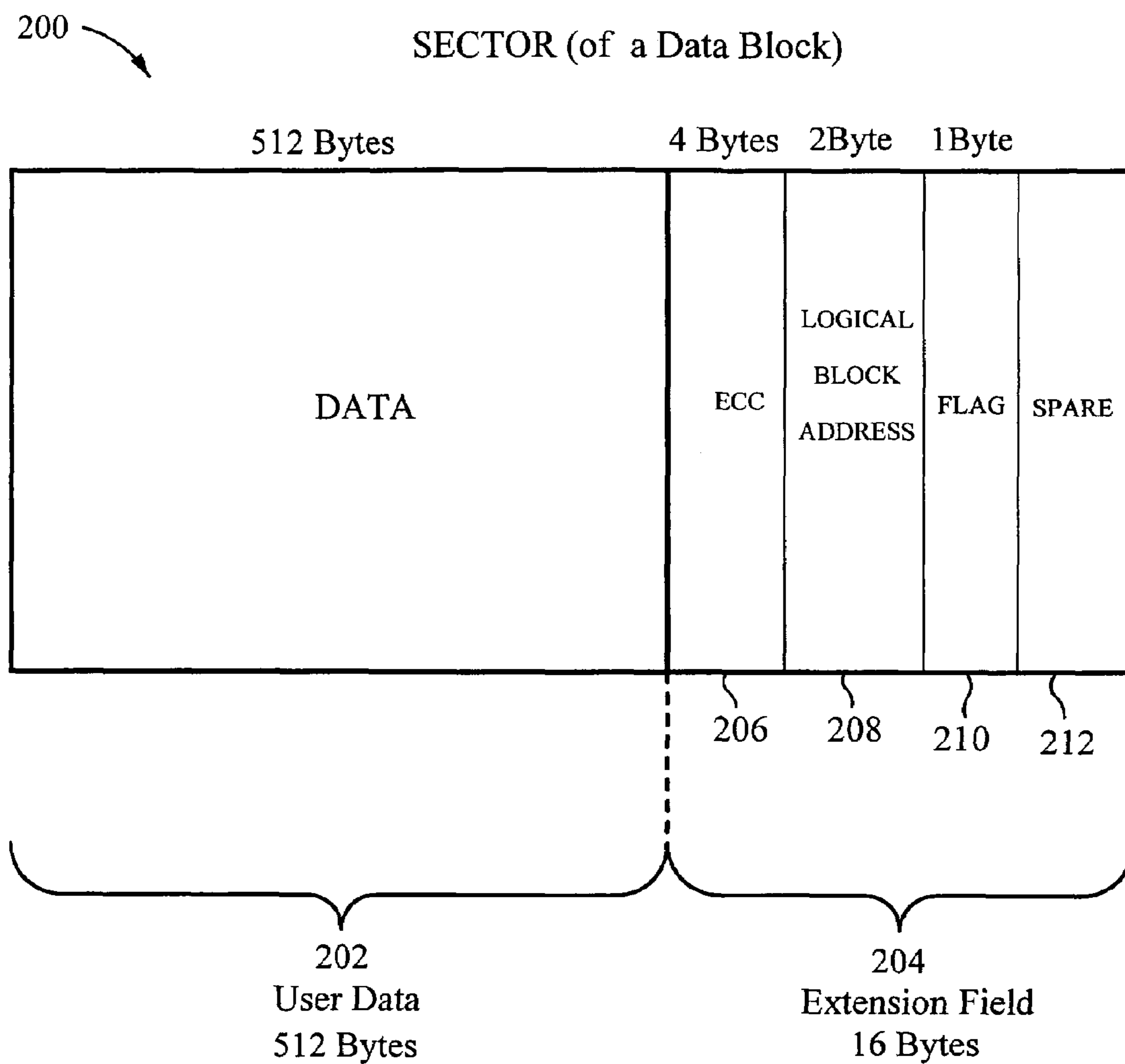
Fig. 2 (PRIOR ART)
