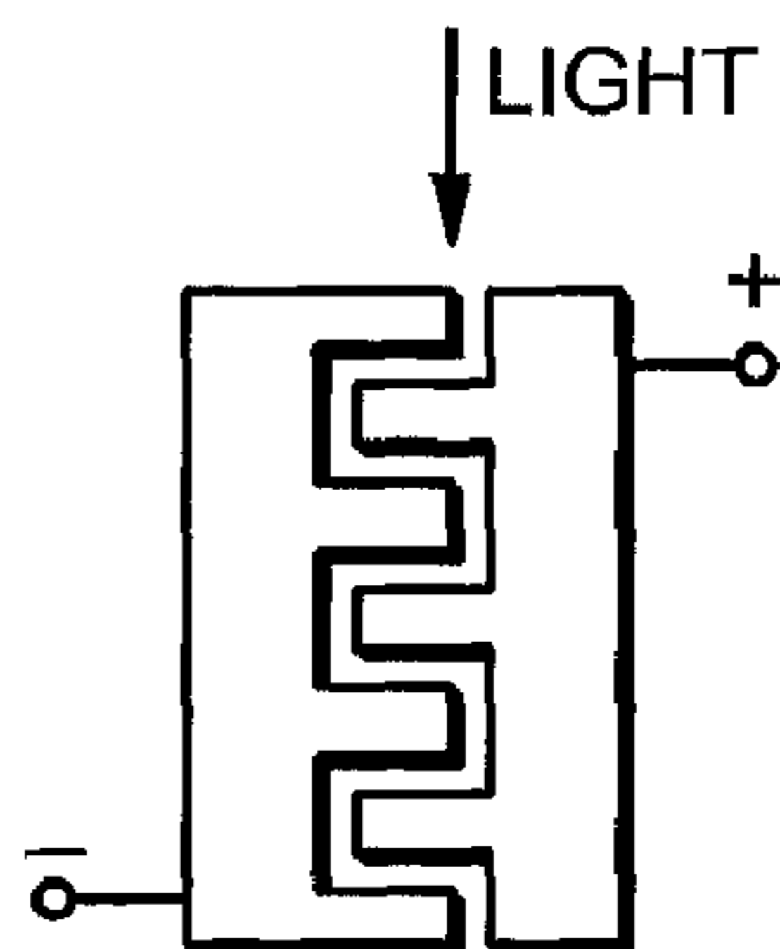
FIG. 27 (PRIOR ART)
