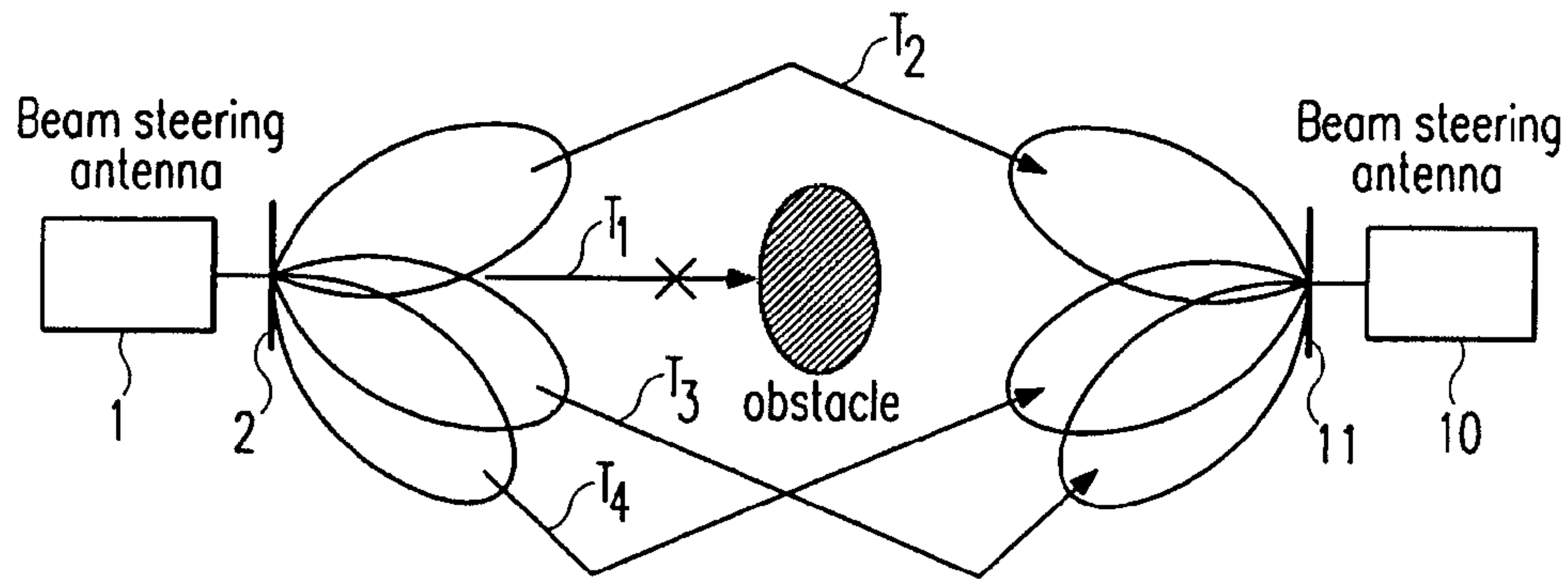
Fig. 1 : System concept
