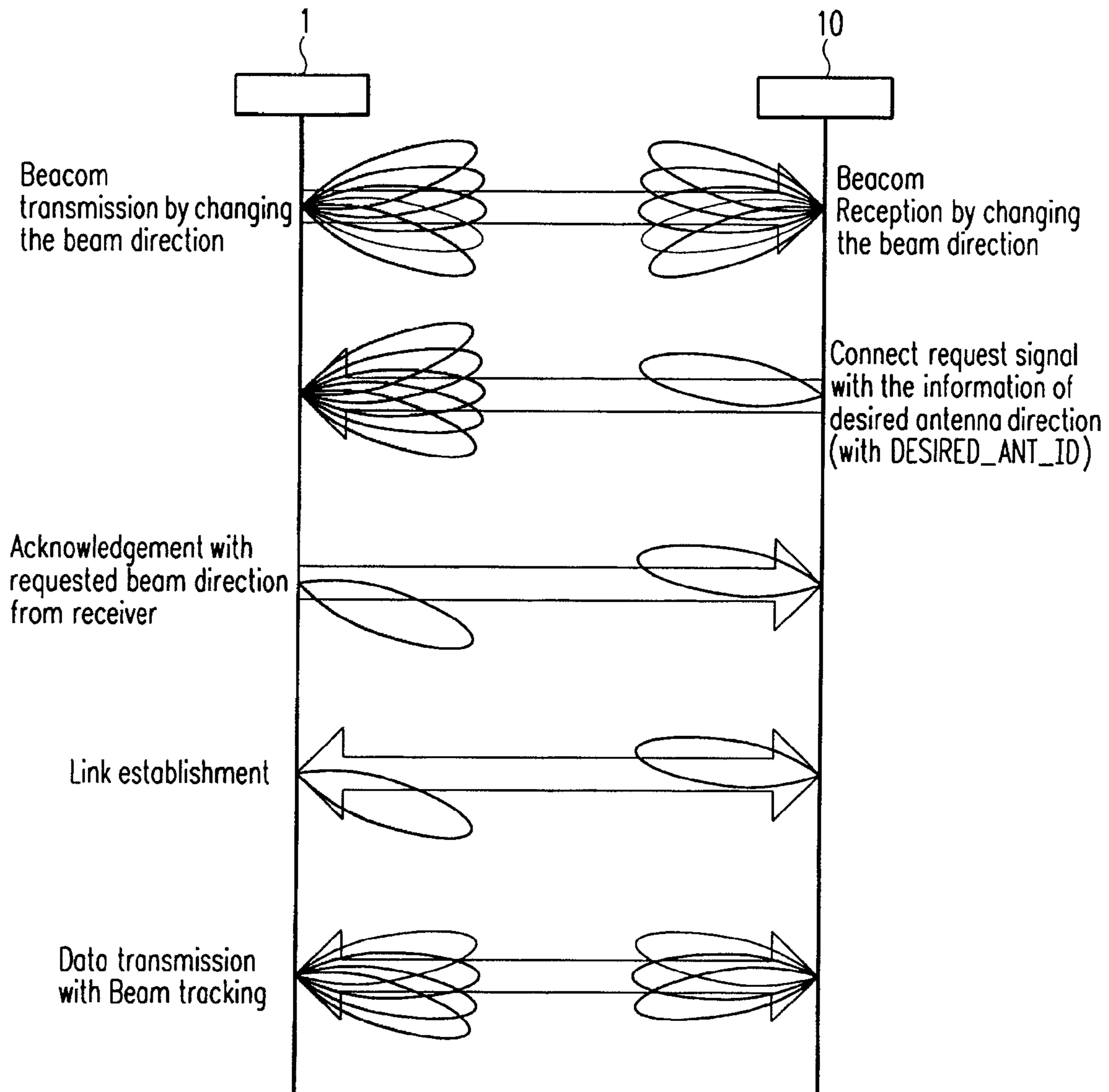
Fig. 5: Sequence chart of the invention
