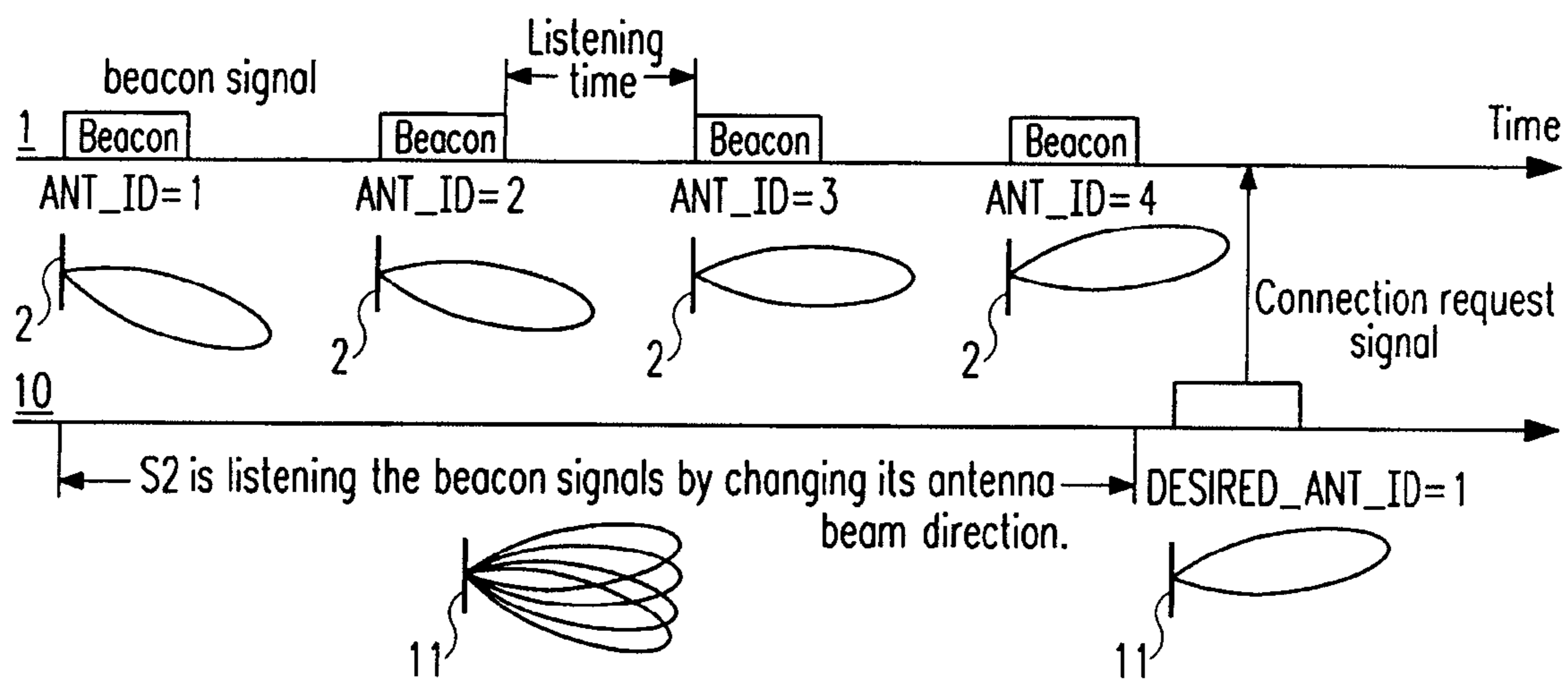
Fig. 4 : Example of initial sequence (Beacon transmission and connection request signal)
