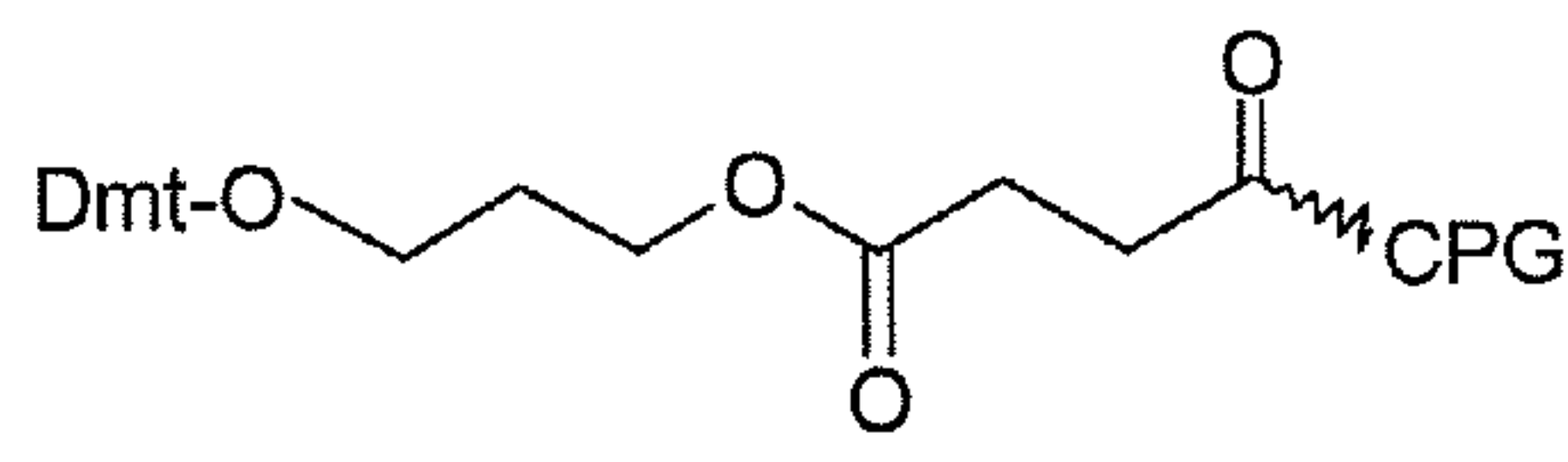
3'-Spacer-C3 support 2
