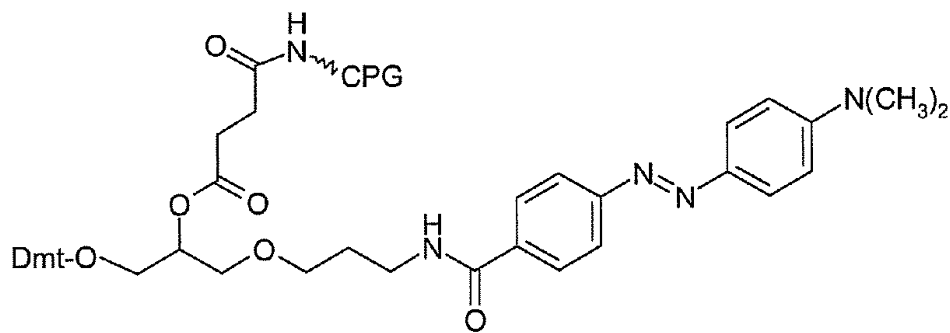
DABCYL support 6
