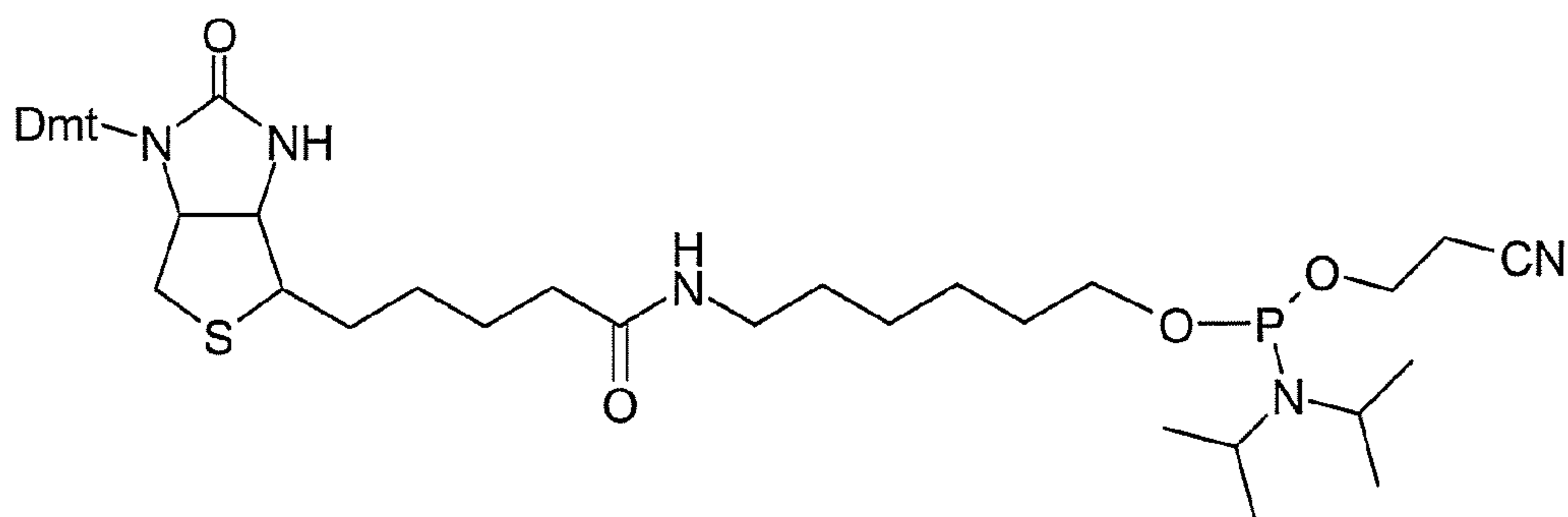
Biotin phosphoramidit 5 (monofunctional)
