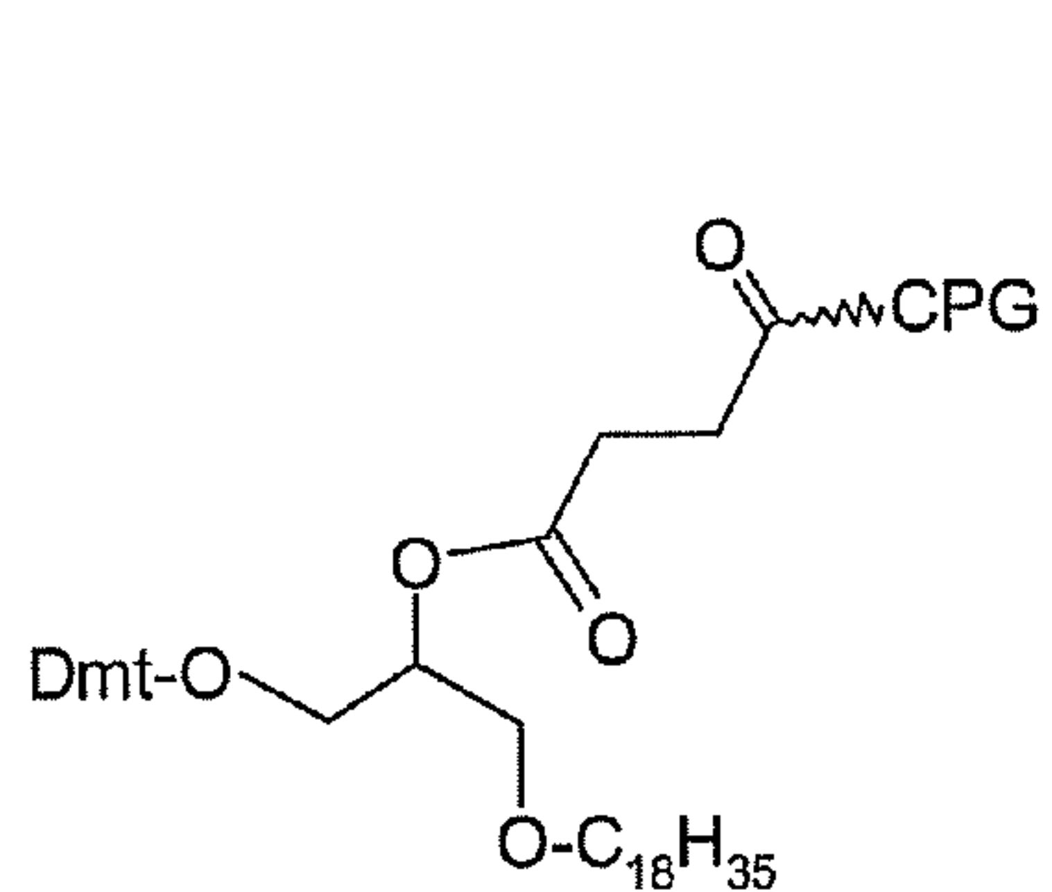
3'-Batyl support 4
