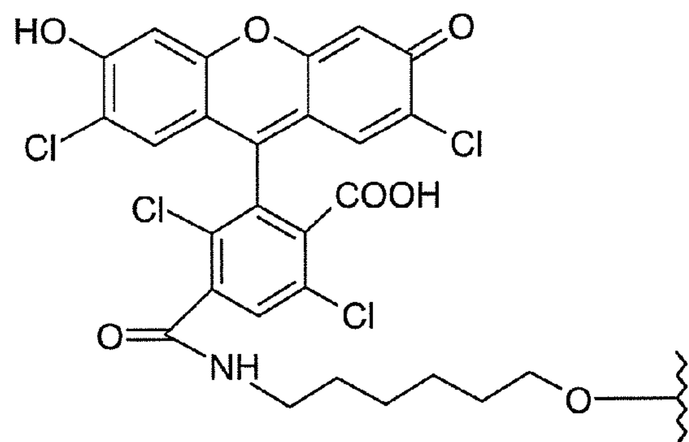
Tetrachlorofluorescein
