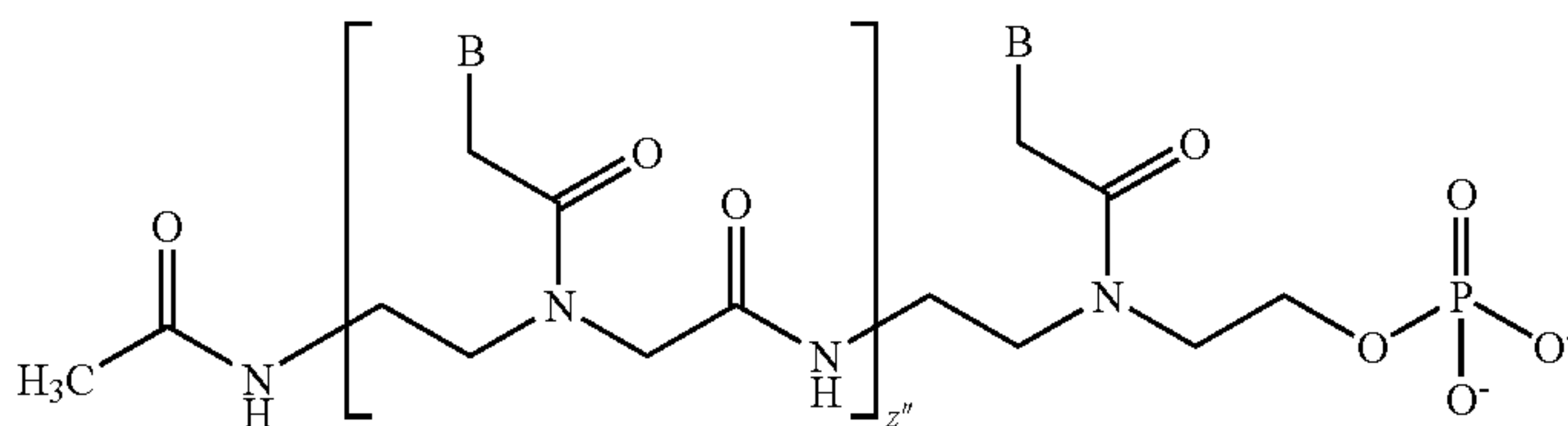
PNA-2:
