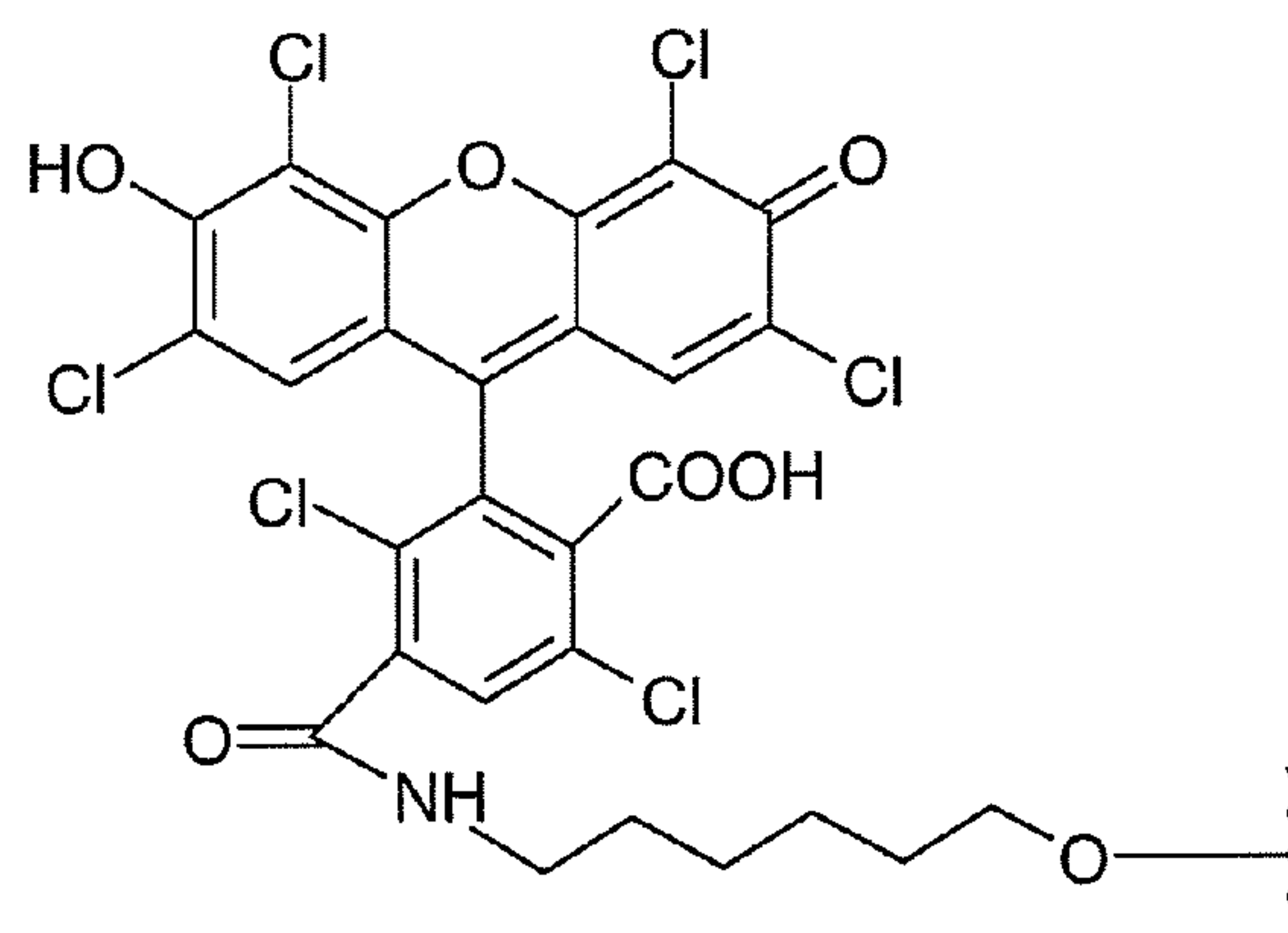
Hexachlorofluorescein
