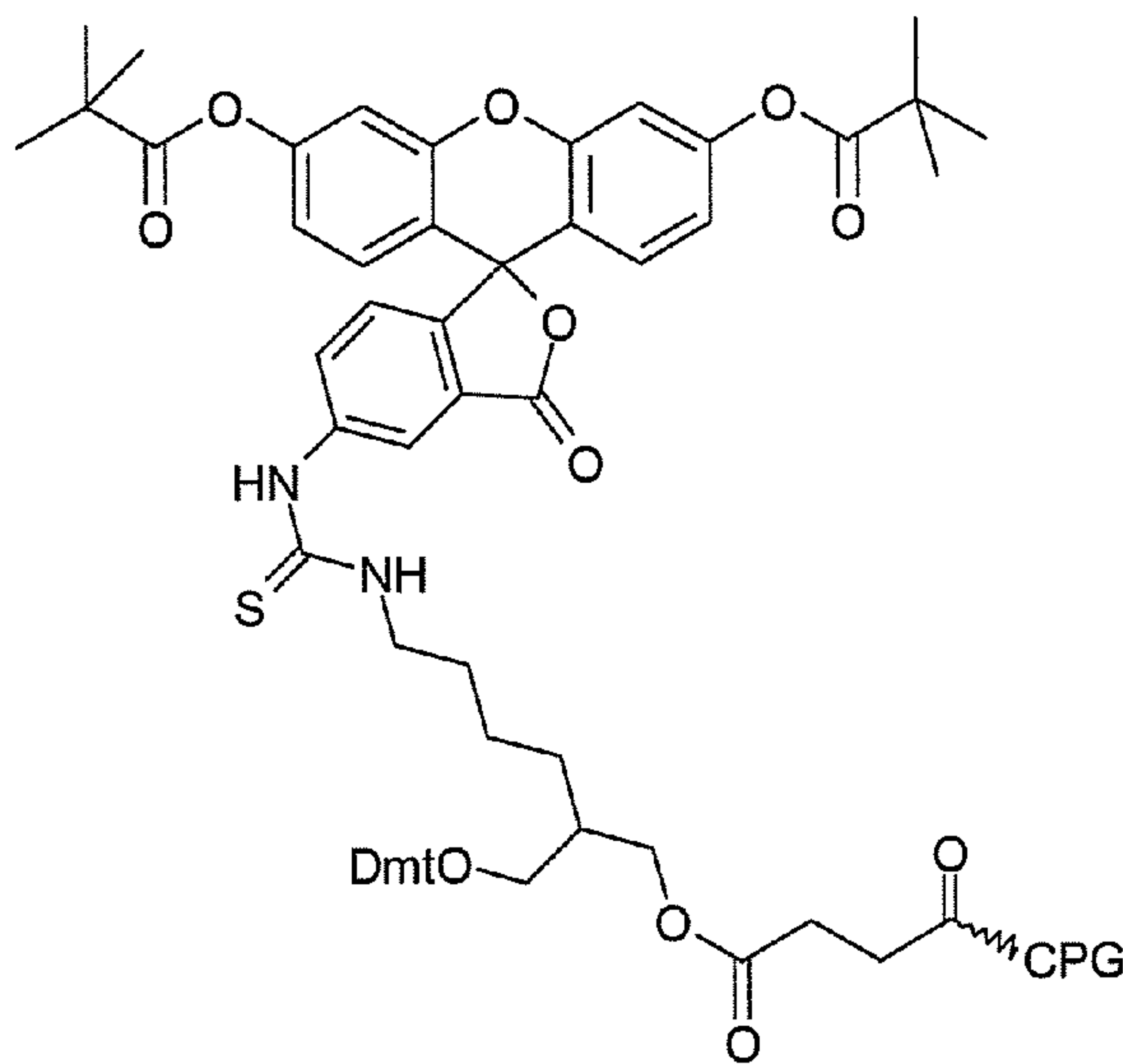
Fluorescein support 3
