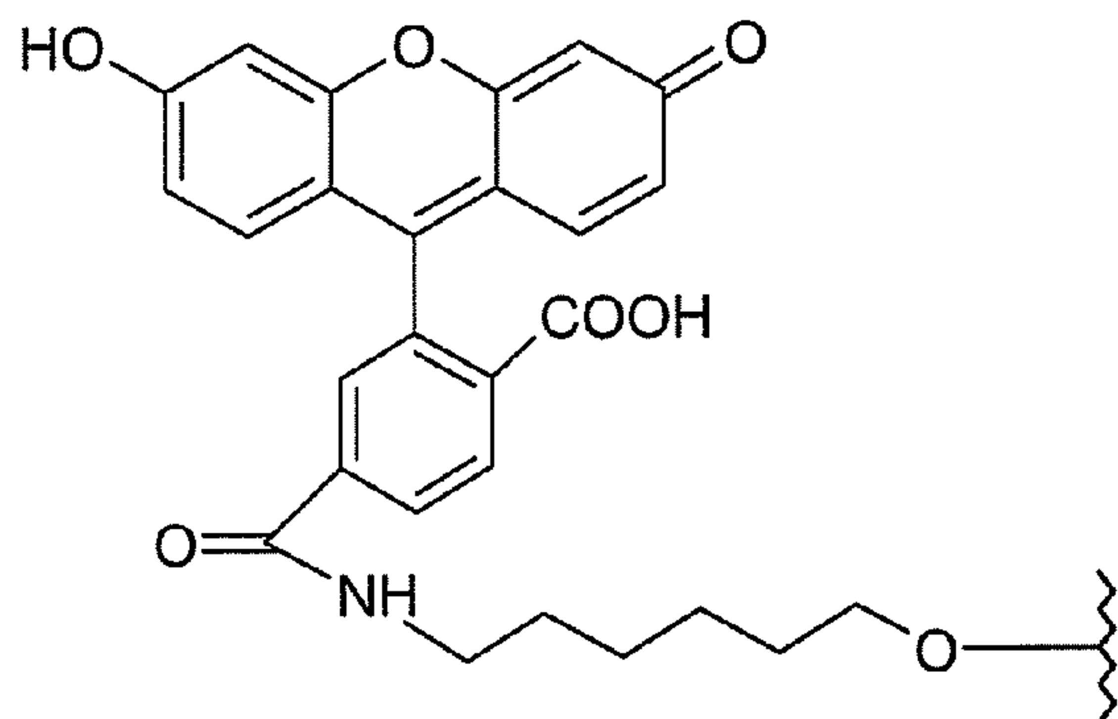
Fluorescein (Amide)
