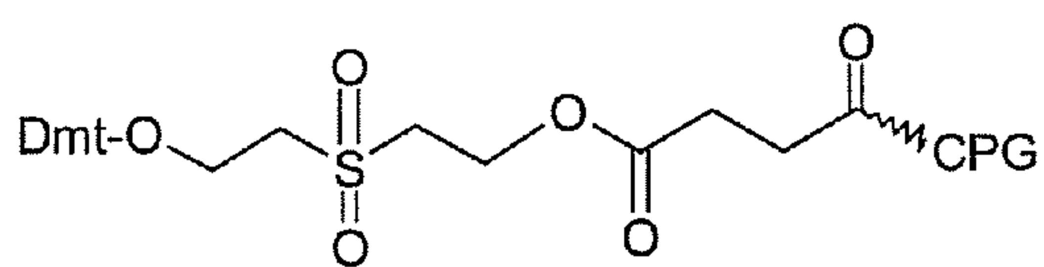
Bishydroxyethylsulfonyl support 1
