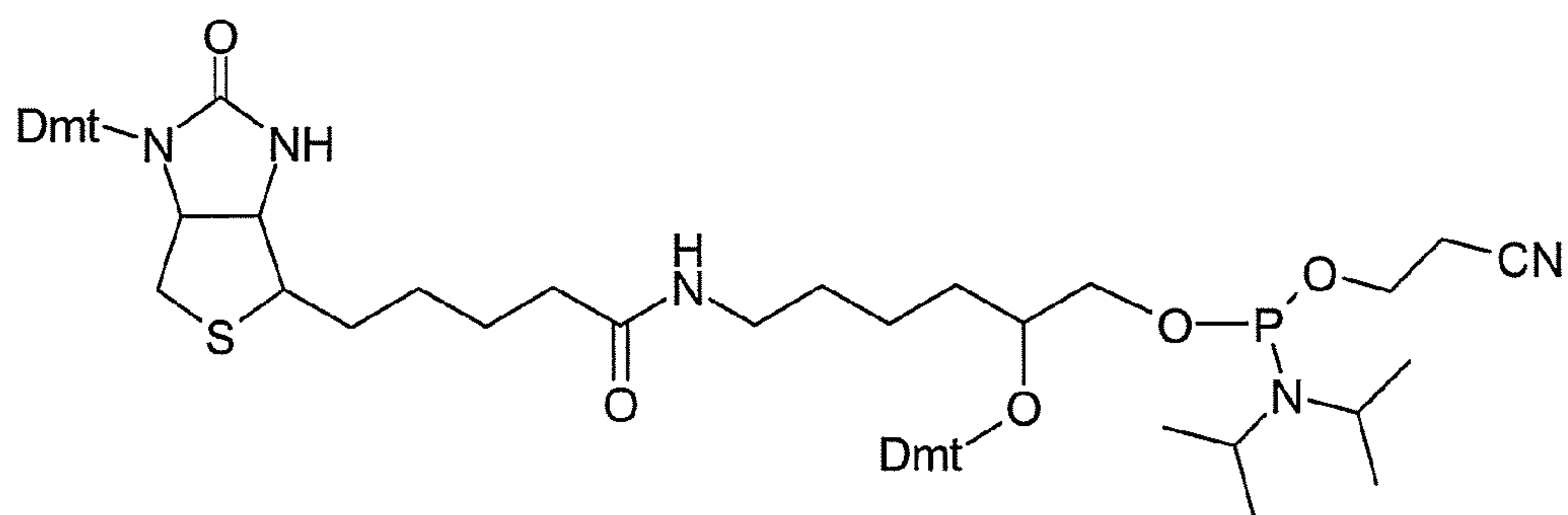
Biotin phosphoramidit 6 (bifunctional)
