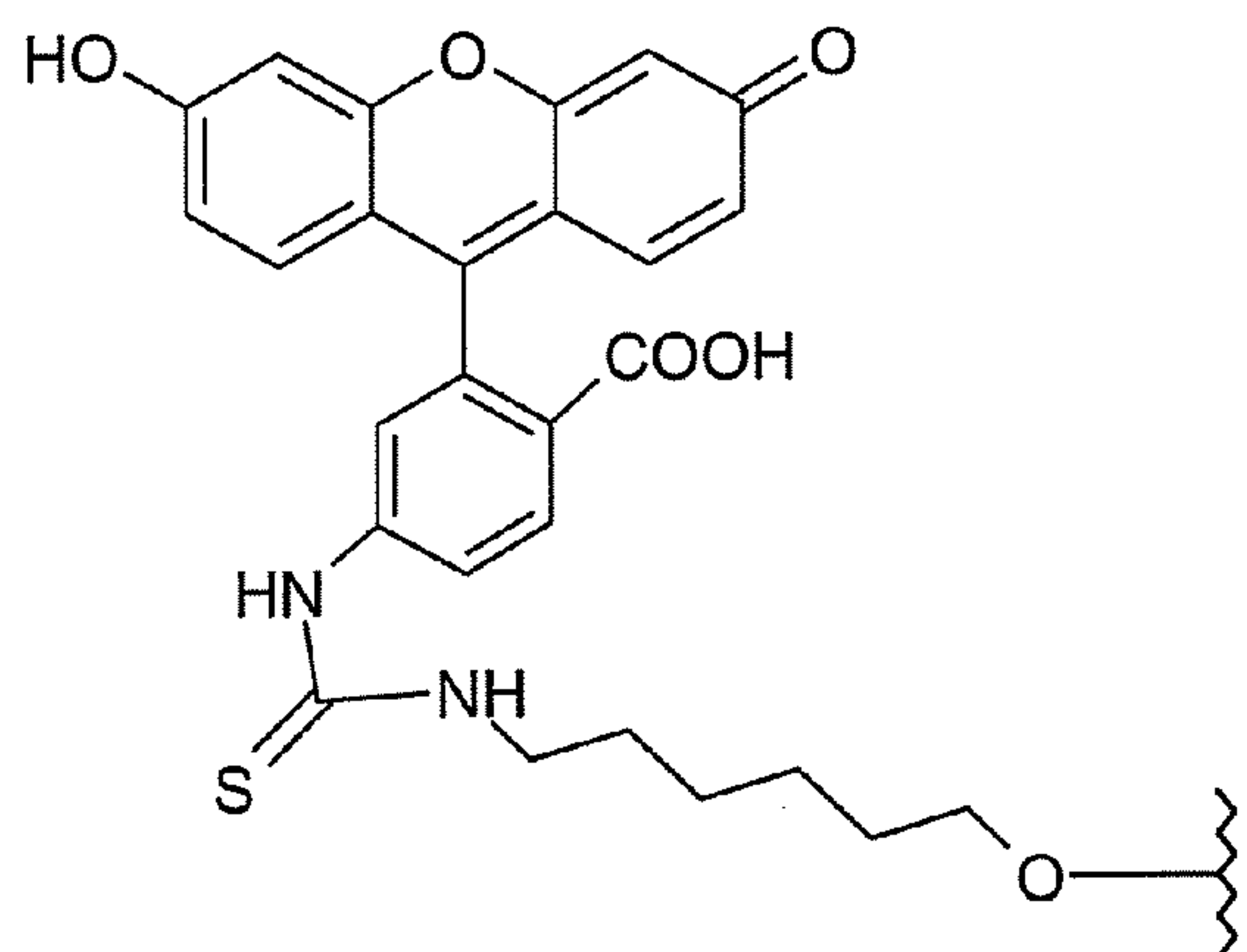
Fluorescein (Thiourea)
