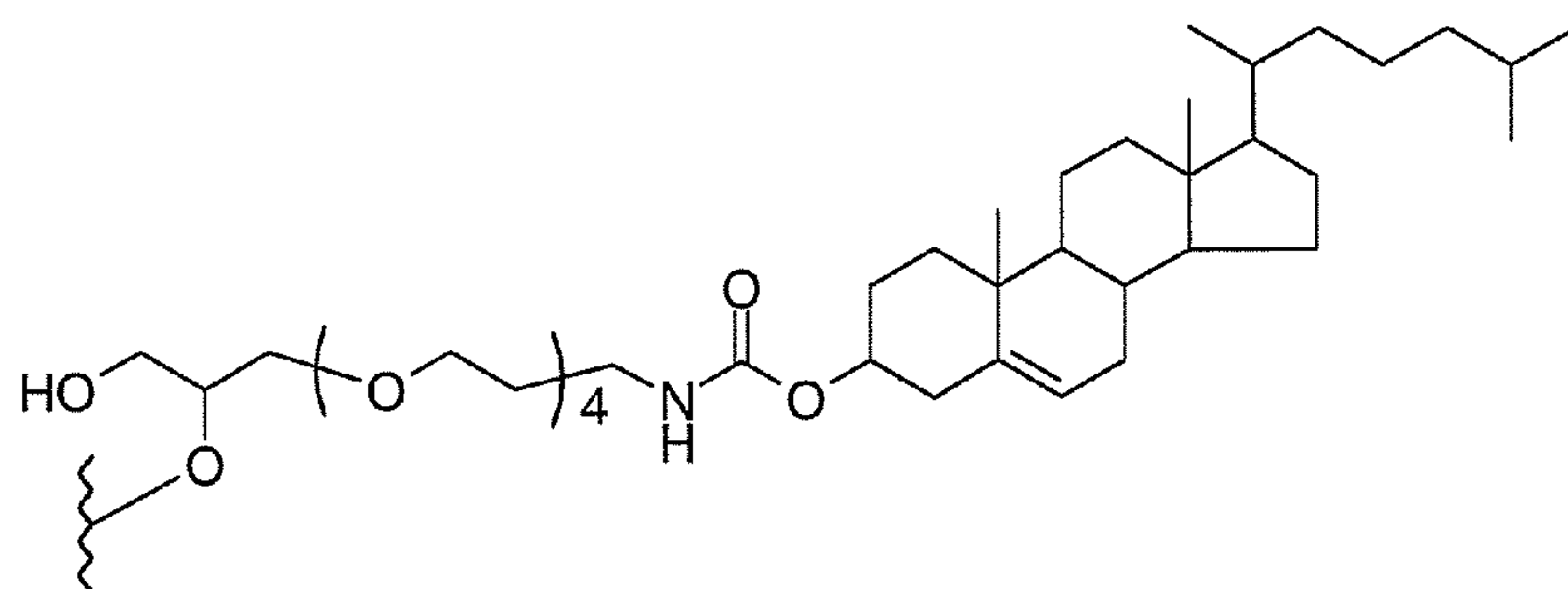
Cholesterol
