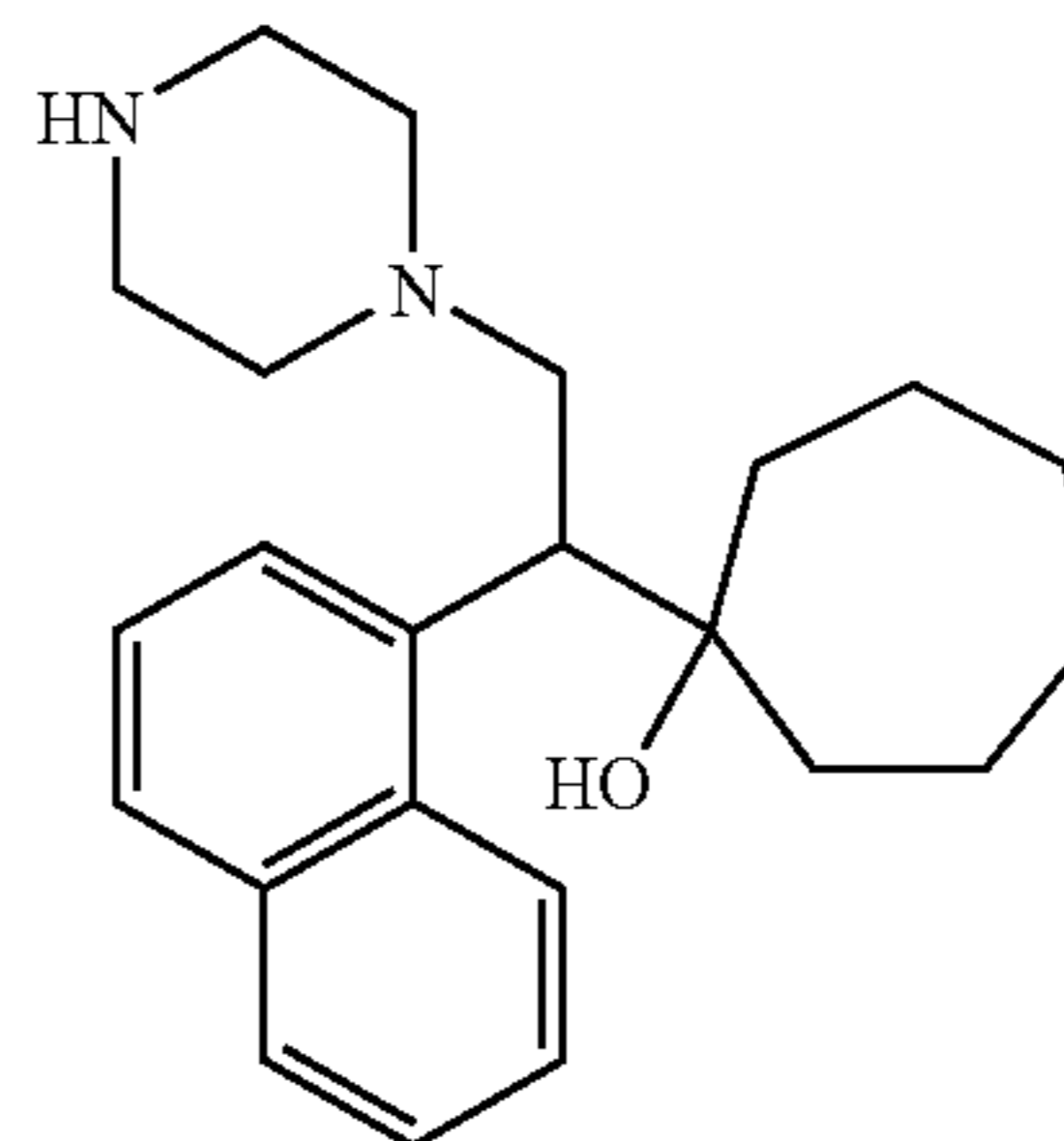
1-[1-(1-naphthyl)-2-piperazin-1-ylethyl]cycloheptanol dihydrochloride
