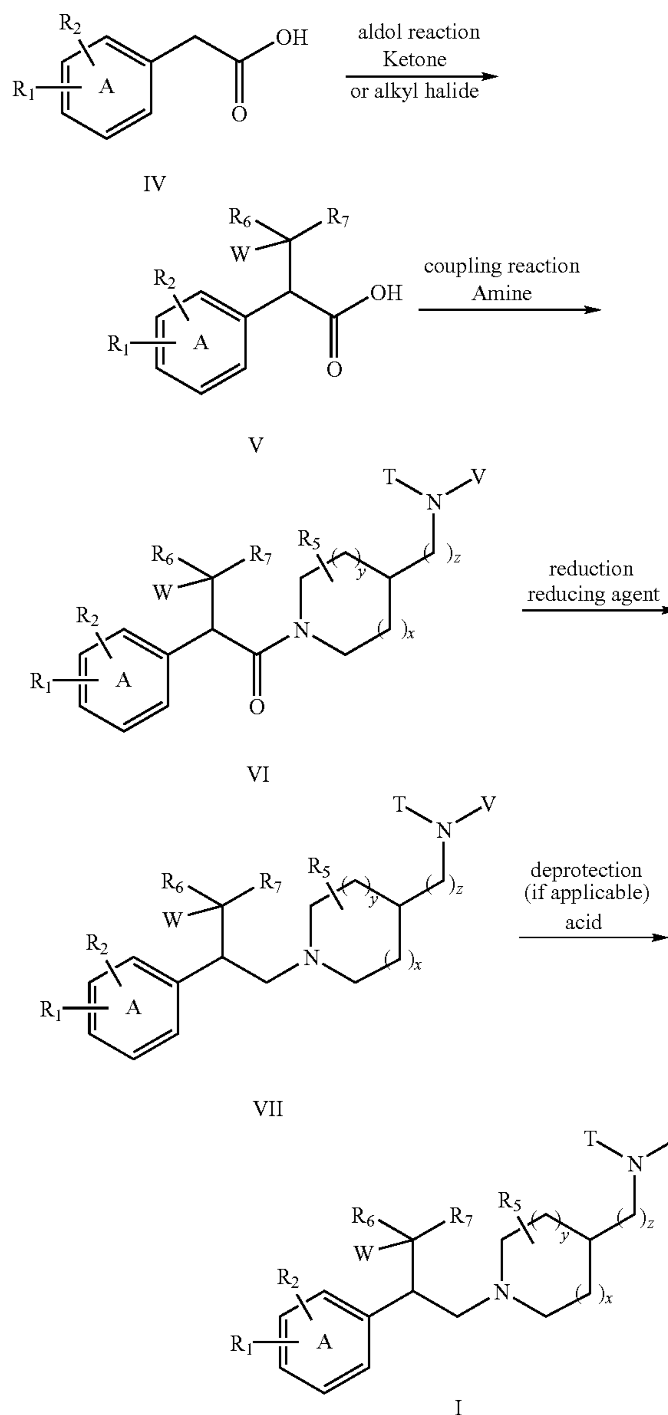
Scheme 1
