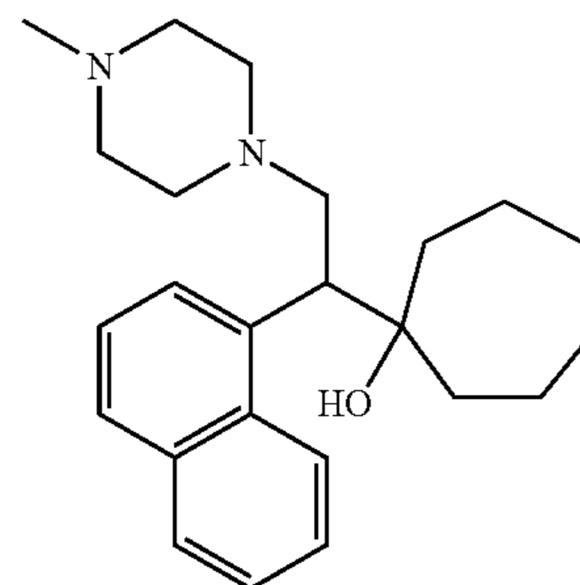
1-[2-(4-methylpiperazin-1-yl)-1-(1-naphthyl)ethyl]cycloheptanol dihydrochloride
