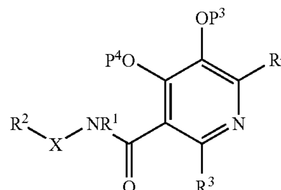
[Chemical formula 47]
