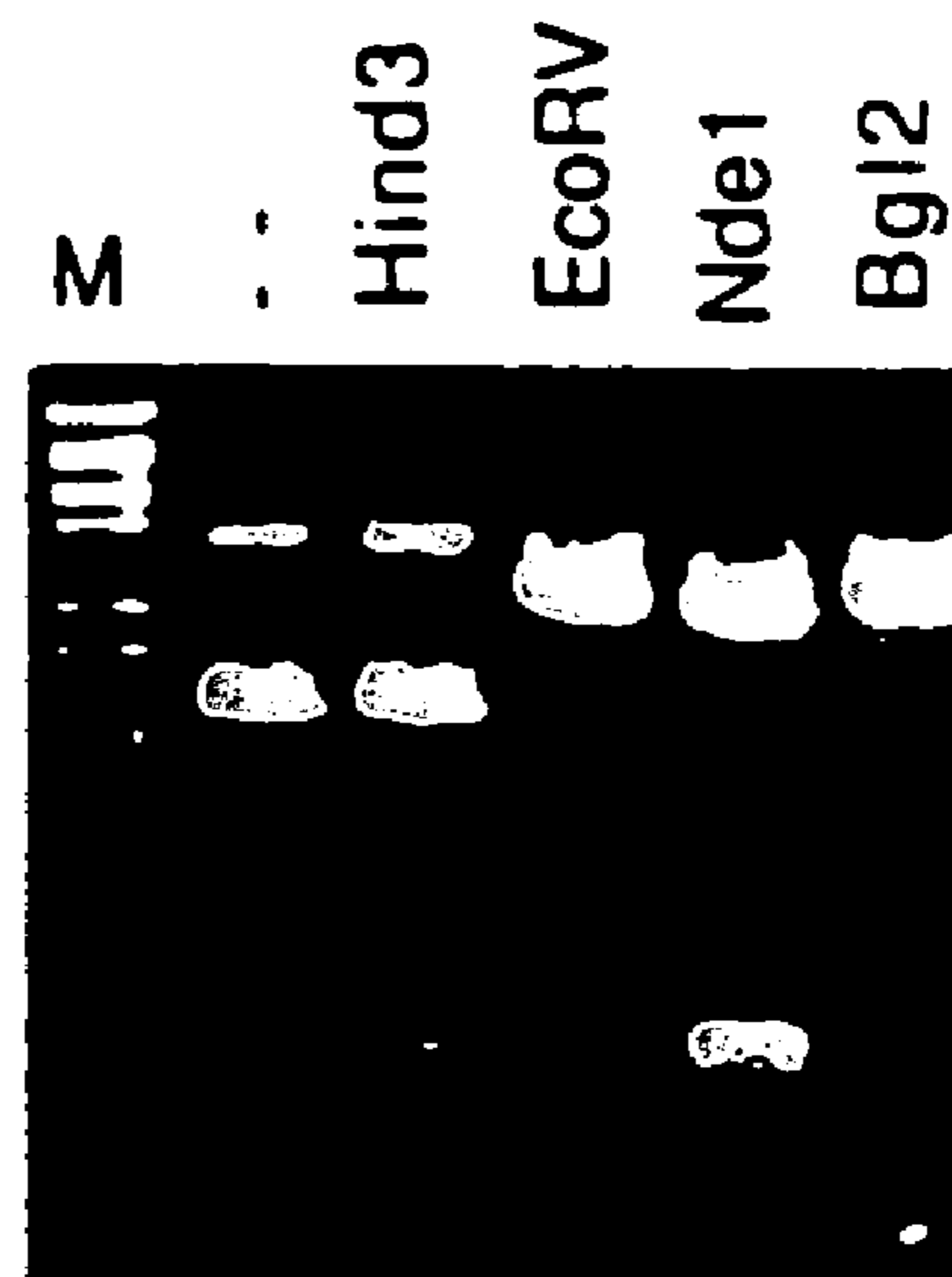
pUC-T11
