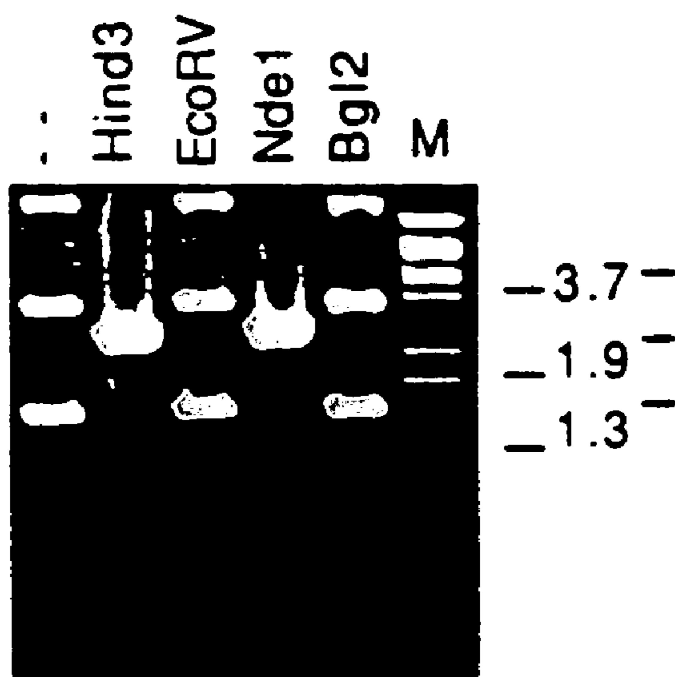
pUC18
