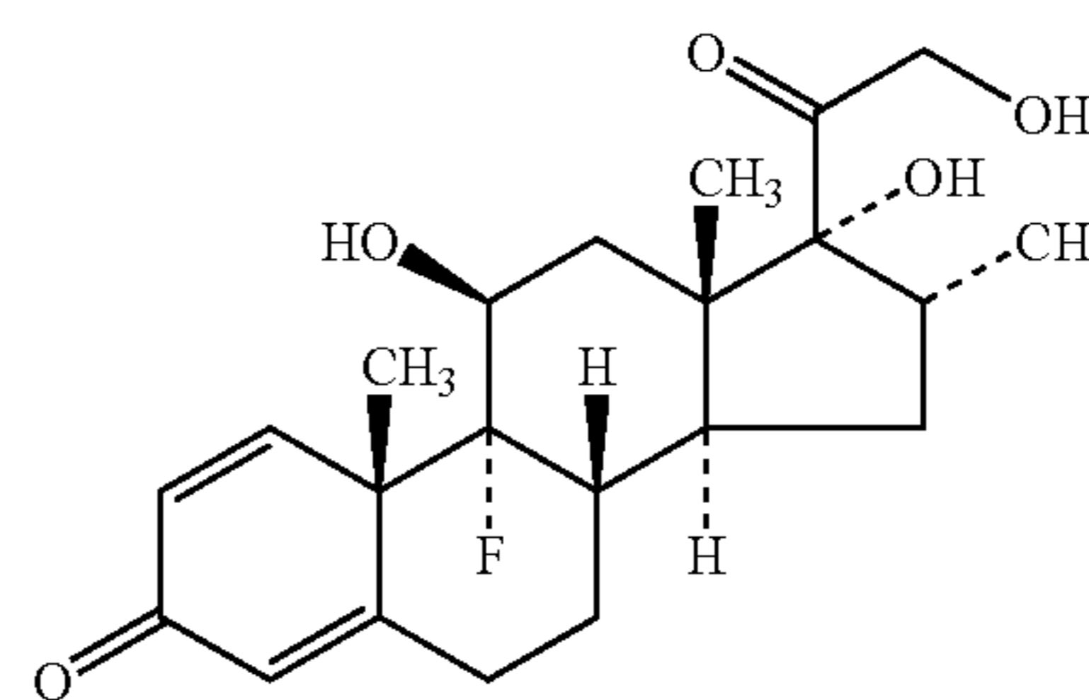
Dexamethasone
