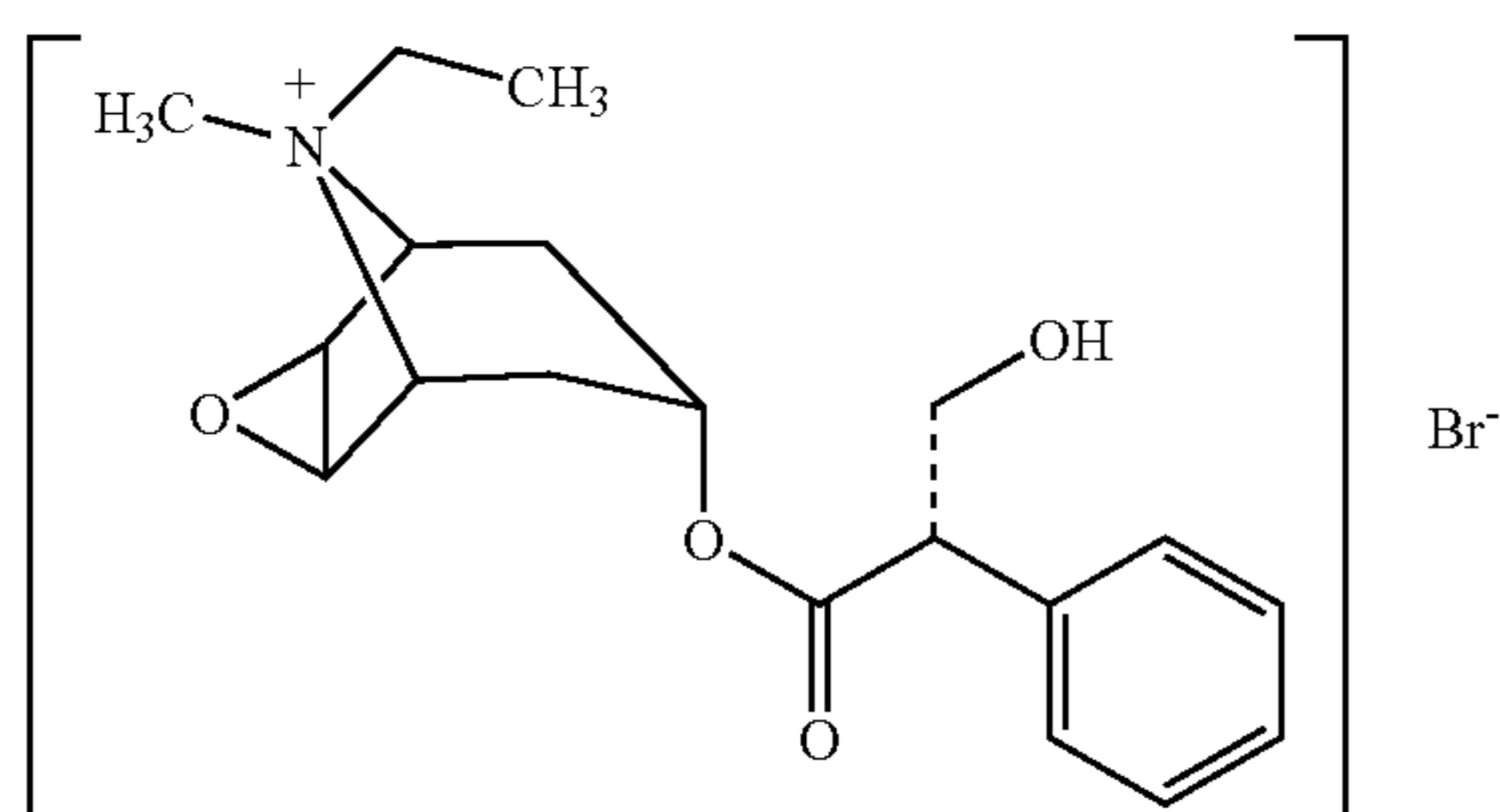
Oxotropium Bromide
