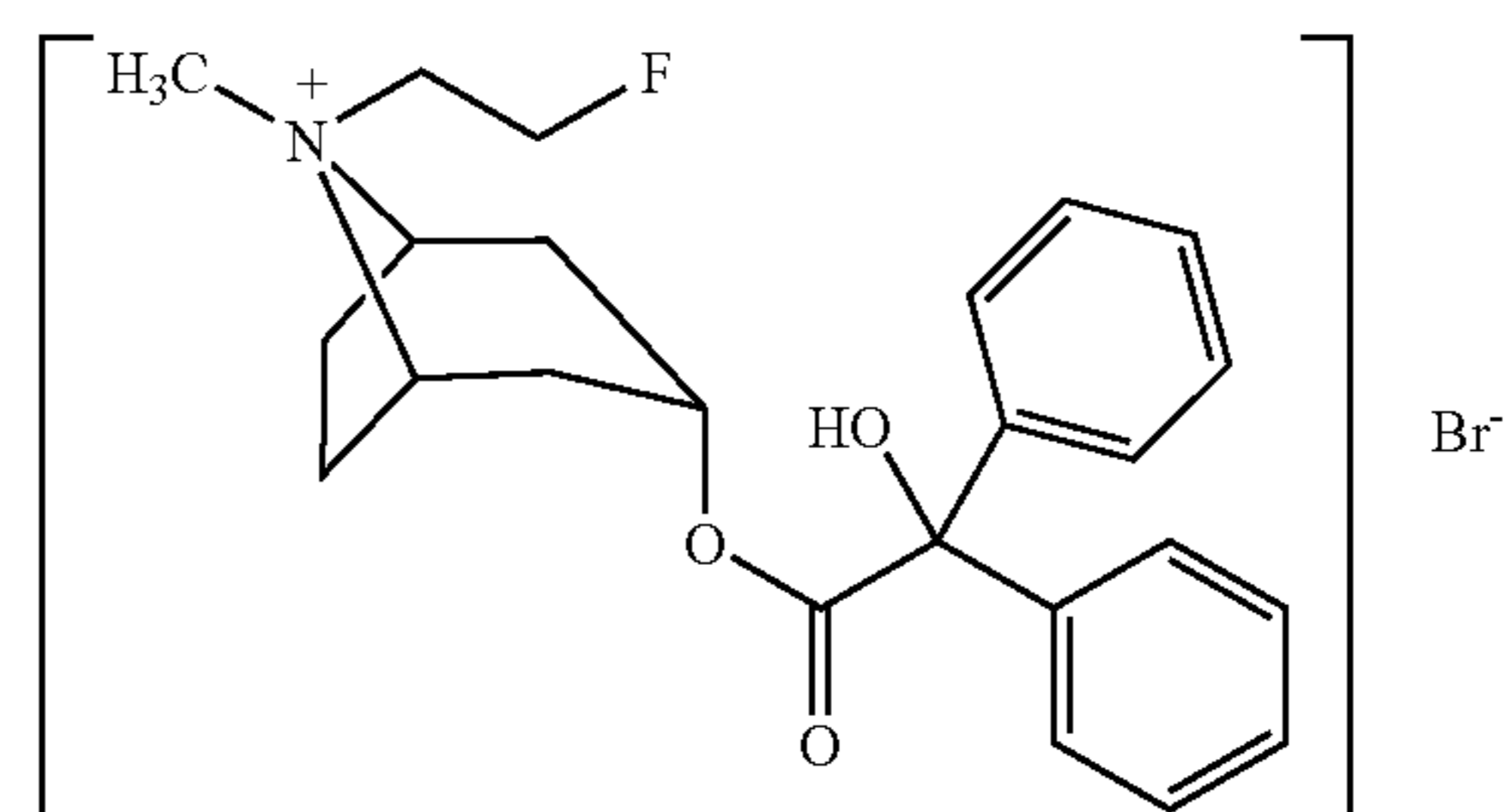
Flutropium Bromide
