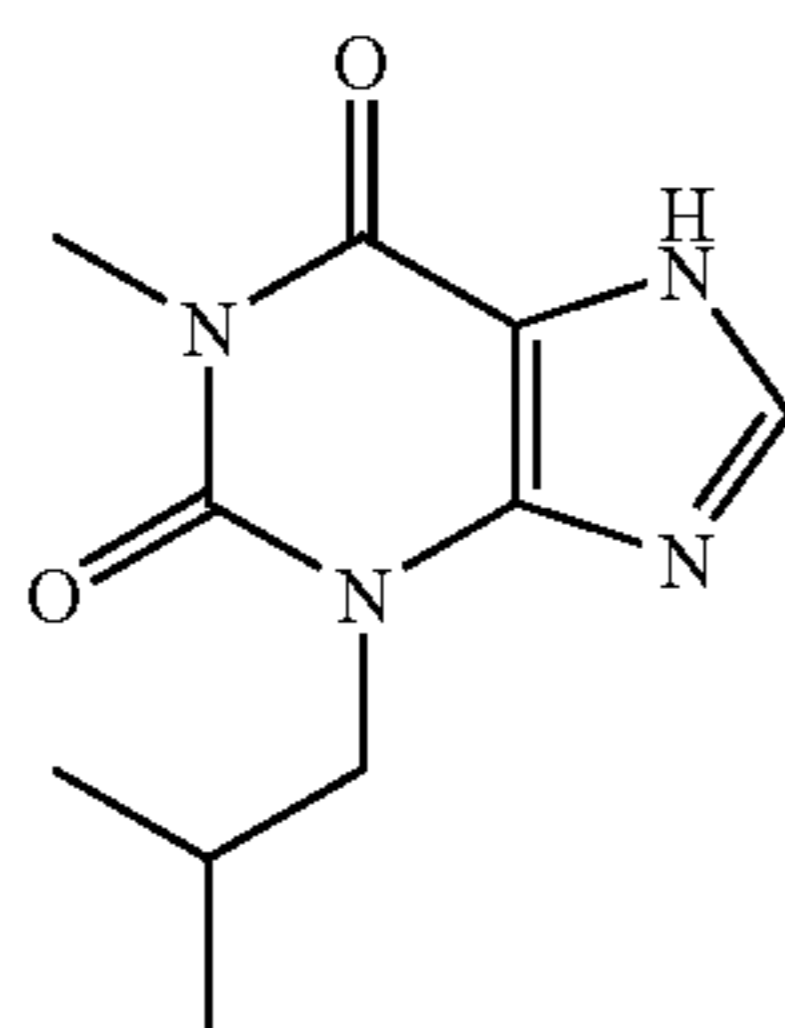
IBMX
