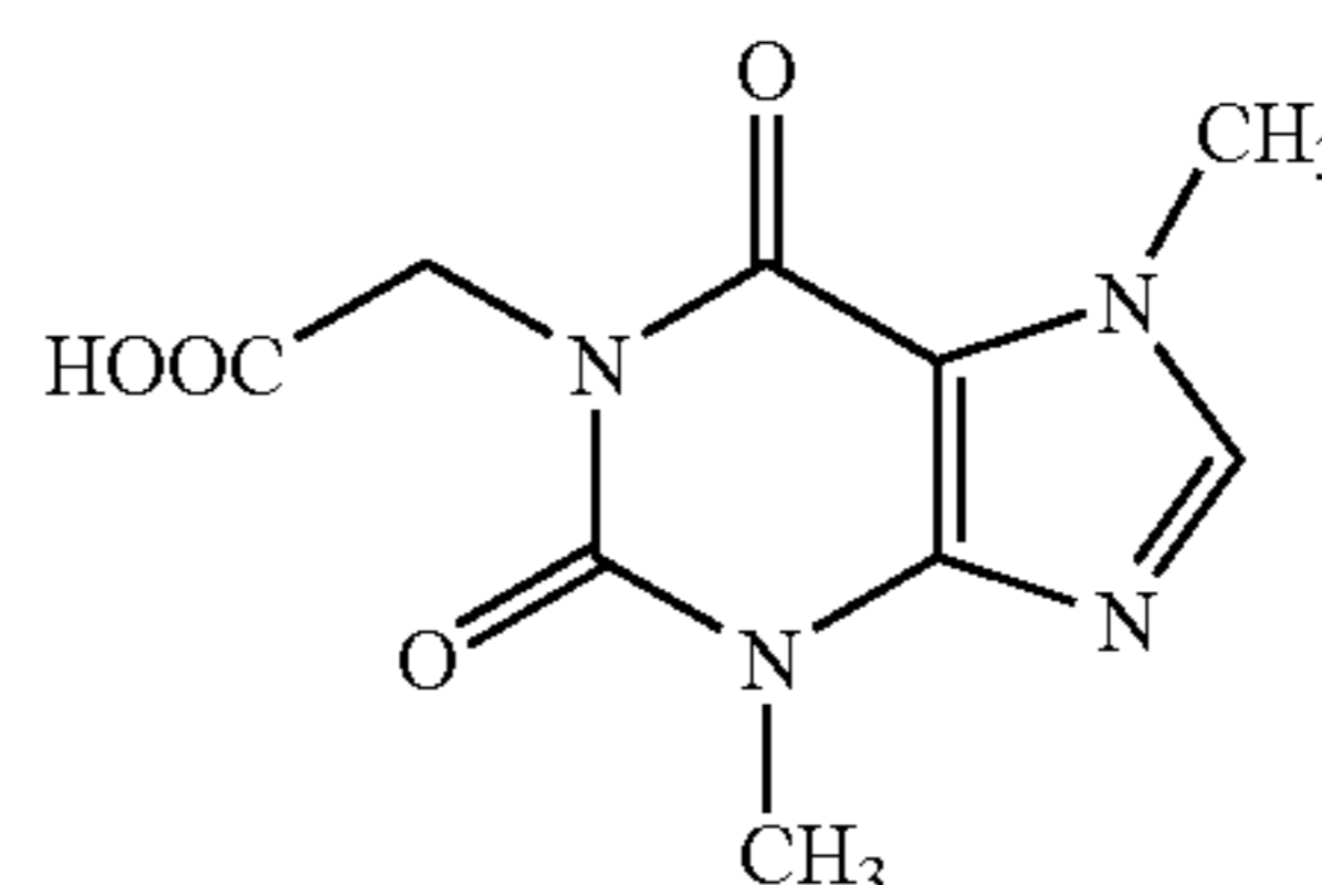
Theobromine-1-acetic Acid
