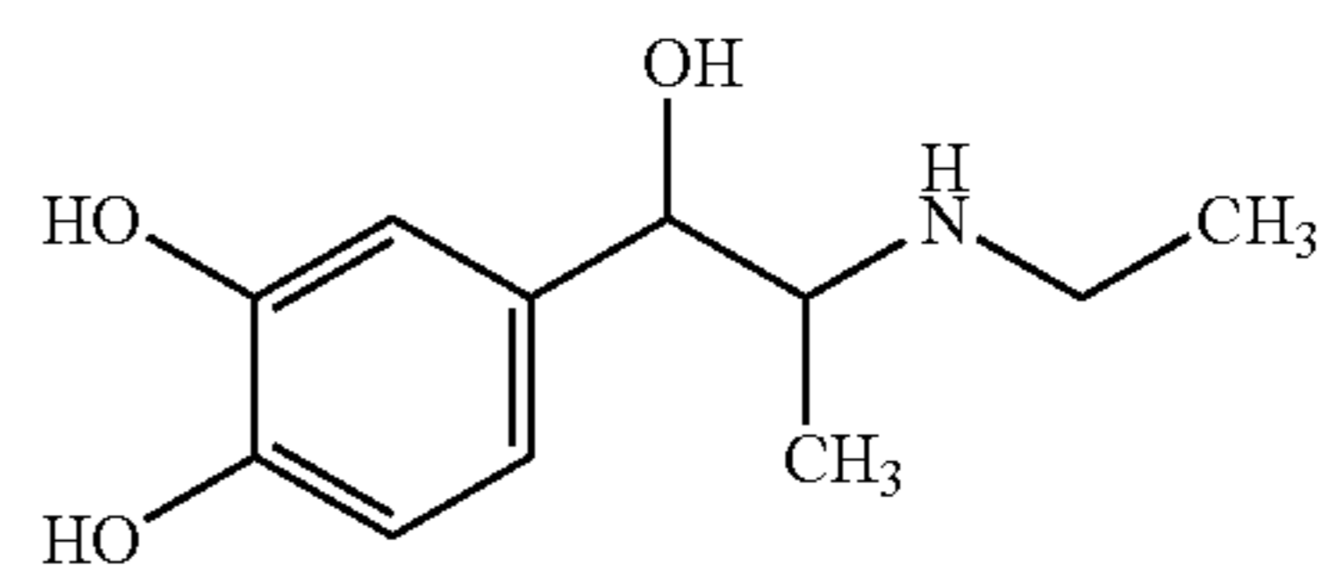
Dioxethedrine
