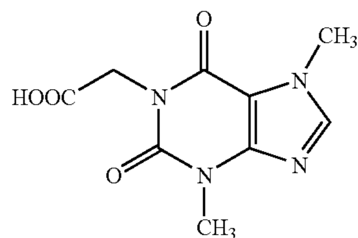
Theobromine-1-acetic Acid
