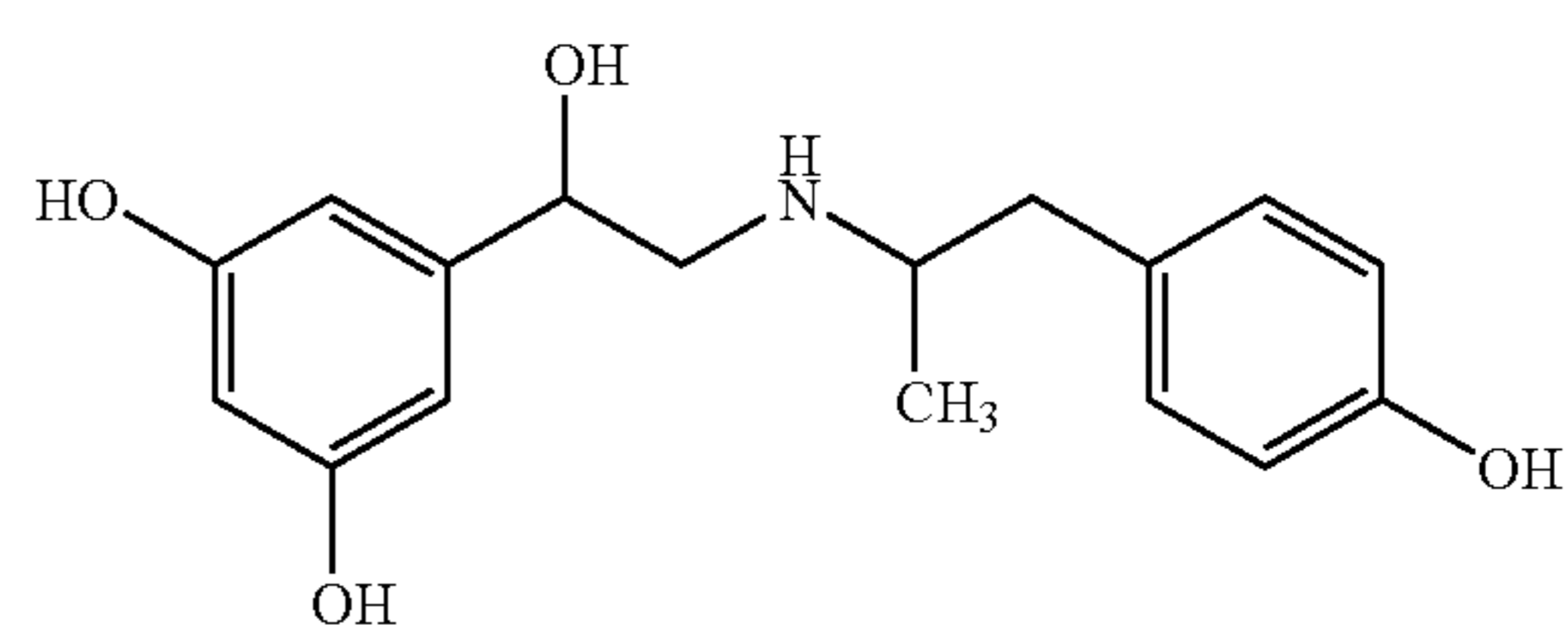
Fenoterol
