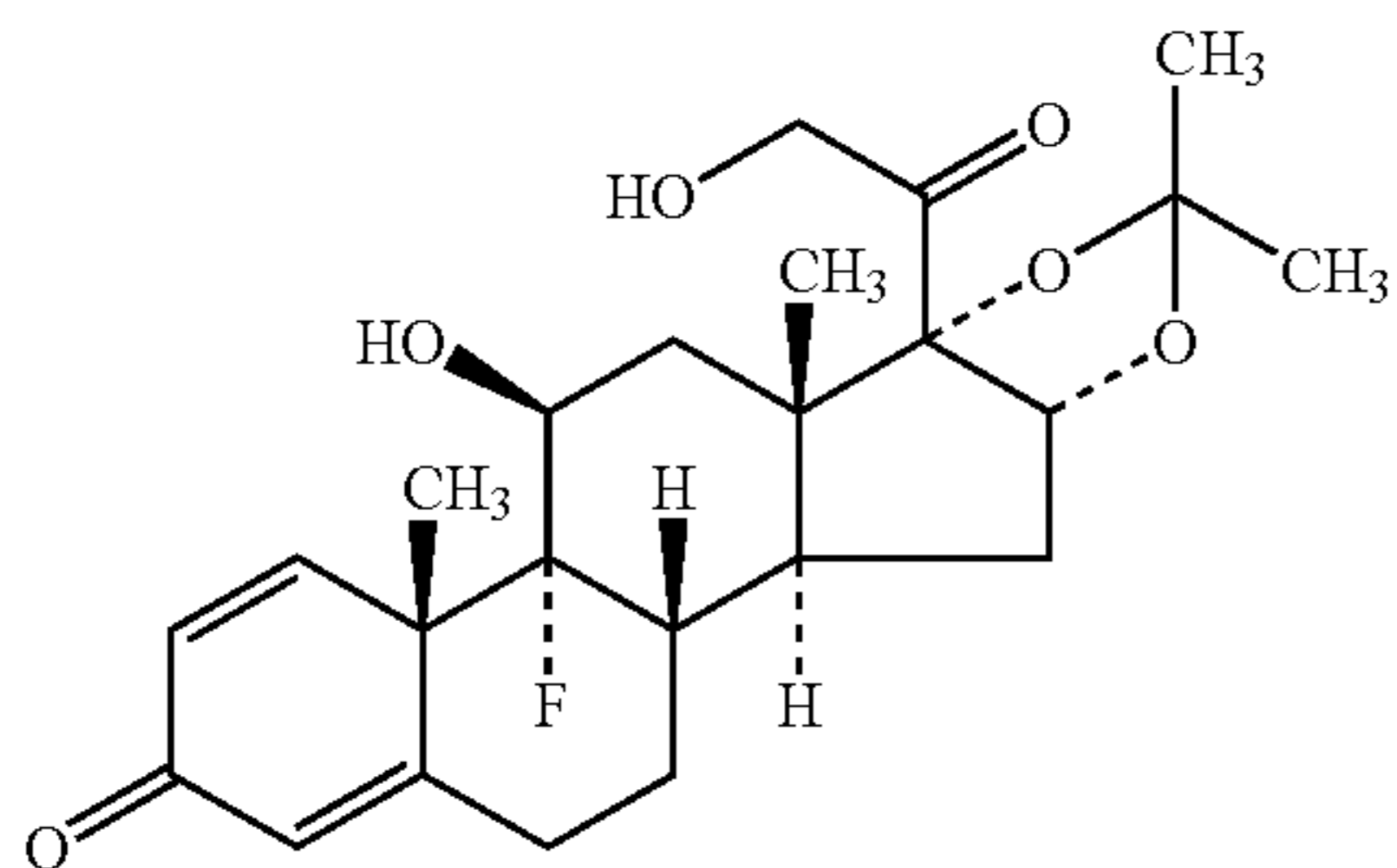
Triamcinolone Acetonide
