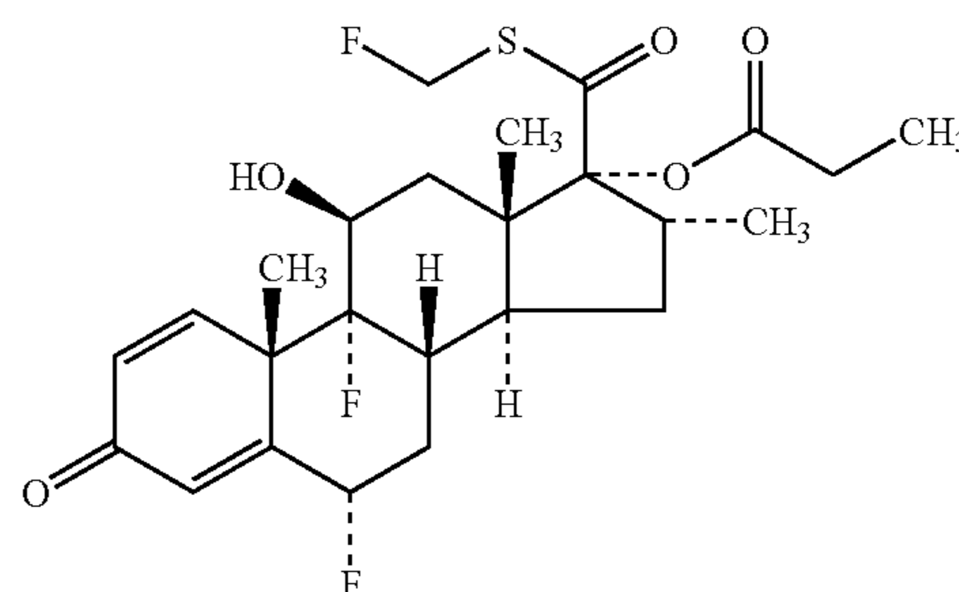
Fluticasone Propionate
