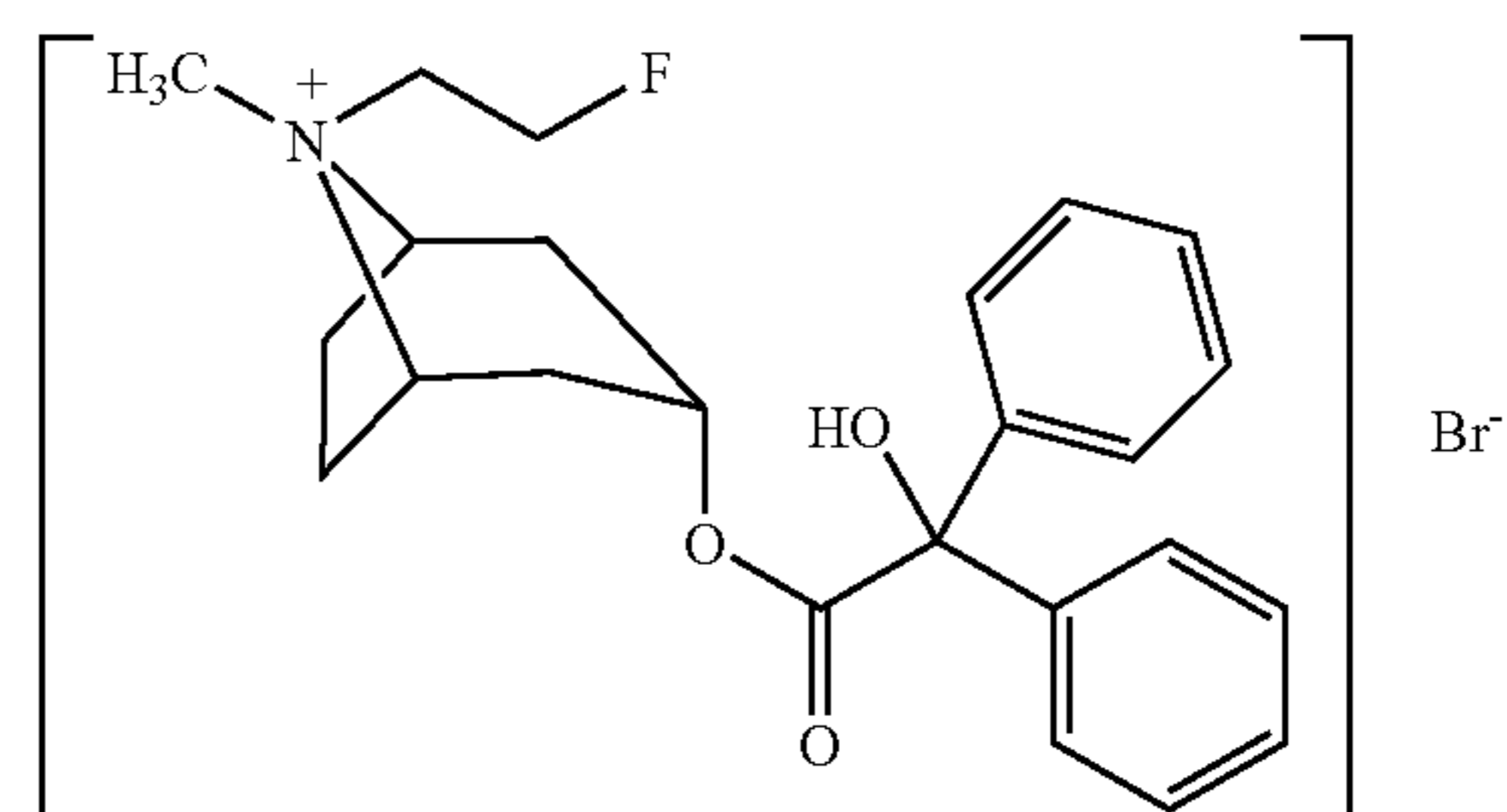
Flutropium Bromide
