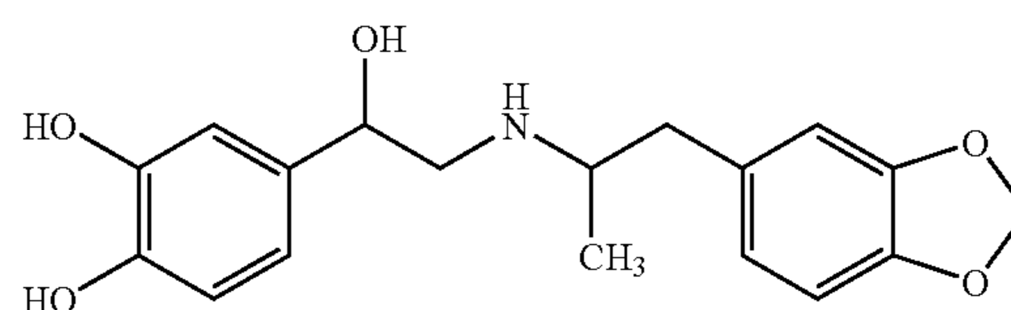
Protokylol
