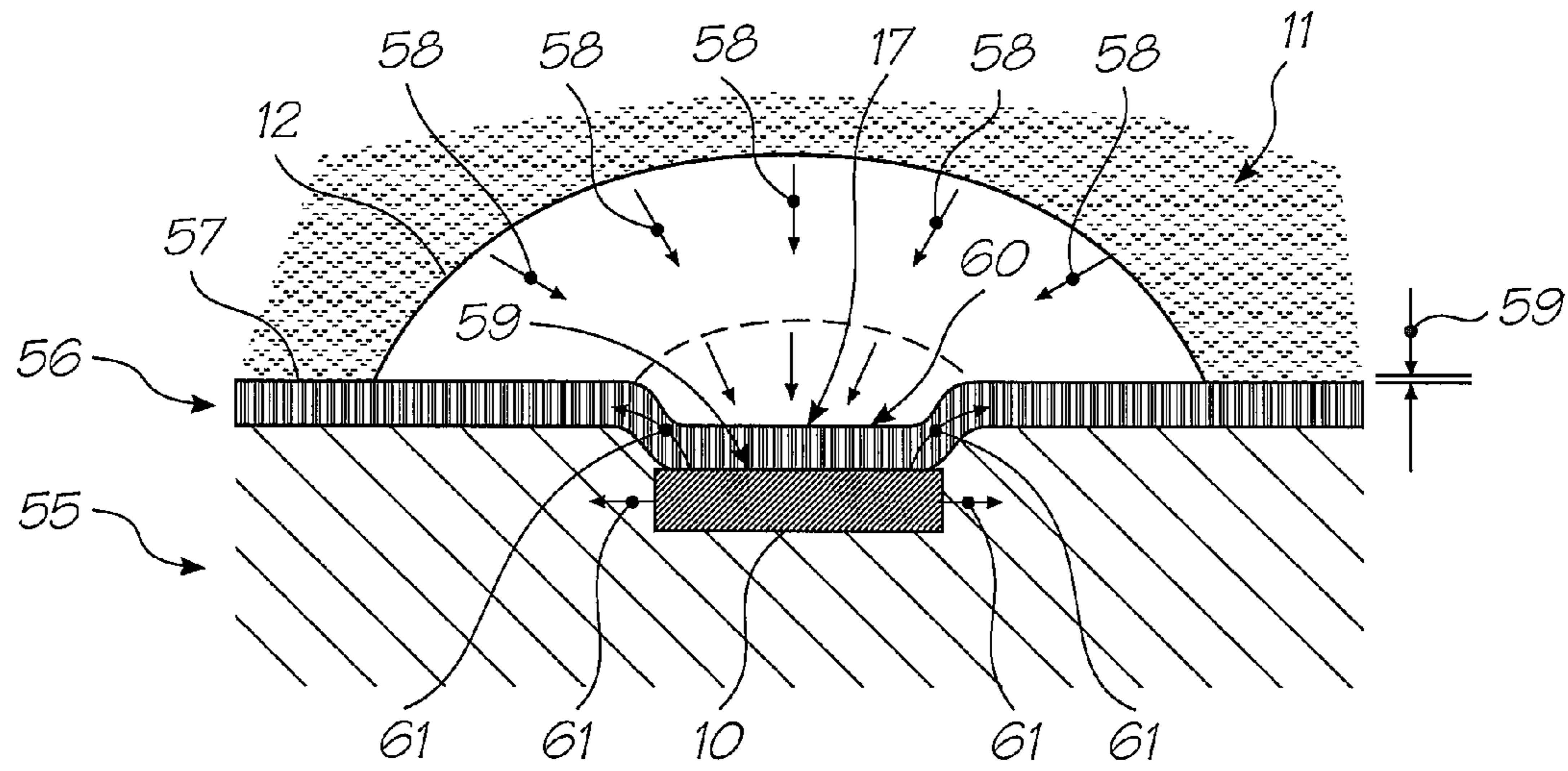
FIG. 47 (PRIOR ART)
