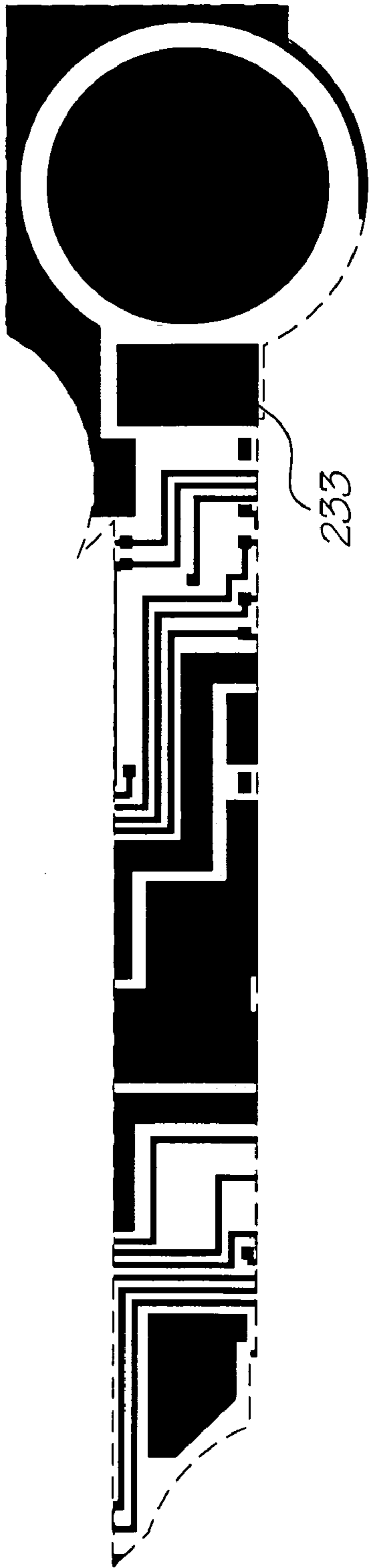
Metal 2 mask
