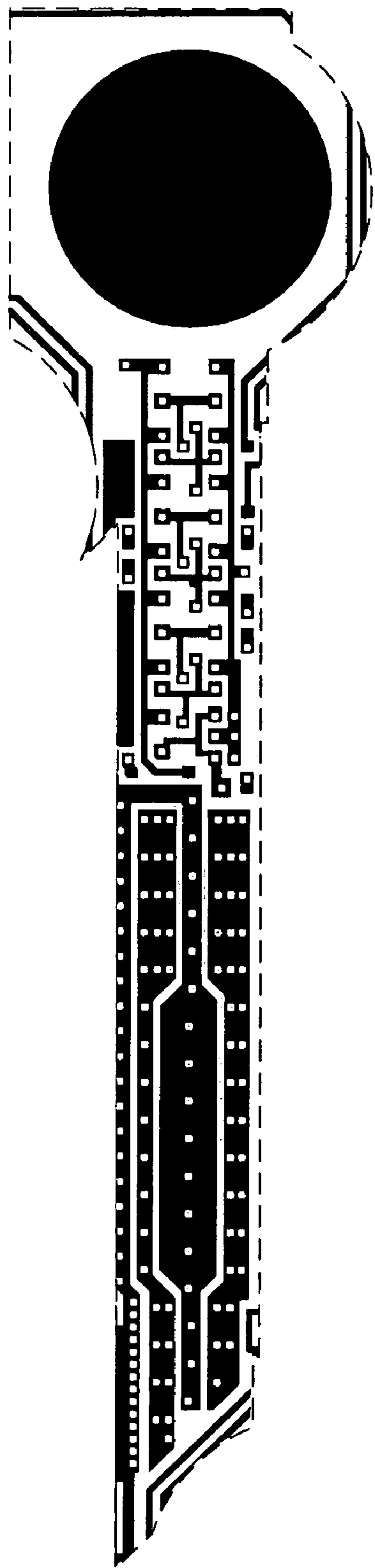
Metal 1 mask
