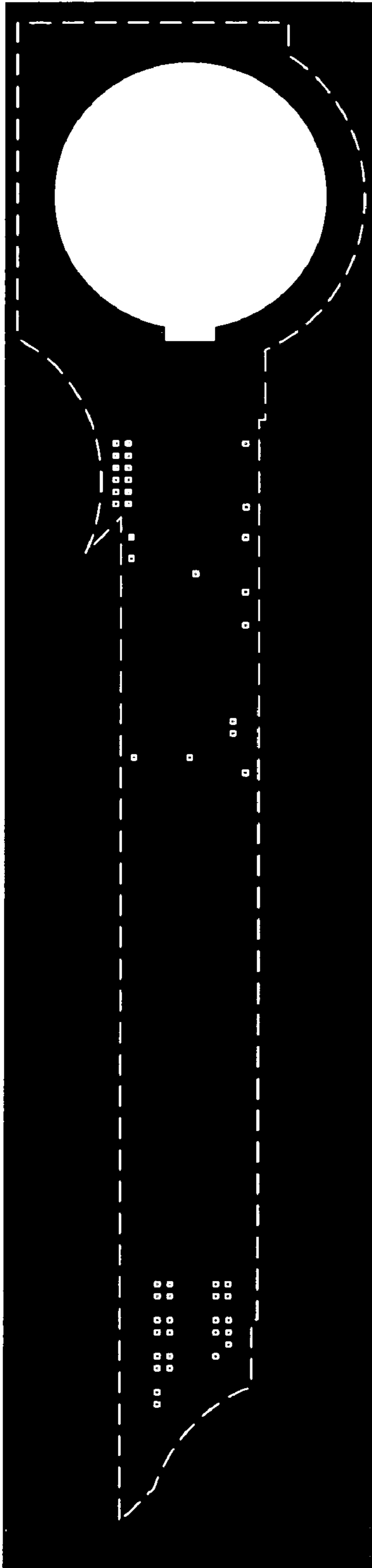
Via 1 mask
