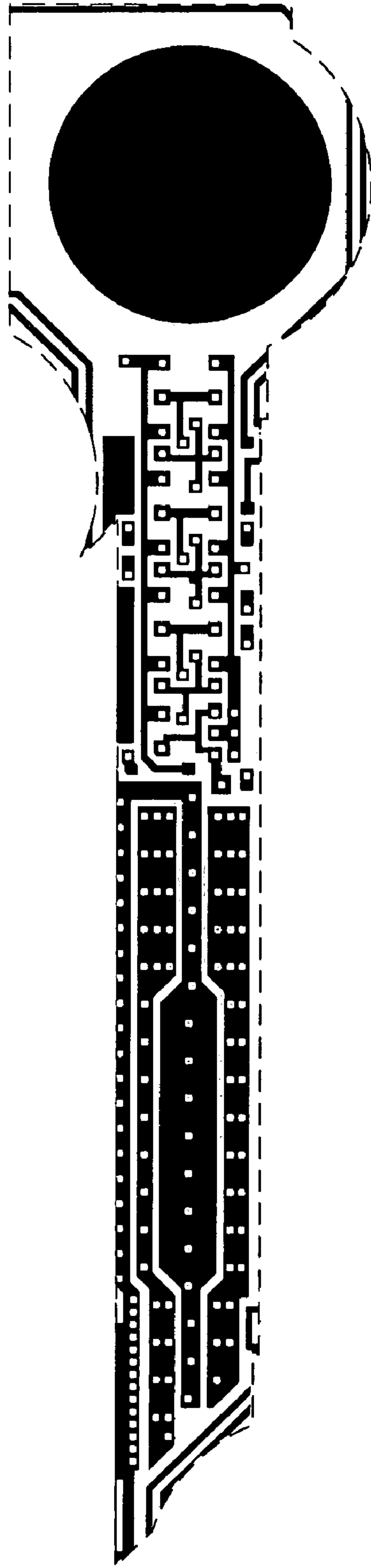
Metal 1 mask
