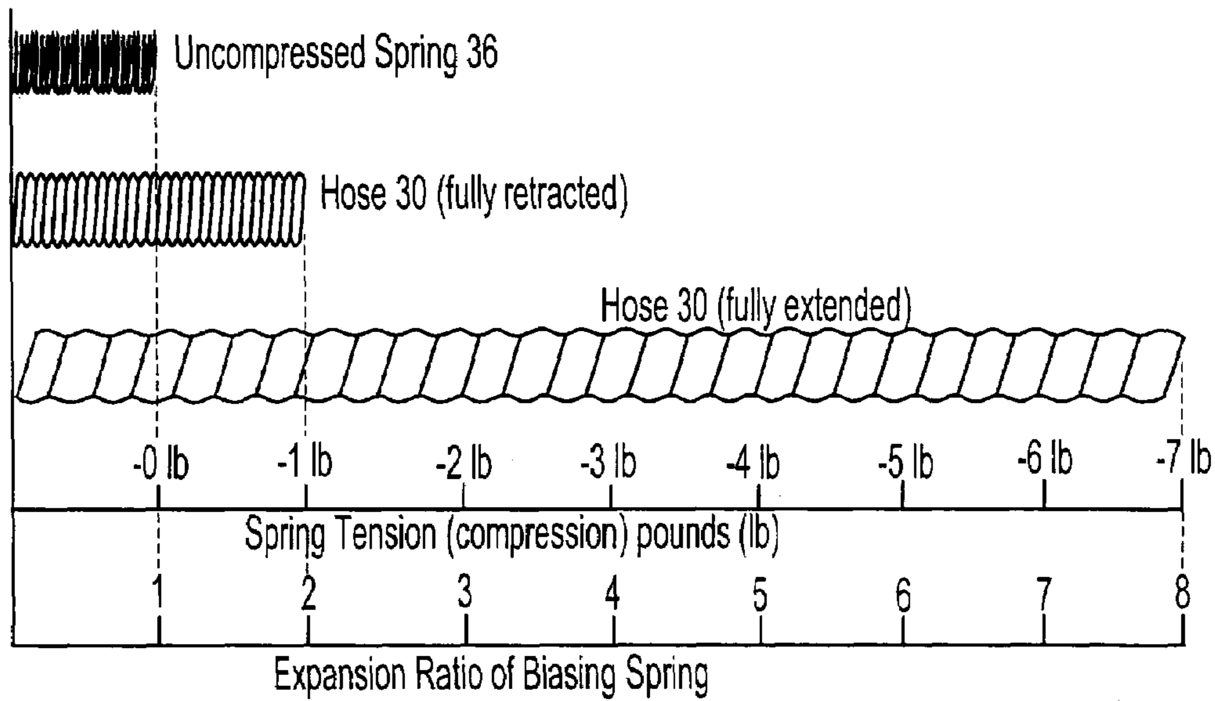
Fig. 5 - Spring-Bias Effects on Pressure Hose
