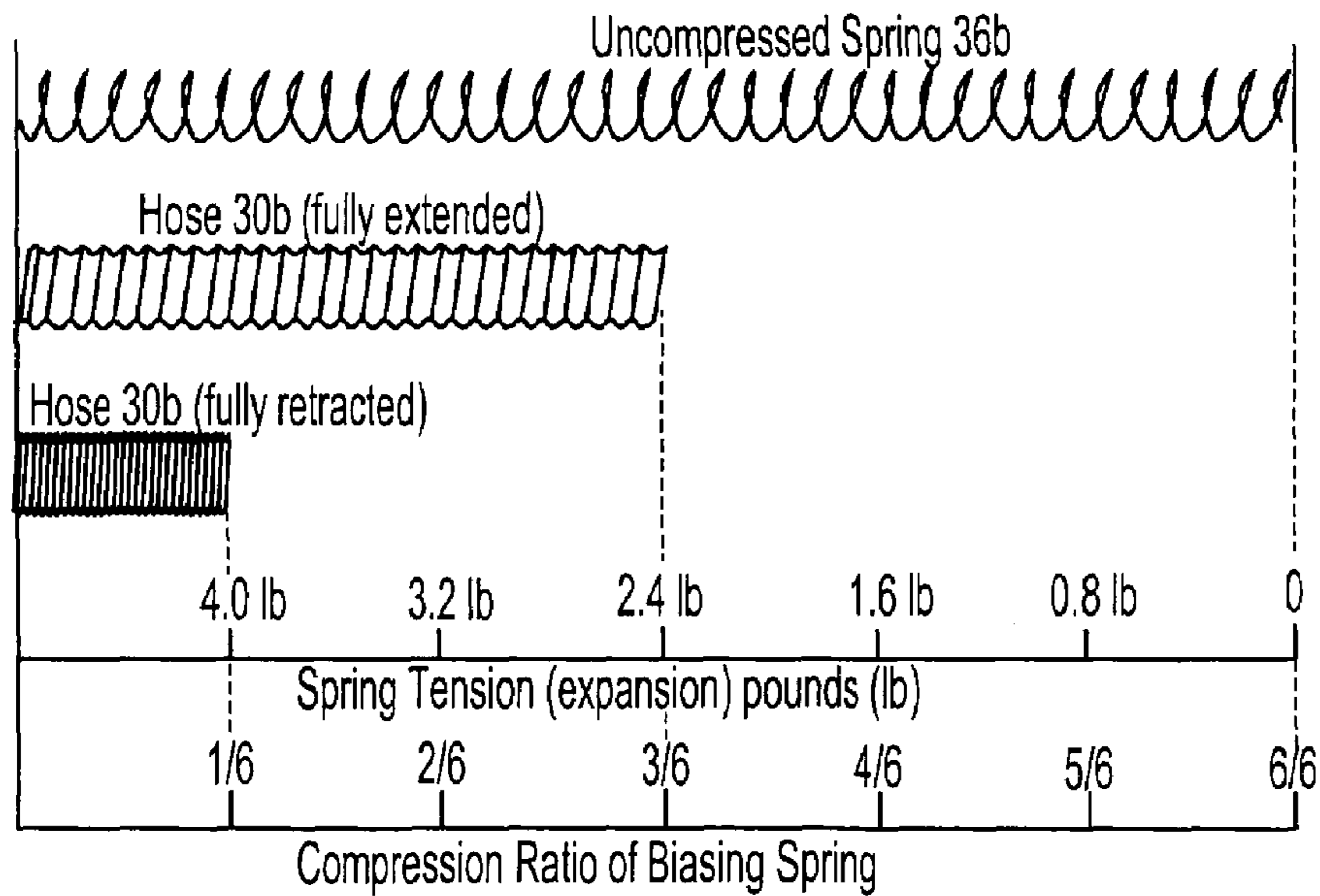
Fig. 6 - Spring Bias Effect on Vacuum Hose
