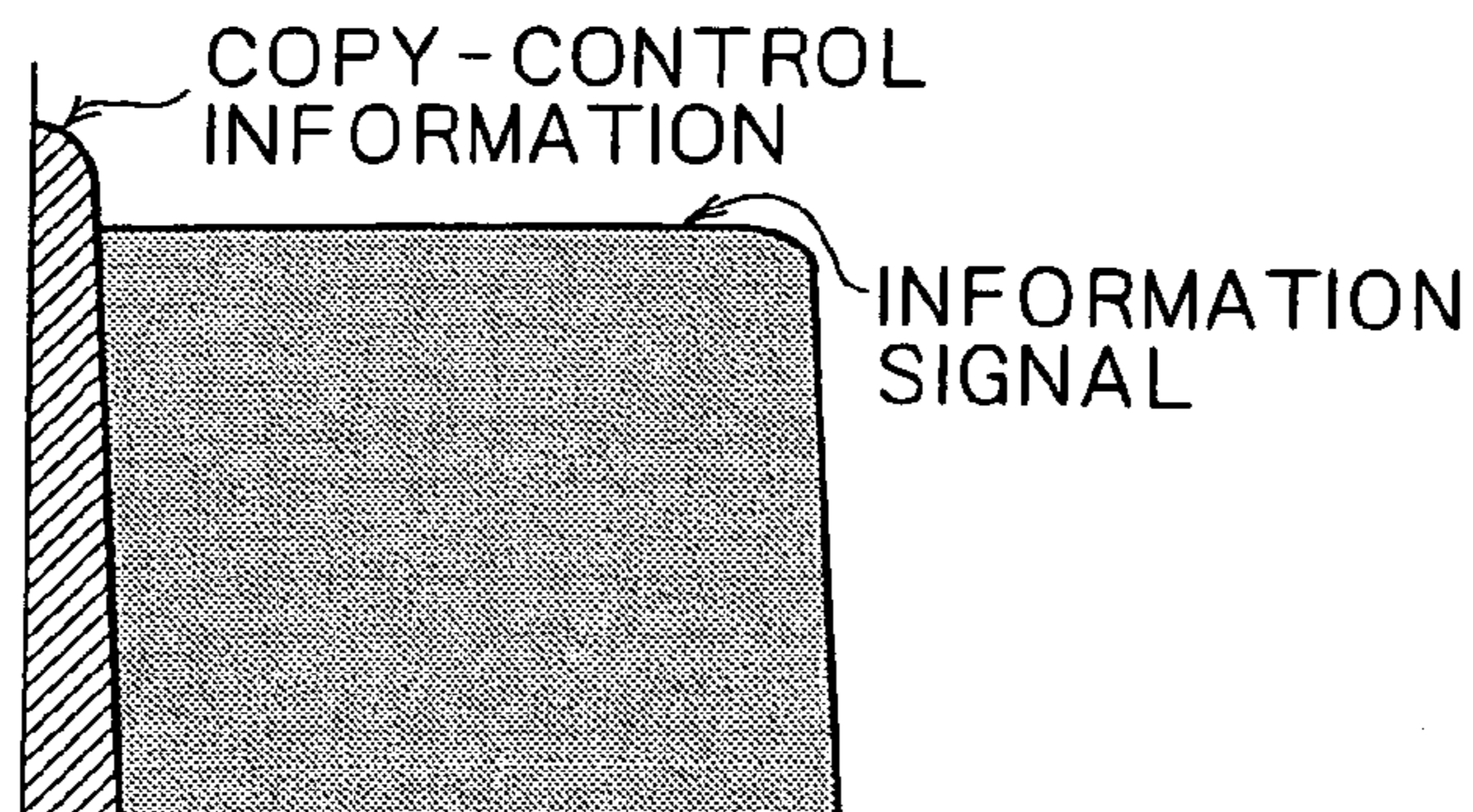
SIGNAL SPECTRUM AFTER SPECTRUM INVERSE SPREADING
