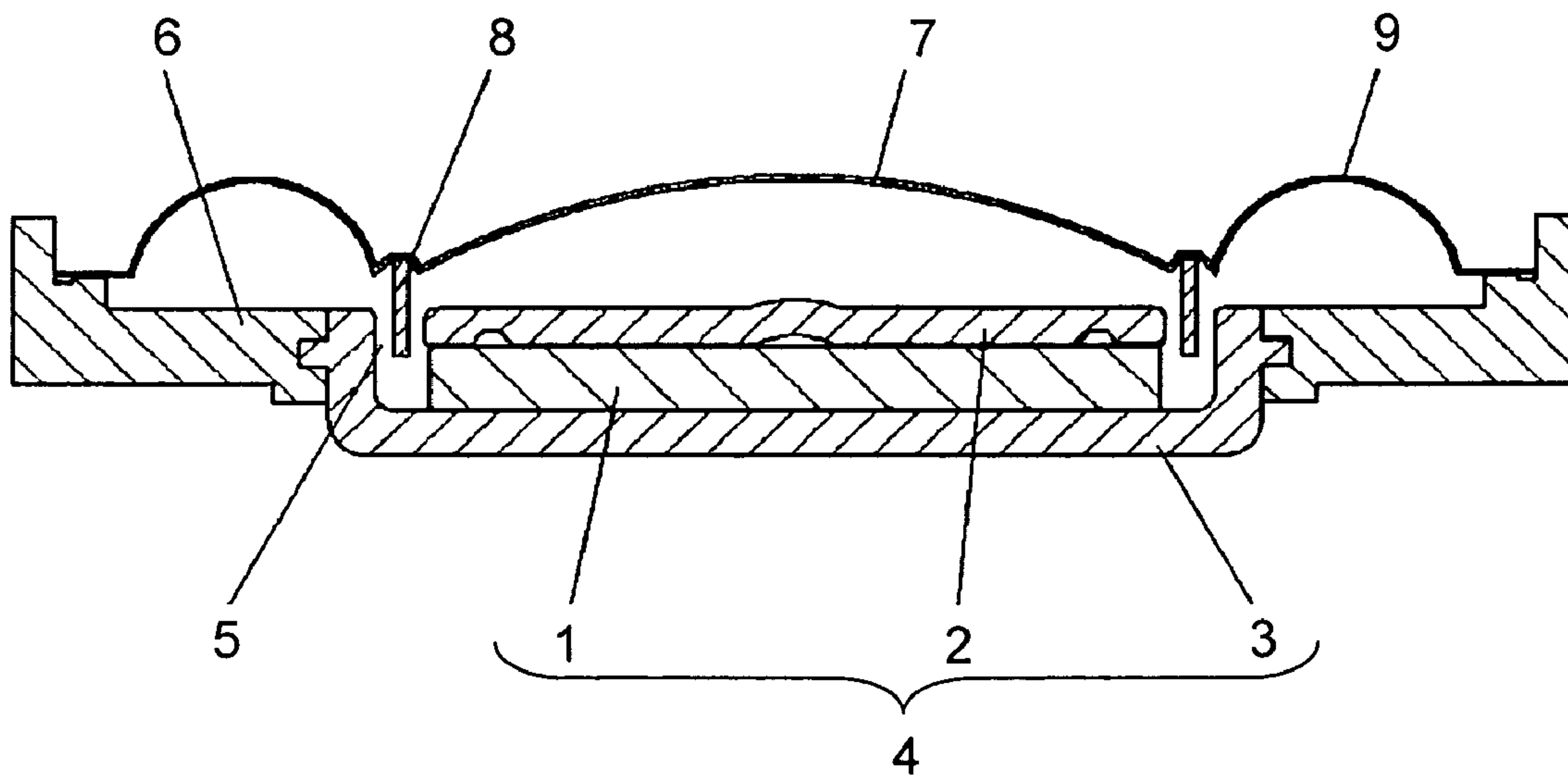
FIG. 16 - PRIOR ART
