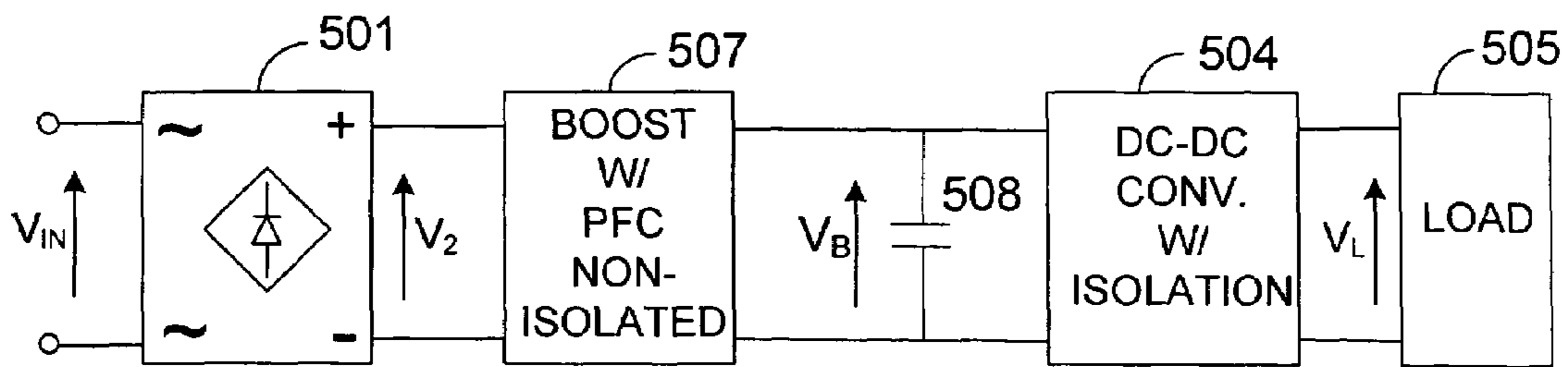
PRIOR ART FIG. 11
