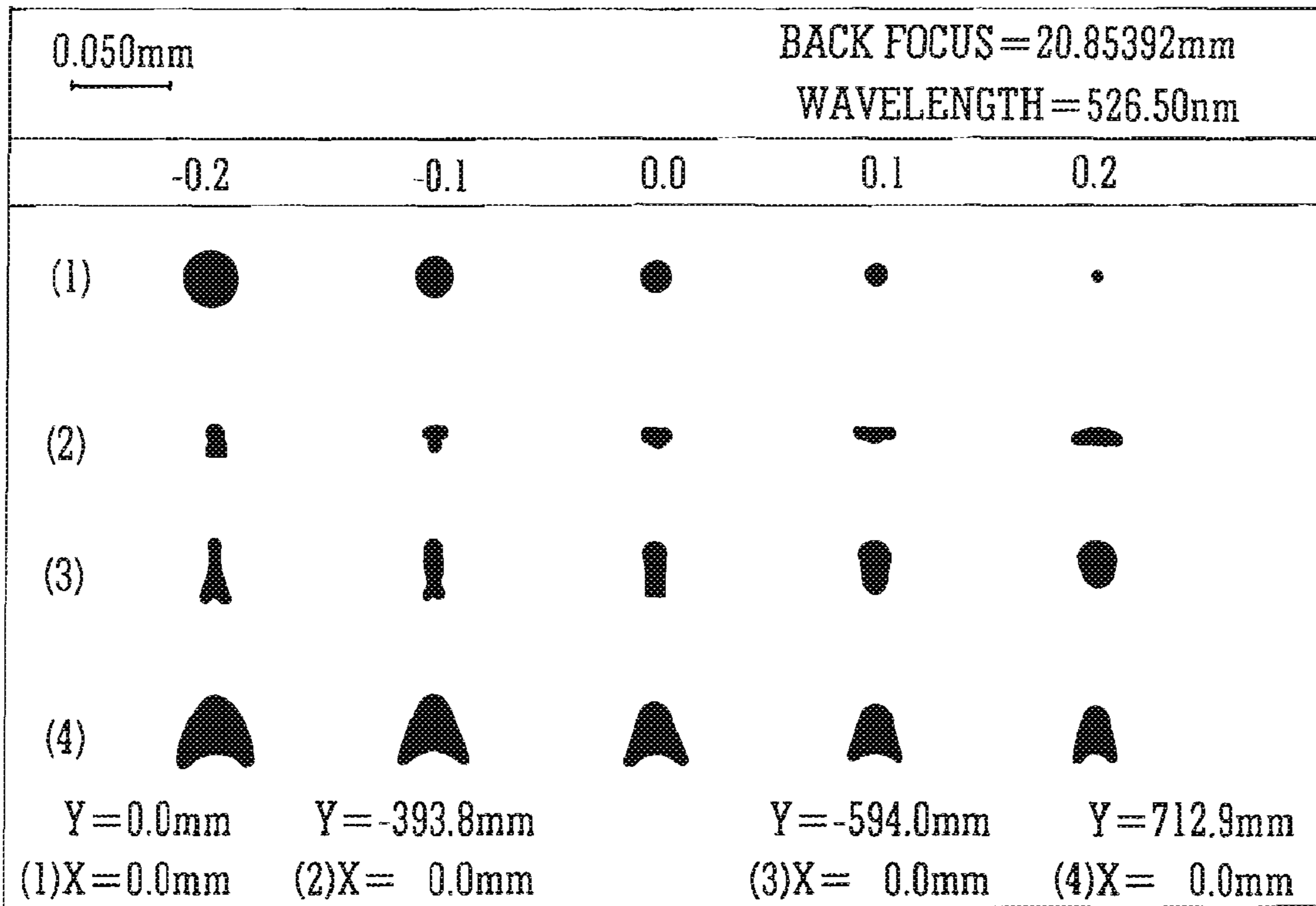
ZOOM CONFIGURATION 3
