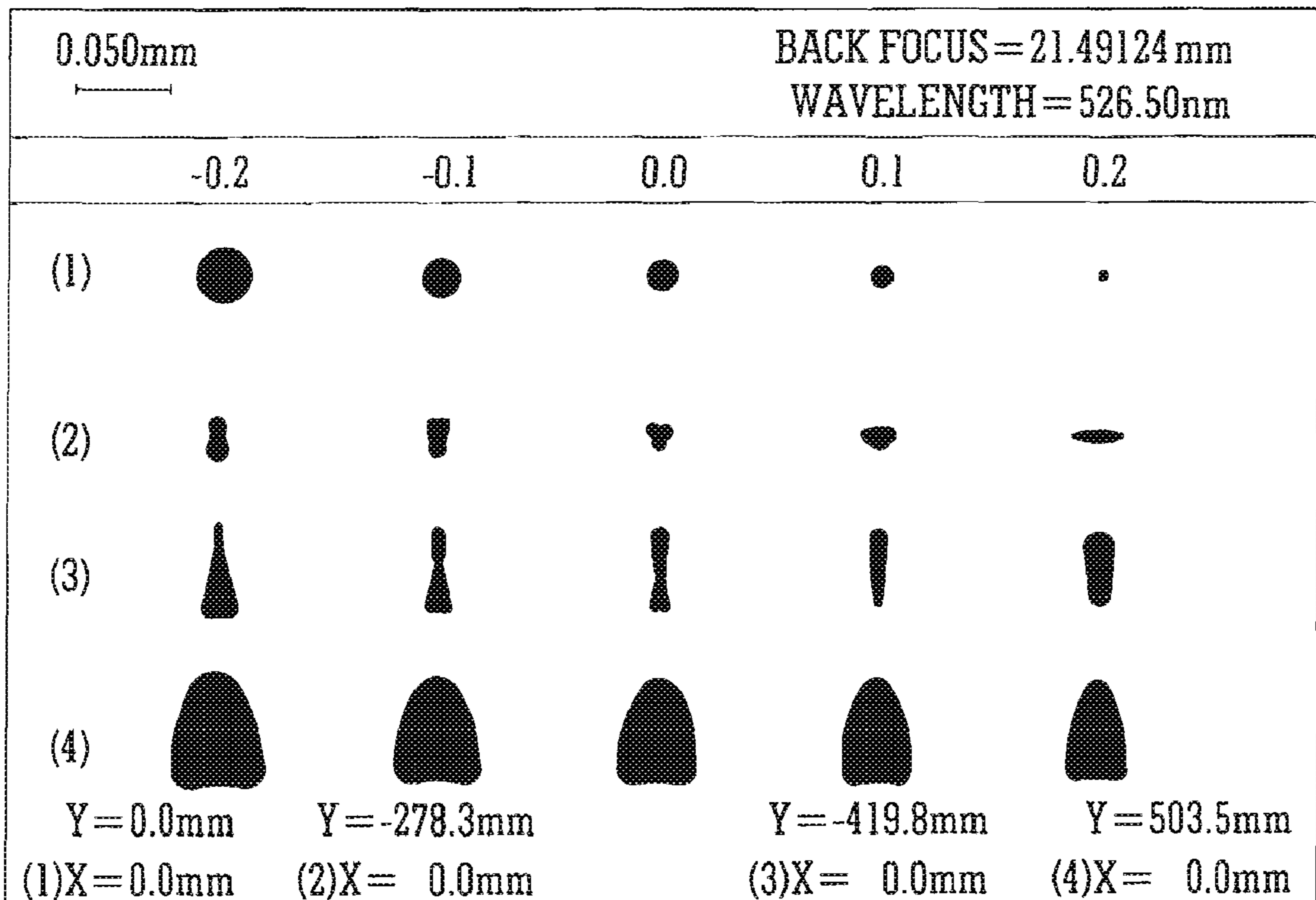
ZOOM CONFIGURATION 4
