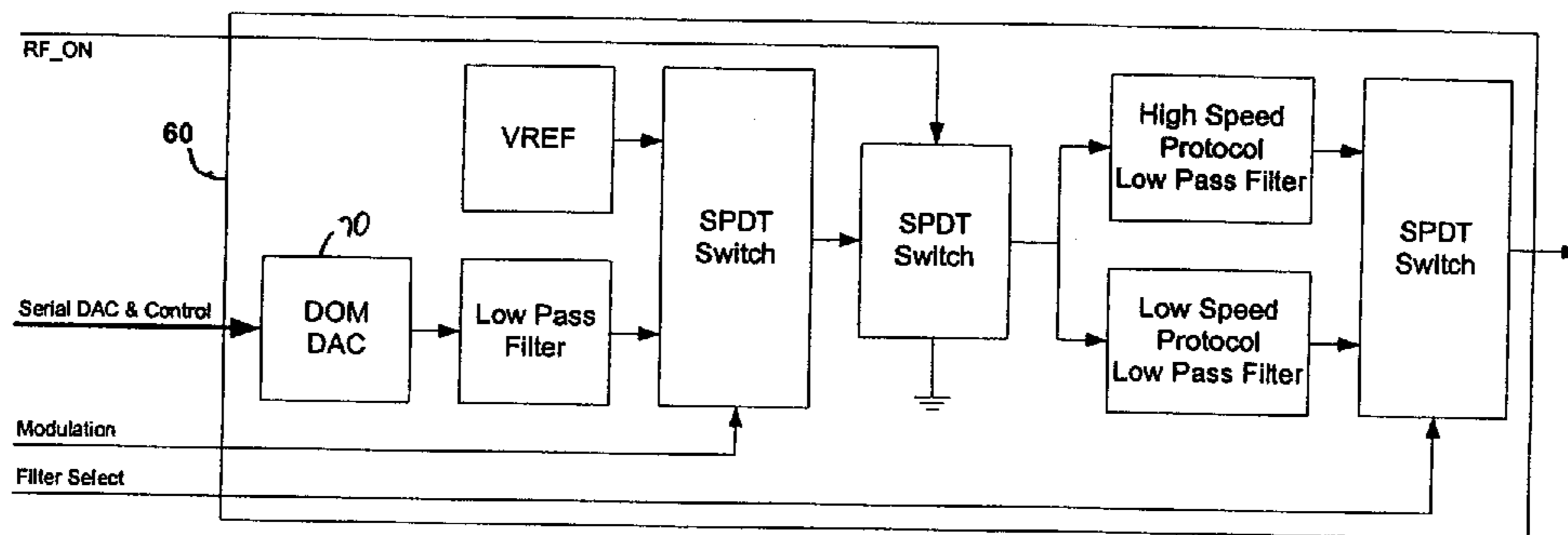
Figure 7 DOM DAC and Modulation Control Block Diagram
