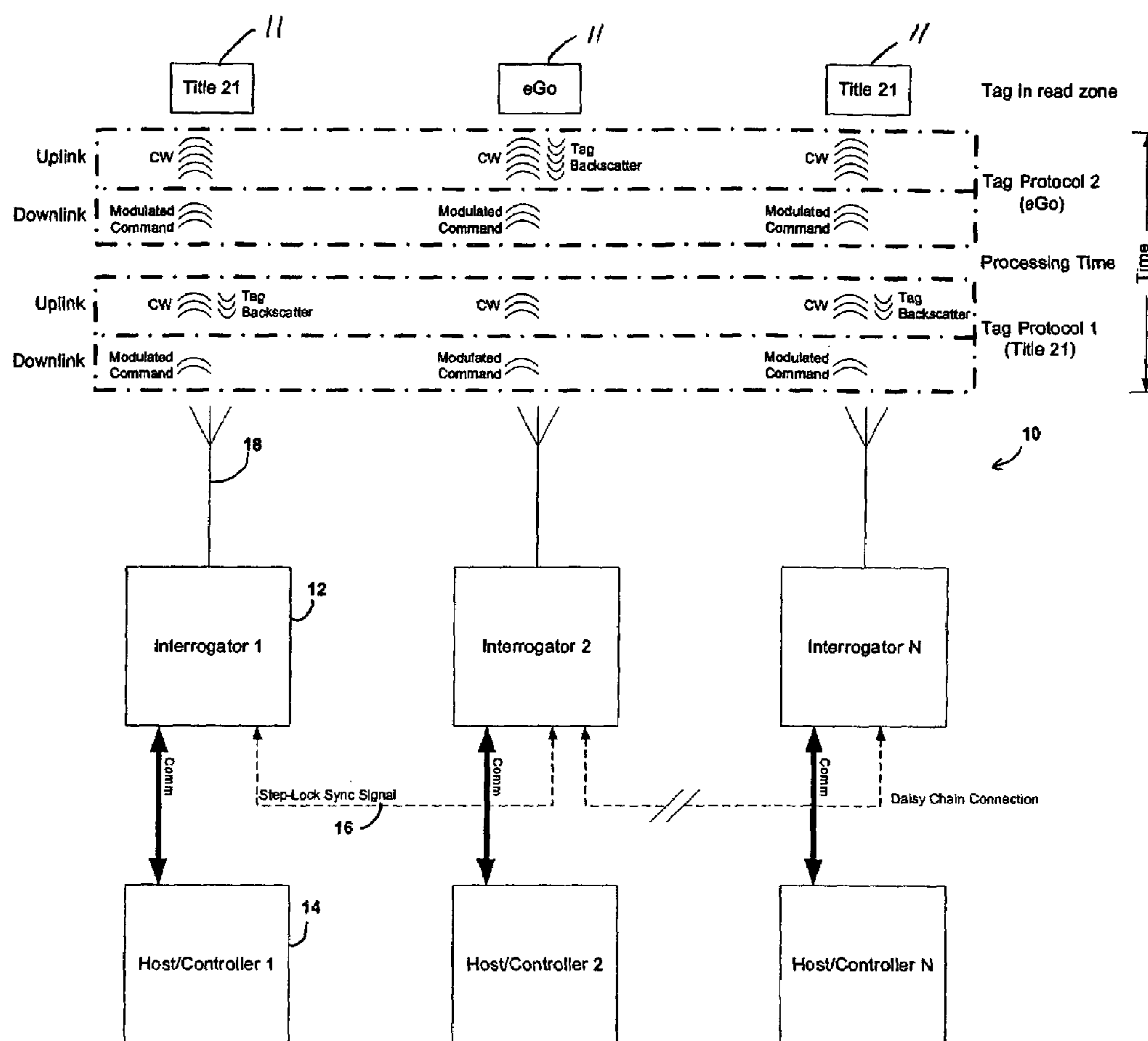
Figure 1 Step-Locked Interrogator Cluster (Internal Sync Signal)
