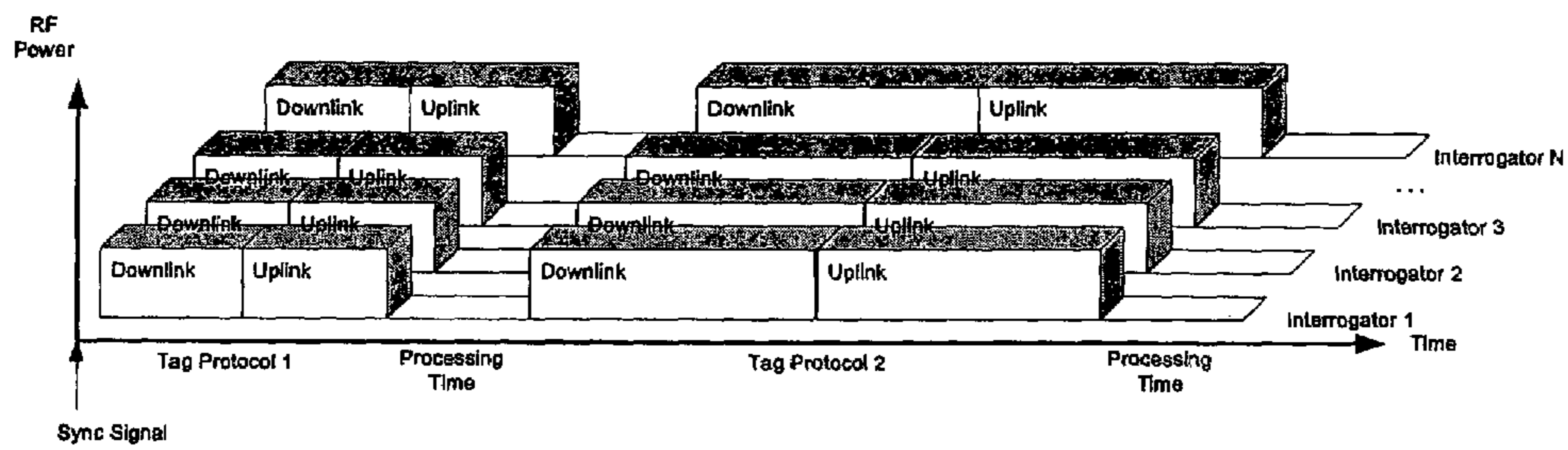
Figure 3(a) - Step Lock Timing Diagram
