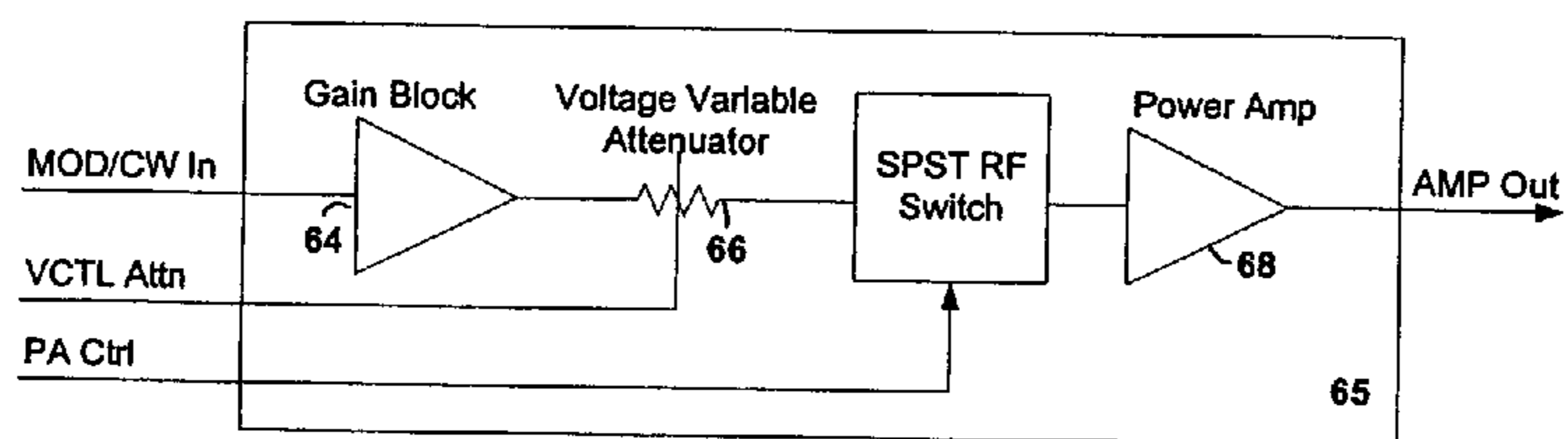
Figure 8 Power Amplifier Block Diagram
