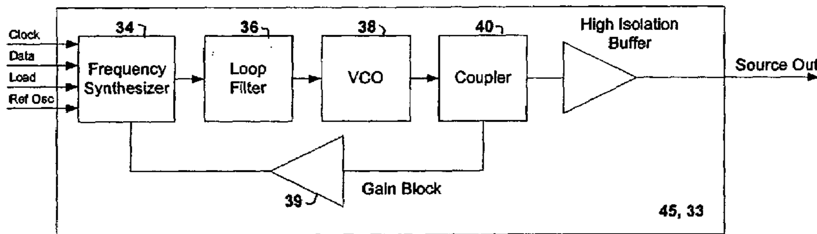
Figure 5 Synthesized Source Block Diagram
