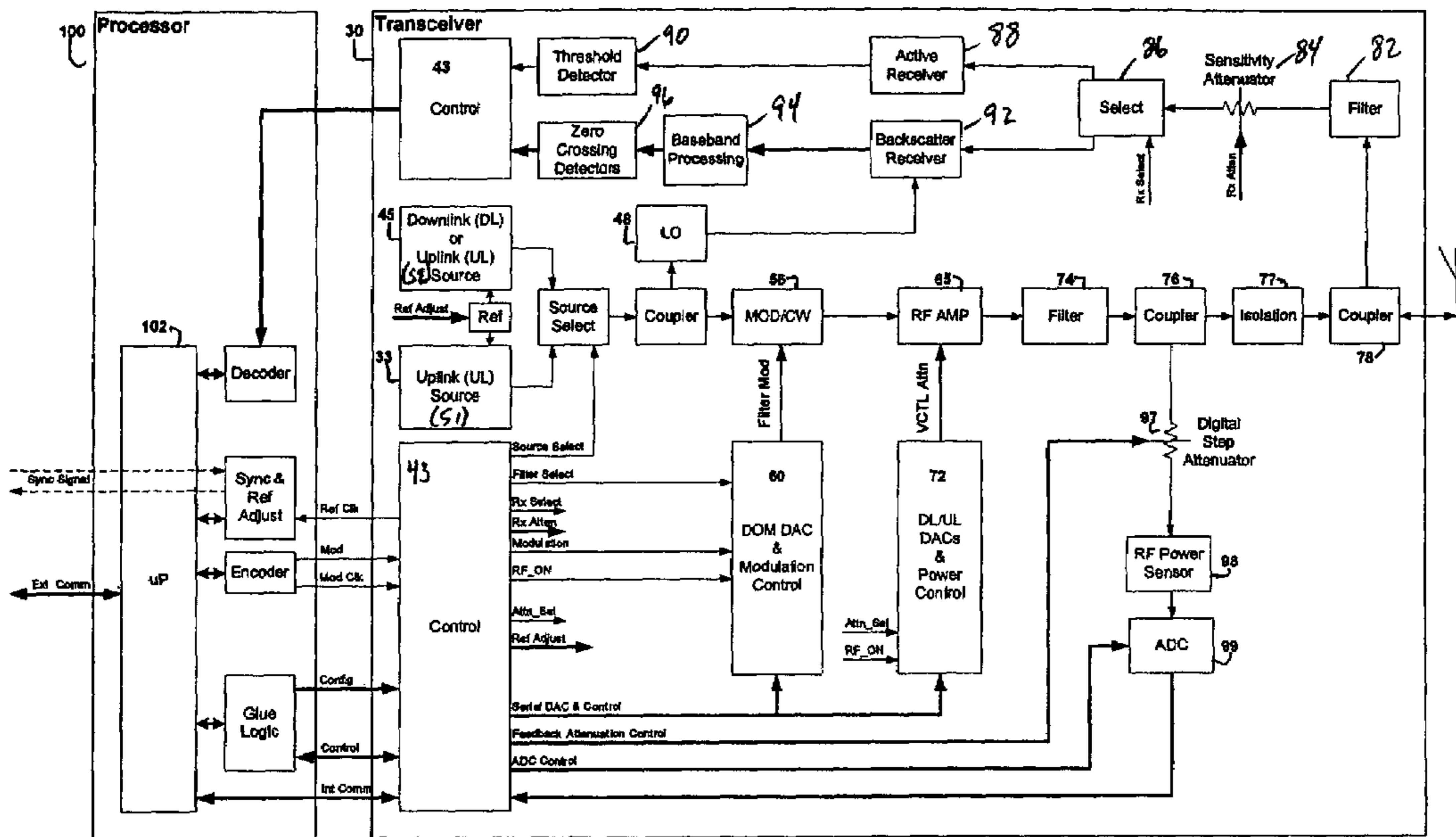
Figure 4 Interrogator Block Diagram
