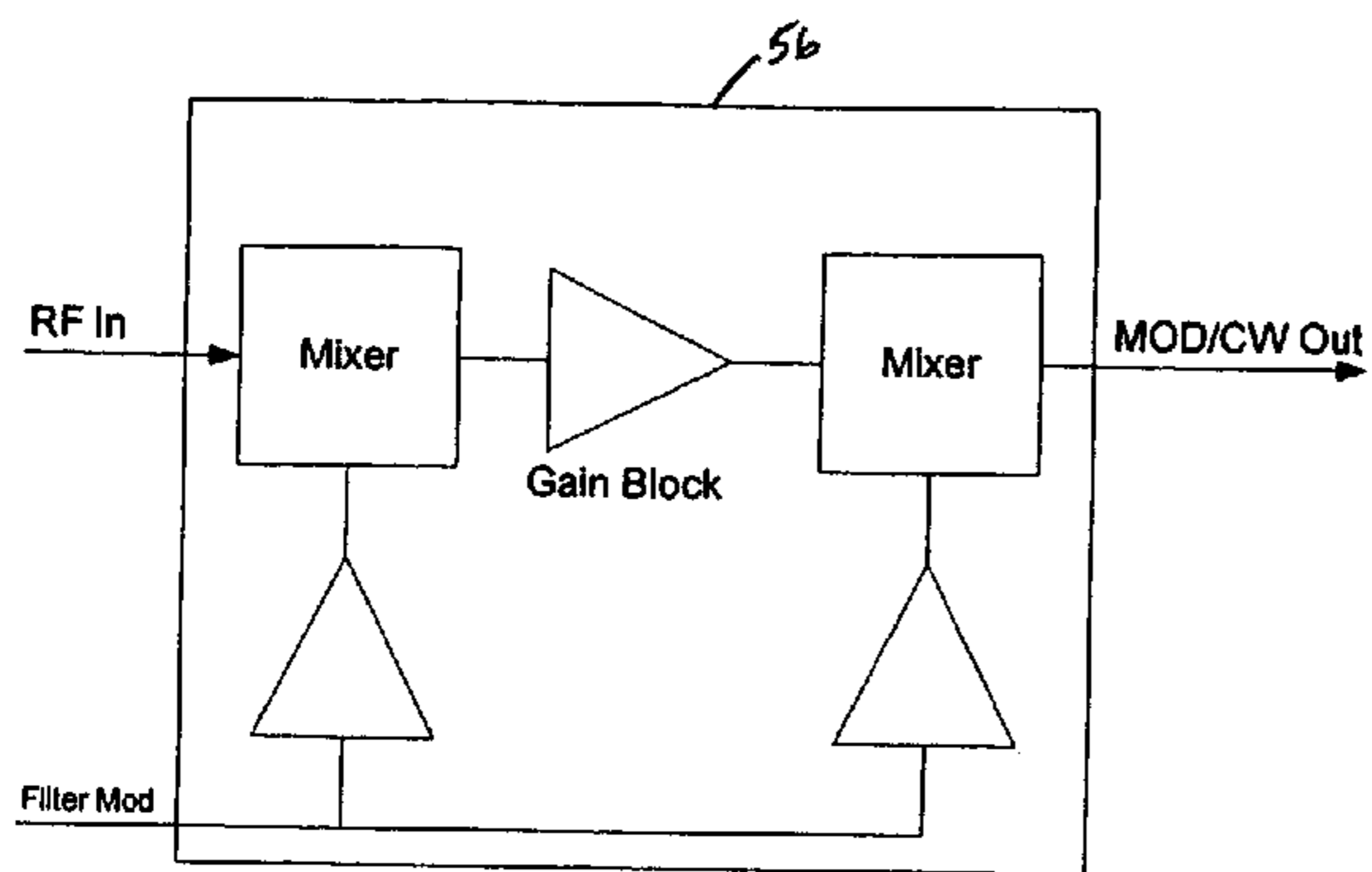
Figure 6 Dual Mixer Block Diagram
