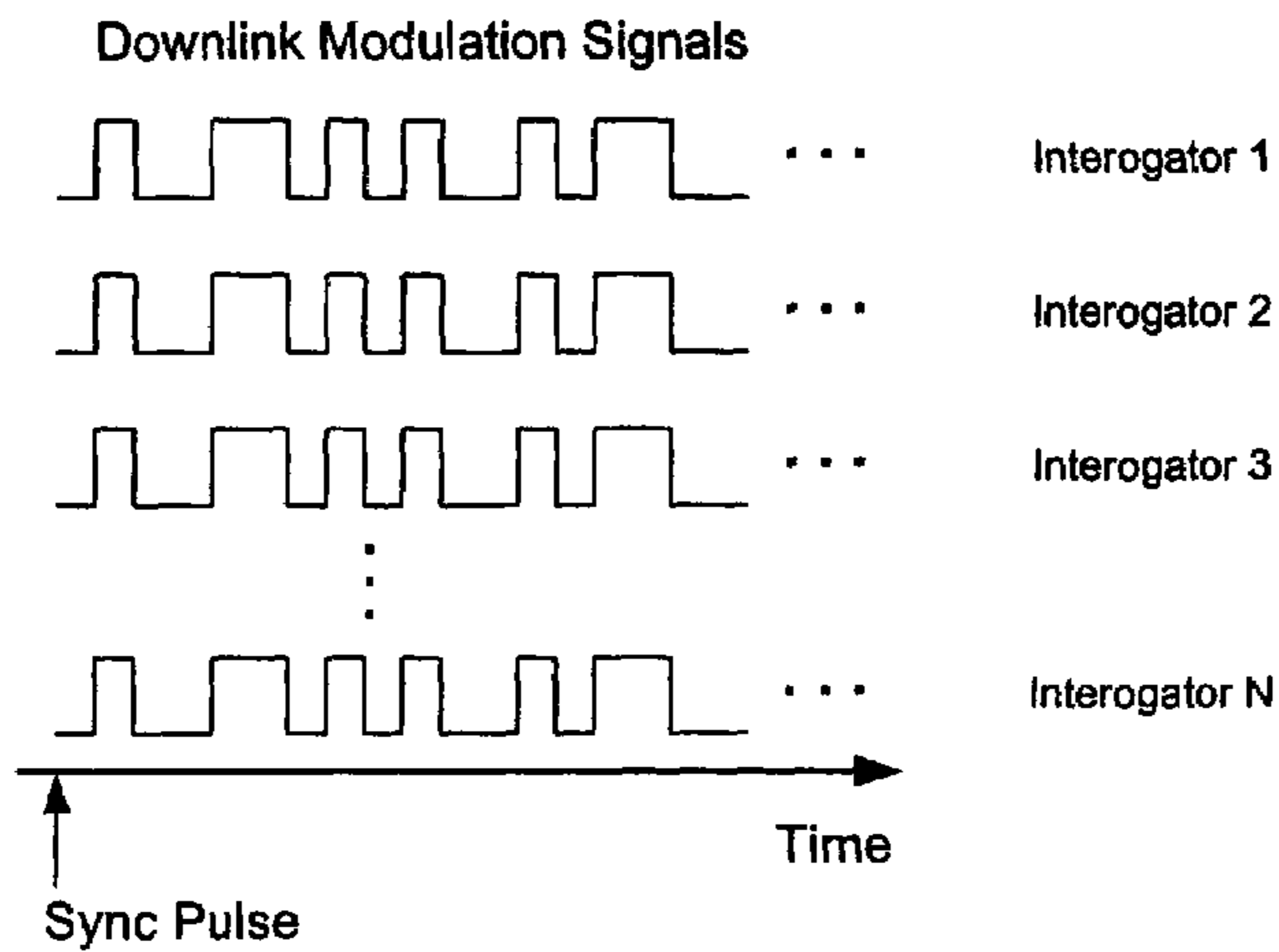
Figure 3(b) - Step Lock with Bit Synchronization
