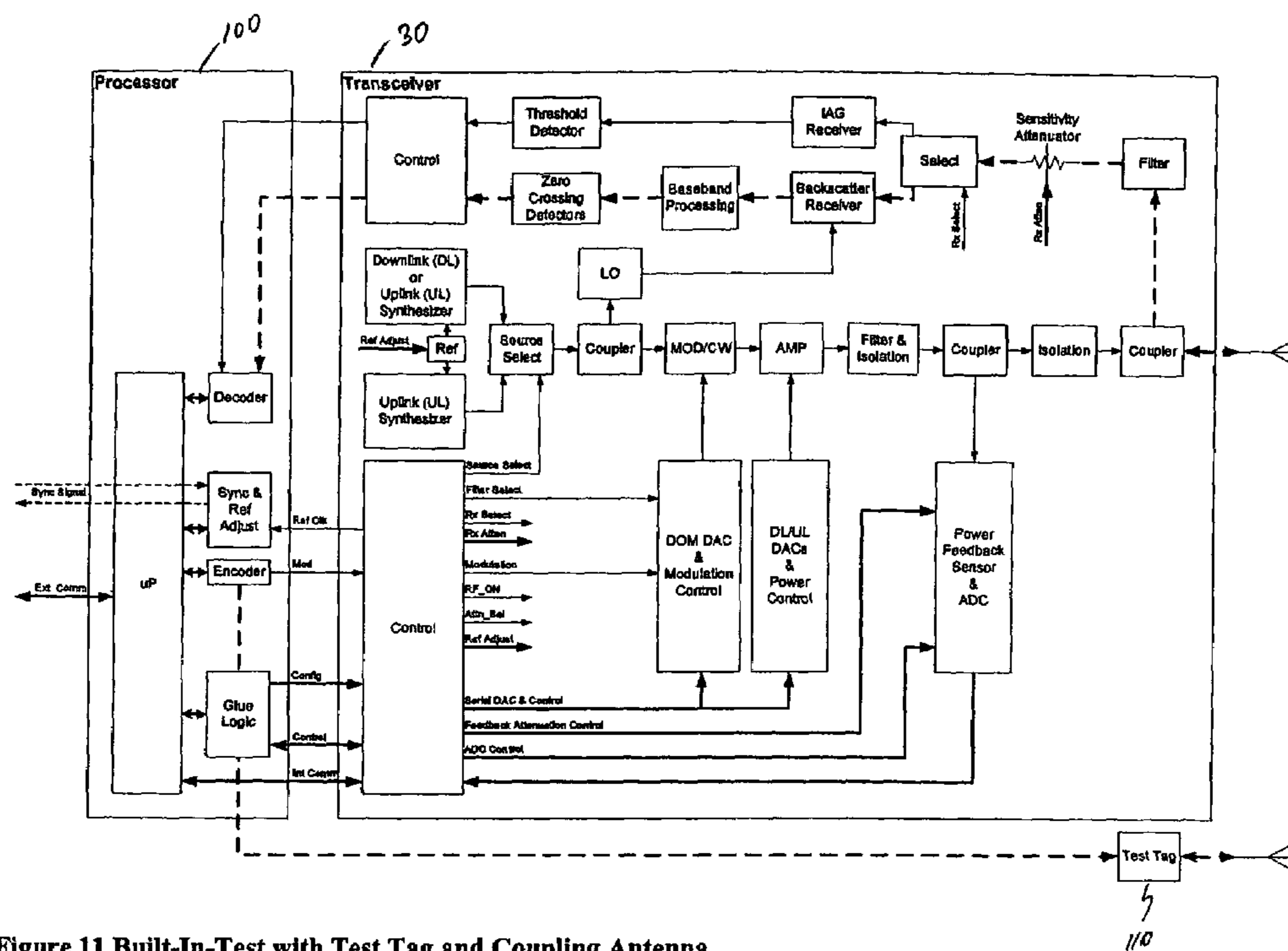
Figure 11 Built-In-Test with Test Tag and Coupling Antenna
