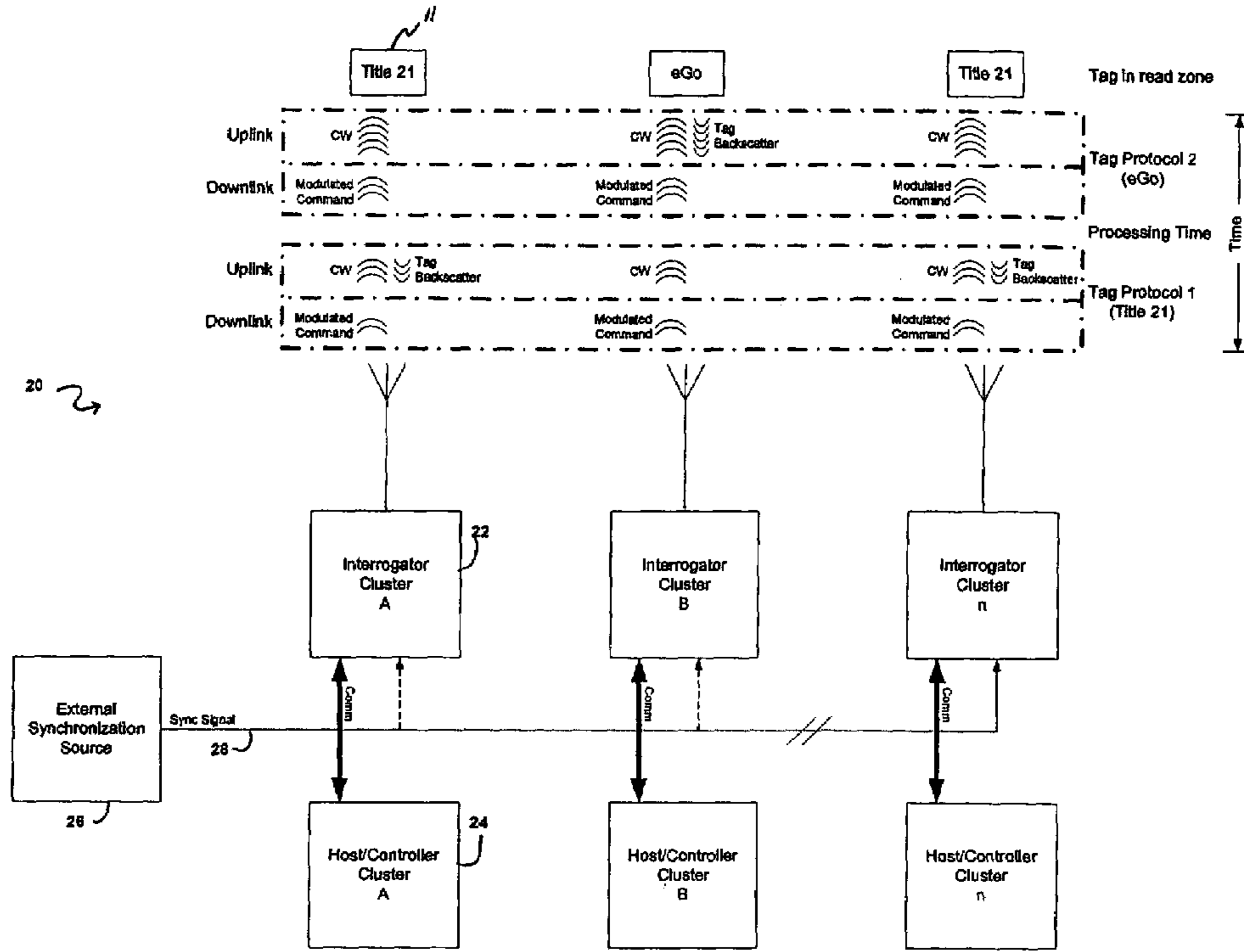
Figure 2 Step-Locked Interrogator Clusters (External Sync Signal)
