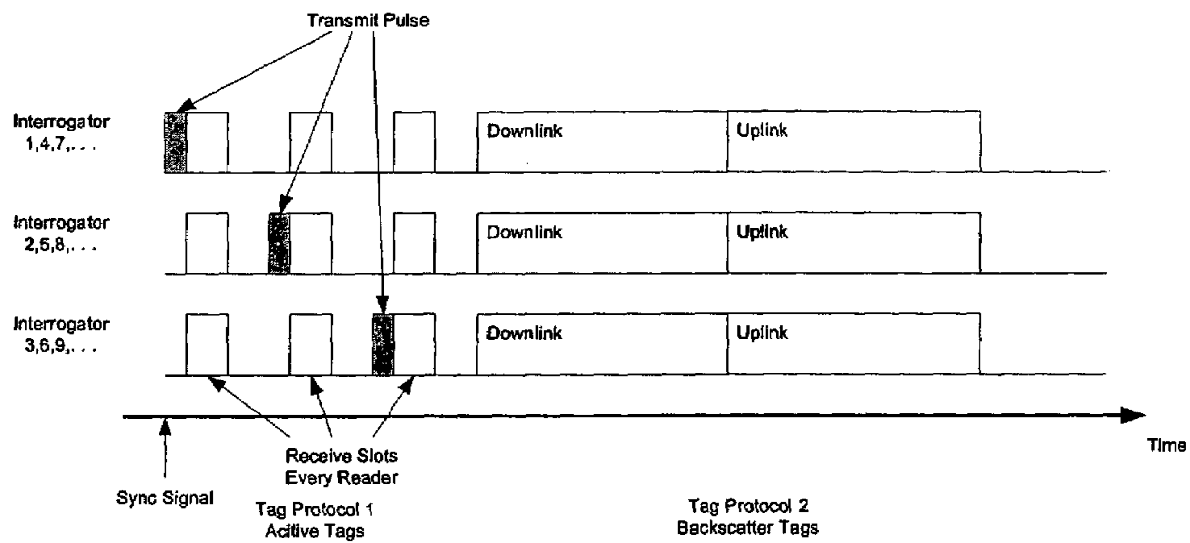
Figure 3(c) - Time Division Multiplexing and Step Lock Combination for Active and Backscatter
