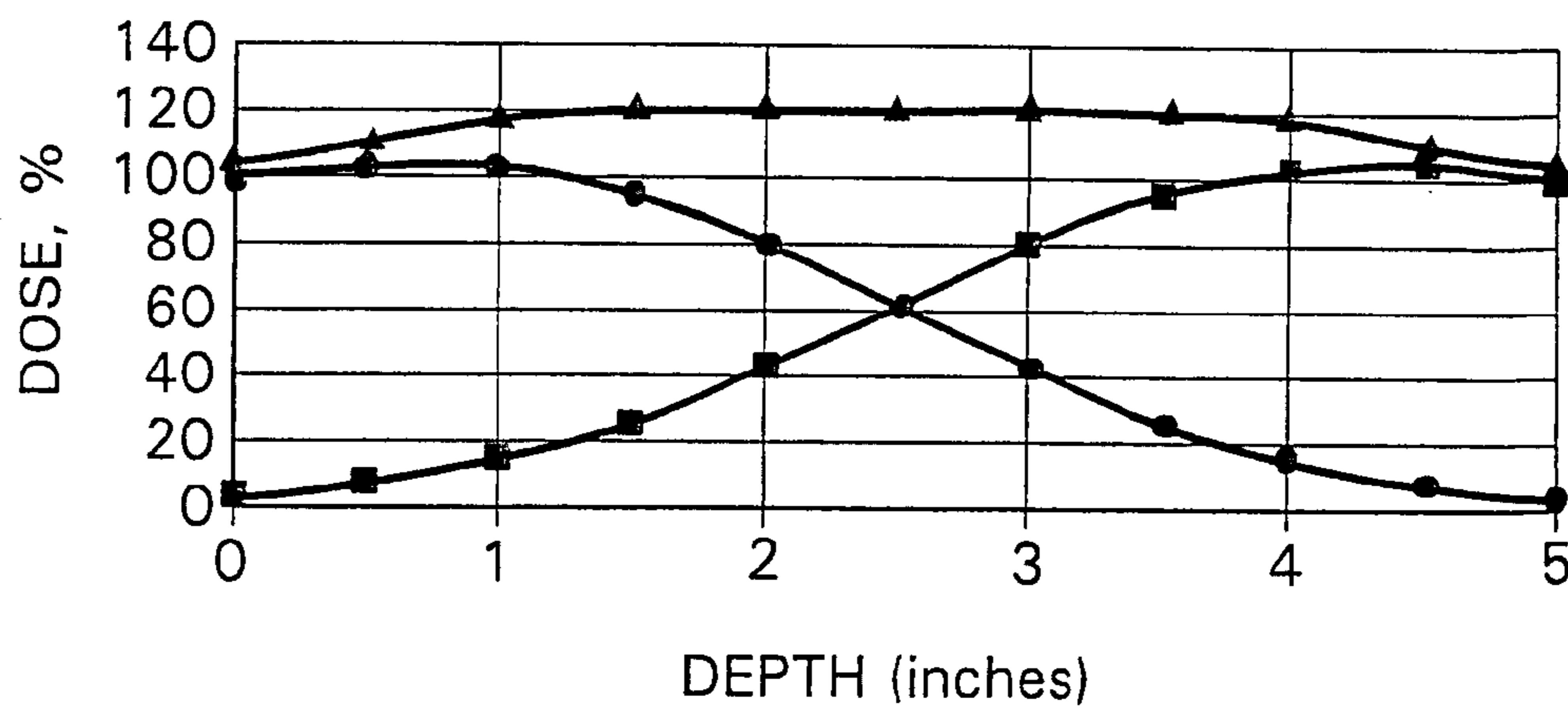
TYPICAL ENERGY DISTRIBUTION Two Opposing Emitters Shooting into Duct
