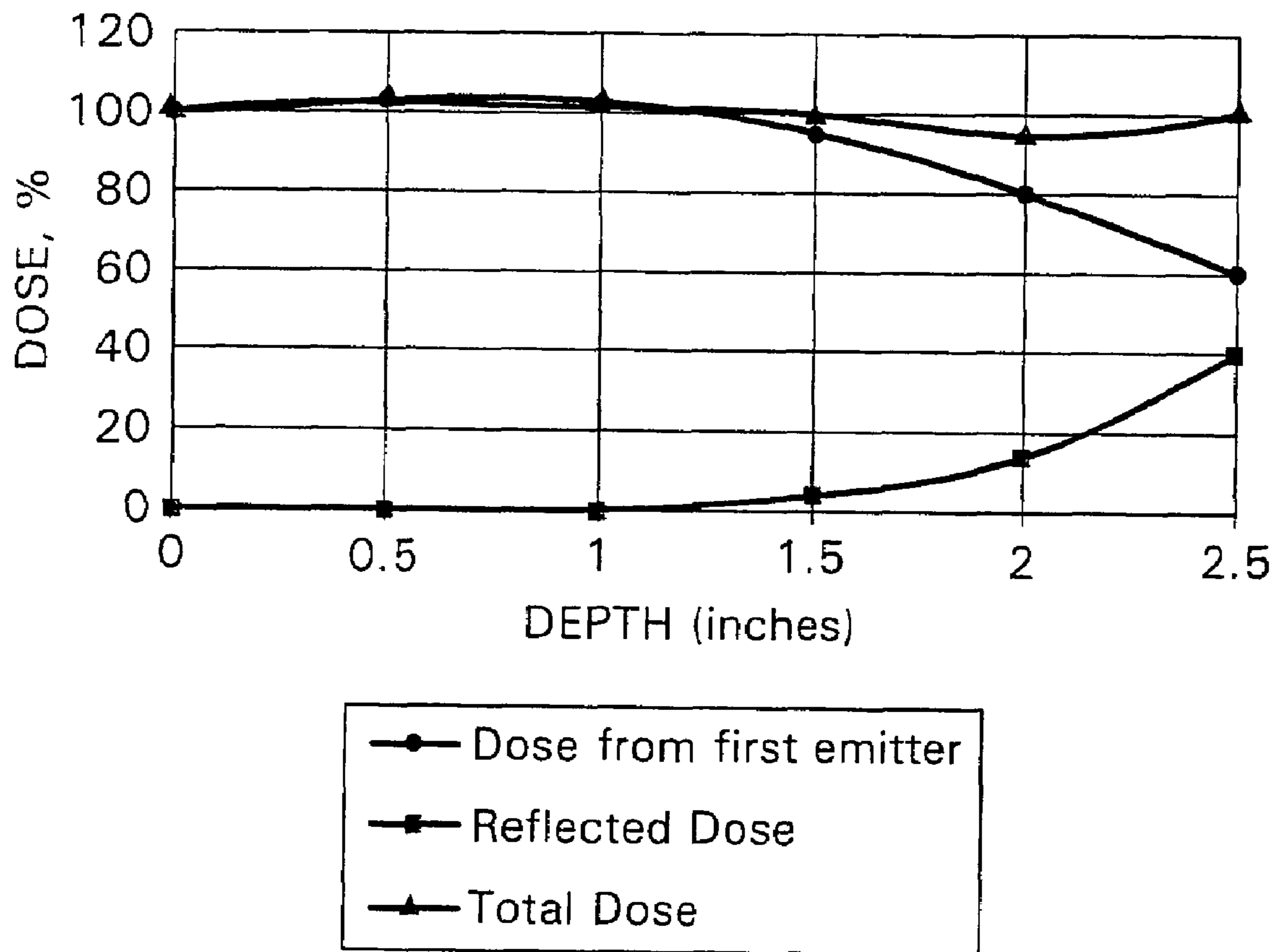
TYPICAL ENERGY DISTRIBUTION One Emitter Shooting from Left to Right
