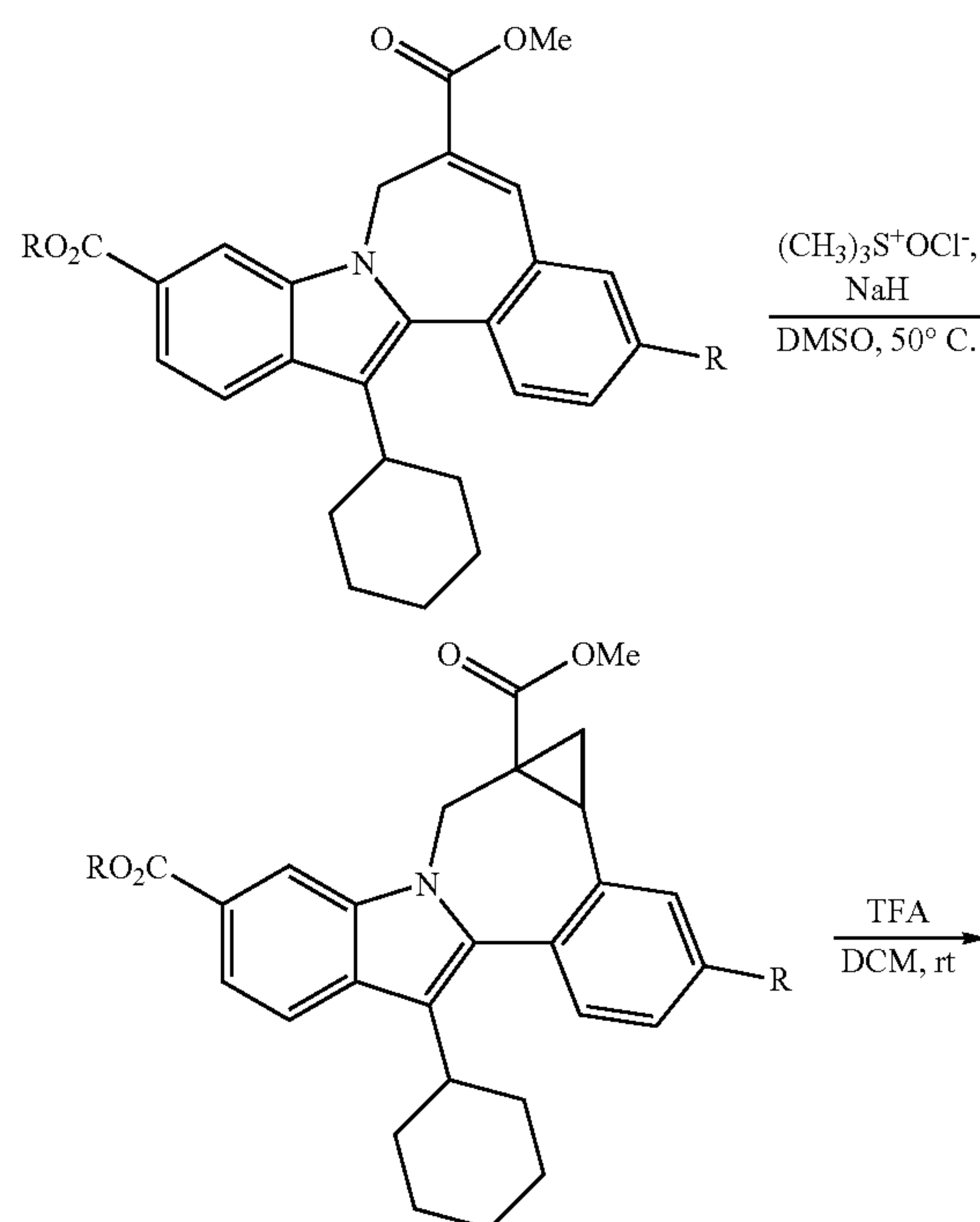
Scheme 4.
