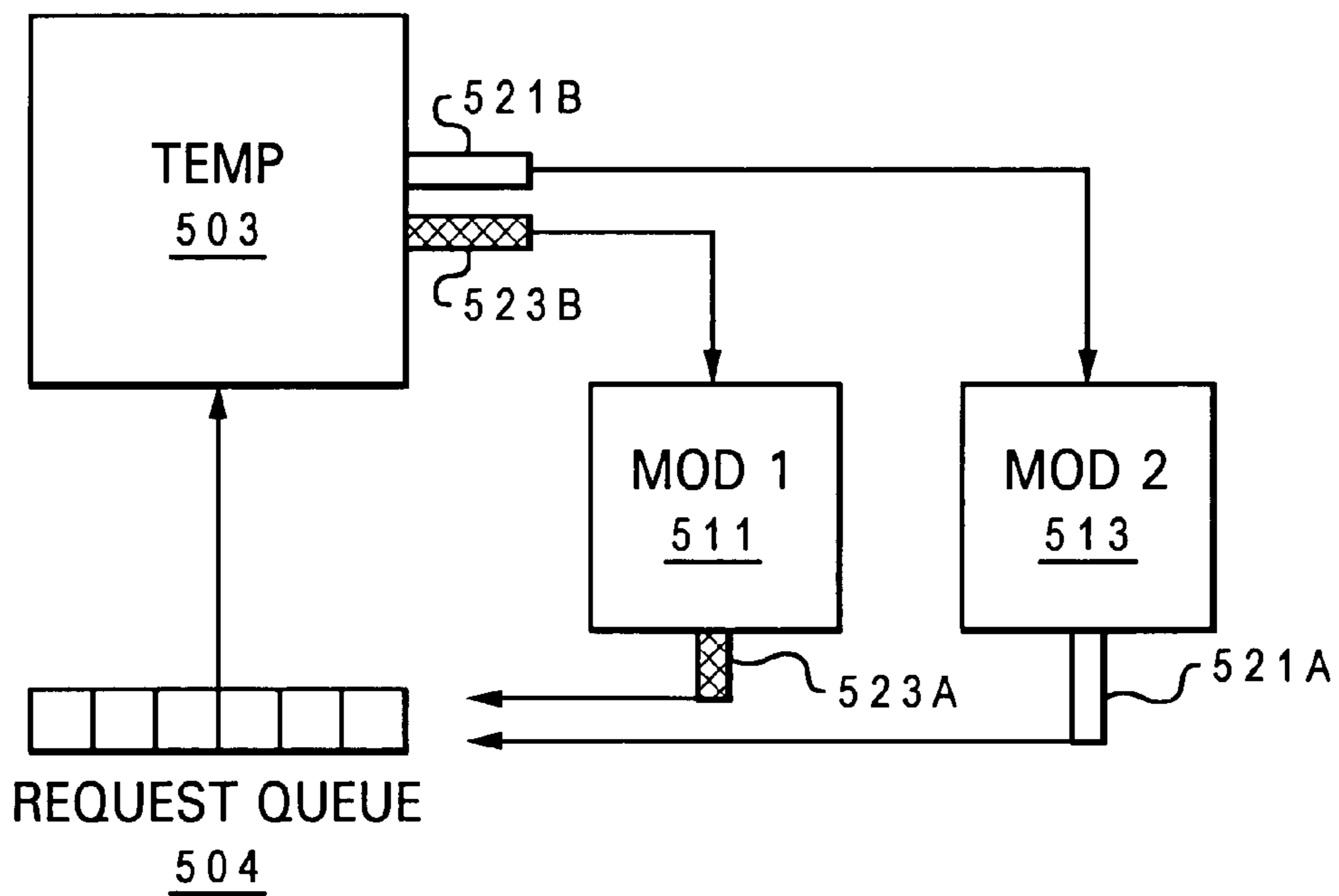
Fig. 5c Prior Art
