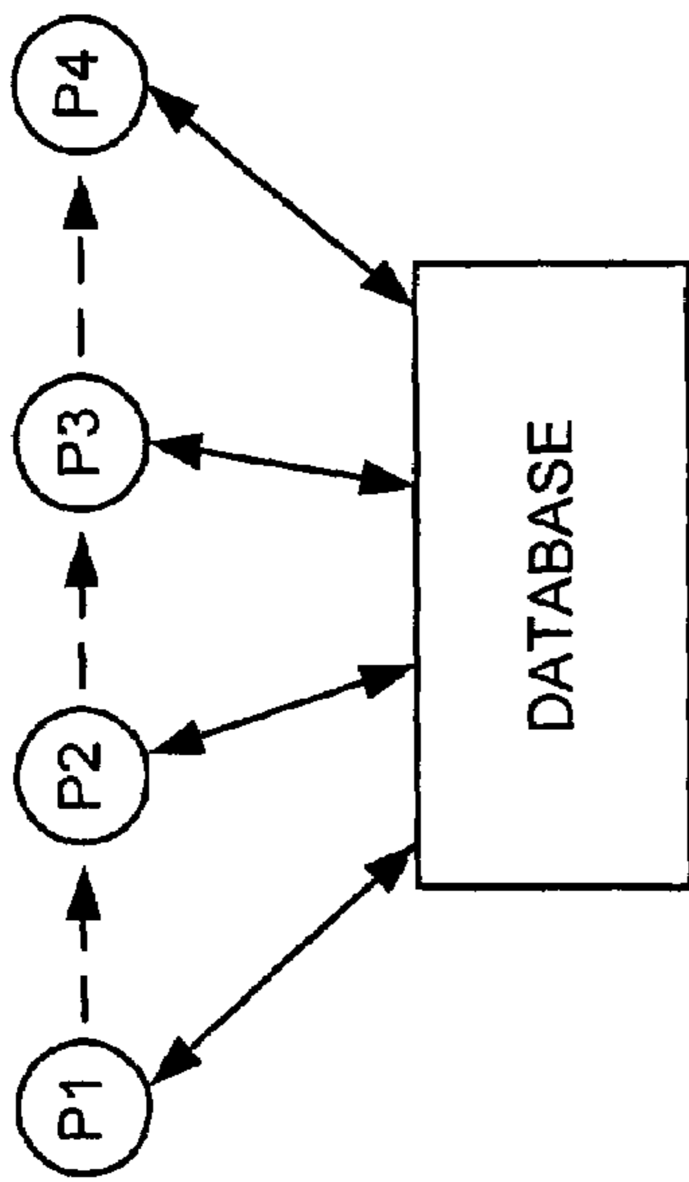
DATABASE WORKFLOW
