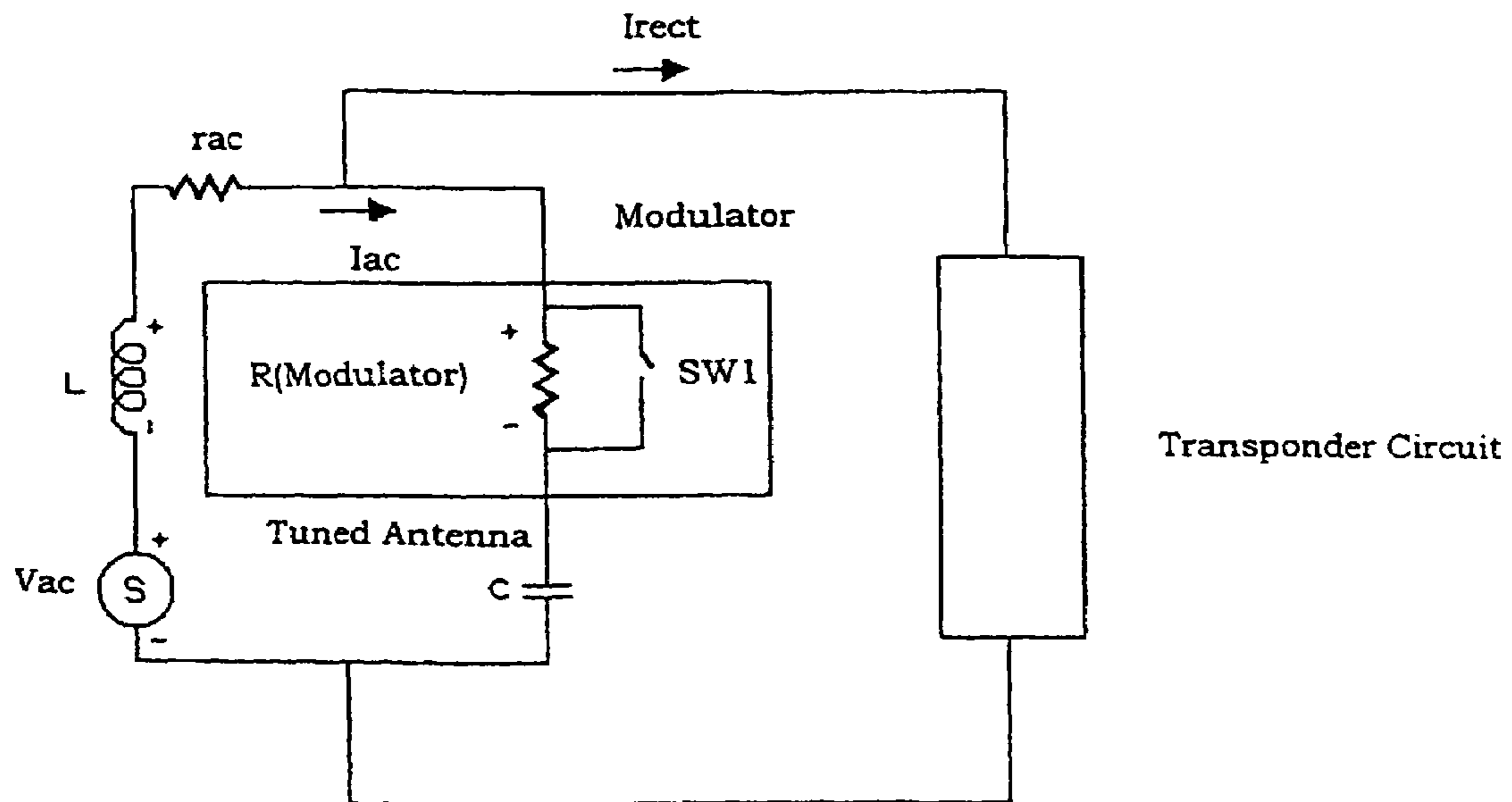
Figure 15(a): Invention with Transponder connected across Coil
