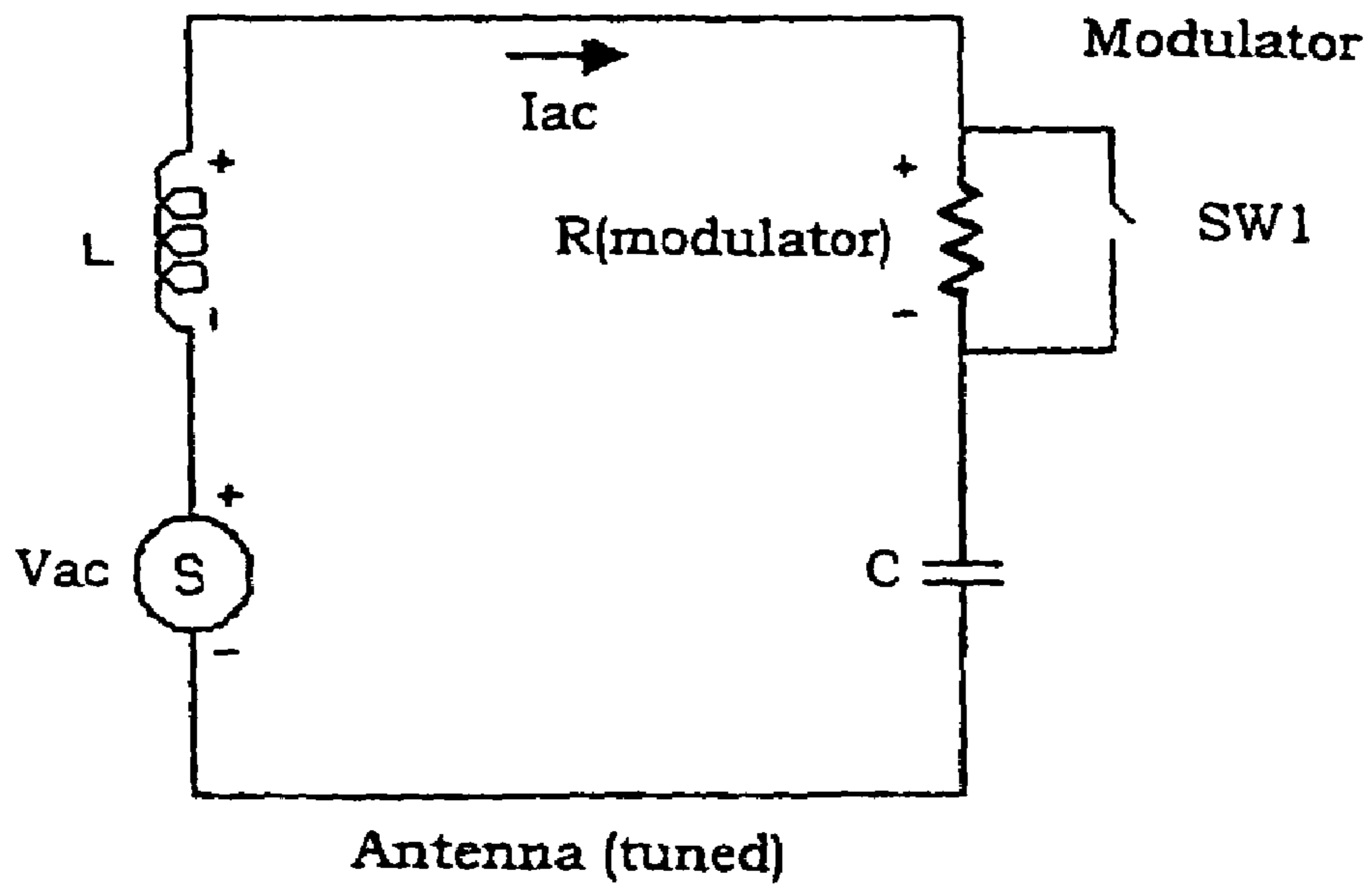
Figure 16: Embodiment of Invention
