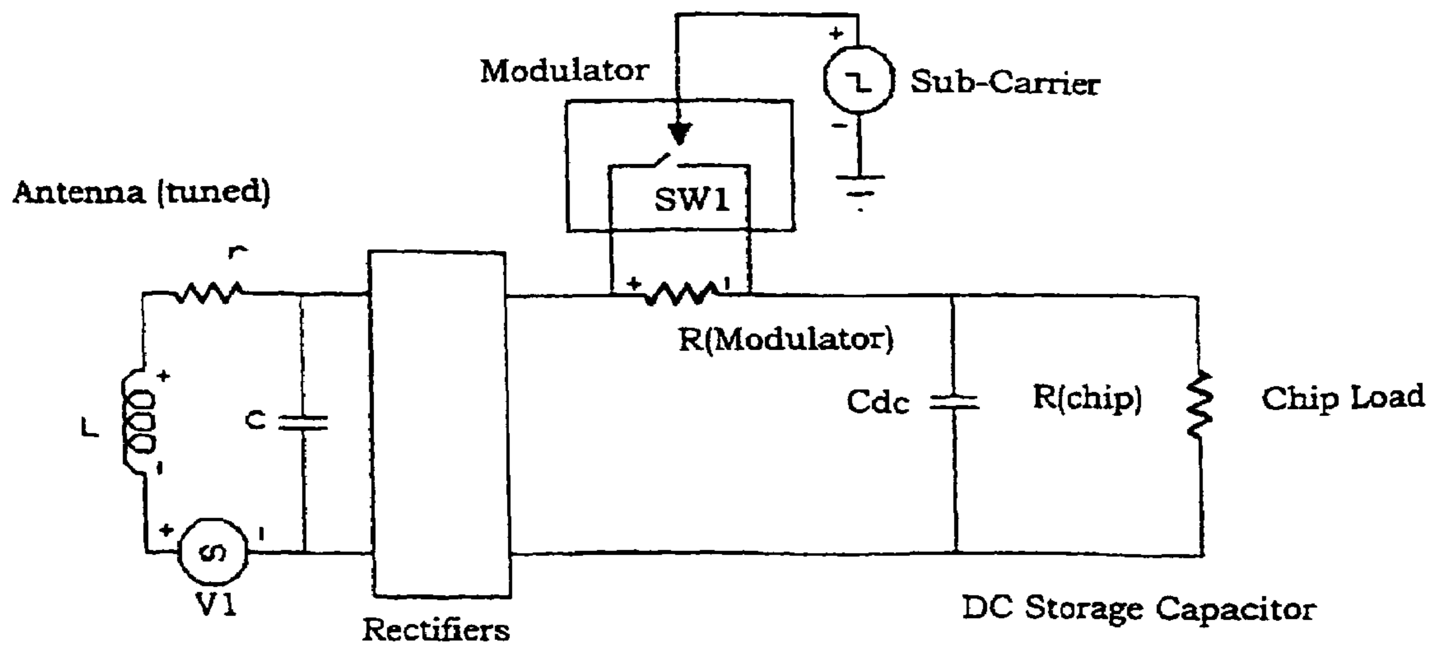
Figure 8(b): Invention with Sub-Carrier Modulation of Modulator in DC Circuit
