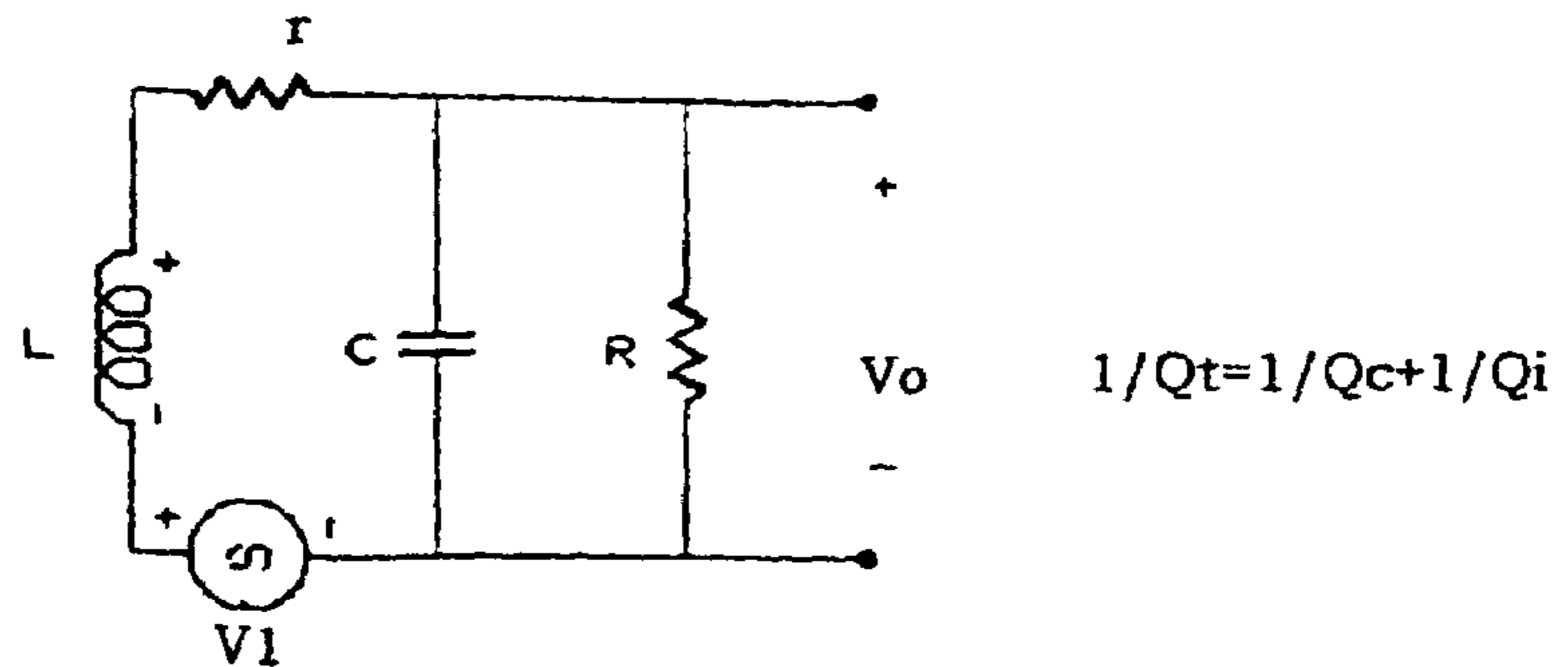
Figure 4(a): Data Rate Limited due to Q factor
