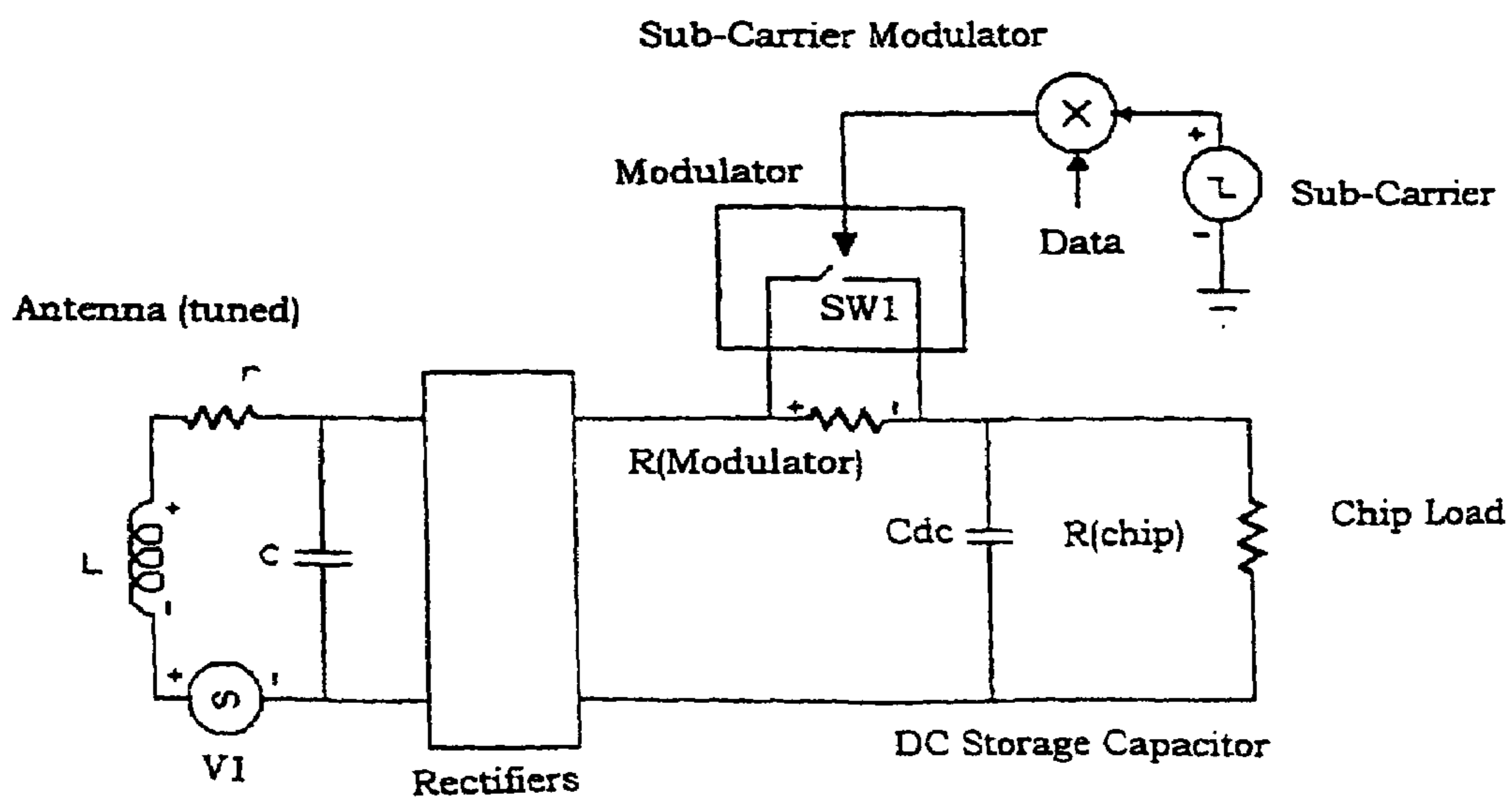
Figure 9(b): Invention with Data Modulated onto Sub-Carrier with Modulator in DC Circuit
