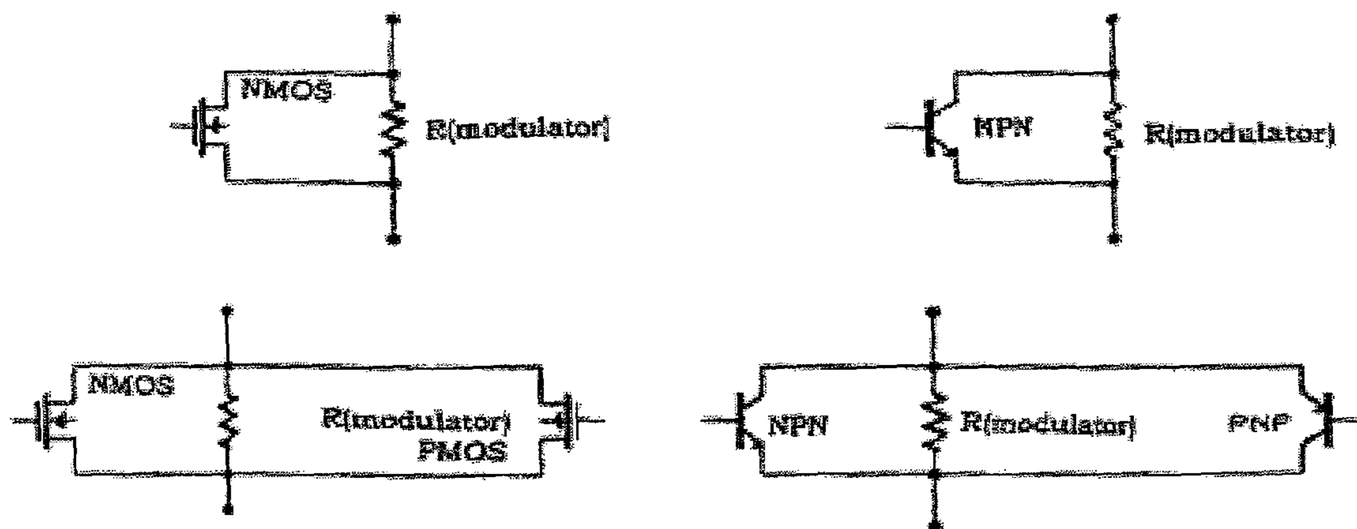
Figure 20(b): Examples of Modulation Switches
