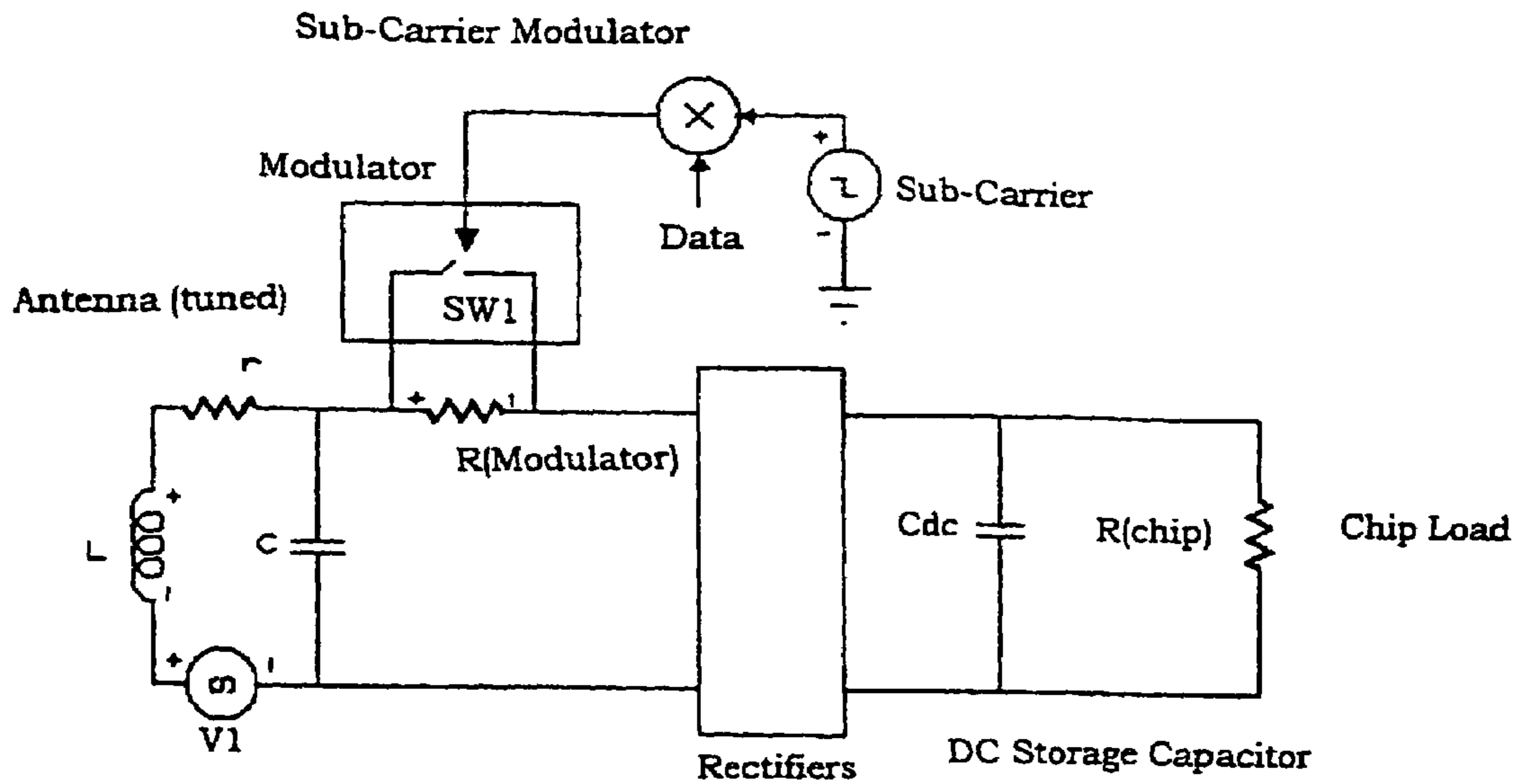
Figure 9(a): Invention with Data Modulated onto Sub-Carrier with Modulator in AC Circuit
