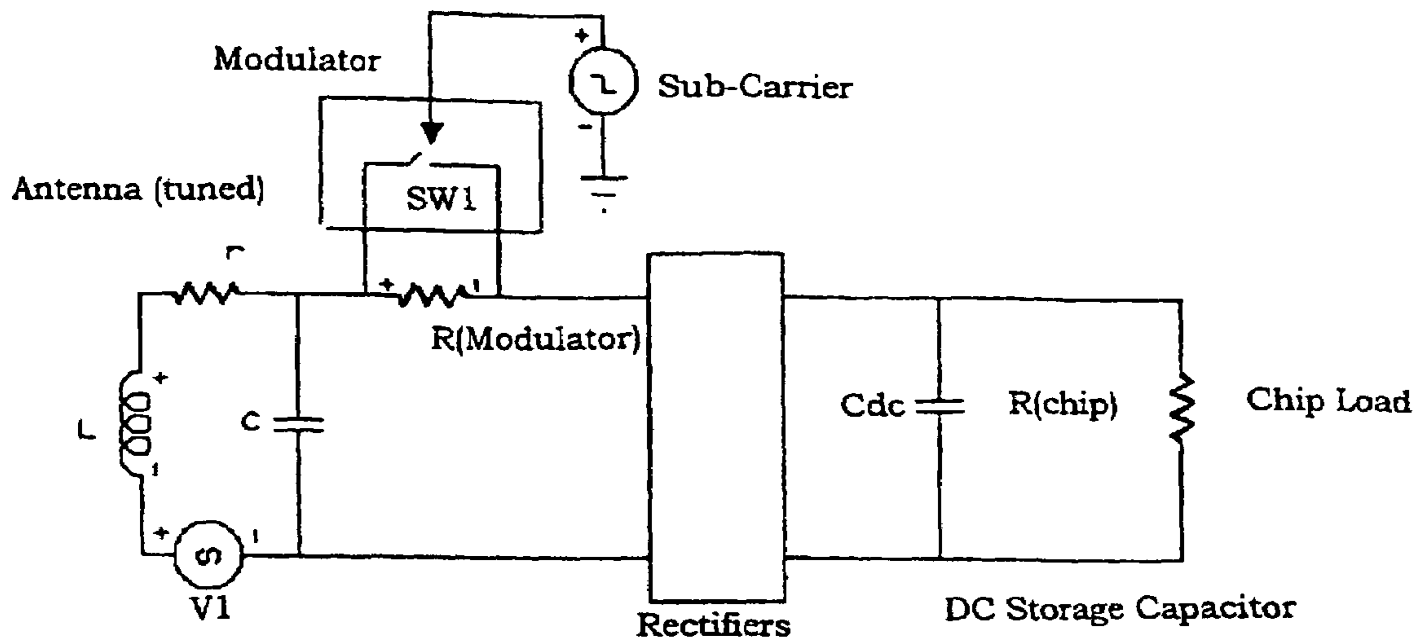
Figure 8(a): Invention with Sub-Carrier Modulation of Modulator in AC Circuit
