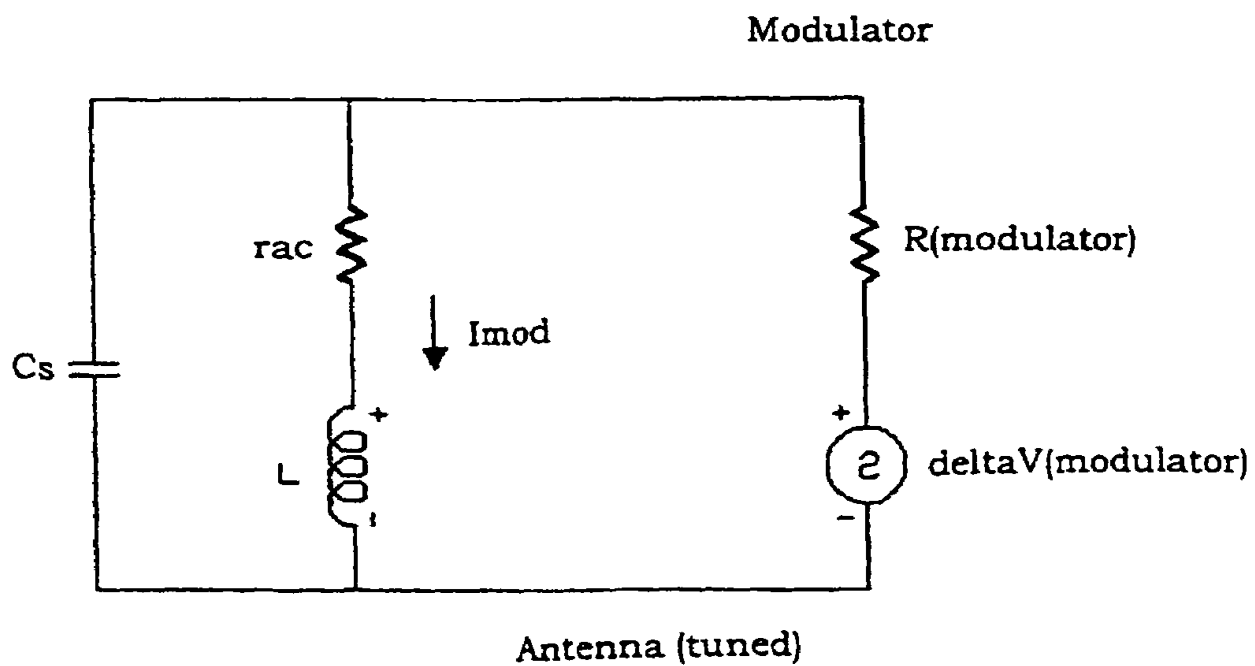
Figure 17(b): Electrical Model of the Invention at Radio Frequency
