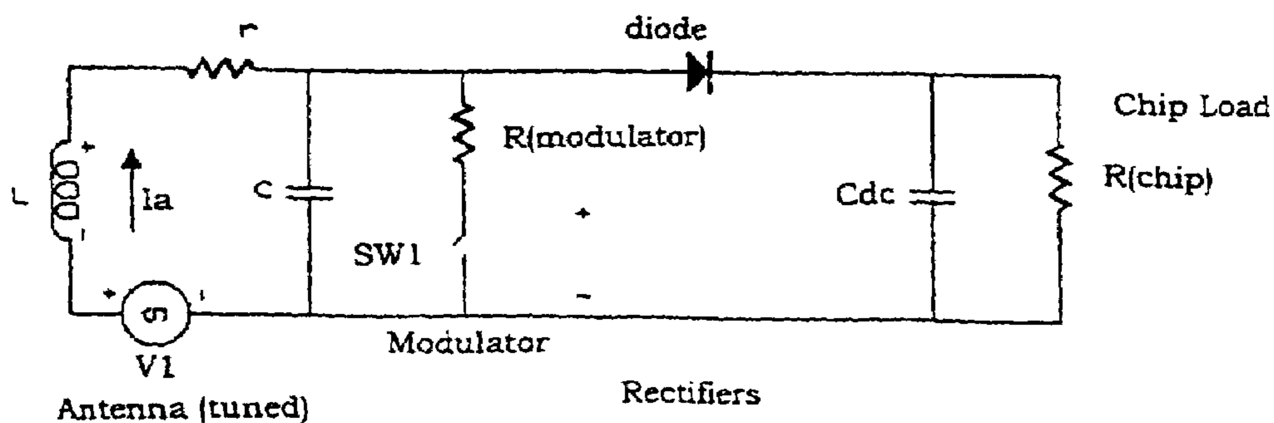
Figure 3: Electrical Model for Prior Art Circuit
