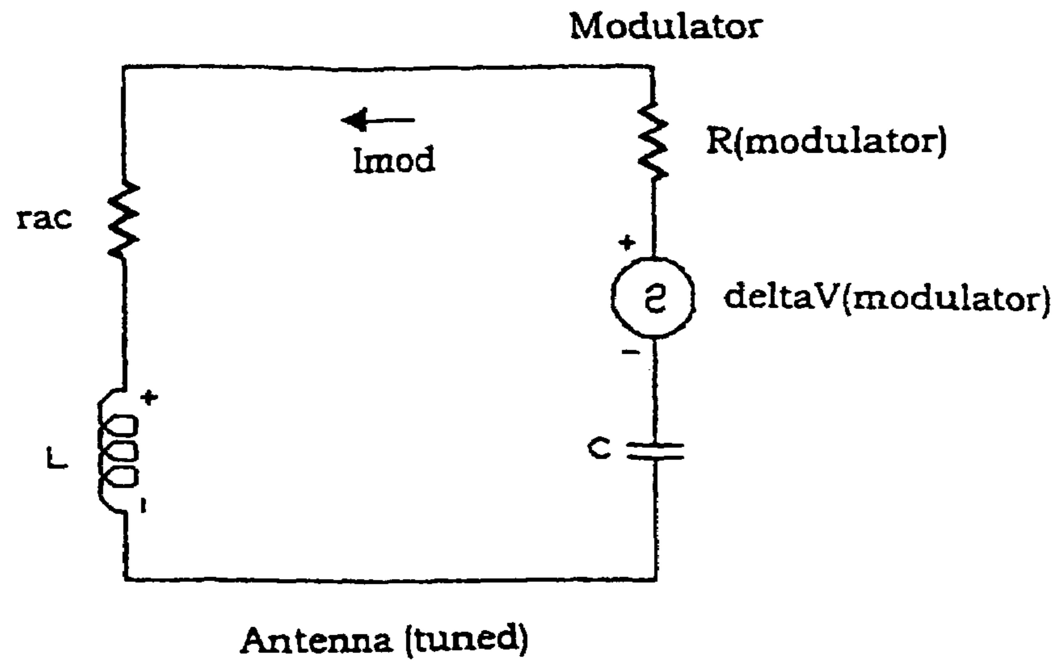
Figure 17(a): Electrical Model of the Invention at Tuned Frequency
