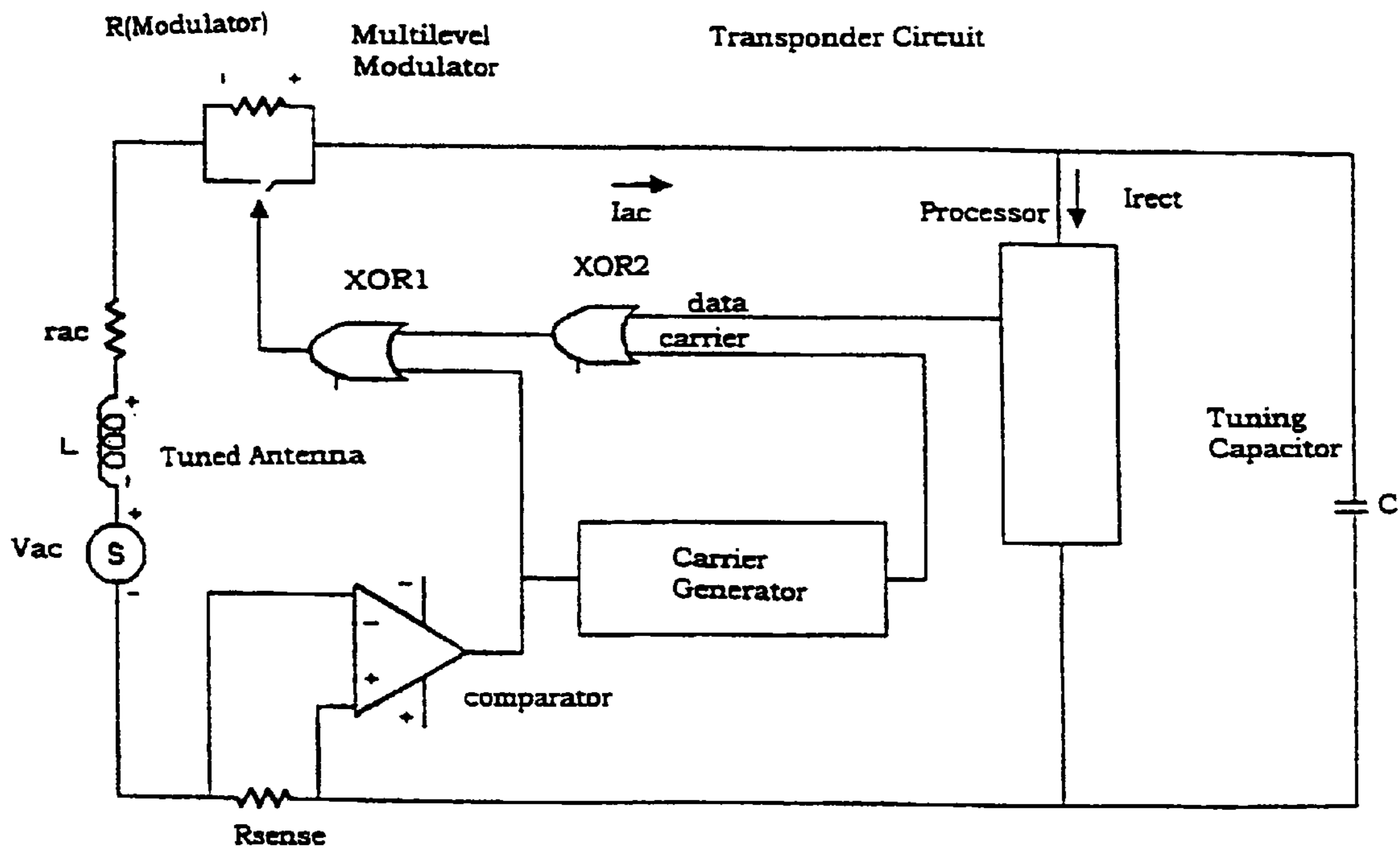
Figure 21: Circuit embodiment of Invention
