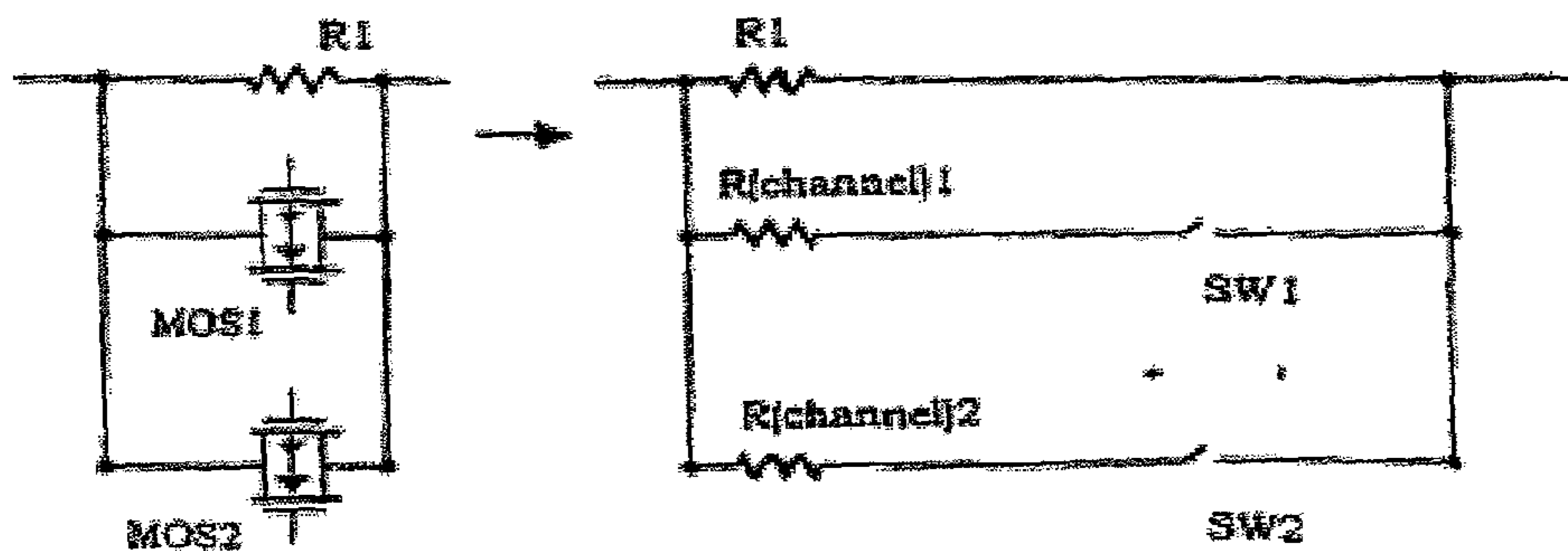
Figure 20(d): Resistance varied between several values
