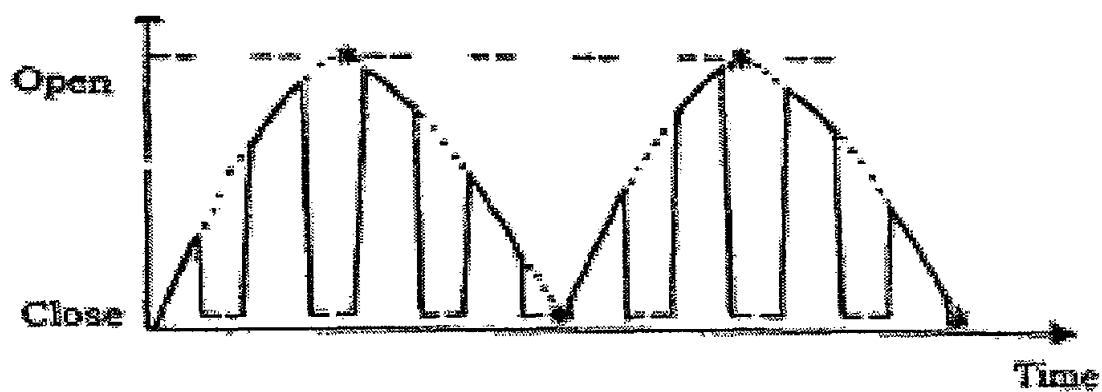
Figure 18(c): Magnitude of V(\text{modulator})
