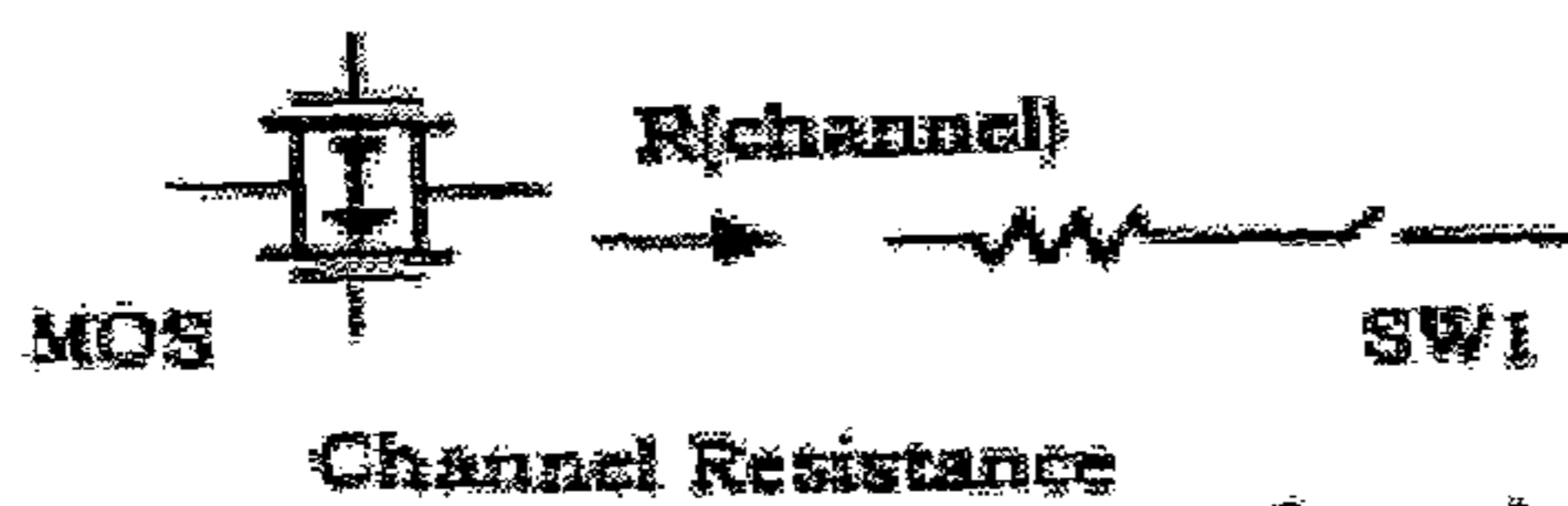
Figure 20(c): Use of Channel Resistance to make Switchable Resistances
