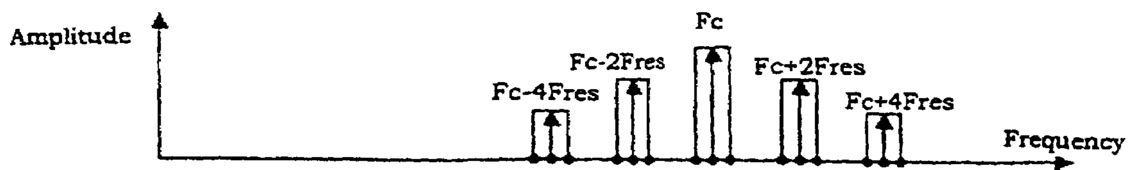
Figure 19(c): Spectrum of V(\text{modulator})
