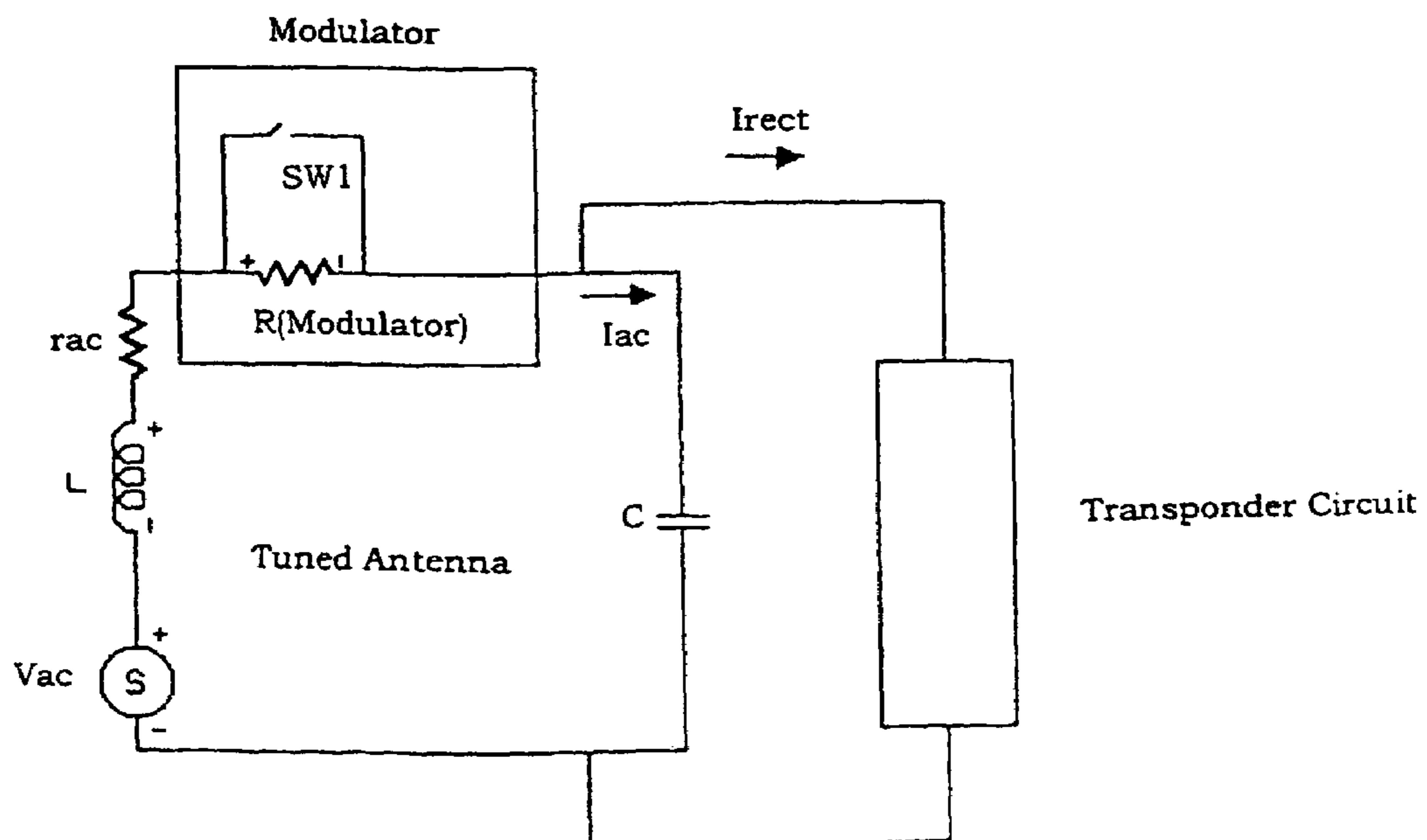
Figure 15(b): Invention with Transponder connected across Tuning Capacitor
