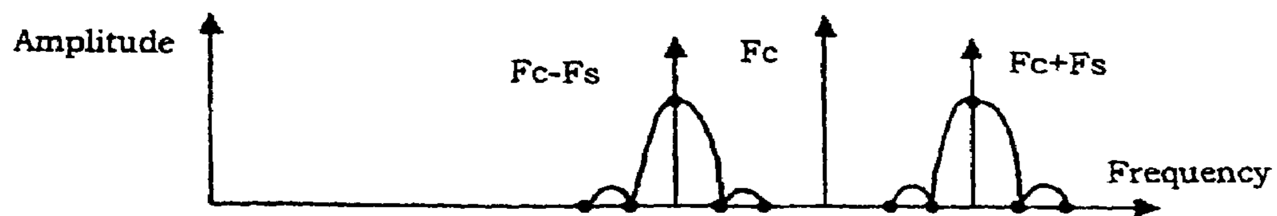
Figure 10(g): Spectrum Data Modulated Sub-Carrier Amplitude Modulated onto Excitation Frequency
