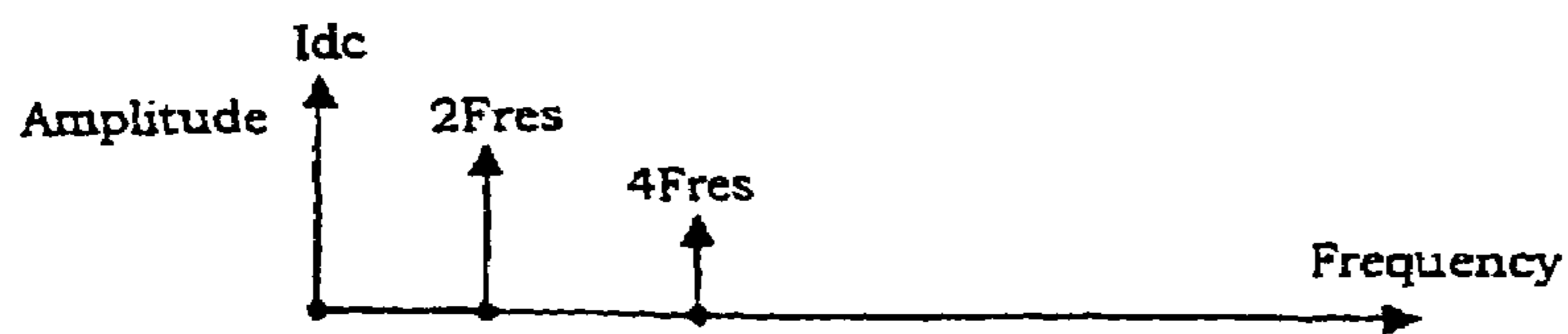
Figure 19(a): Spectrum of I_{dc} Fullwave Rectified
