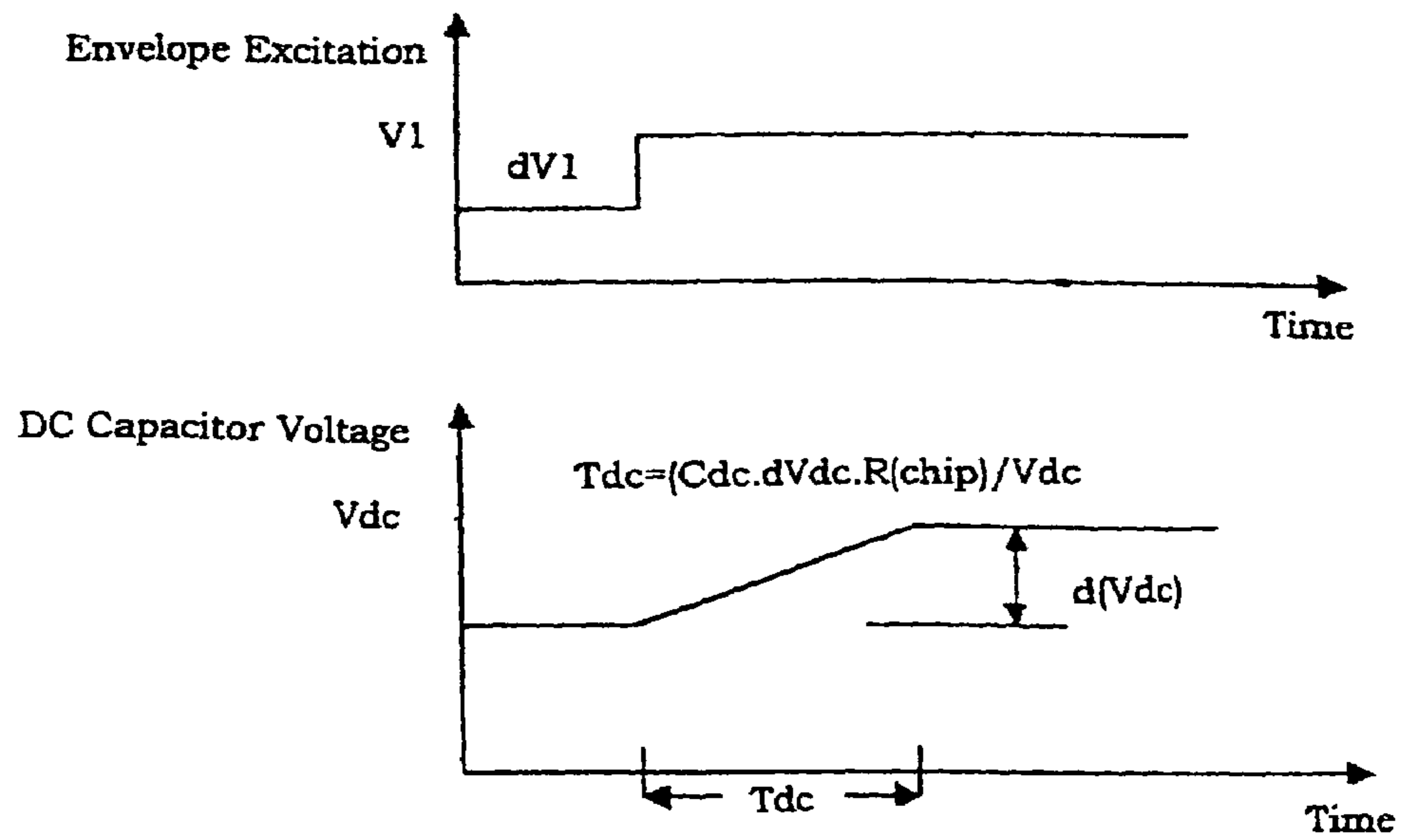
Figure 4(d): DC Waveform associated with DC Storage Limit
