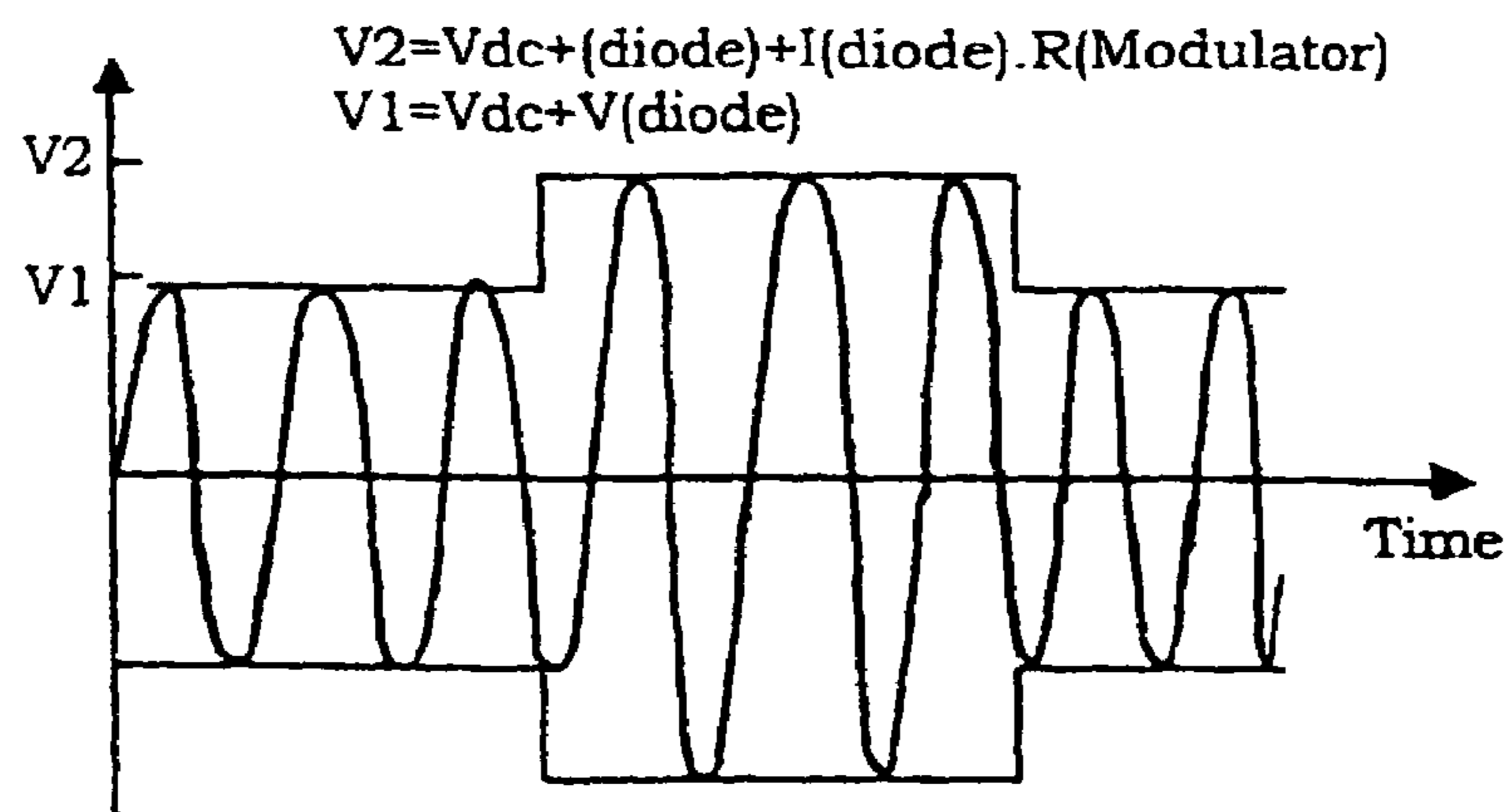
Figure 10(a): Switch Function
