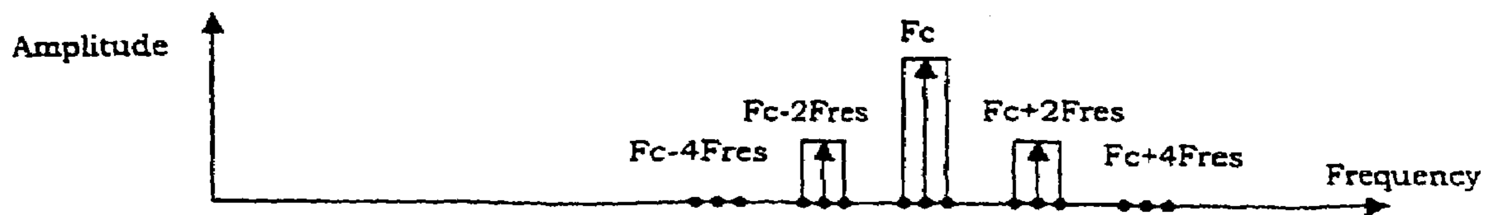
Figure 19(d): Spectrum of V(\text{modulator}) with Waveshaping
