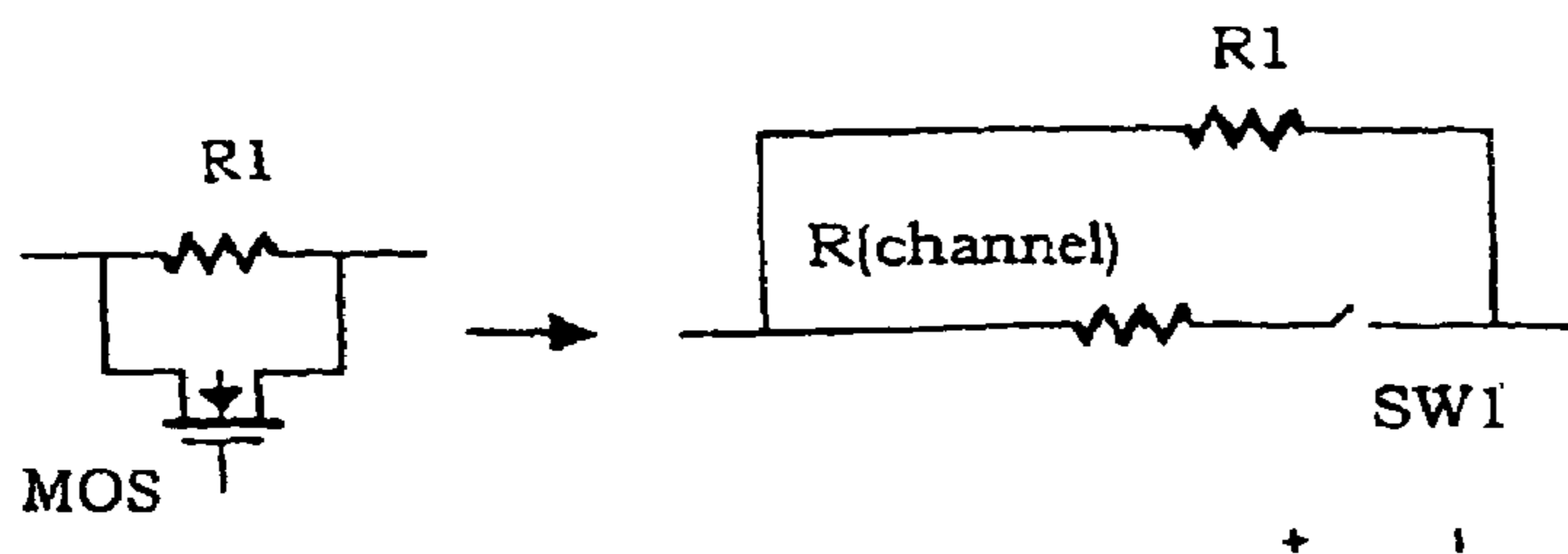
Figure 12(d): Resistance varied between Two Values
