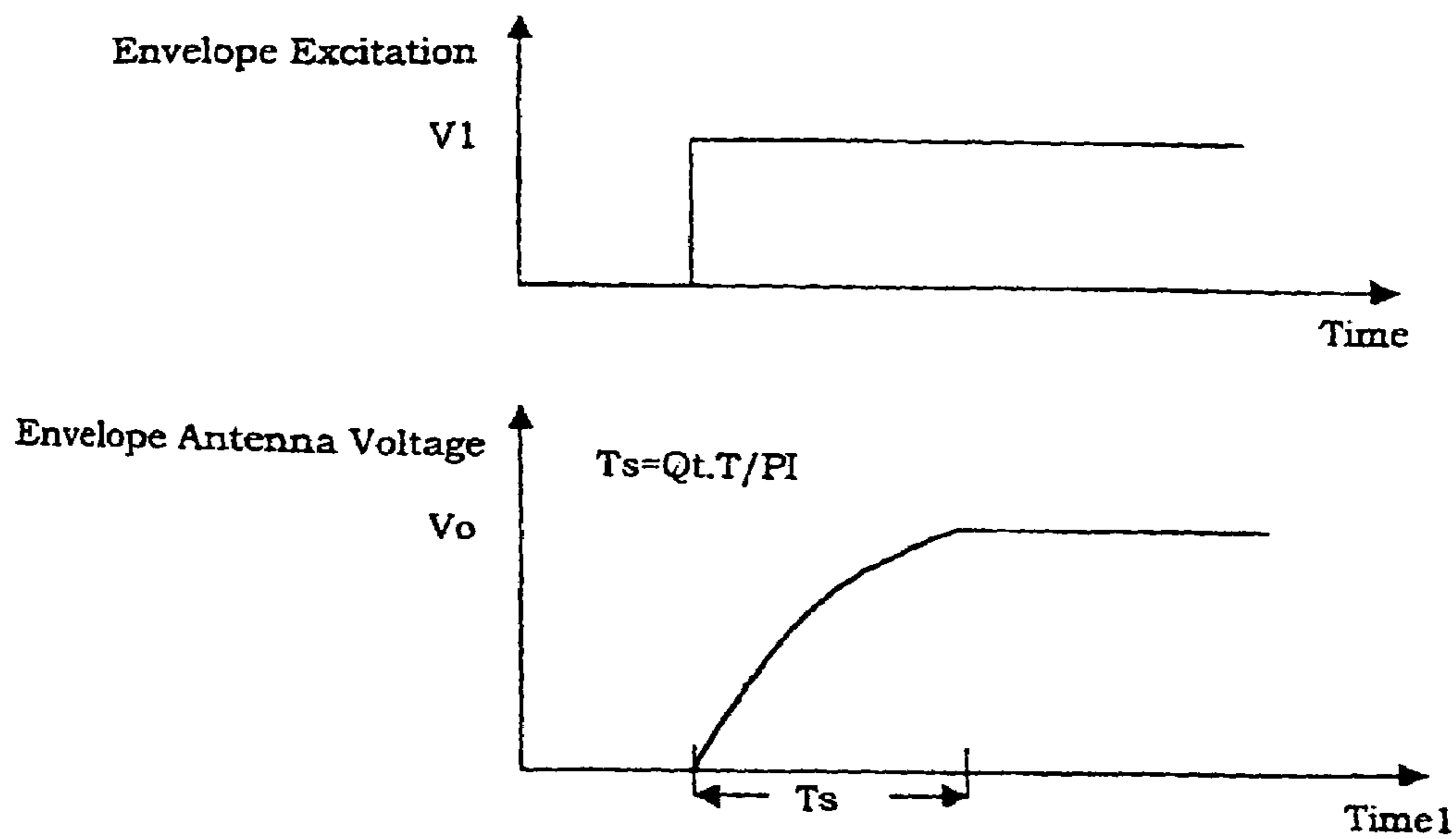
Figure 4(b): Envelope of Waveform associated with Q factor
