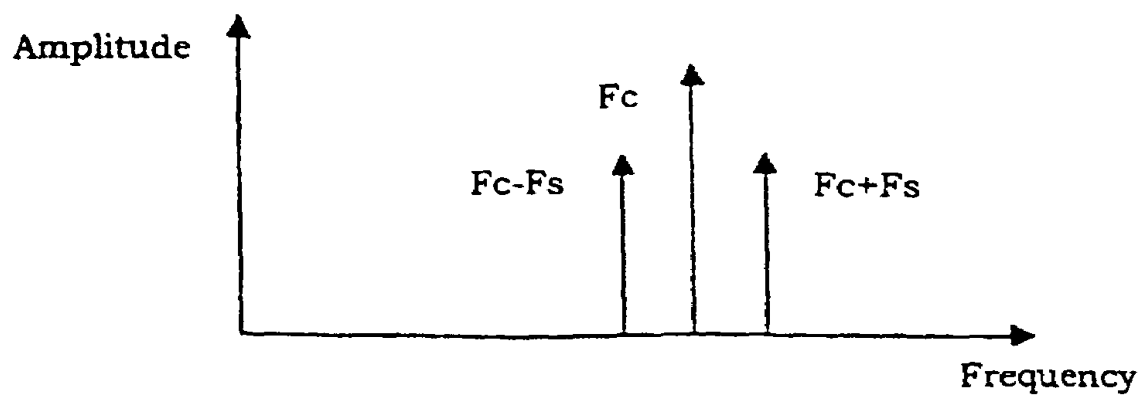
Figure 10(c): Sub-Carrier Spectrum
