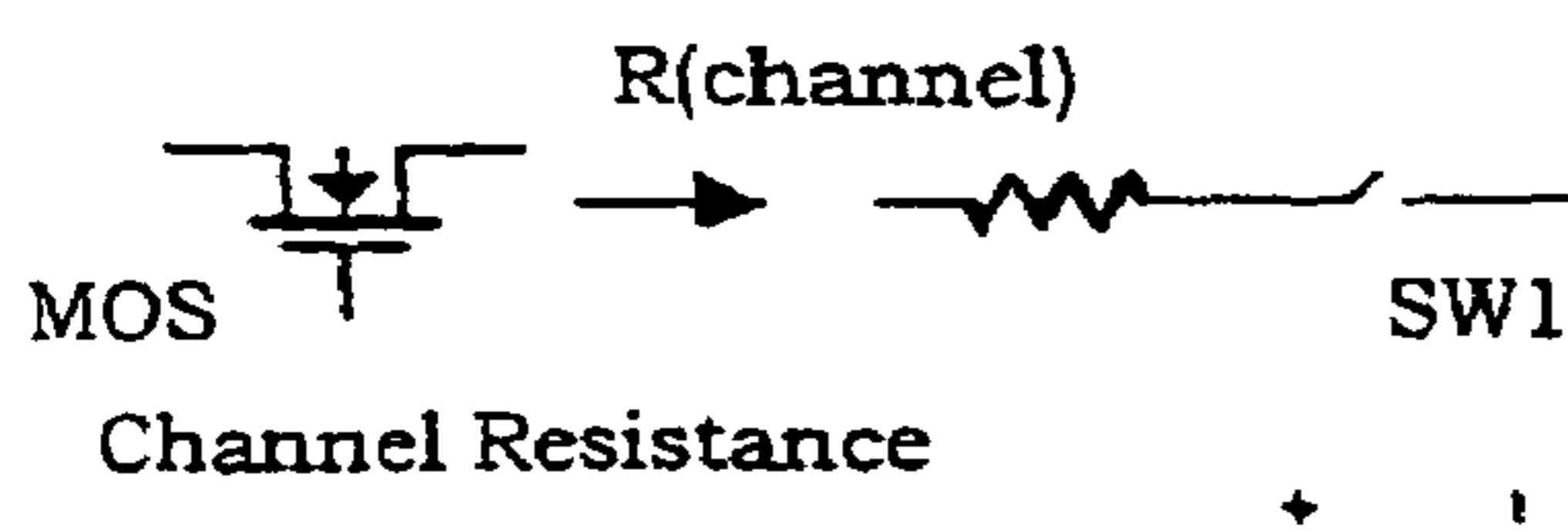
Figure 12(c): Use of Channel Resistance to make Switchable Resistances
