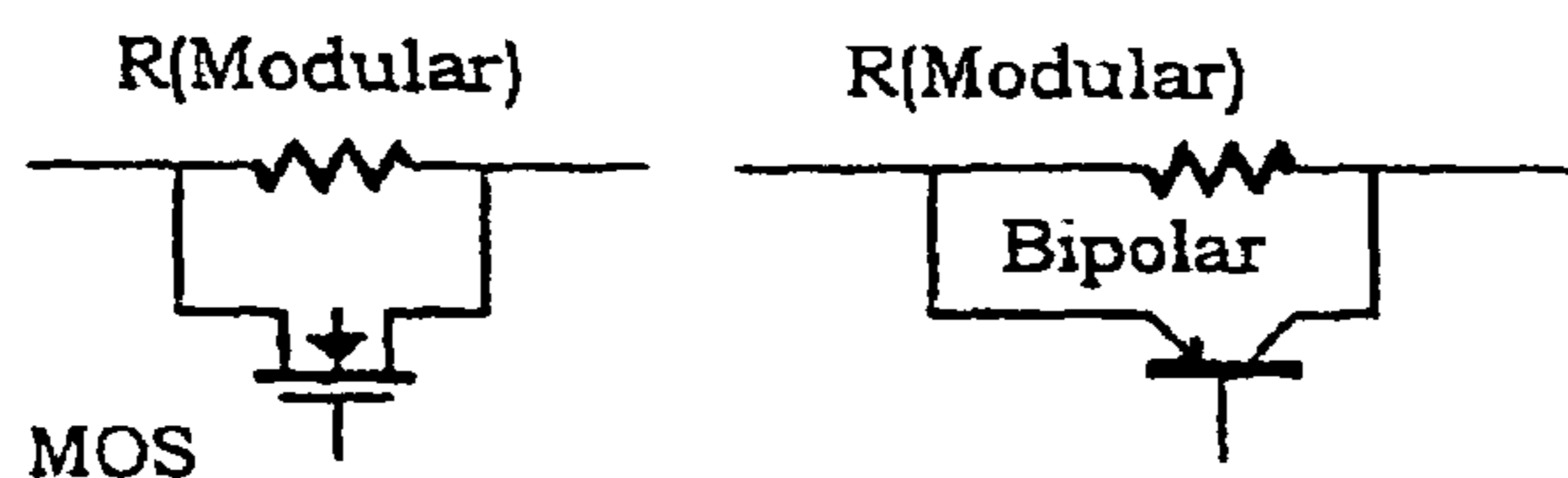
Figure 12(b): Examples of Modulation Switches
