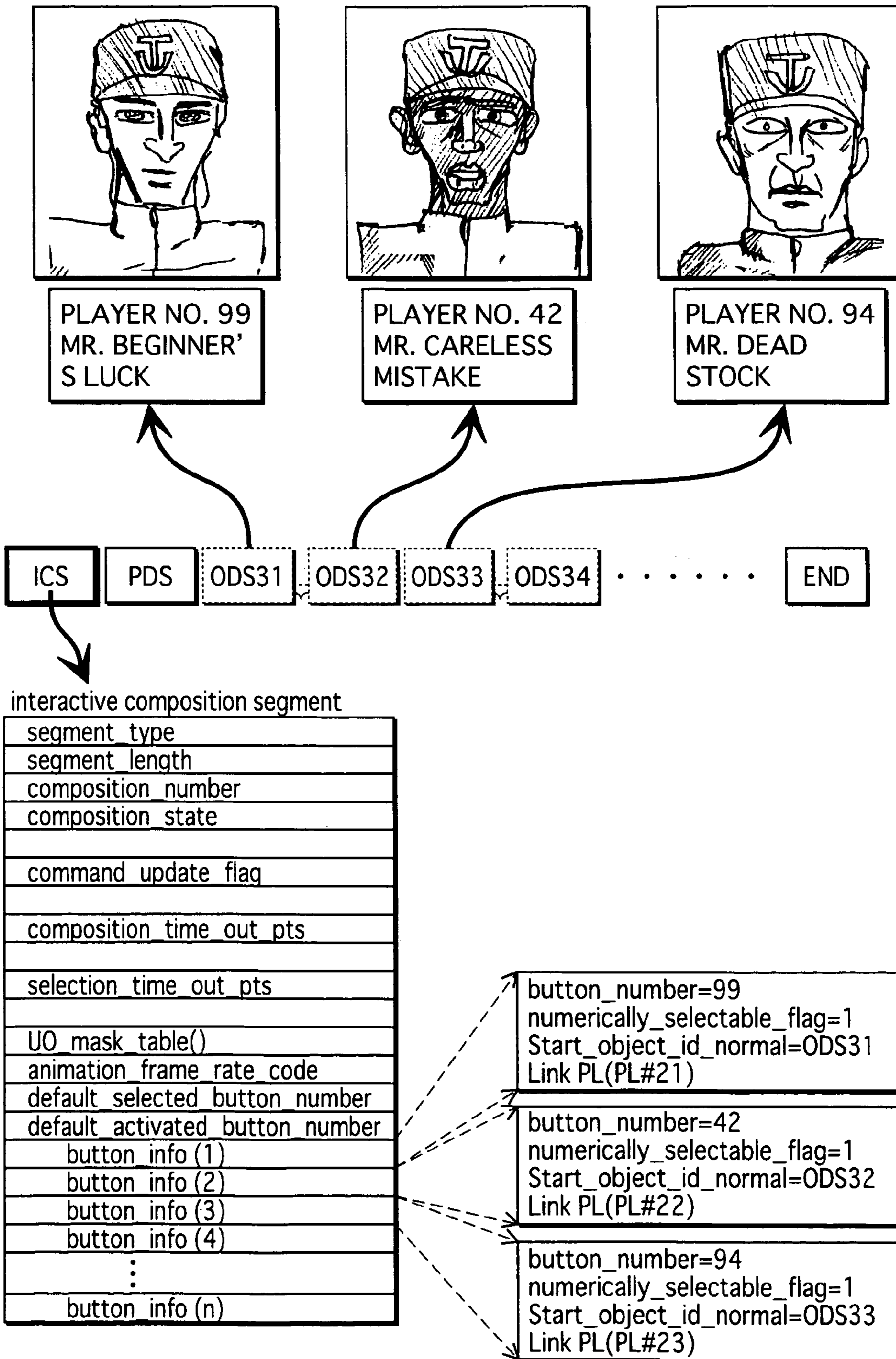
FIG. 18 PLAYERS LIST
