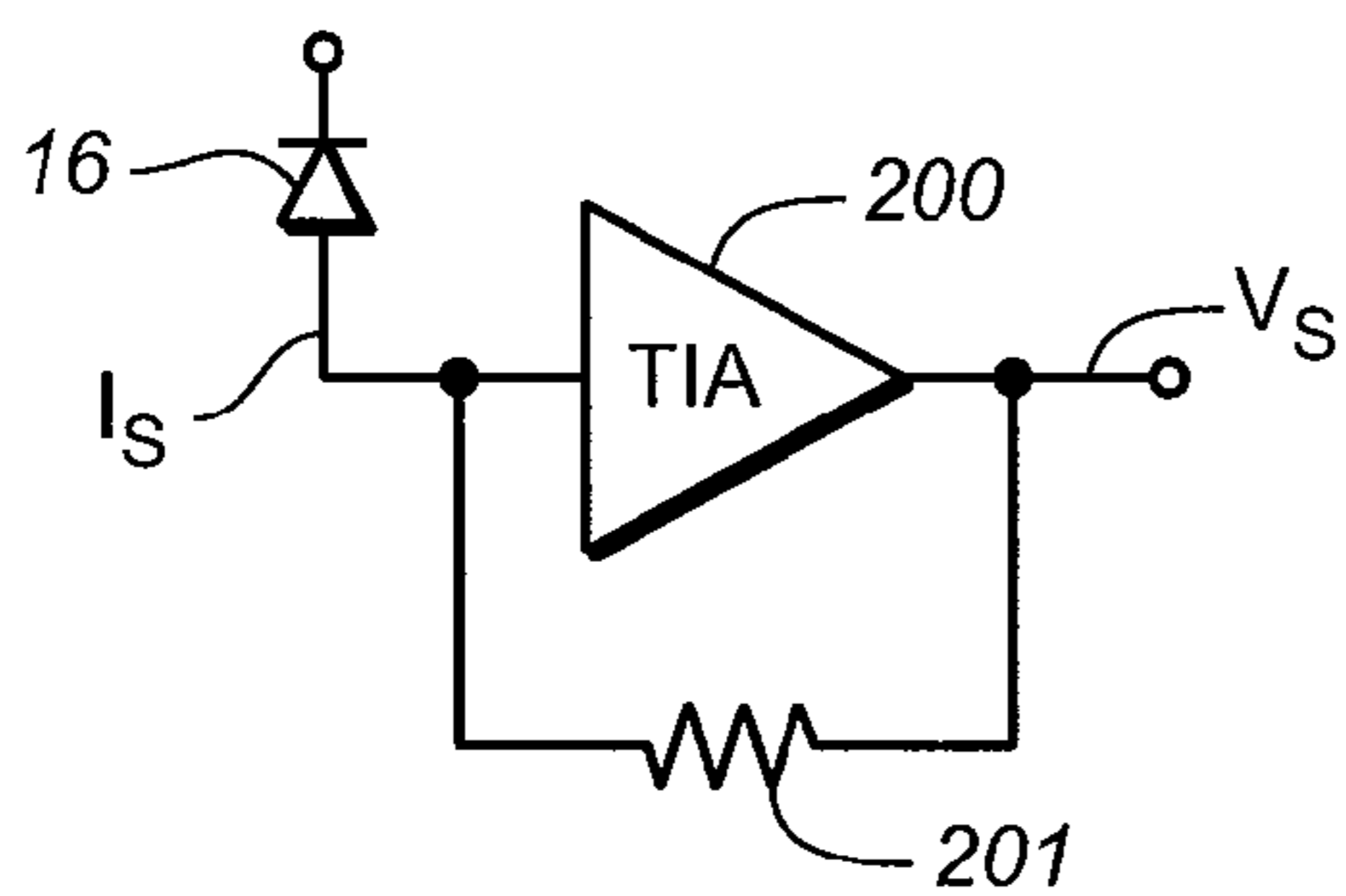
FIG. 48 (PRIOR ART)
