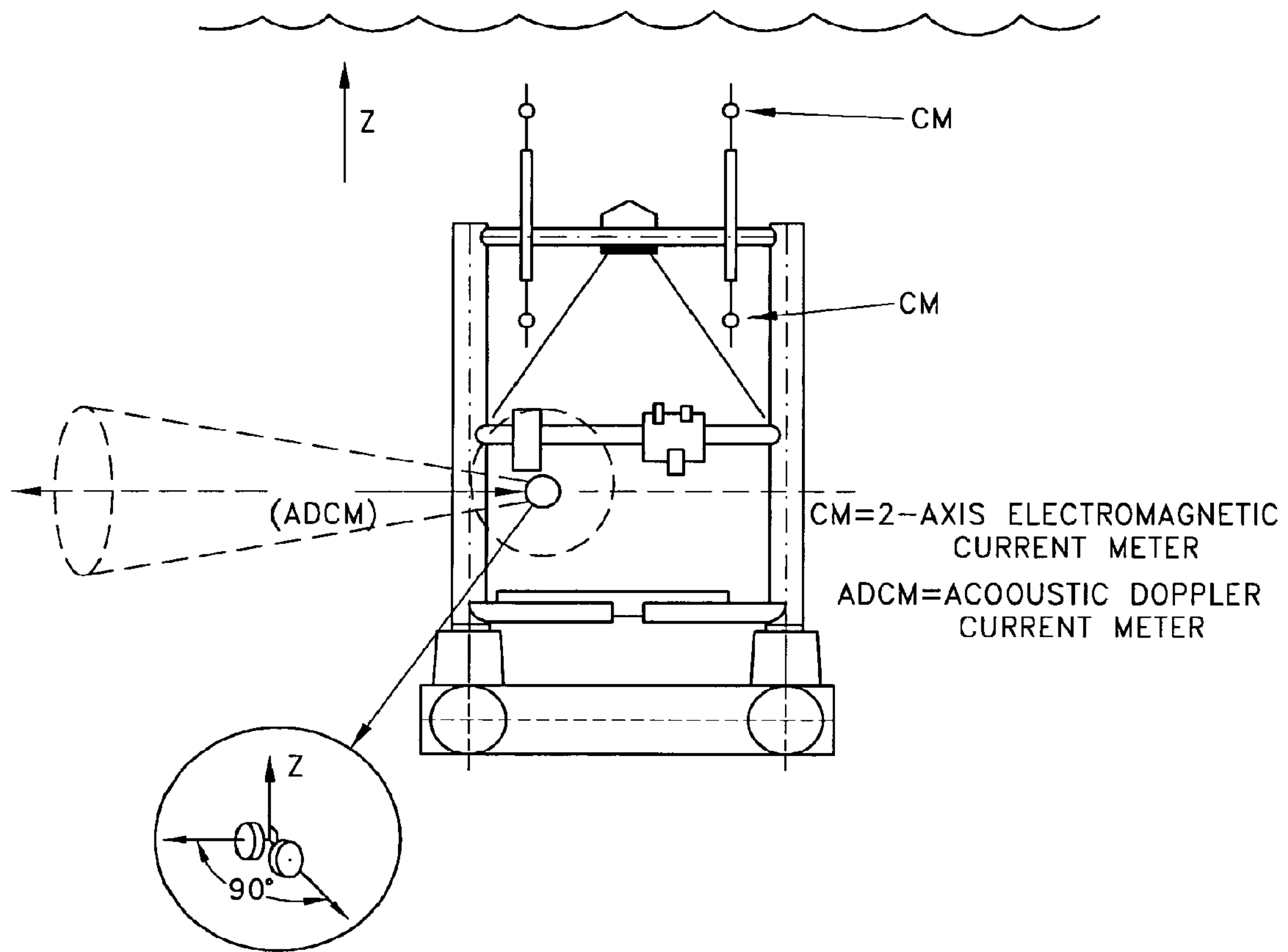
FIG. 1 (PRIOR ART)
