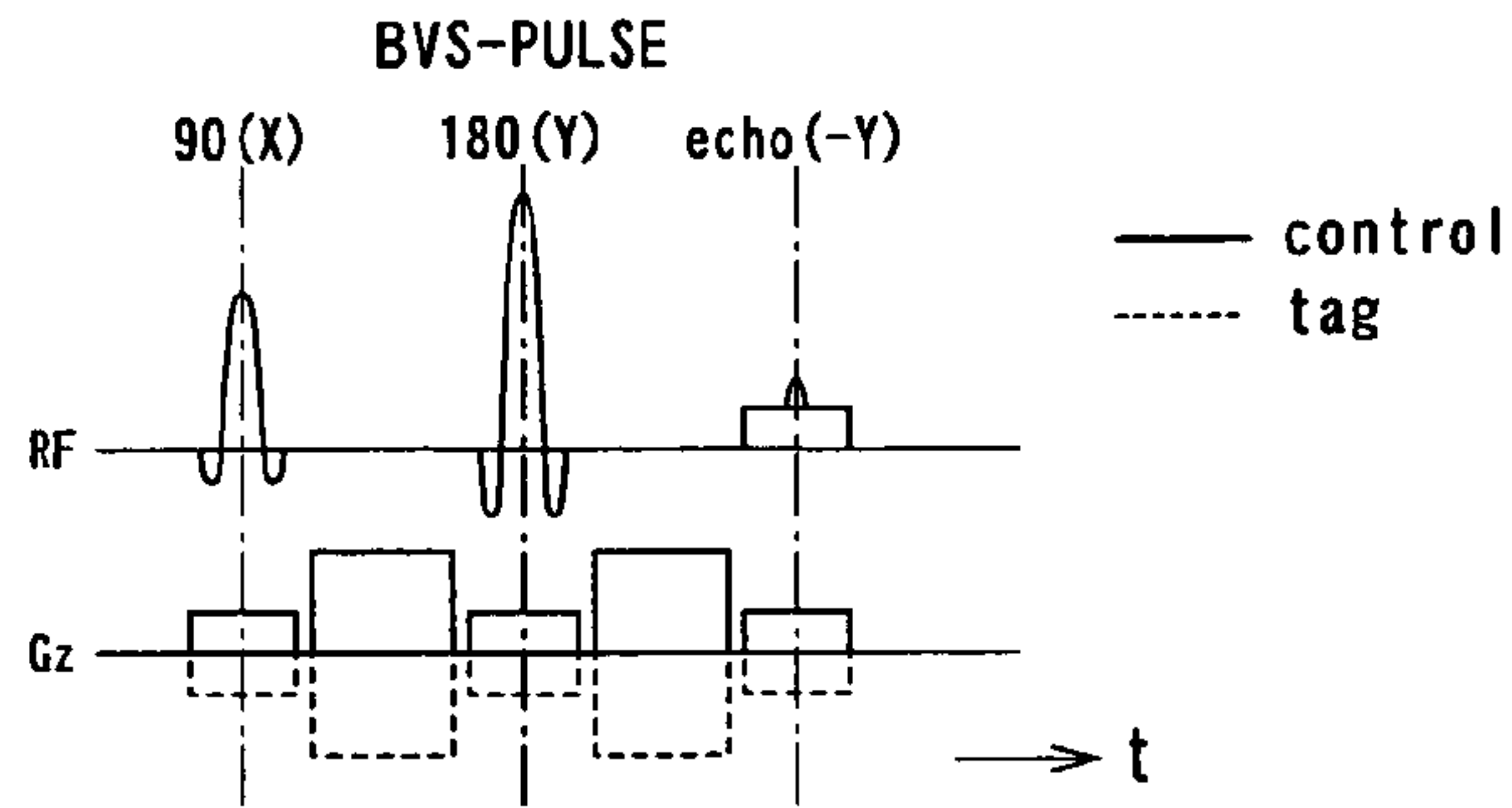
MEASUREMENT BY PHASE-MEASURING PULSE SEQUENCE (IN EACH OF CONTROL AND TAG MODES)
