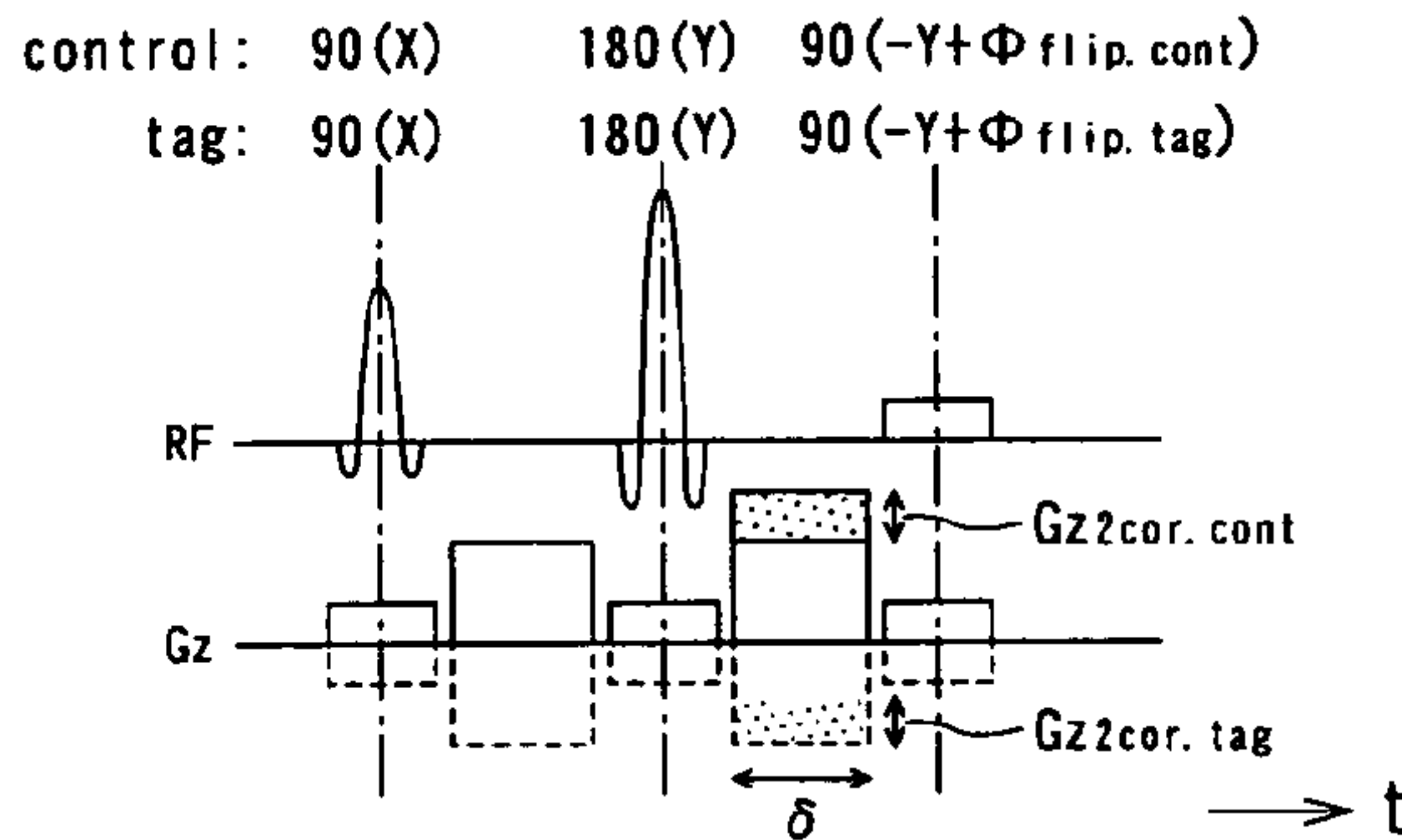
SEQUENCE AFTER PHASE COMPENSATION (IN EACH OF CONTROL AND TAG MODES)
