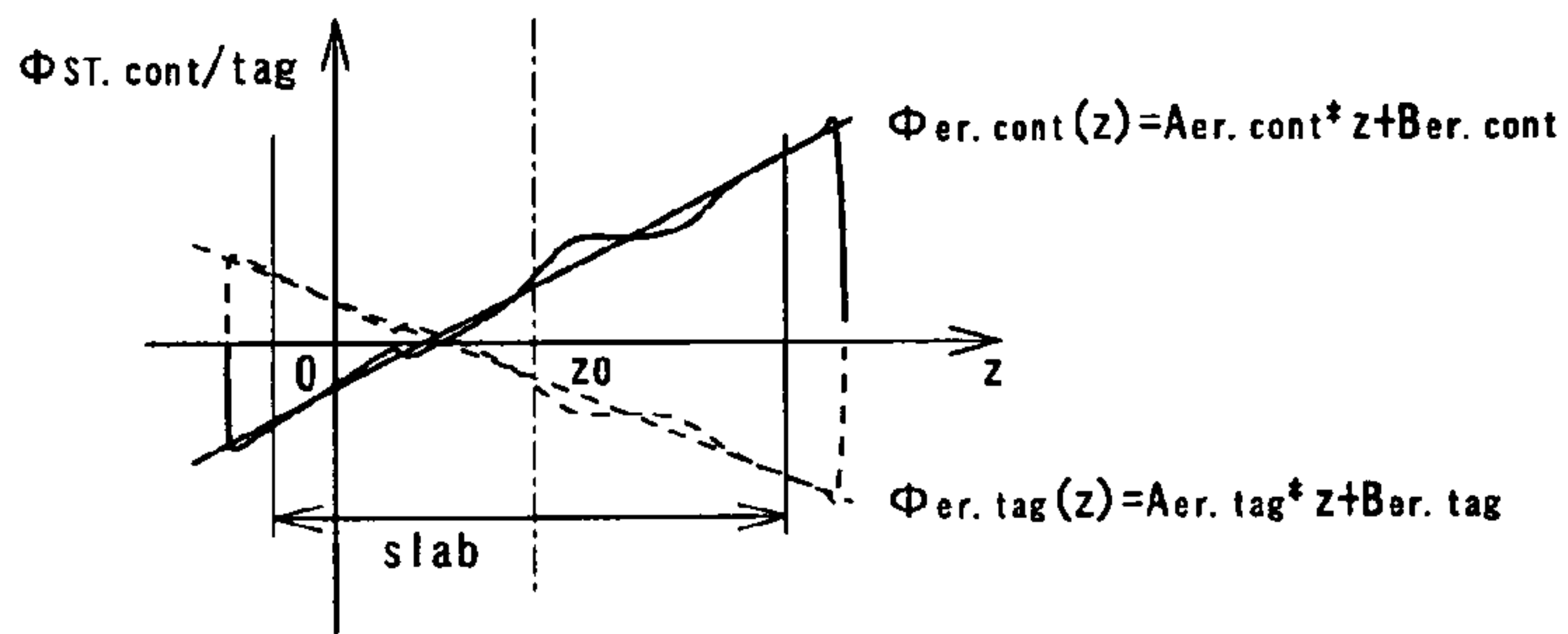
COMPUTATION OF PHASE DISTRIBUTION (IN EACH OF CONTROL AND TAG MODES)
