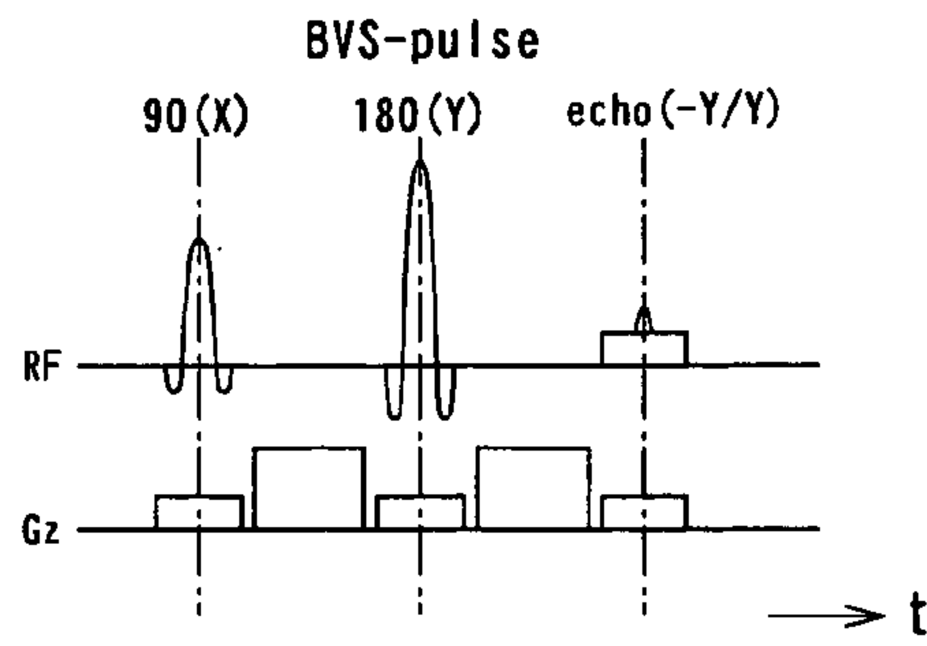
MEASUREMENT BY PHASE-MEASURING PULSE SEQUENCE (IN EACH OF CONTROL AND TAG MODES)
