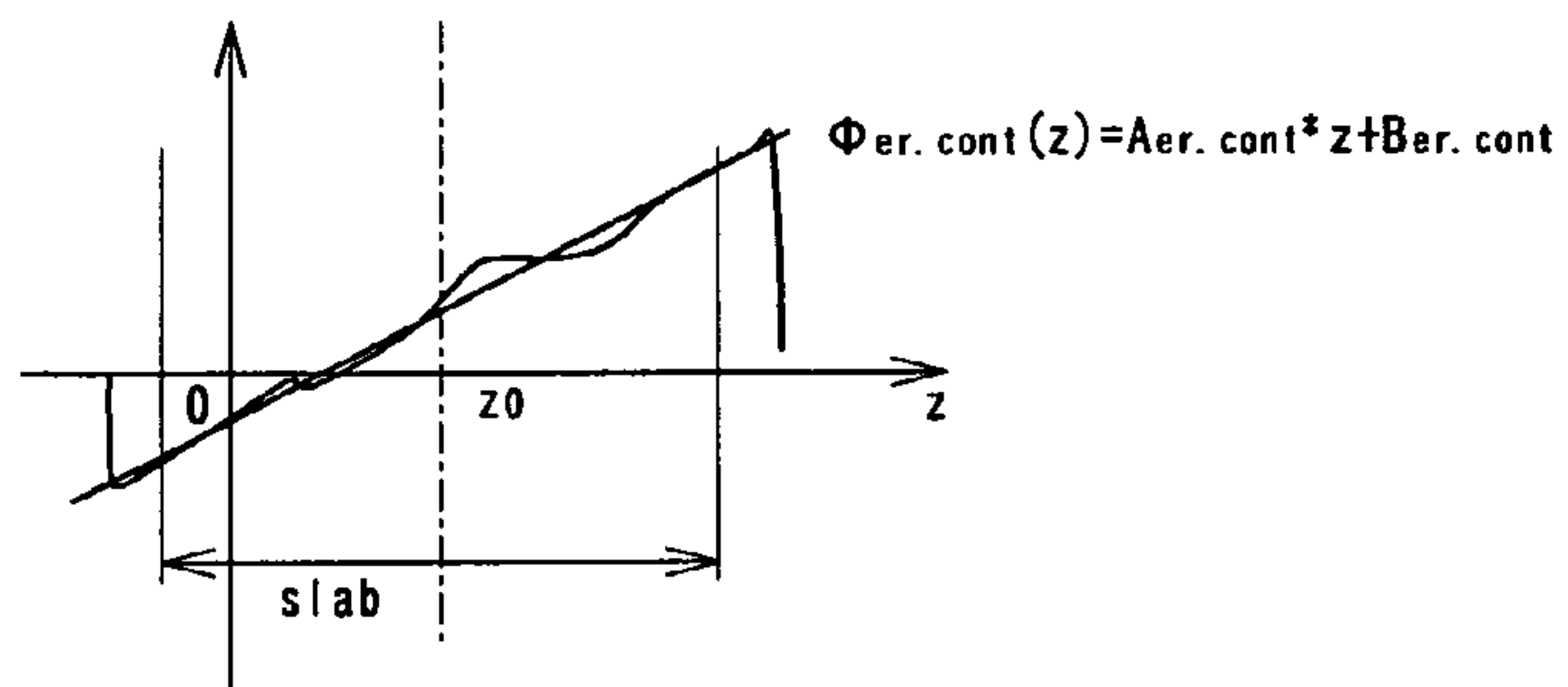
COMPUTATION OF PHASE DISTRIBUTION (IN EACH OF CONTROL AND TAG MODES)
