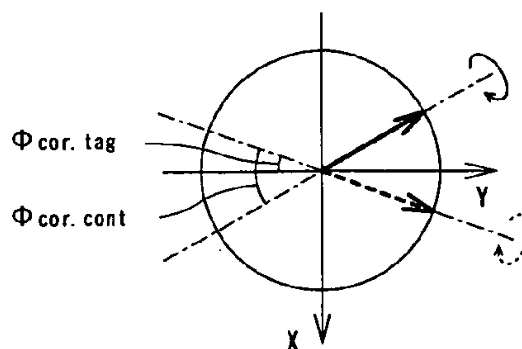
FLIP-BACK PHASE (IN CONTROL/TAG MODE)
