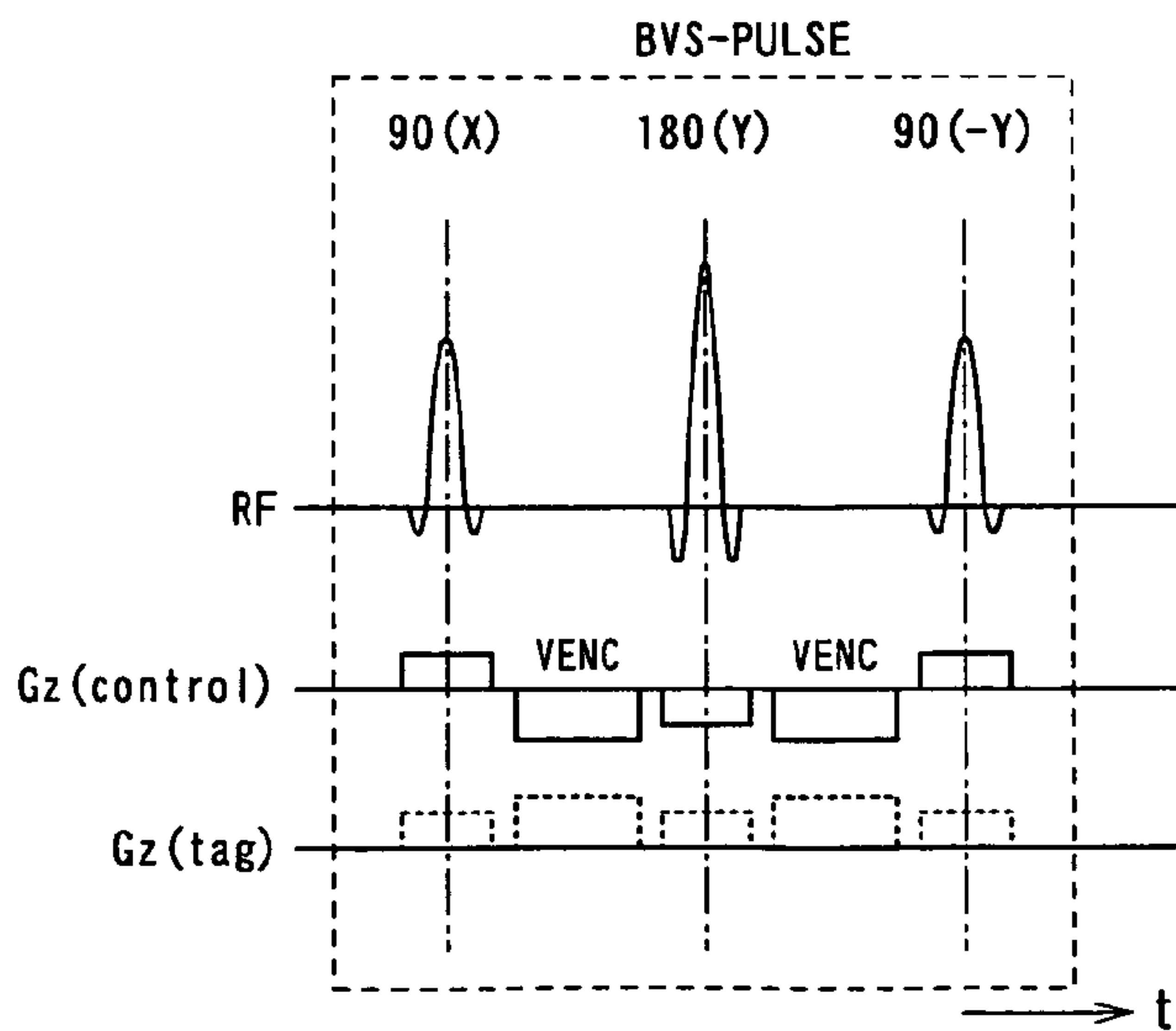
SLICE-SELECTIVE MODIFICATION OF VS-ASL TECHNIQUE OF UNIPOLAR-VENC TYPE
