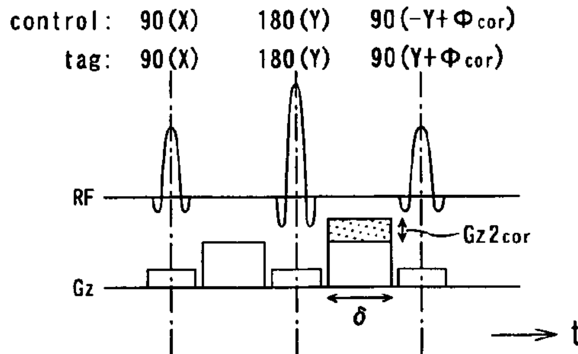
SEQUENCE AFTER PHASE COMPENSATION (QUANTITY OF COMPENSATION, Gz2 , IS COMMON IN CONTROL AND TAG MODES)
