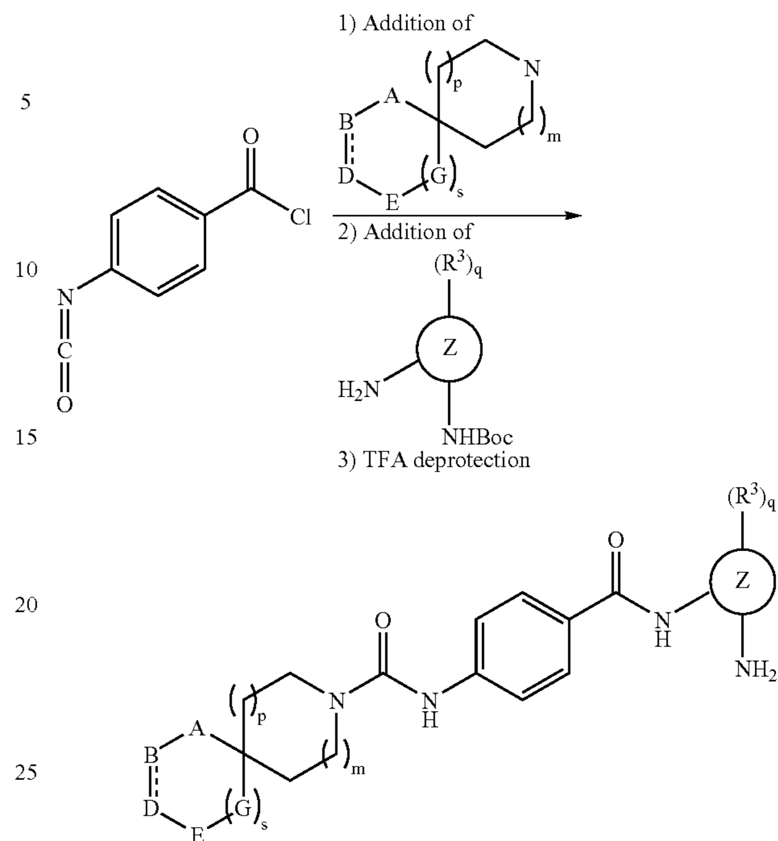
SCHEME 8
