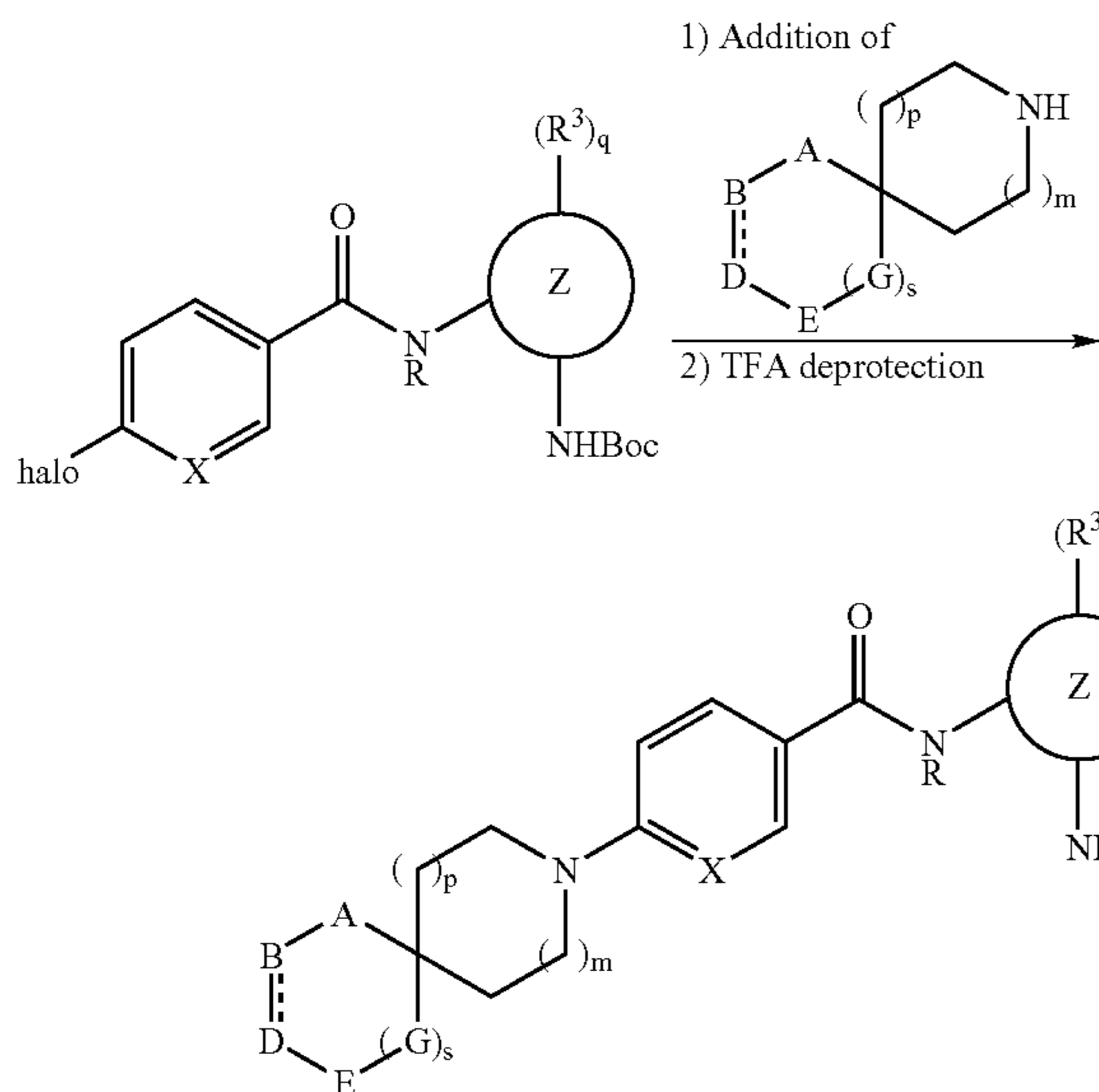
SCHEME 1
