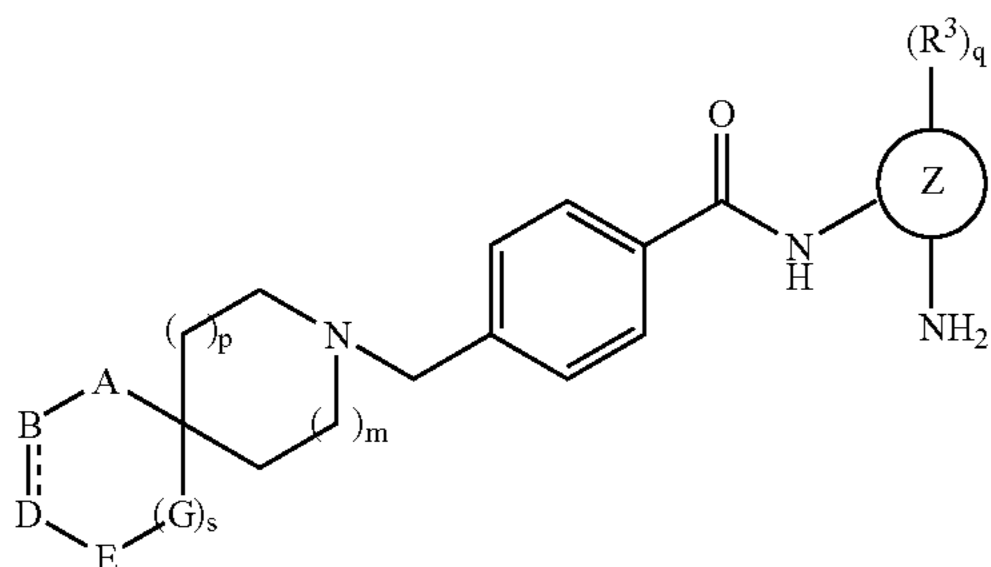
SCHEME 7
