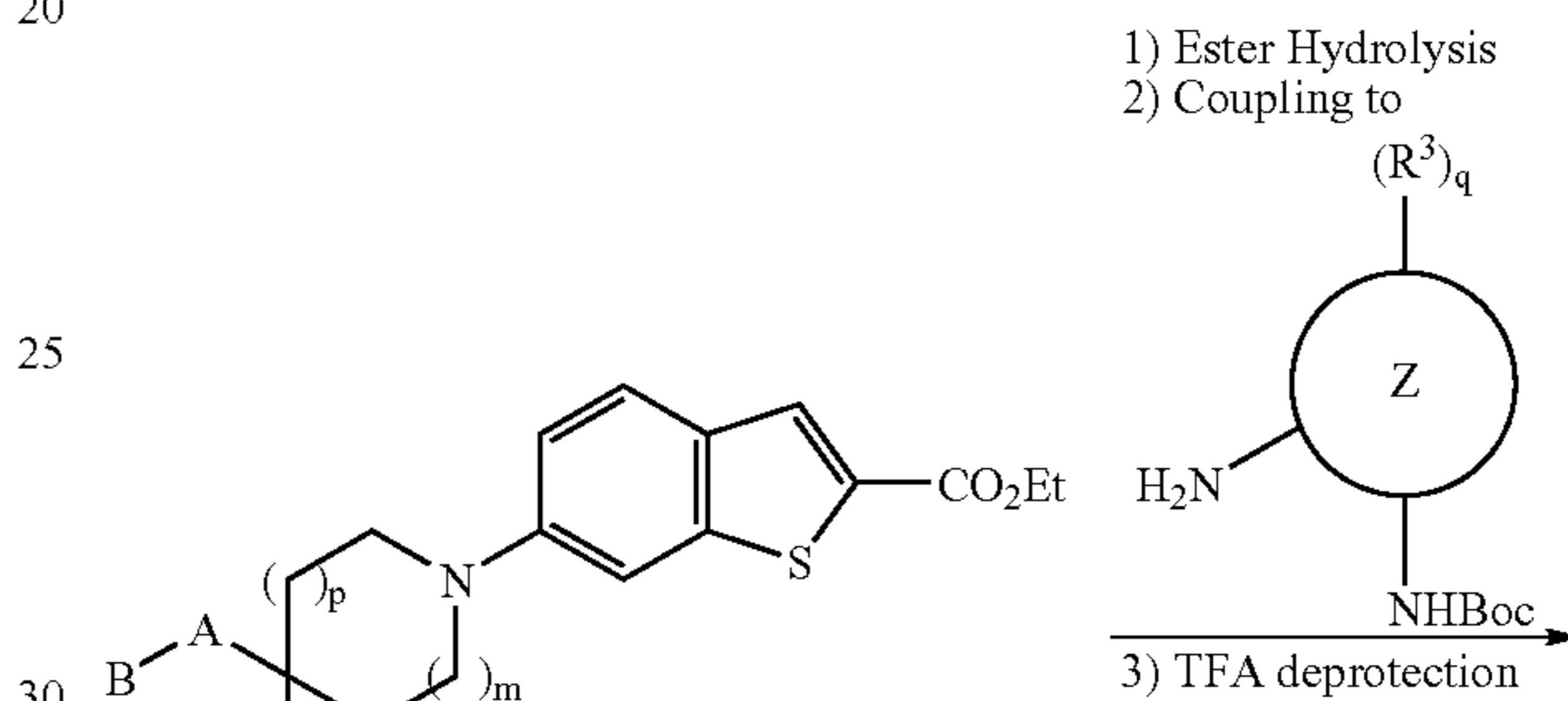
SCHEME 4
