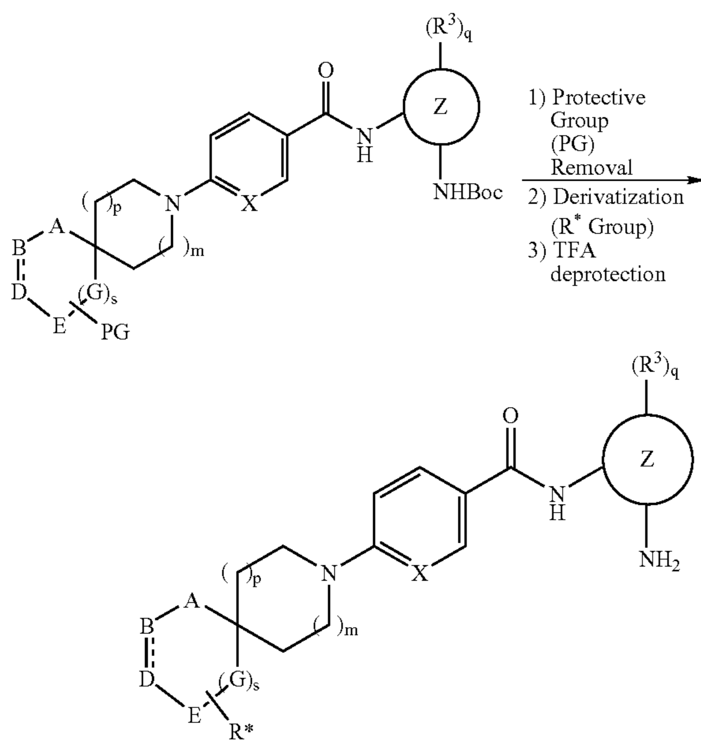
SCHEME 2
