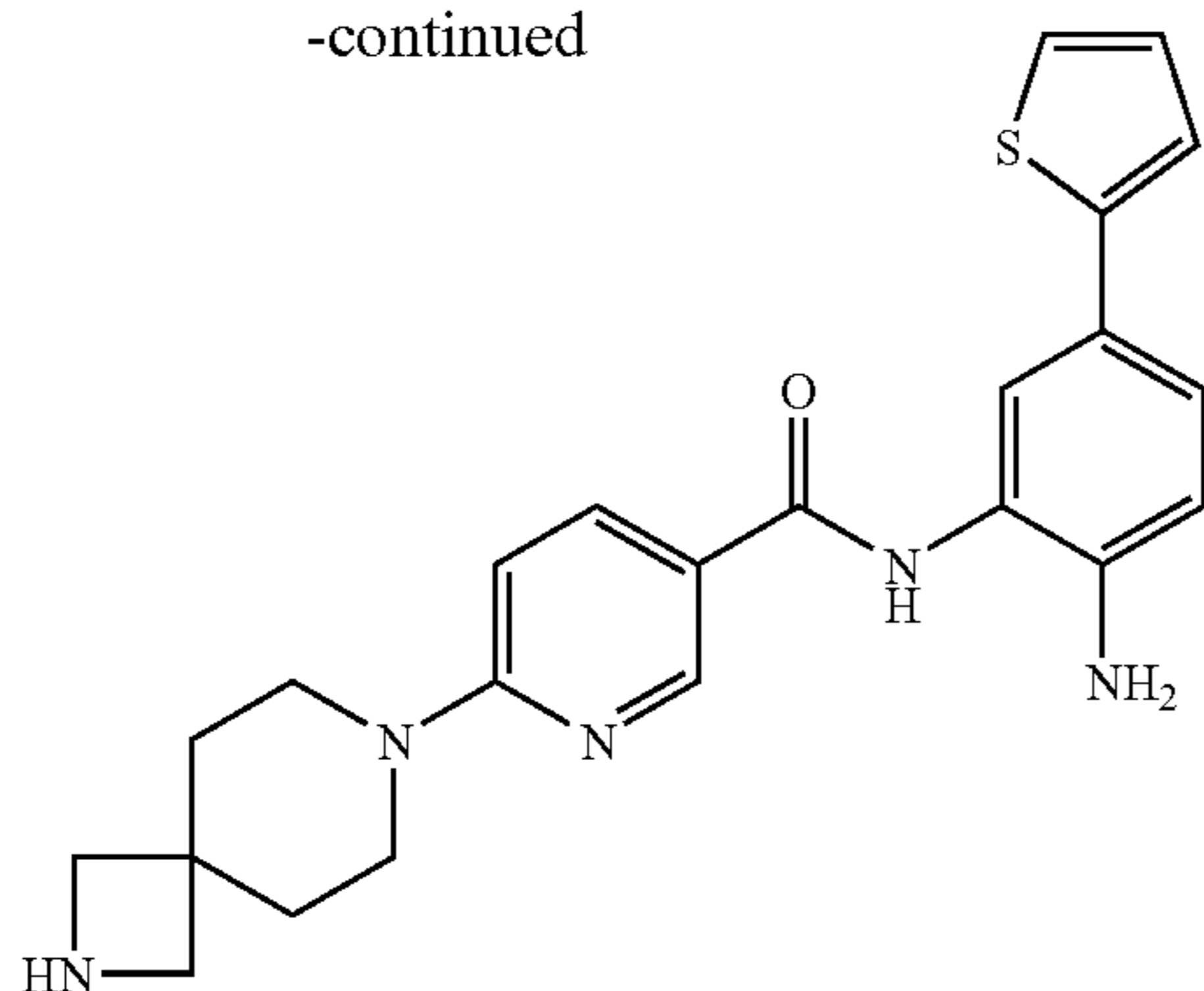
N-[2-Amino-5-(2-thienyl)phenyl]-6-(2,7-diazaspiro [3.5]non-7-yl)nicotinamide tert-Butyl [2-[[[(6-chloropyridin-3-yl)carbonyl]amino]-4-(2-thienyl)phenyl]carbamate F (20 mg, 0.088 mmol) was dis-
