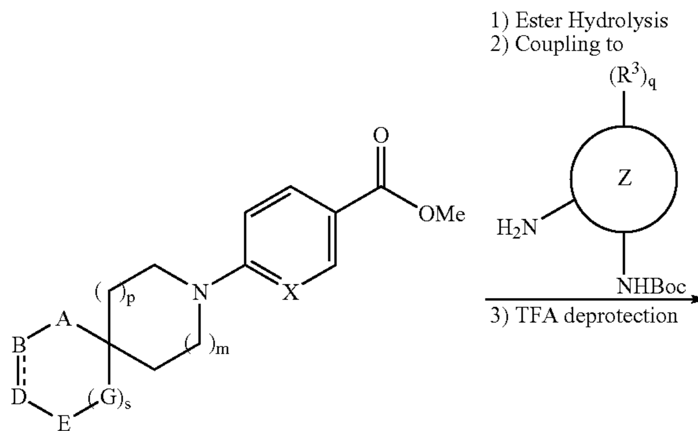
SCHEME 3
