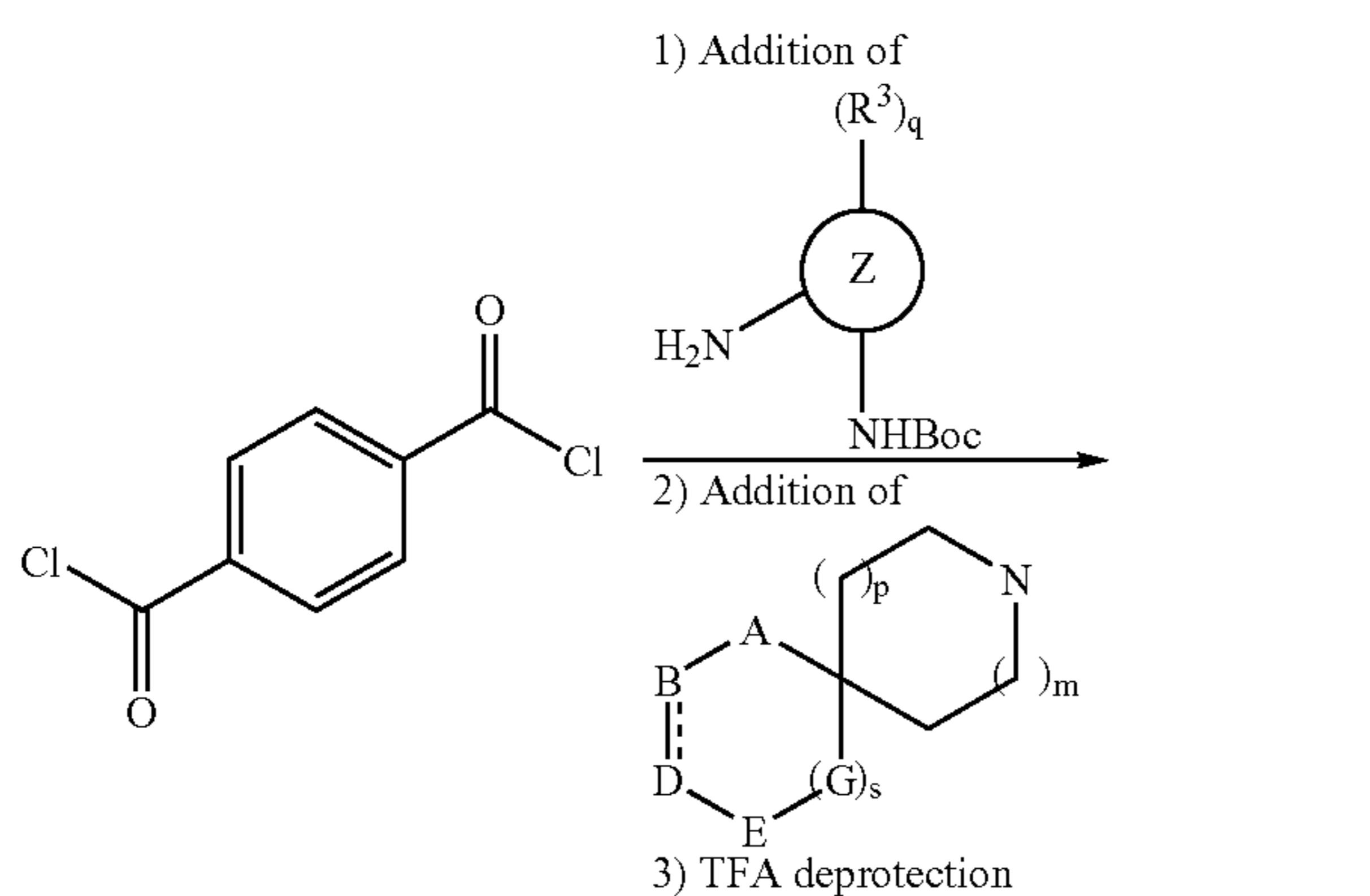
SCHEME 7
