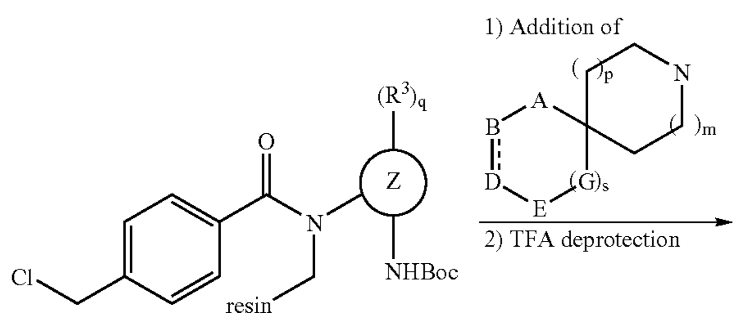
SCHEME 6
