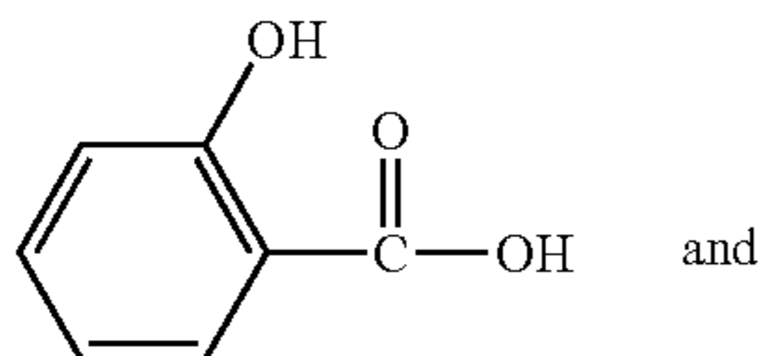
Esters of Salicylic Acid
