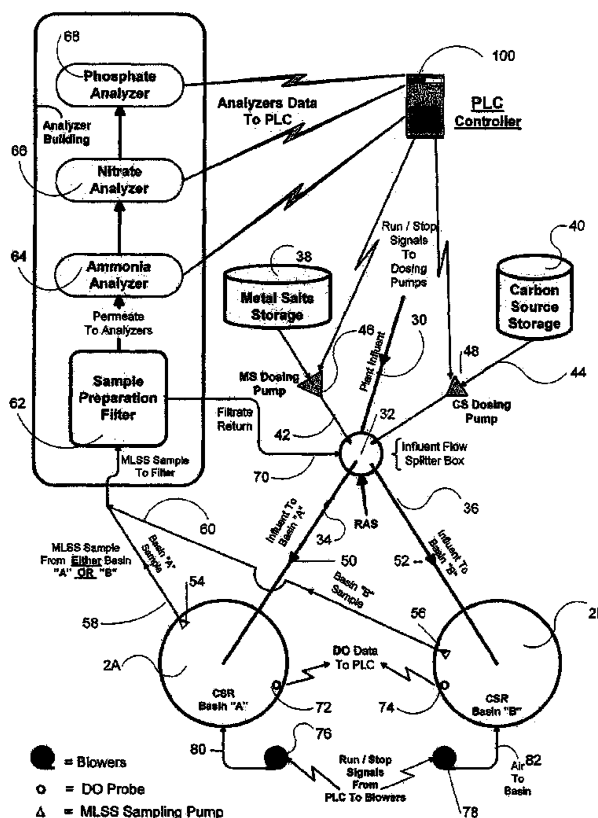
Analyzers, Additives, DO and PLC Control Systems Schematic for Primary Mode
