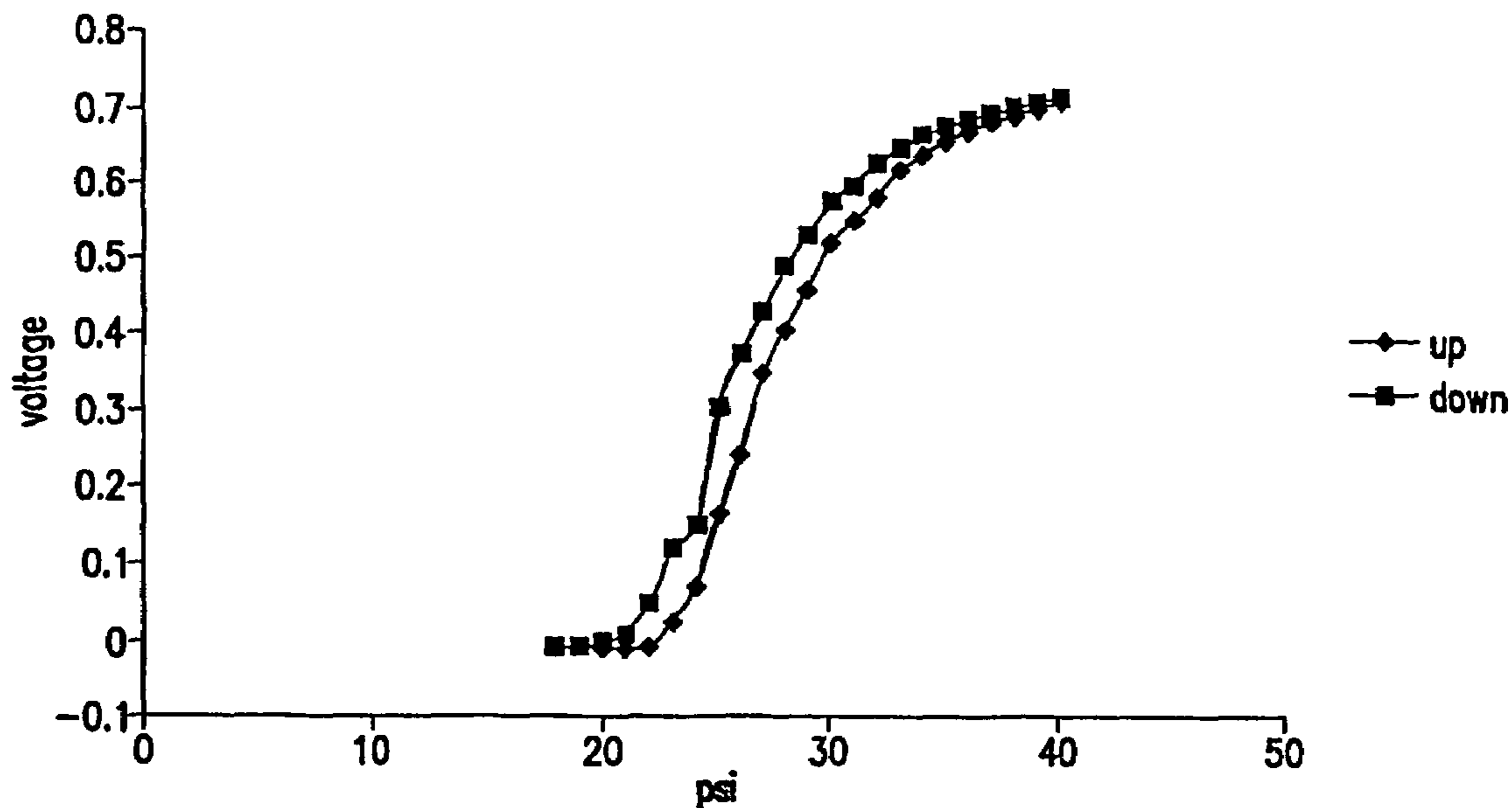
Valve Test 071901 graph B
