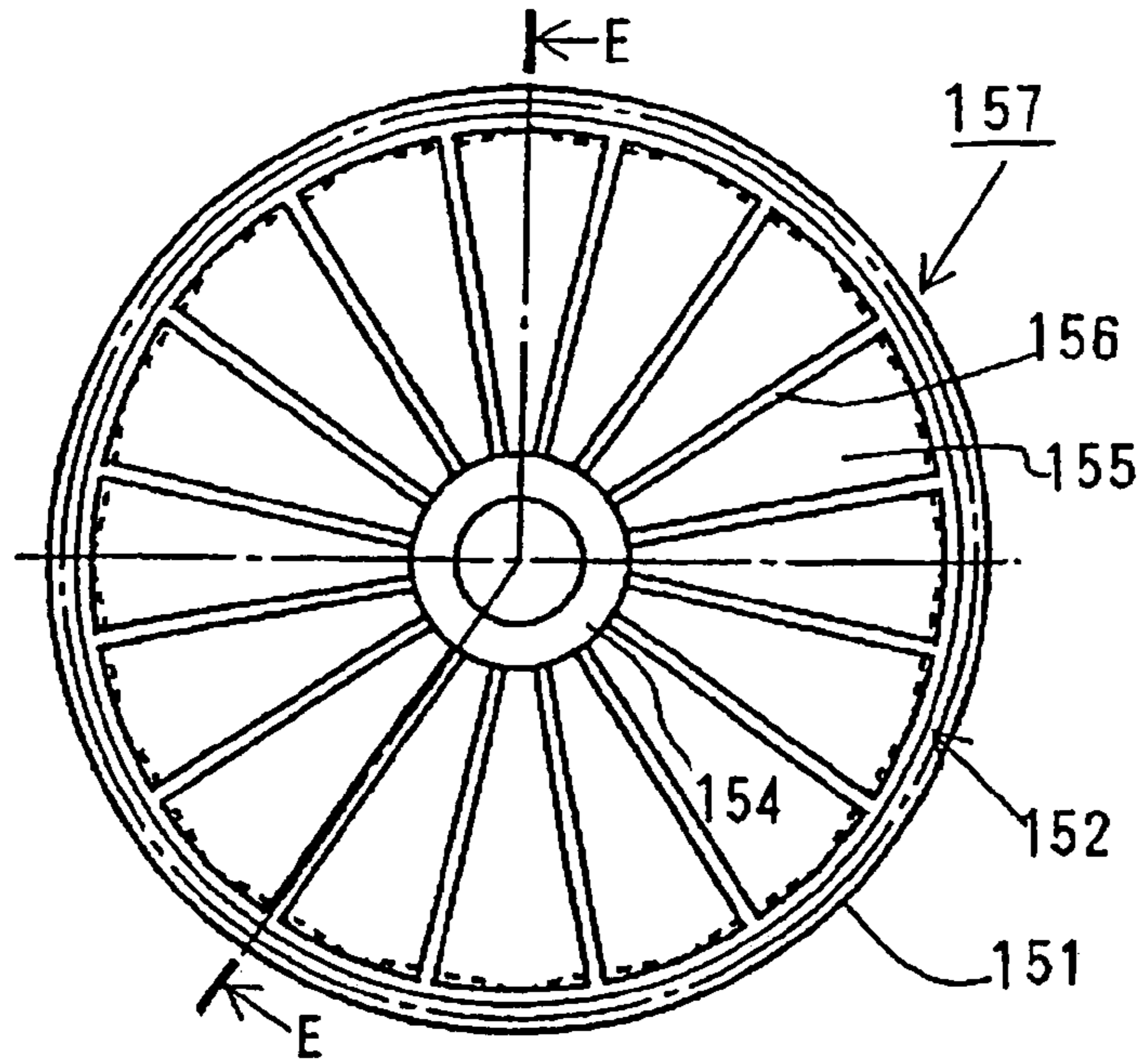
Fig. 5 PRIOR ART
