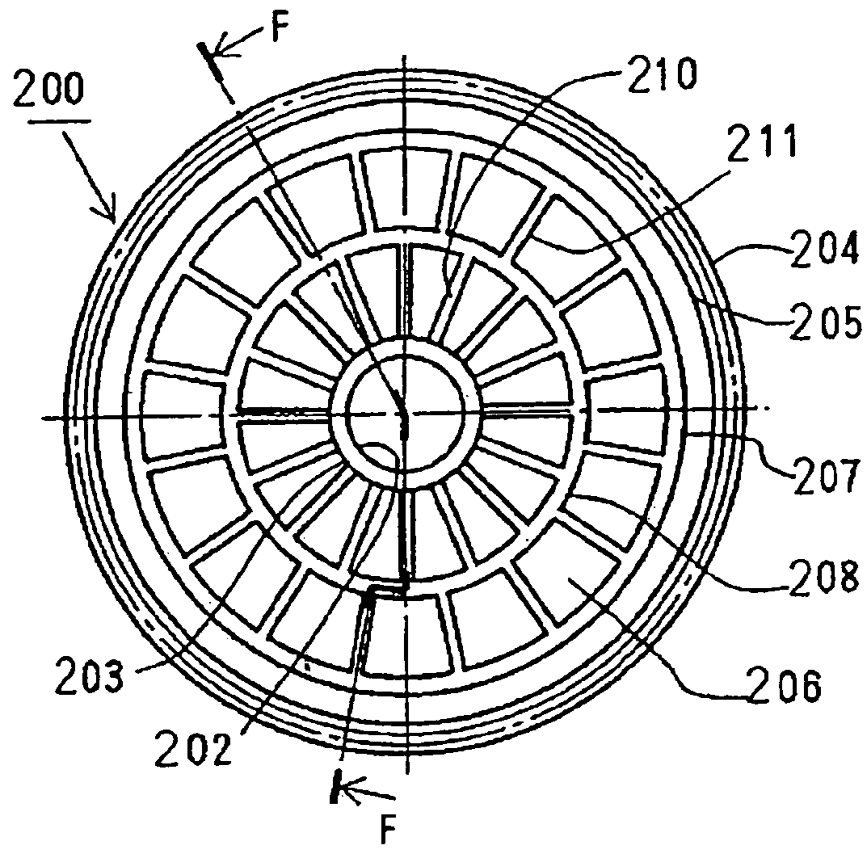
Fig. 9 PRIOR ART
