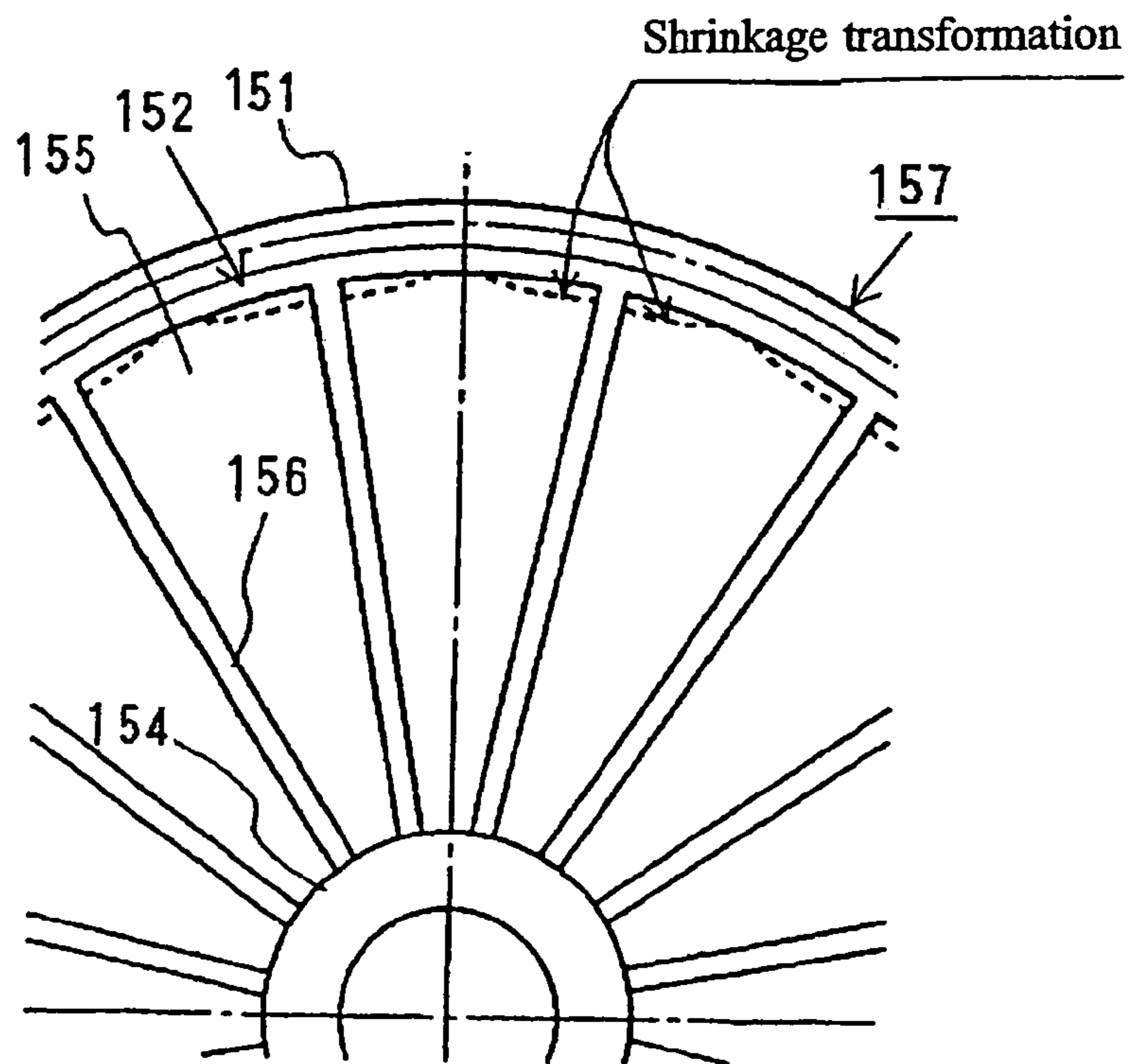
Fig. 6 PRIOR ART
