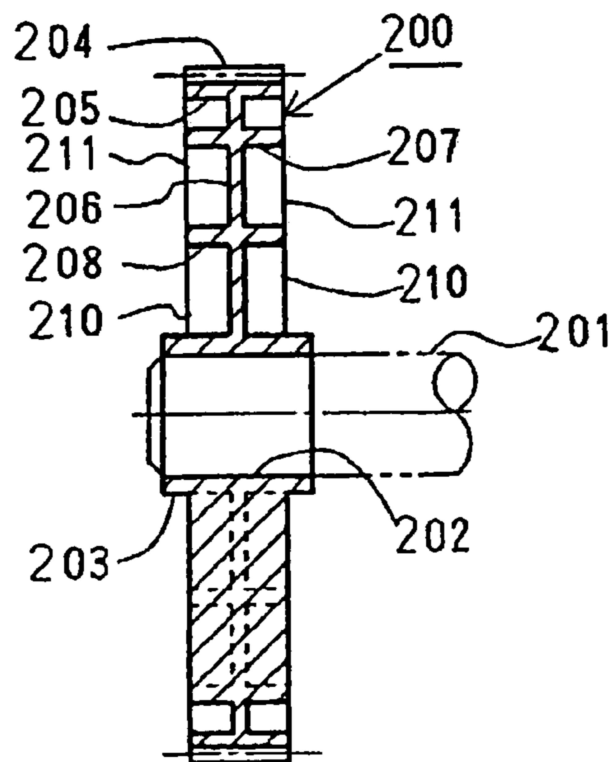
Fig. 10 PRIOR ART
