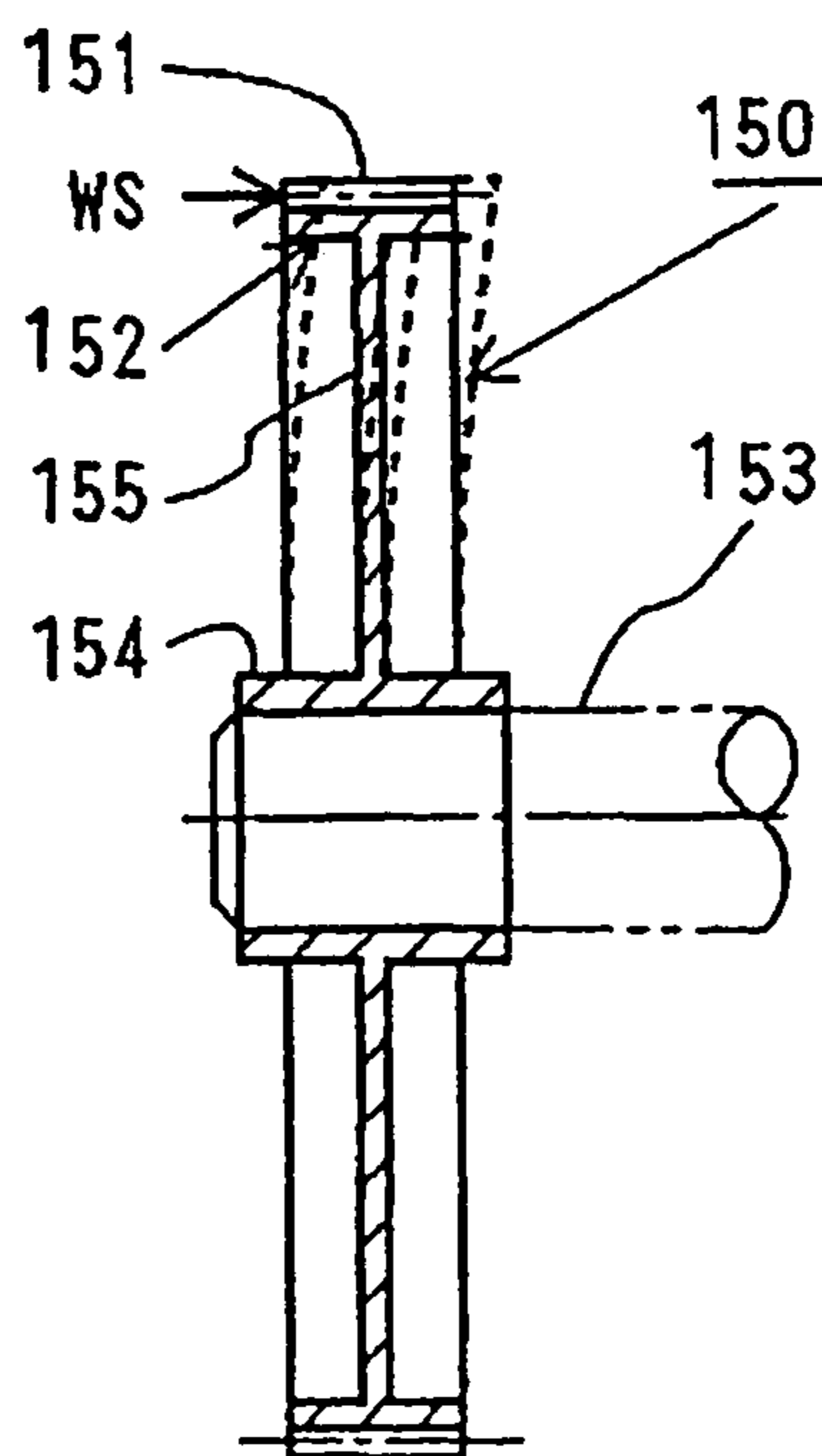
Fig. 4 PRIOR ART
