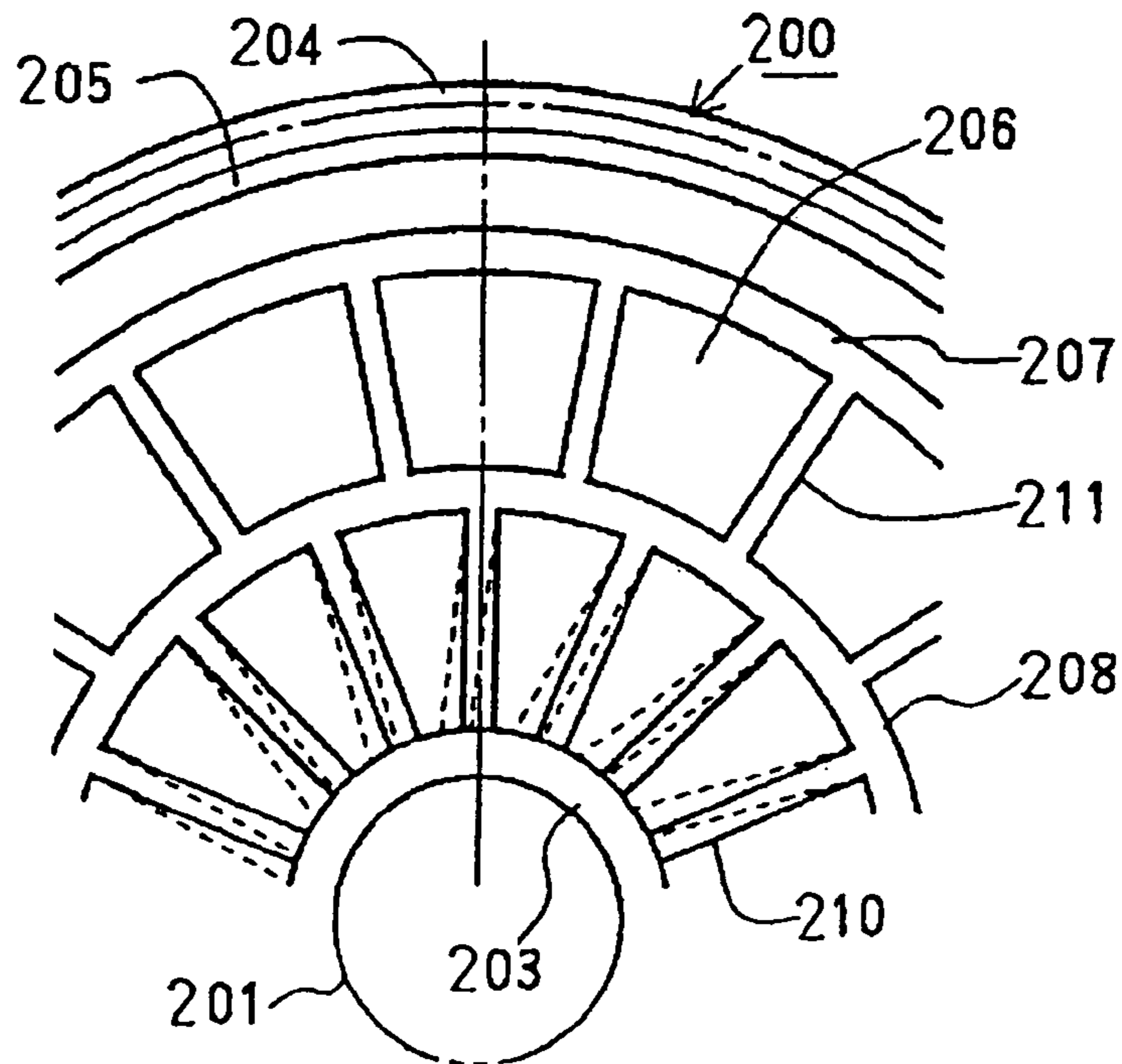
Fig. 12 PRIOR ART
