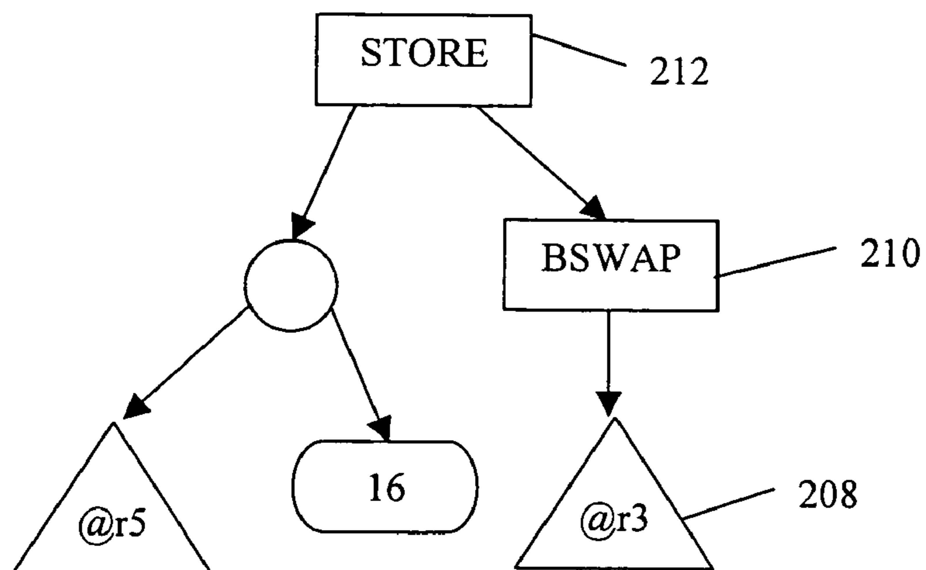
Block 2 IR Without Lazy Byteswapping
