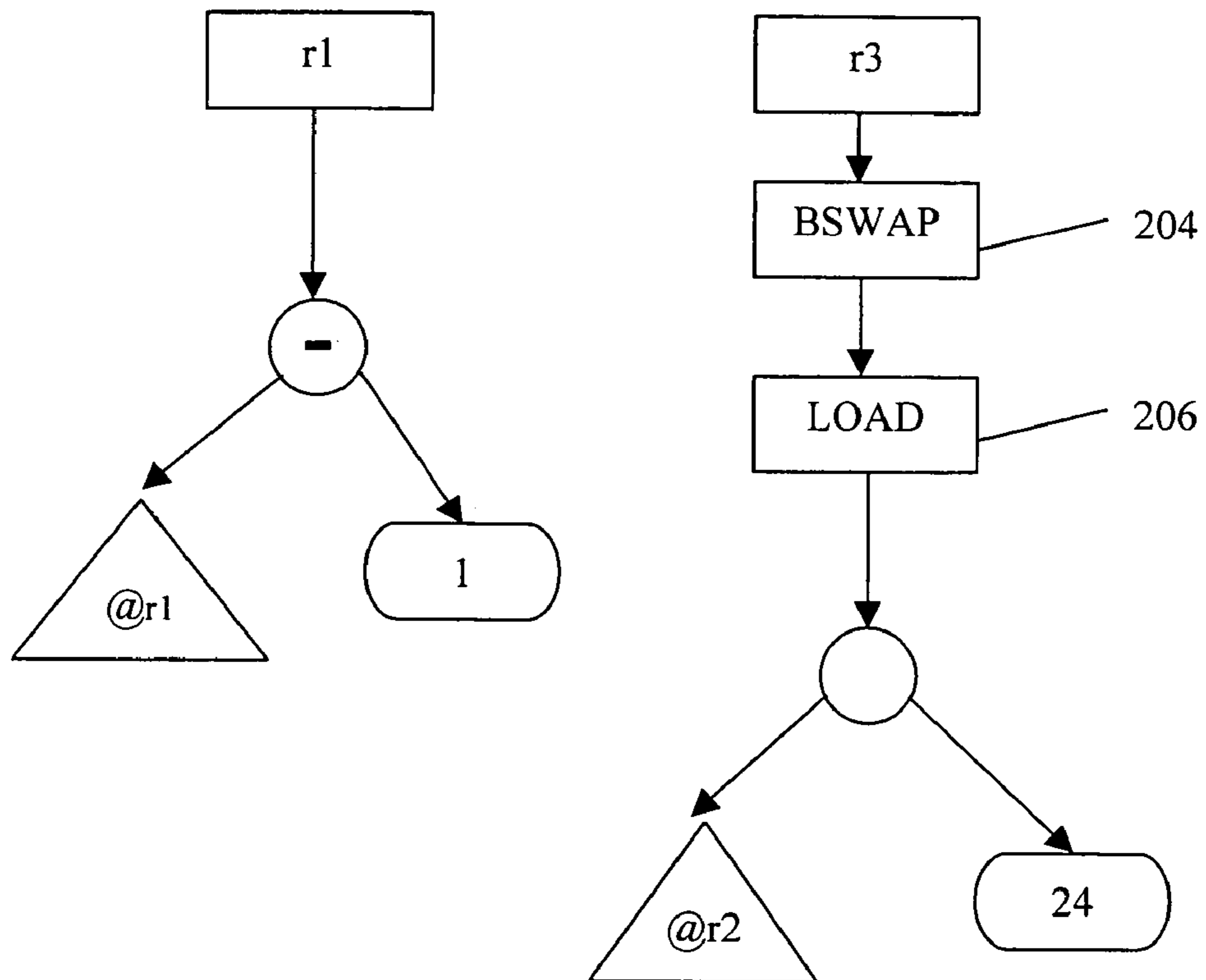
Block 1 IR Without Lazy Byteswapping
