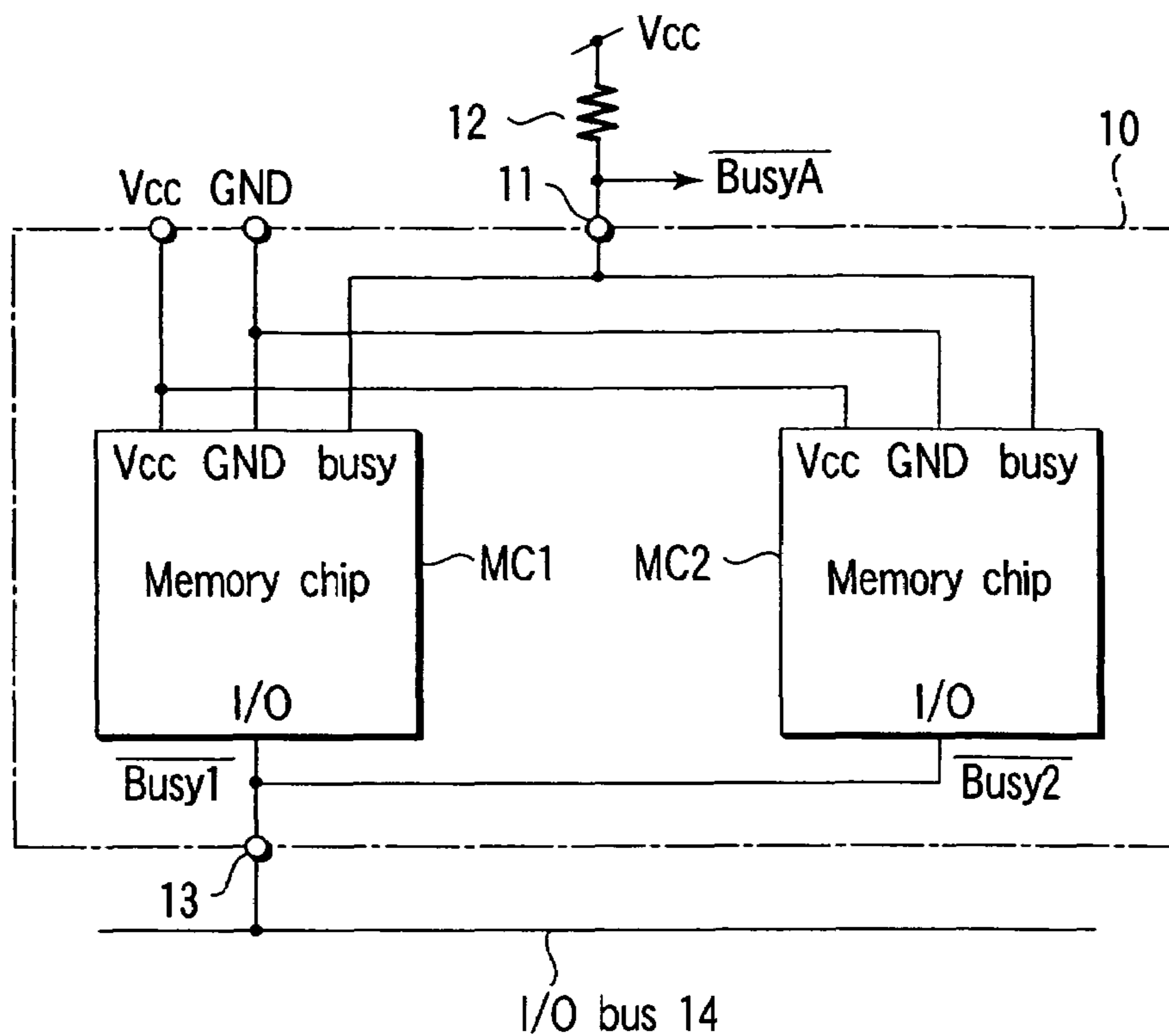
FIG. 1 PRIOR ART
