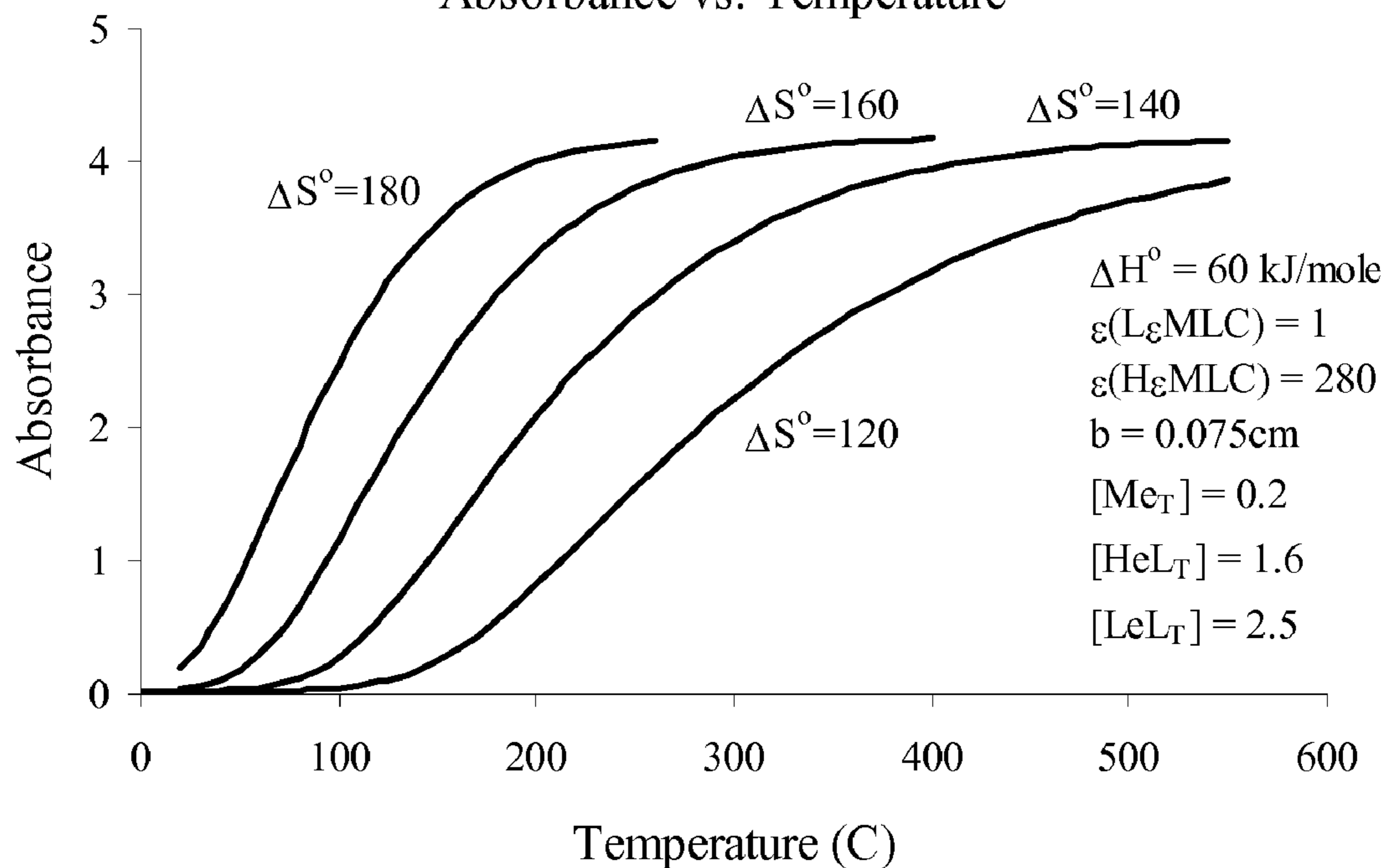
Figure 48. Influence of \Delta S^\circ on Absorbance vs. Temperature
