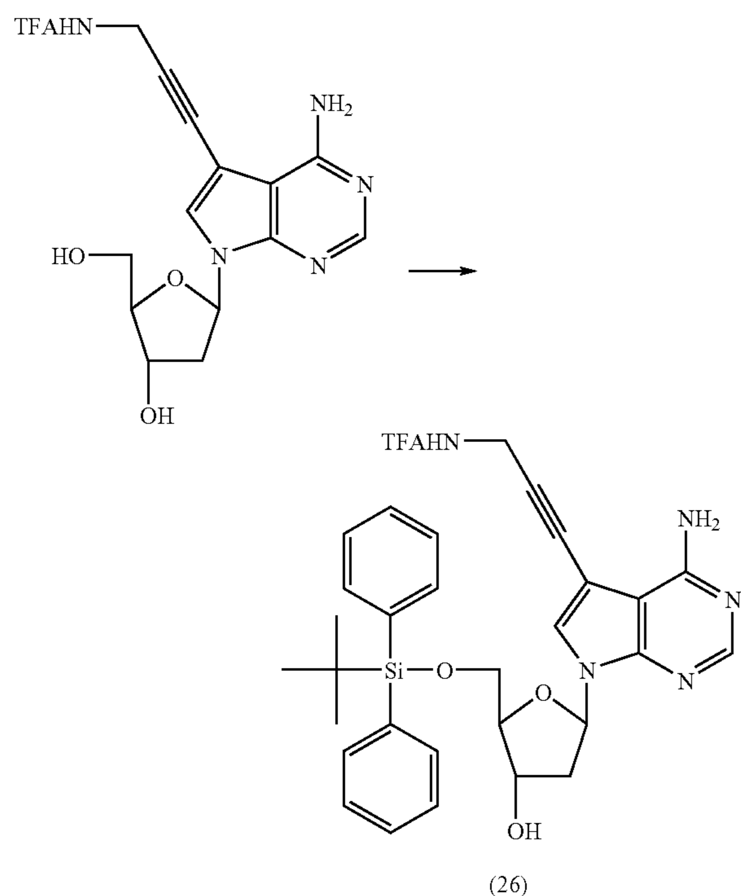
5'-O-(tert-Butyldiphenylsilyl)-7-deaza-7-[3-(2,2,2-trifluoroacetamido)-prop-1-ynyl]-2'-deoxyadenosine (26)
