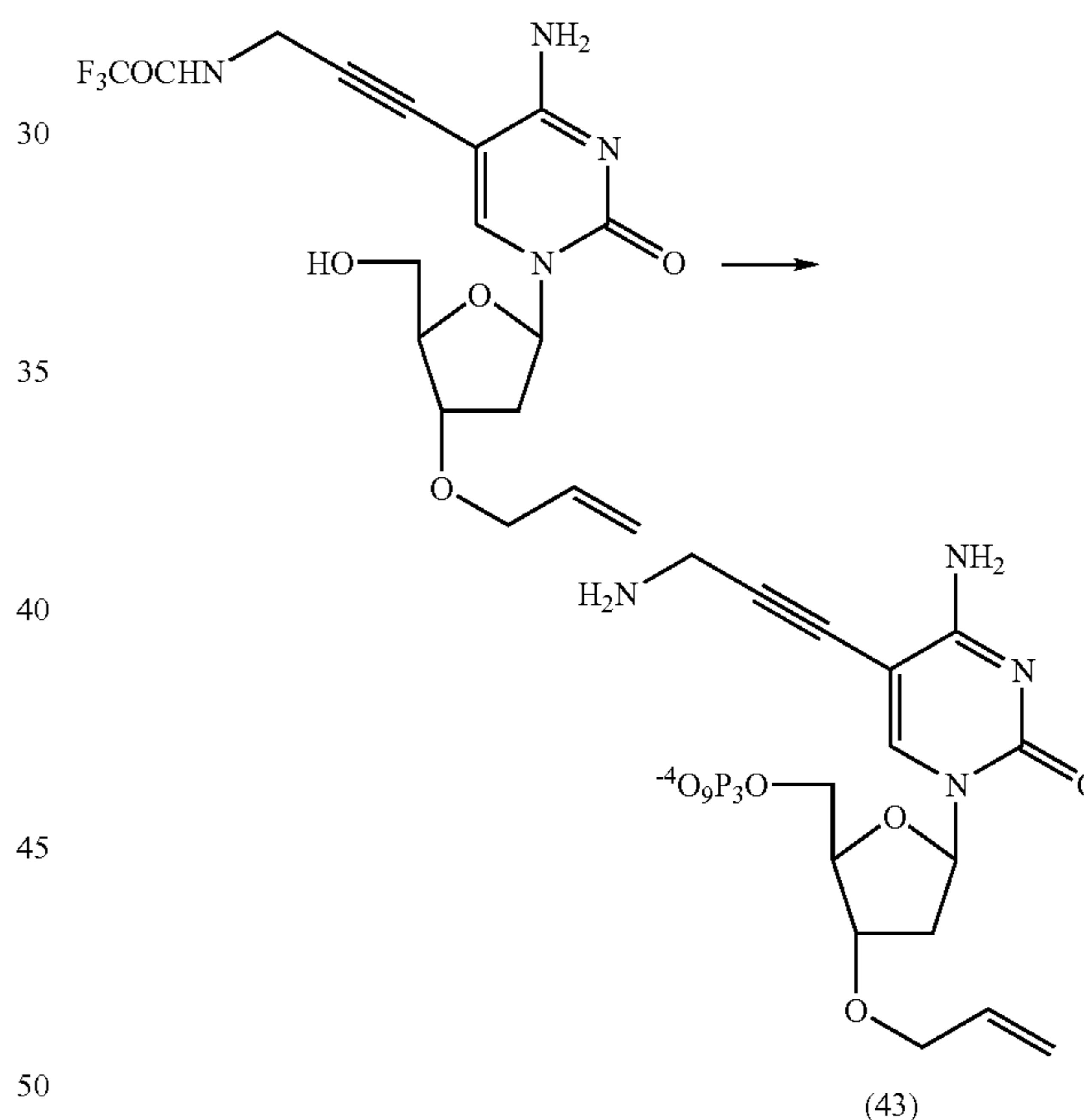
3'-O-Allyl-5-(3-amino-prop-1-ynyl)-5'-O-triphosphate-2'-deoxycytidine (43)
