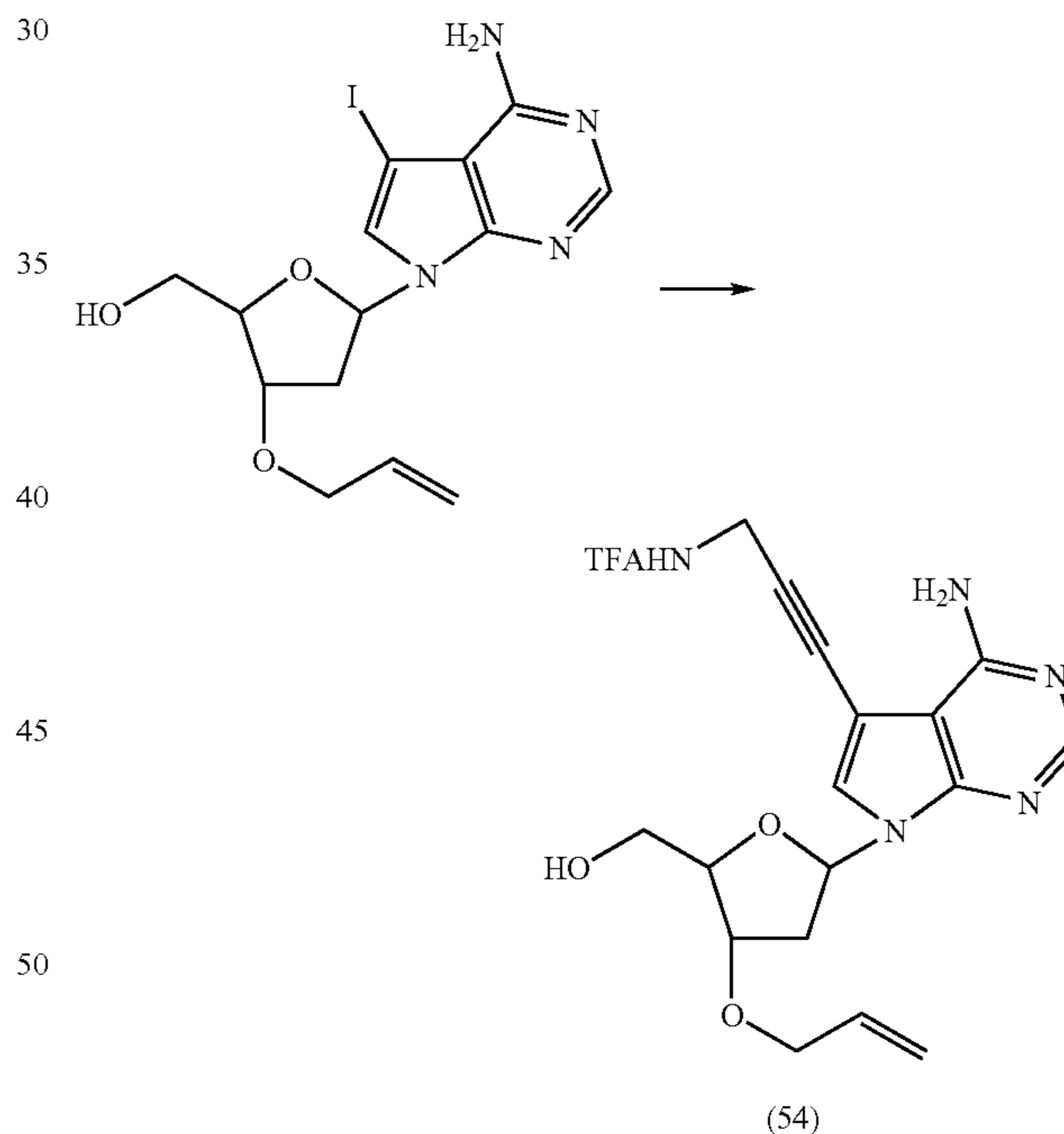
3'-O-Allyl-7-deaza-7-[3-(2,2,2-trifluoroacetamide)]-2'-deoxyadenosine (54)
