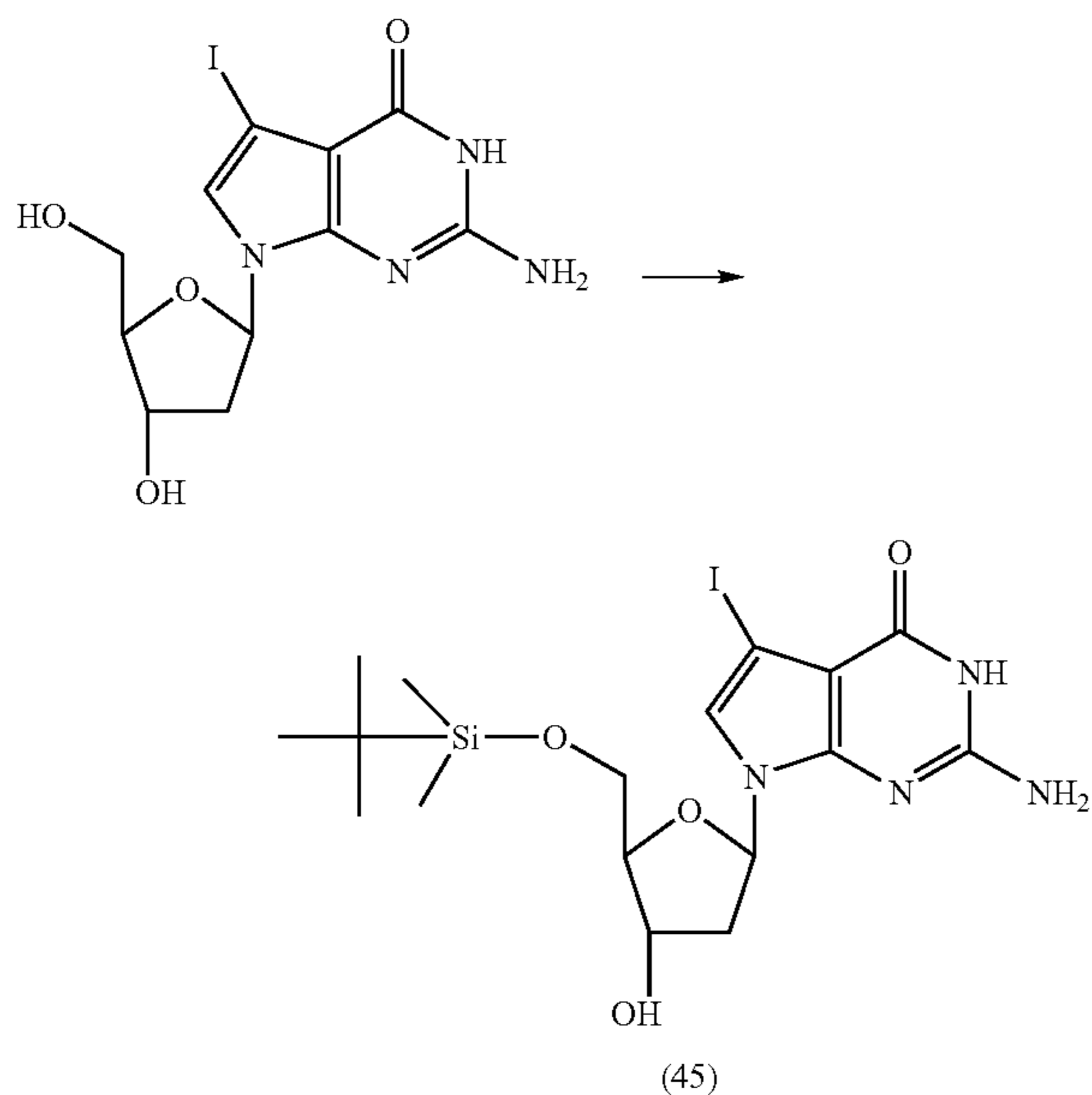
5'-O-(tert-Butyldimethylsilyl)-7-deaza-7-iodo-2'-deoxyguanosine (45)
