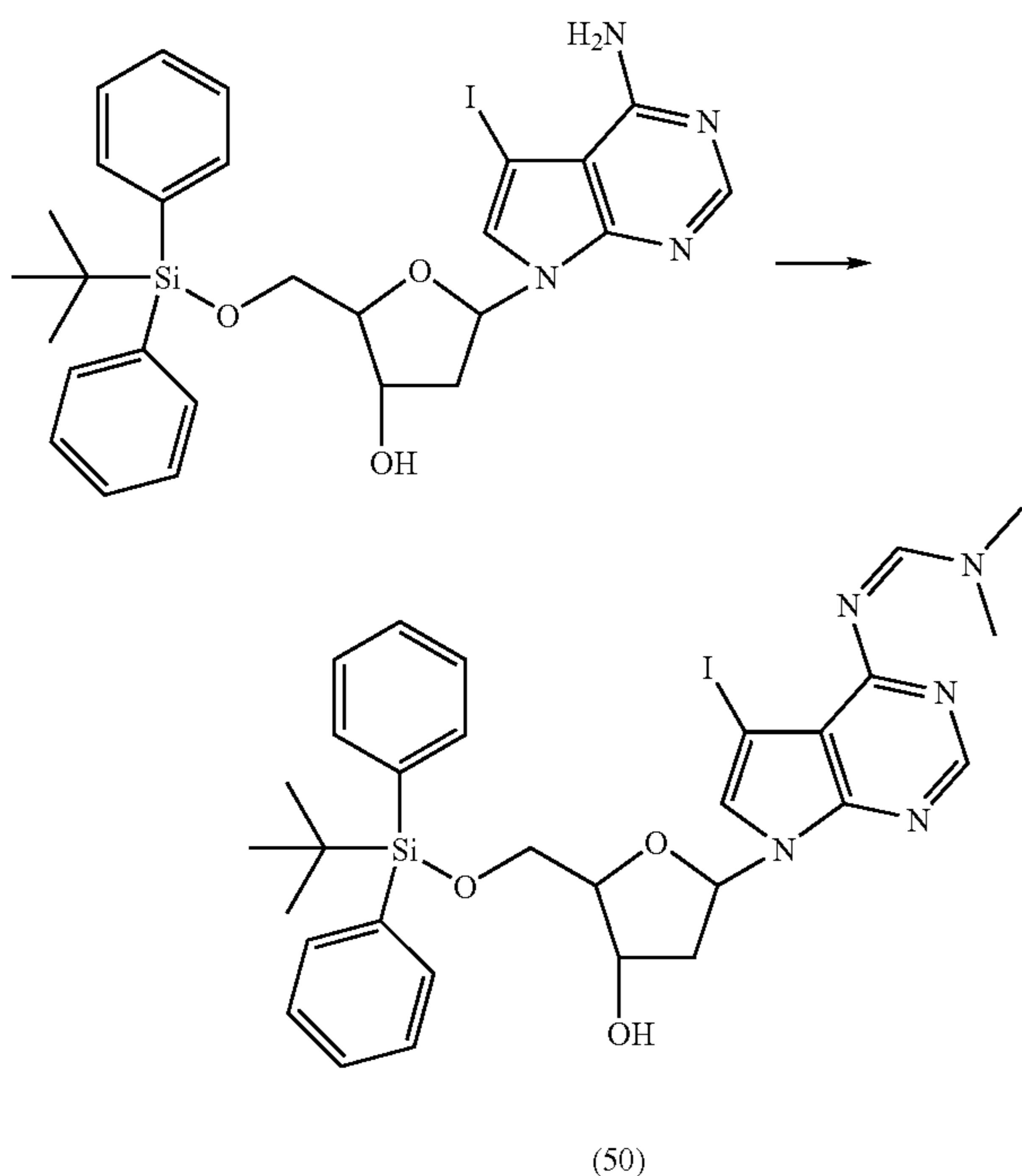
7-Deaza-6-N,N-dimethylformadine-5'-O-diphenylsilyl-7-iodo-2'-deoxyadenosine (50)
