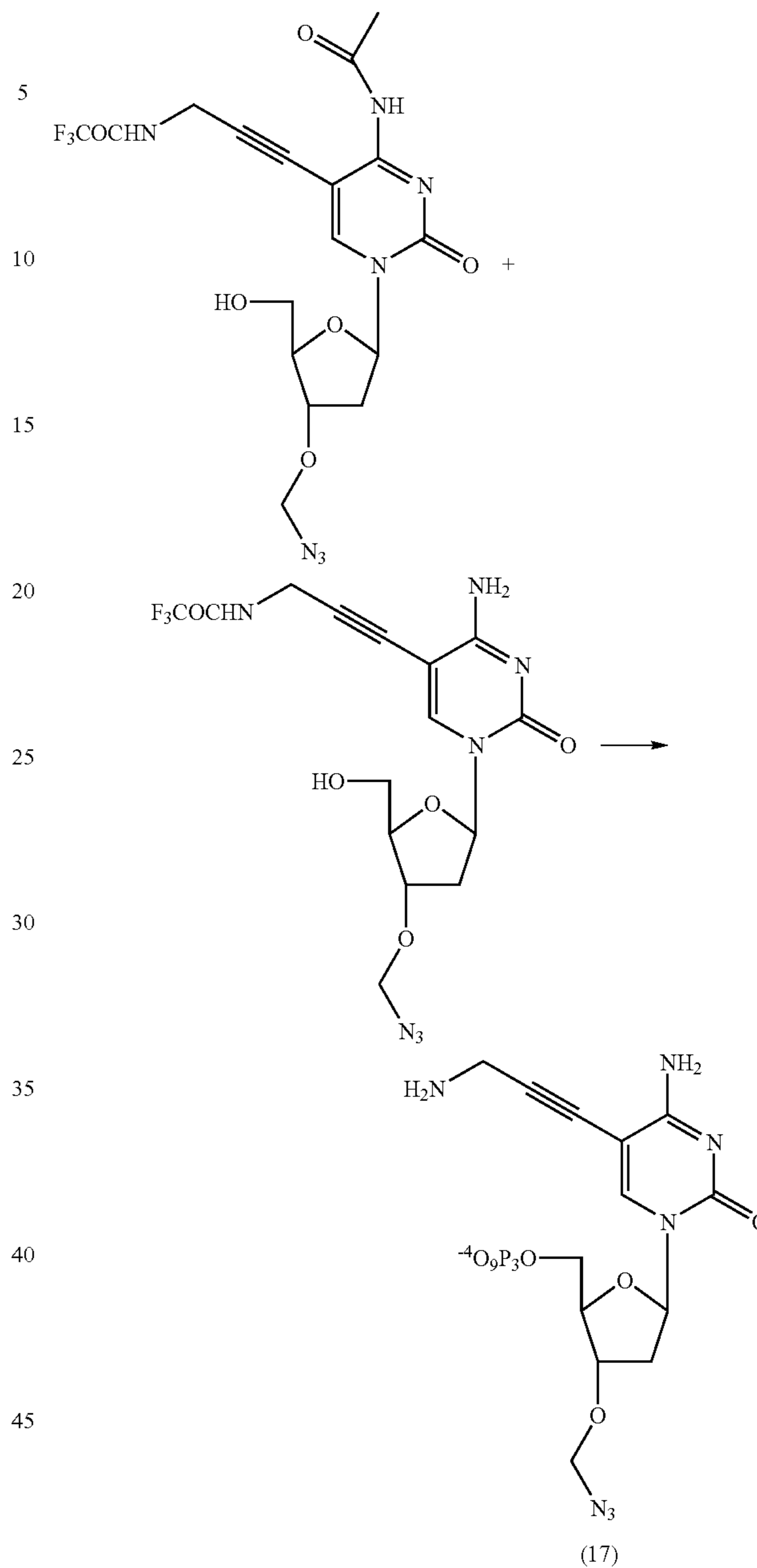
5-(3-Amino-prop-1-ynyl)-3'-O-azidomethyl-2'-deoxycytidine 5'-O-nucleoside triphosphate (17)
