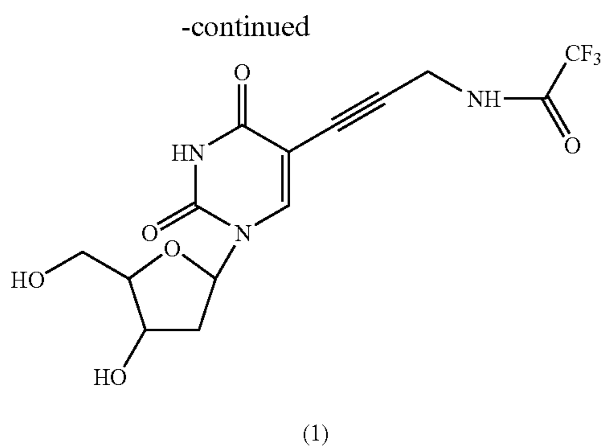
5-[3-(2,2,2-trifluoroacetamido)-prop-1-ynyl]-2'-deoxyuridine (1)
