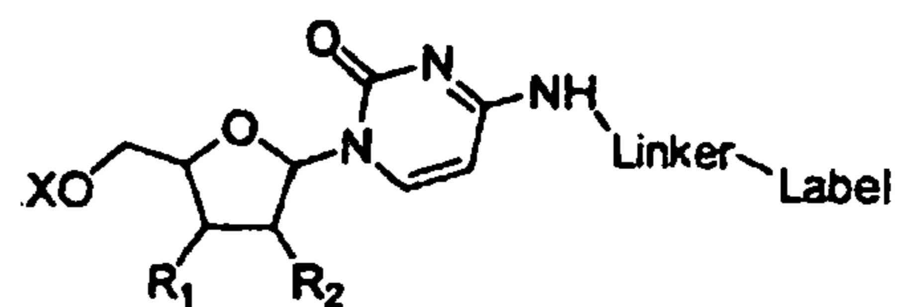
Cytidine N4-linker
