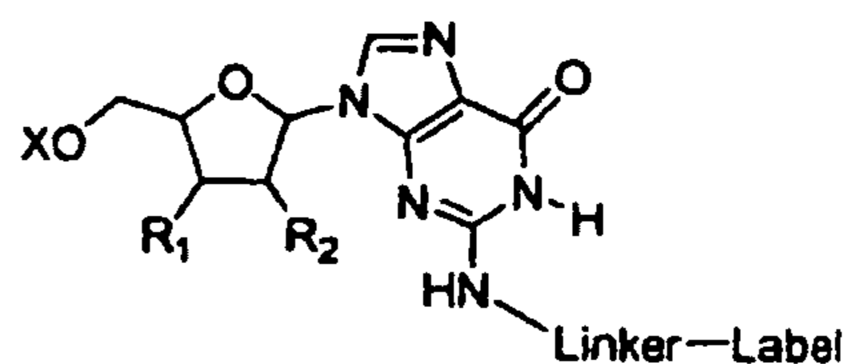
Guanosine N2-linker
