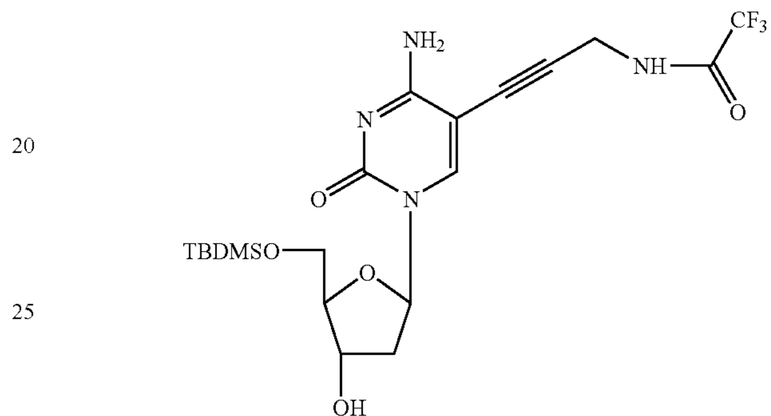
5'-O-(tert-Butyldimethylsilyl)-5-[3-(2,2,2-trifluoroacetamido)-prop-1-ynyl]-2'-deoxycytidine (8)
