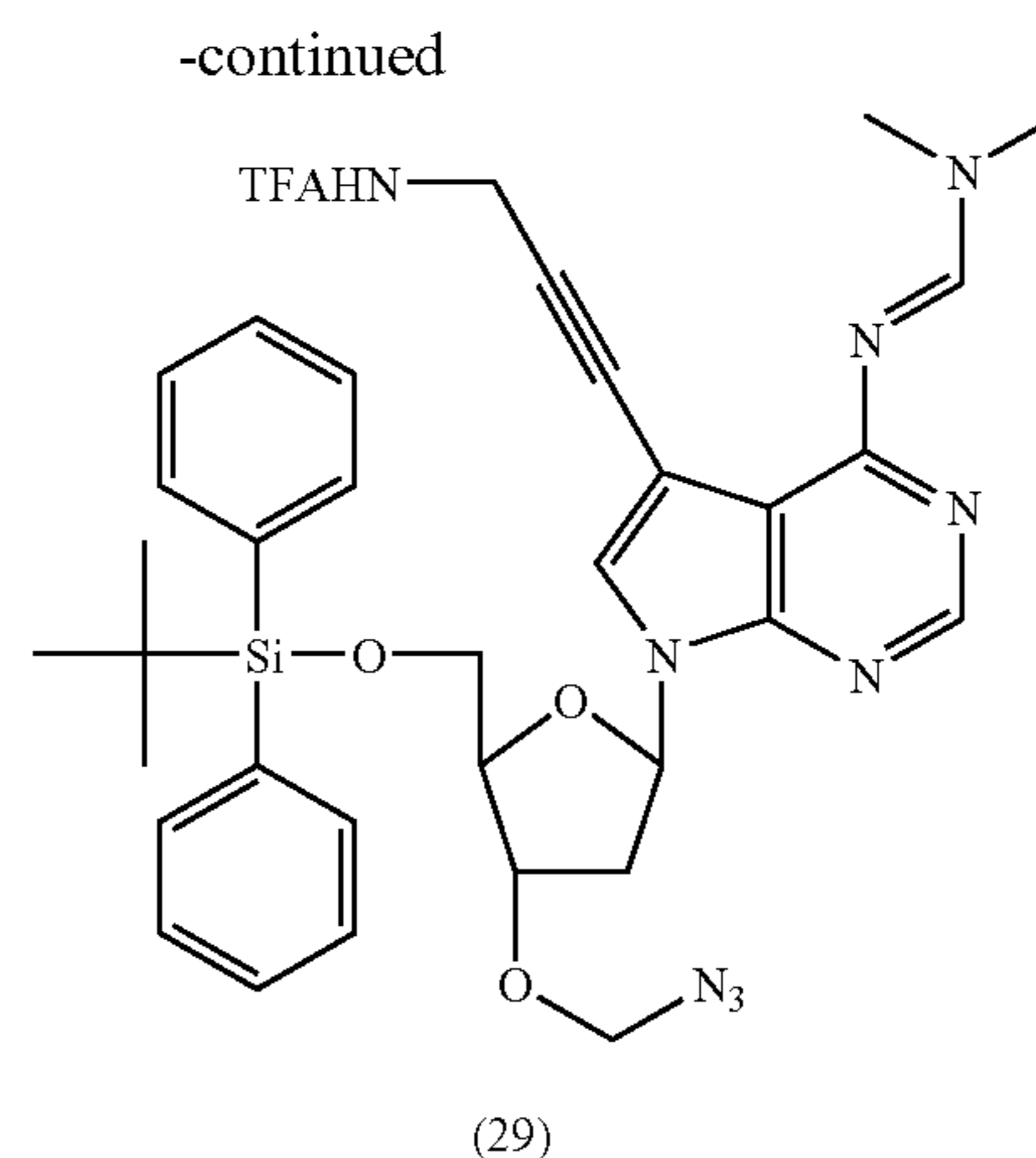
3'-O-Azidomethyl-5'-O-(tert-butyl-diphenylsilyl)-7-deaza-4-N,N-dimethylformadin-7-[3-(2,2,2-trifluoroacetamido)-prop-1-ynyl]-2'-deoxyadenosine (29)
