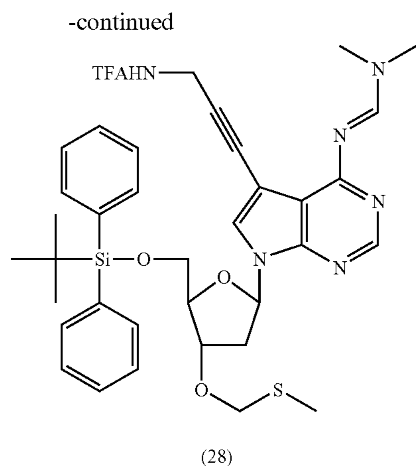
5'-O-(tert-Butyldiphenylsilyl)-7-deaza-4-N,N-dimethylformadin-3'-O-methylthiomethoxy-7-[3-(2,2,2-trifluoroacetamido)-prop-1-ynyl]-2'-deoxyadenosine (28)
