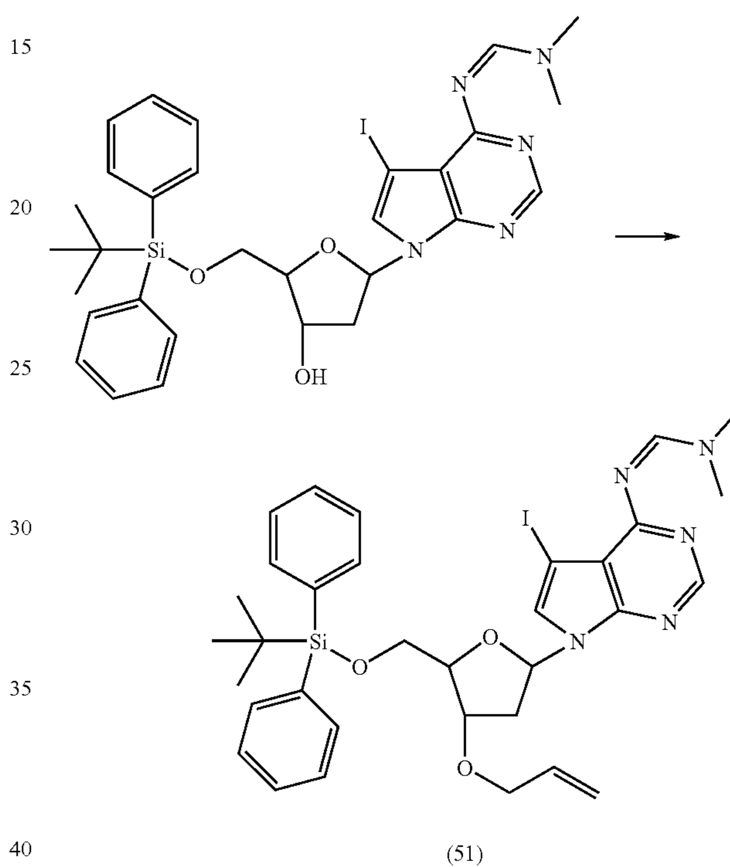
3'-O-Allyl-7-deaza-6-N,N-dimethylformadine-5'-O-diphenylsilyl-7-iodo-2'-deoxyadenosine (51)
