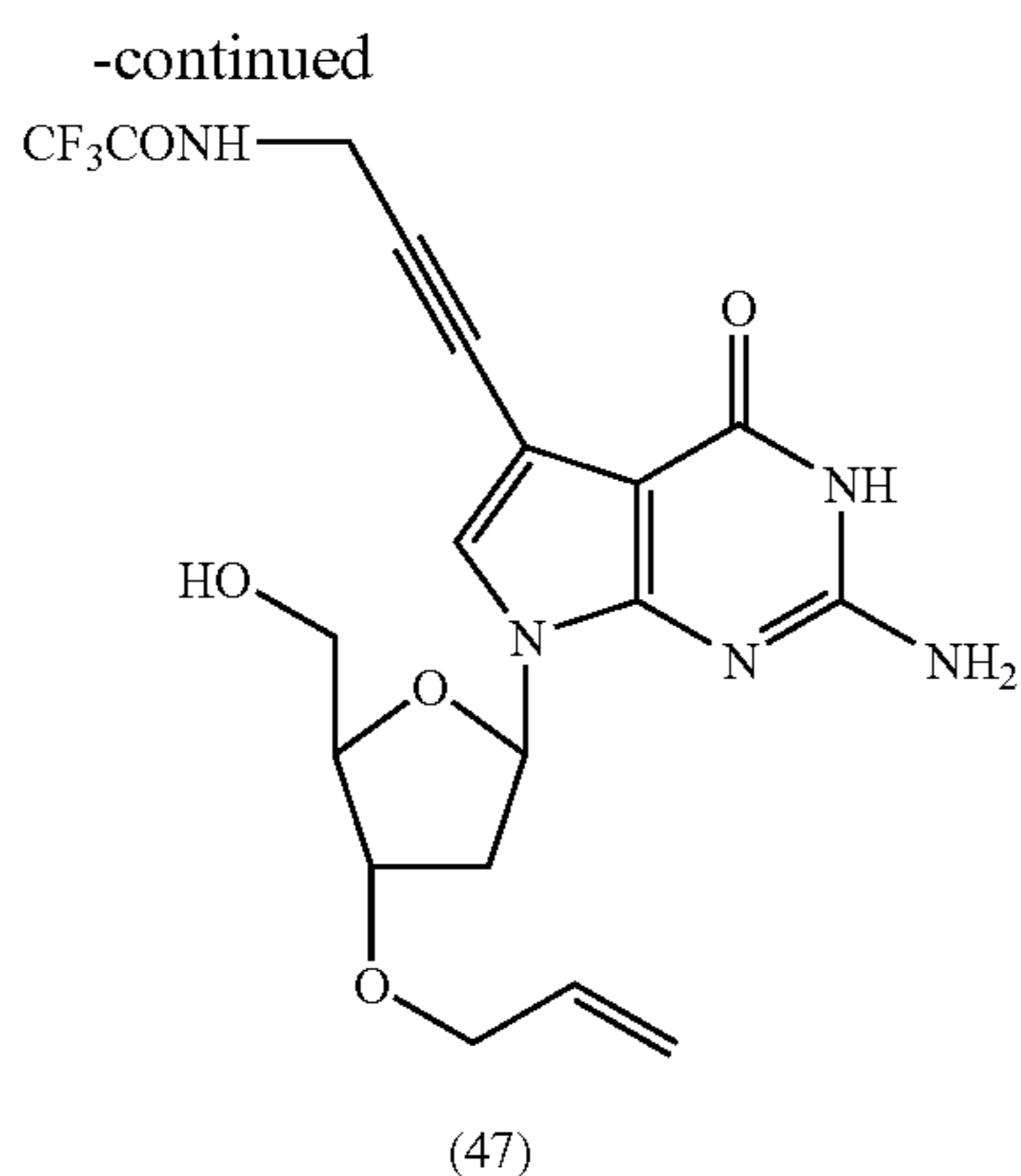
3'-O-Allyl-5'-O-(tert-butyl-dimethylsilyl)-7-deaza-7-[3-(2,2,2-trifluoroacetamido)-prop-1-ynyl]-2'-deoxyguanosine (47)
