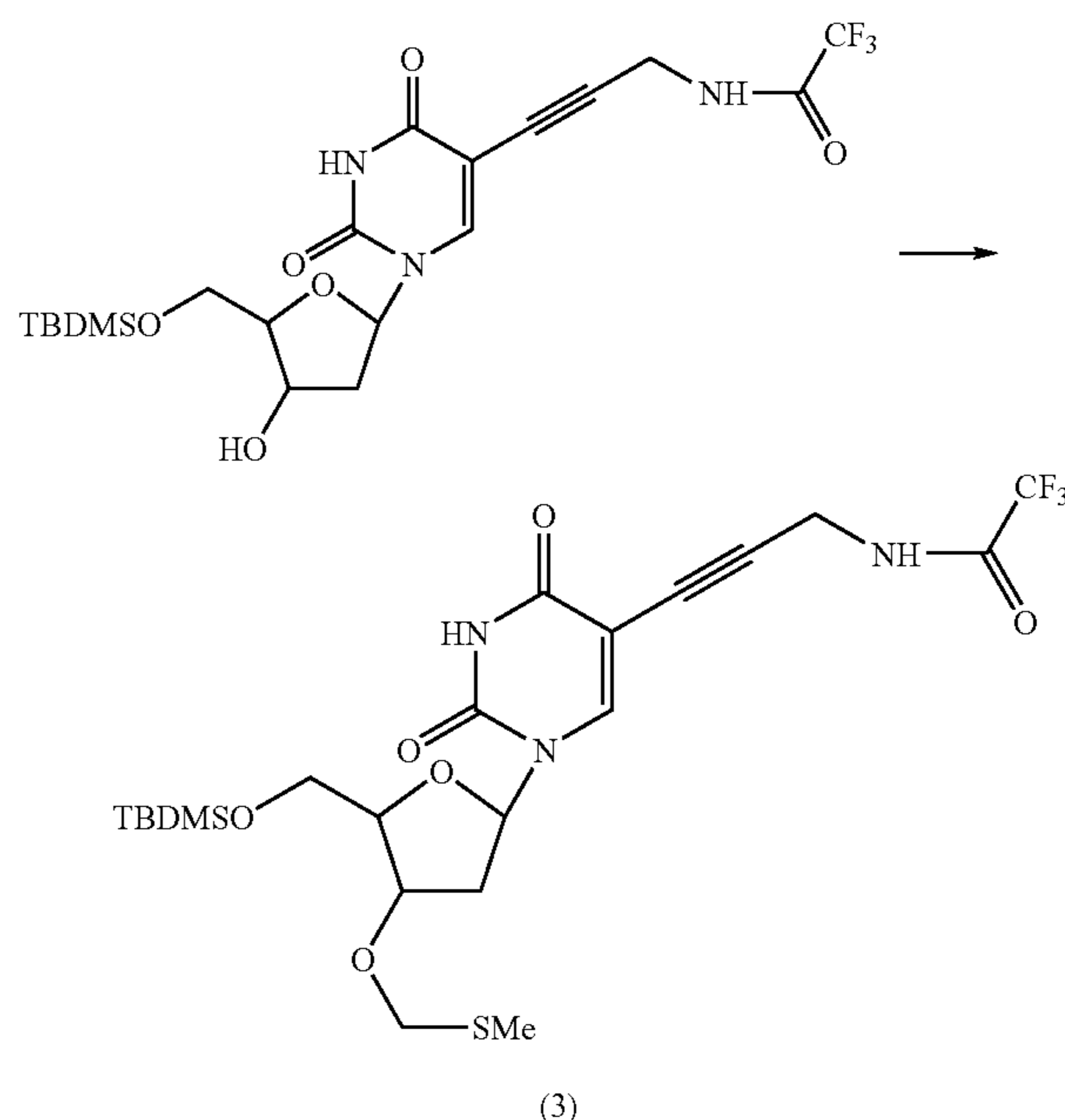
5'-O-(tert-Butyl dimethylsilyl)-3'-O-methylthiomethyl-5-[3-(2,2,2-trifluoroacetamido)-prop-1-ynyl]-2'-deoxyuridine (3)
