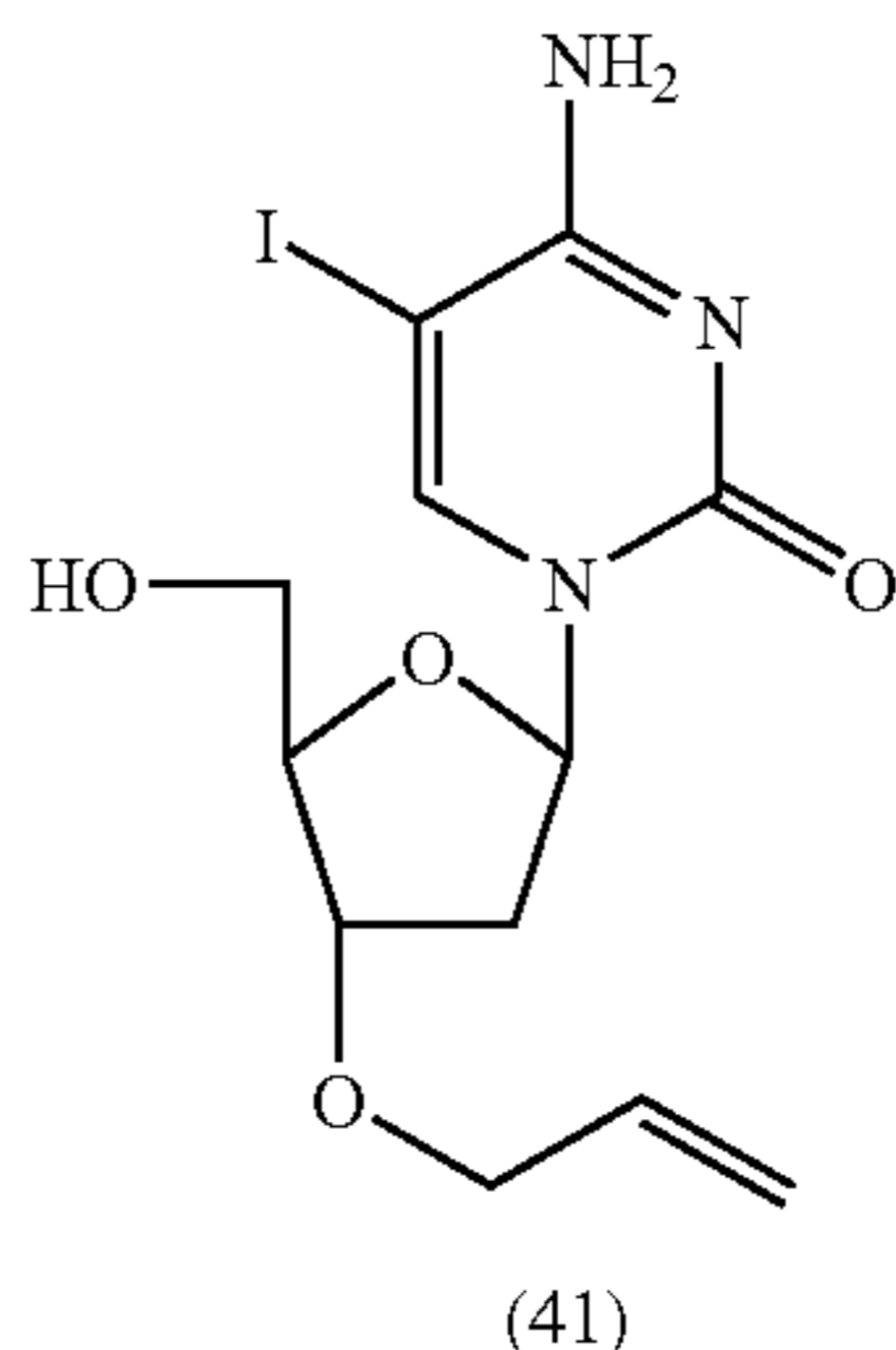
3'-O-Allyl-5-iodo-2'-deoxycytidine (41)
