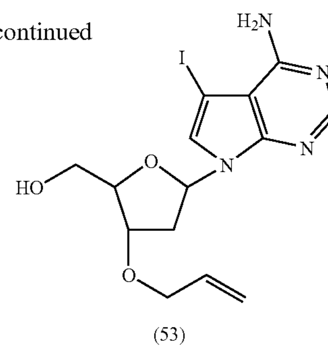
3'-O-Allyl-7-deaza-7-iodo-2'-deoxyadenosine (53)
