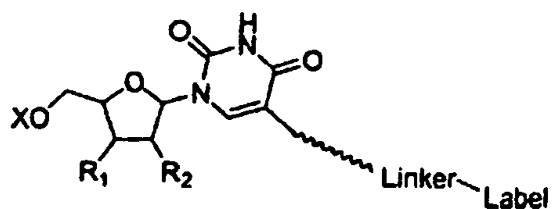
Uridine C5-linker
