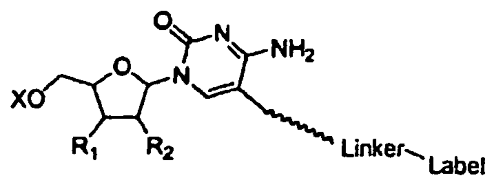
Cytidine C5-linker
