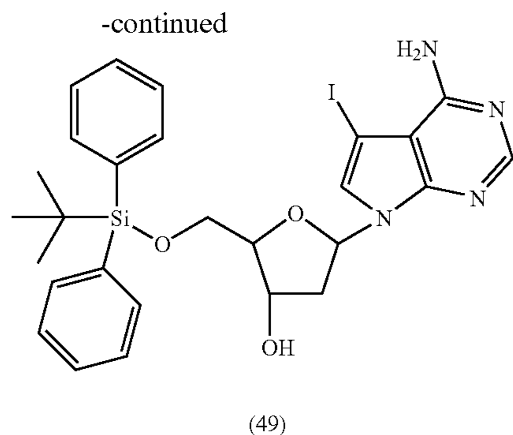
7-Deaza-5'-O-diphenylsilyl-7-iodo-2'-deoxyadenosine (49)
