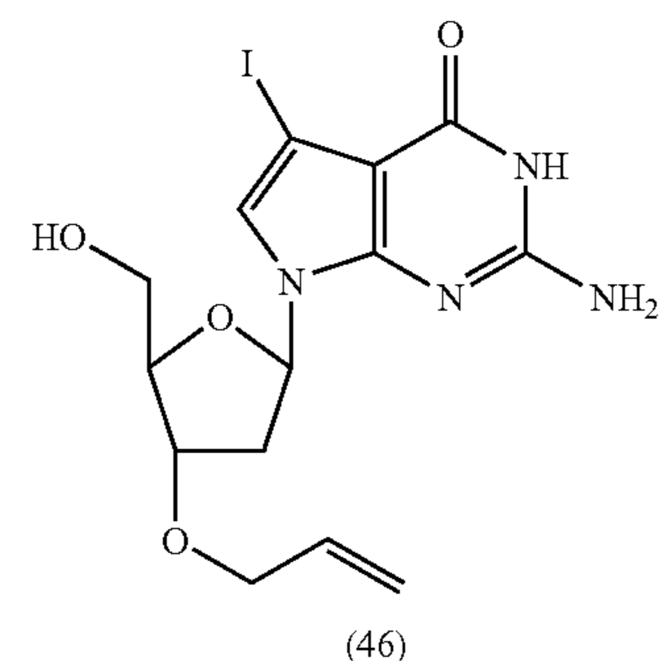
3'-O-Allyl-5'-O-(tert-butyltrimethylsilyl)-7-deaza-7-iodo-2'-deoxyguanosine (46)
