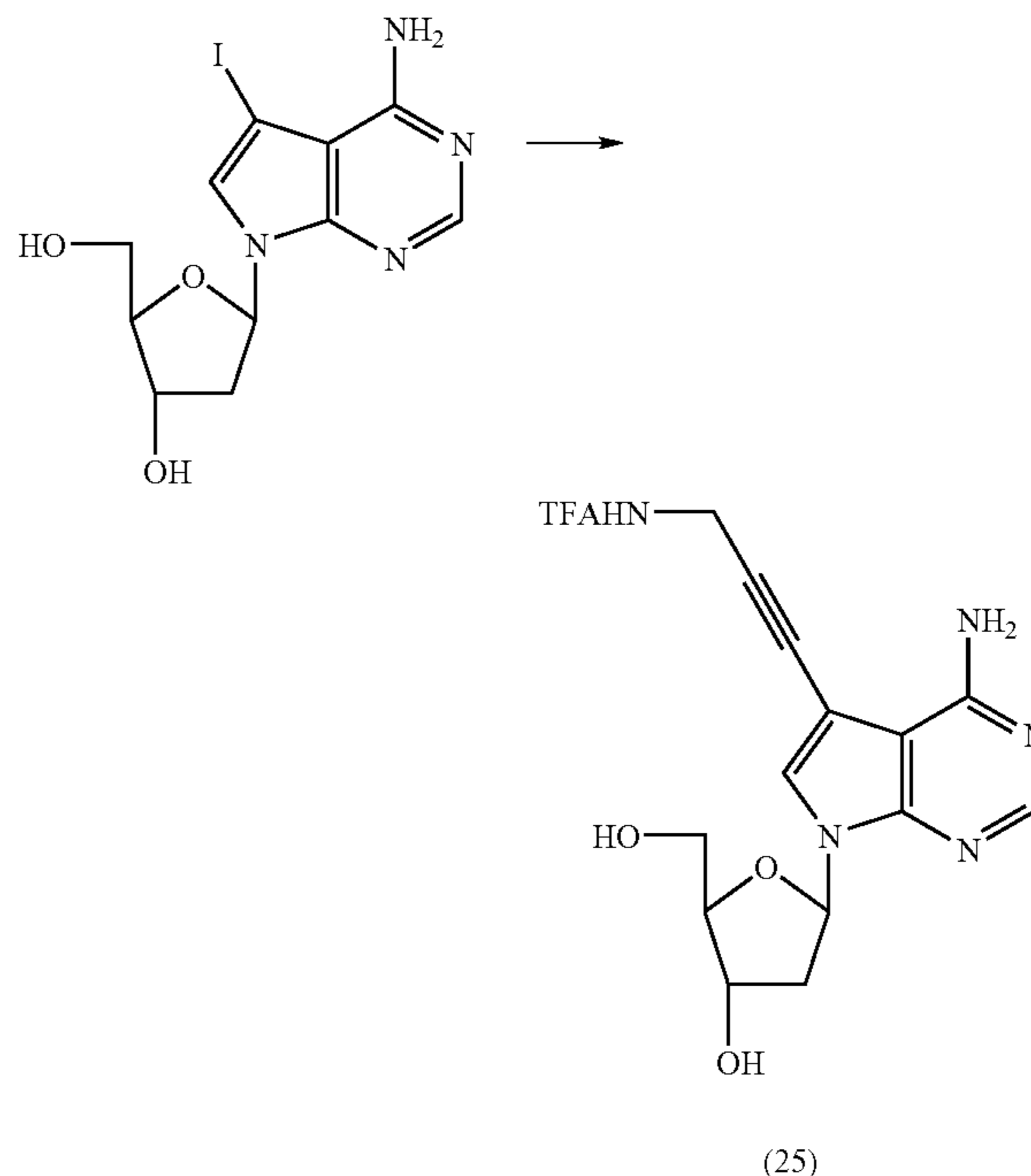
7-Deaza-7-[3-(2,2,2-trifluoroacetamido)-prop-1-ynyl]-2'-deoxyadenosine (25)
