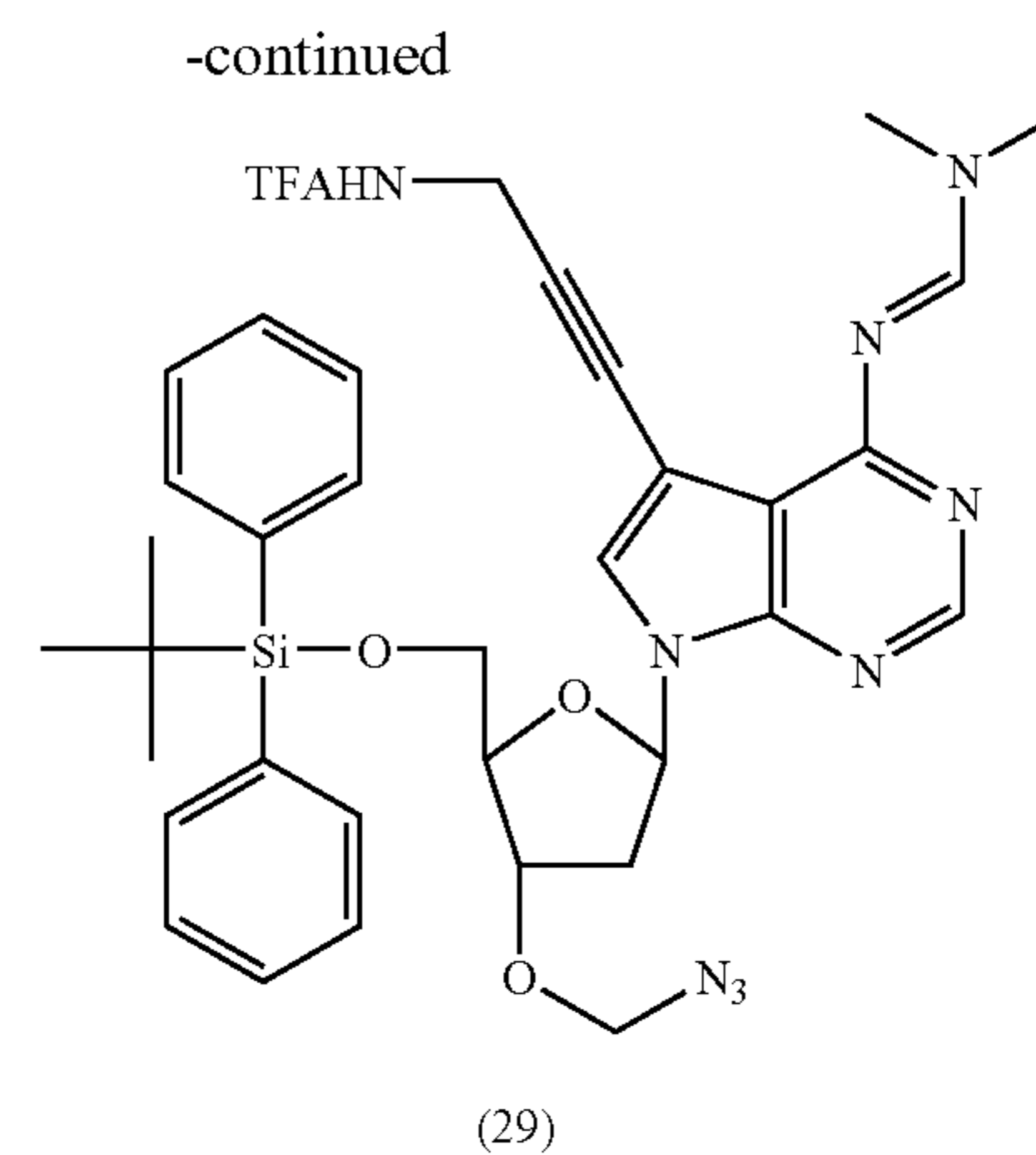
3'-O-Azidomethyl-5'-O-(tert-butyl-diphenylsilyl)-7-deaza-4-N,N-dimethylformadin-7-[3-(2,2,2-trifluoroacetamido)-prop-1-ynyl]-2'-deoxyadenosine (29)
