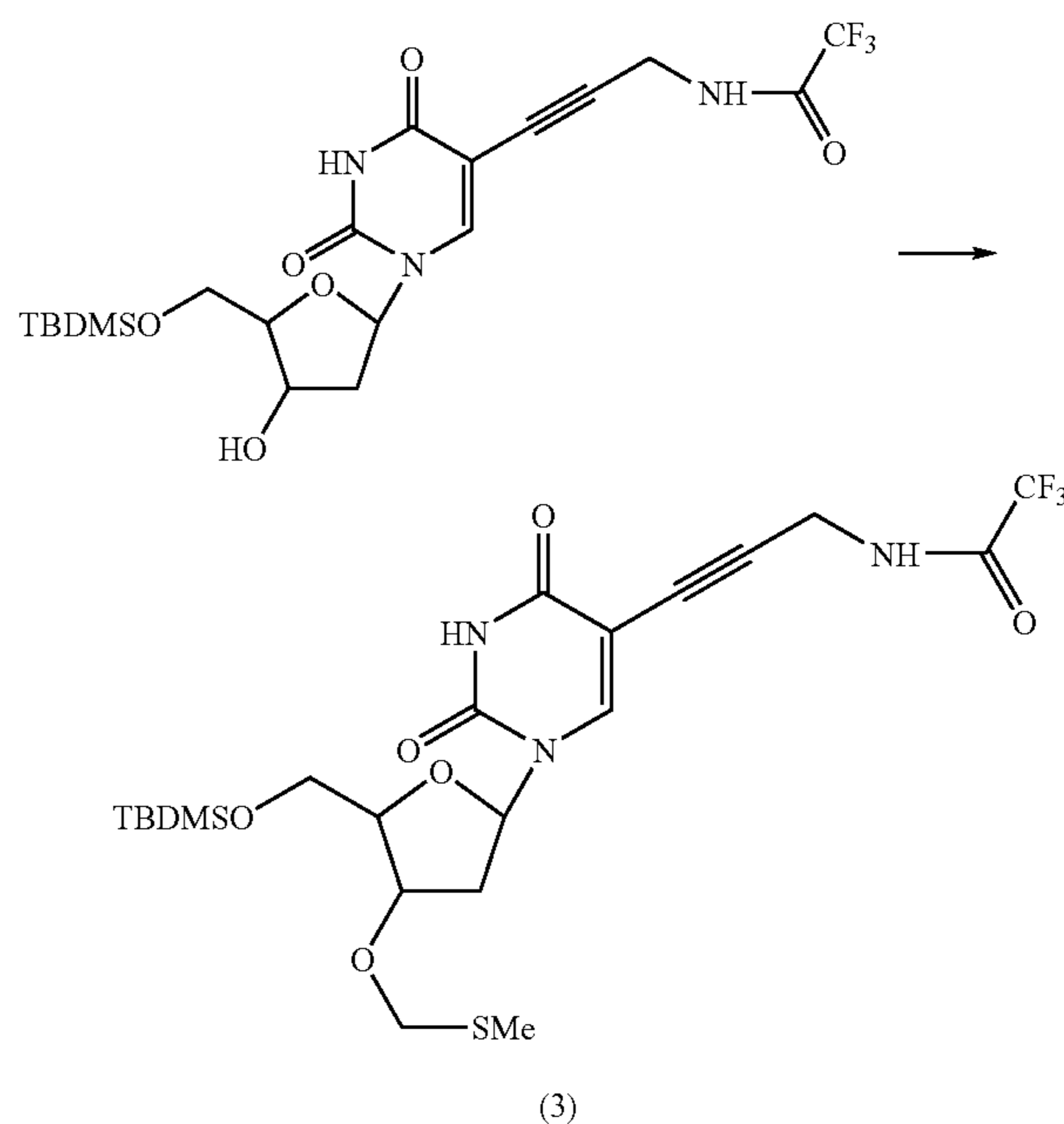
5'-O-(tert-Butyldimethylsilyl)-3'-O-methylthio- ethyl-5-[3-(2,2,2-trifluoroacetamido)-prop-1-ynyl]- 2'-deoxyuridine (3)
