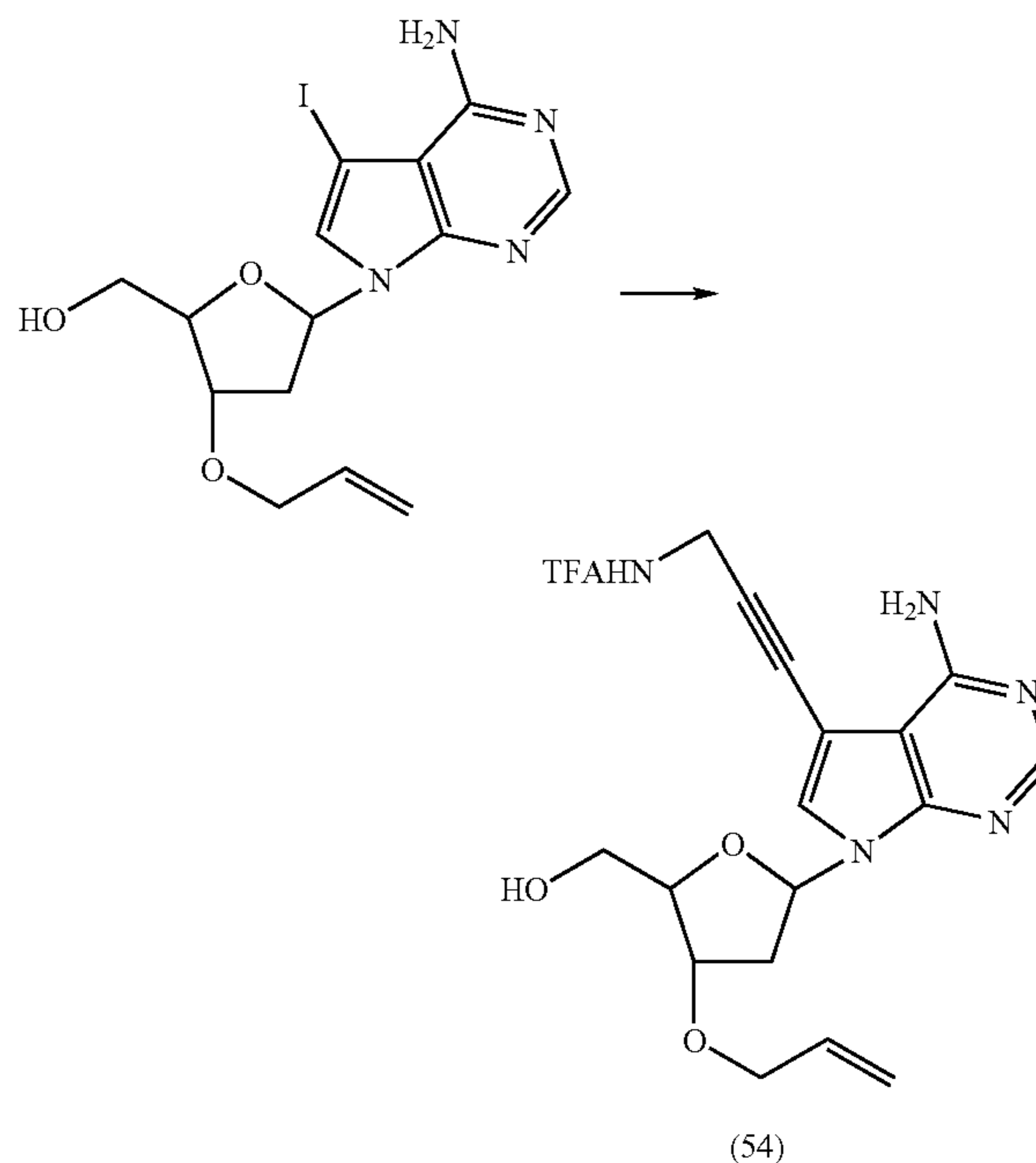
3'-O-Allyl-7-deaza-7-[3-(2,2,2-trifluoroacetamide)]-2'-deoxyadenosine (54)
