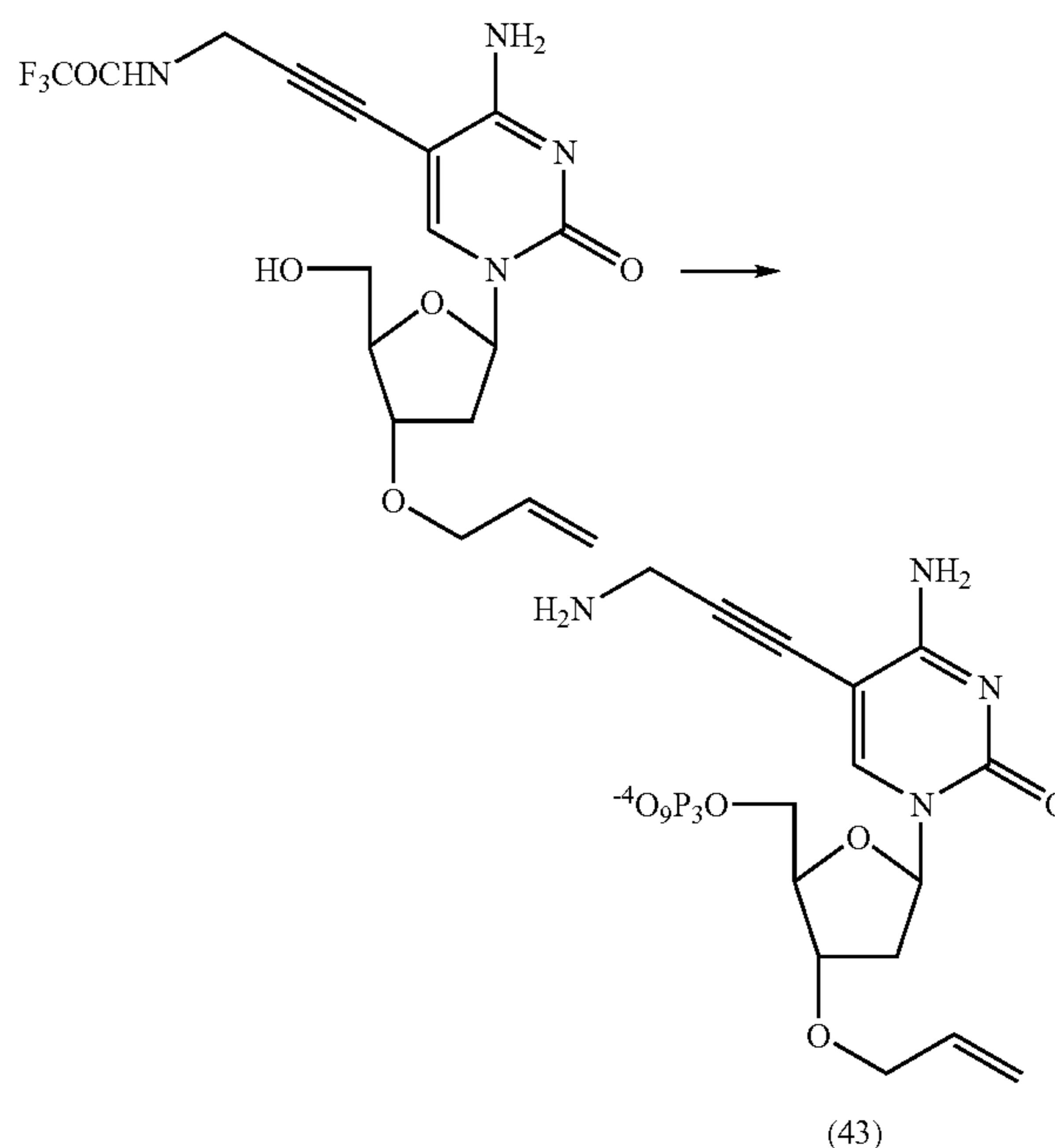
3'-O-Allyl-5-(3-amino-prop-1-ynyl)-5'-O-triphosphate-2'-deoxycytidine (43)
