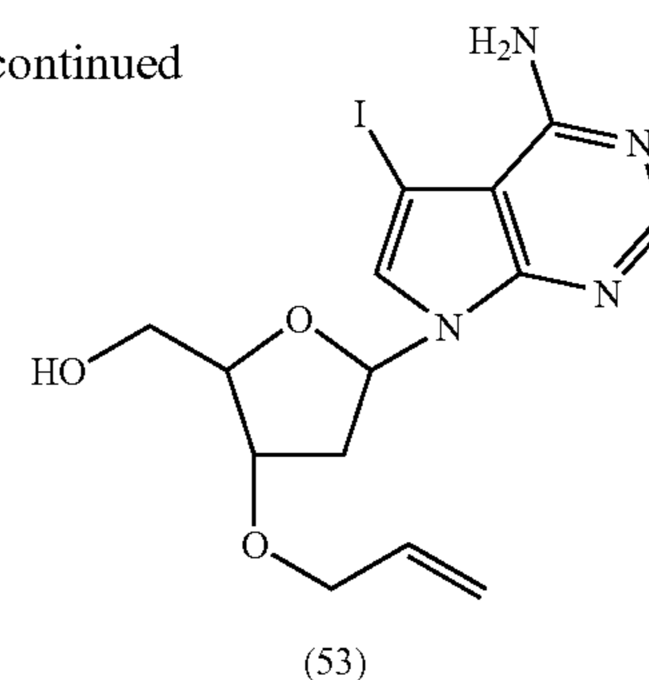
3'-O-Allyl-7-deaza-7-iodo-2'-deoxyadenosine (53)
