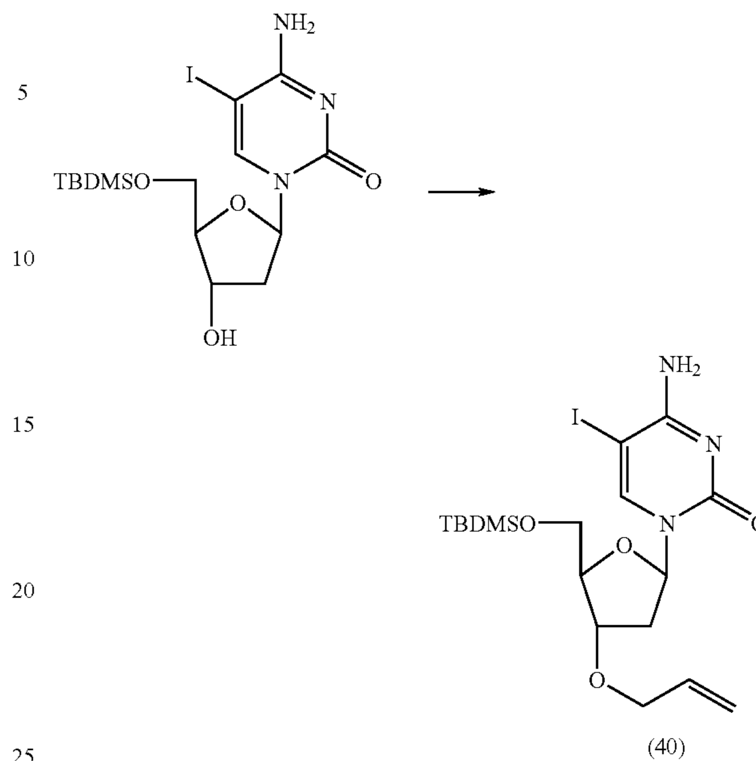
3'-O-Allyl-5'-O-(tert-butyl dimethylsilyl)-5-iodo-2'-deoxycytidine (40)
