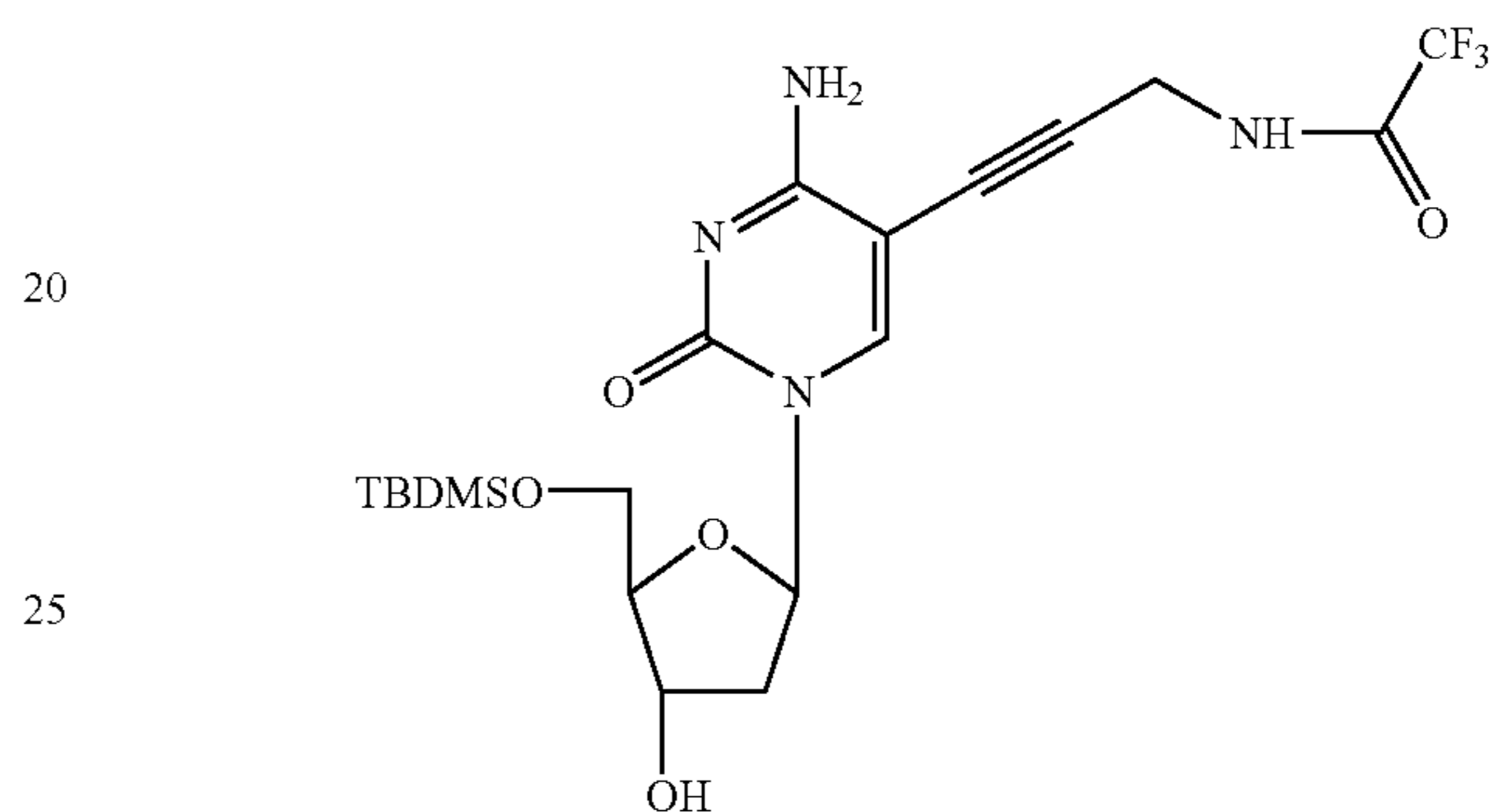
5'-O-(tert-Butyldimethylsilyl)-5-[3-(2,2,2-trifluoroacetamido)-prop-1-ynyl]-2'-deoxycytidine (8)
