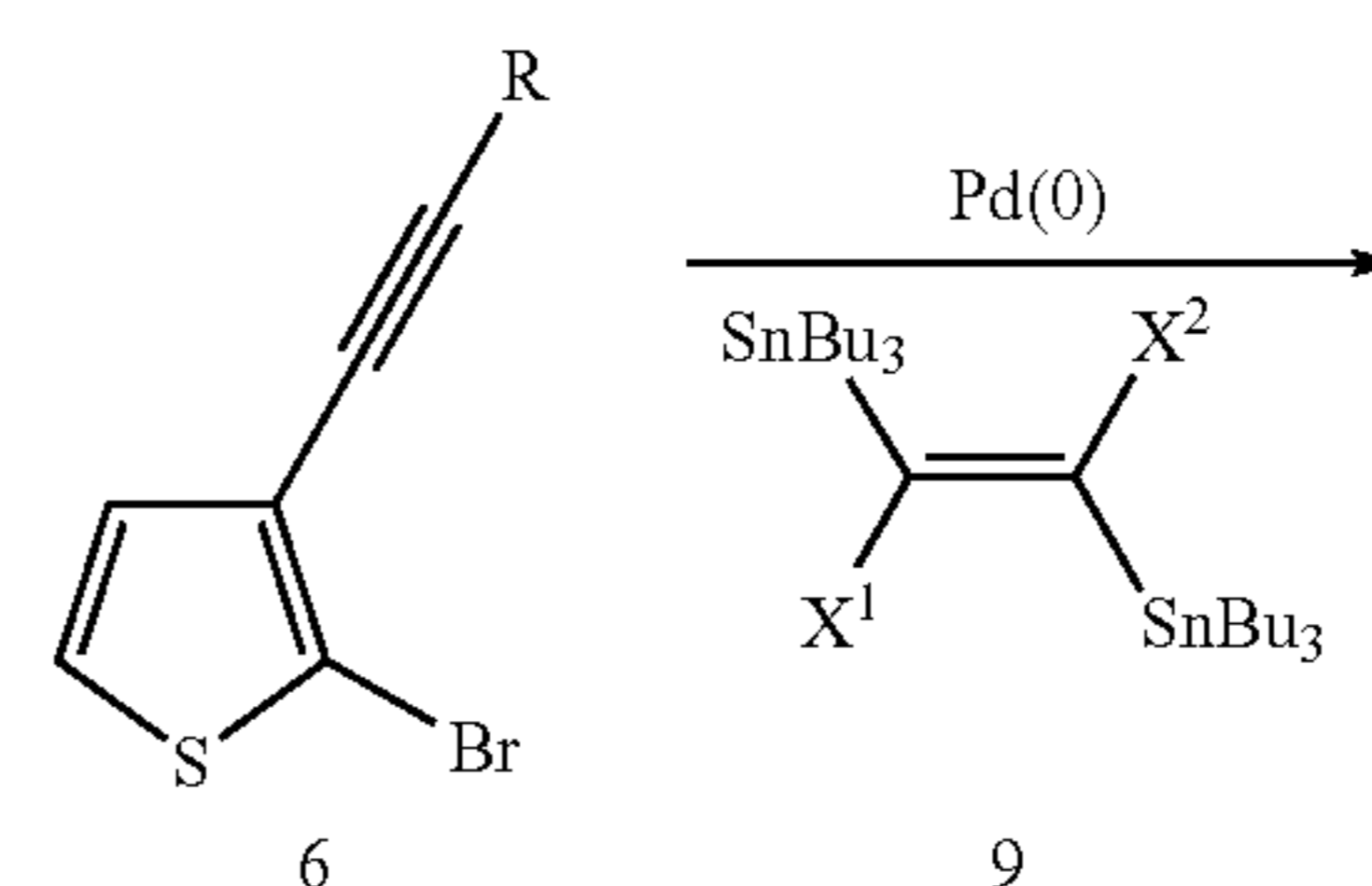
Scheme 7:
