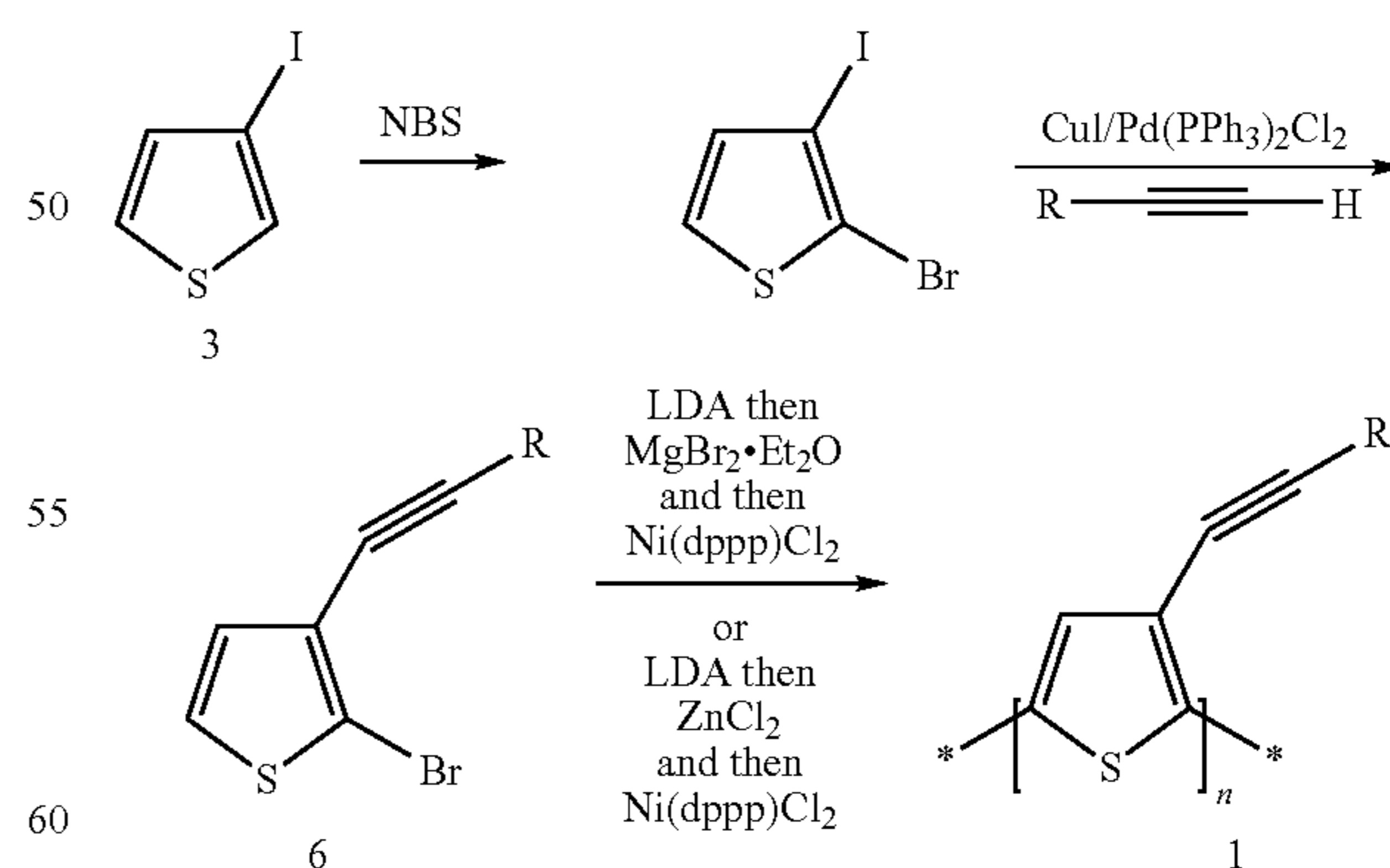
Scheme 3:
