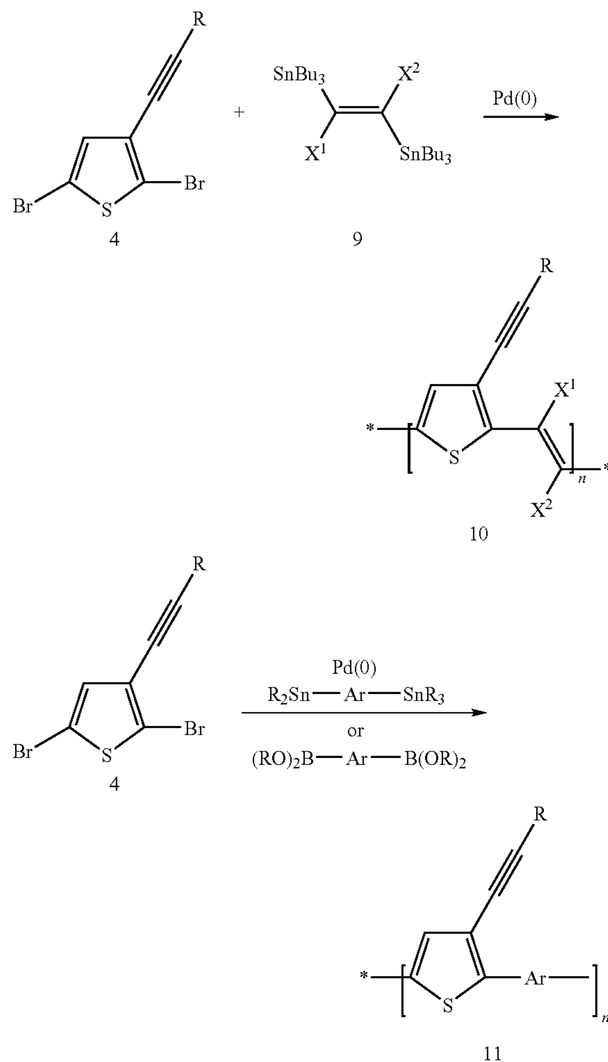
Scheme 6:
