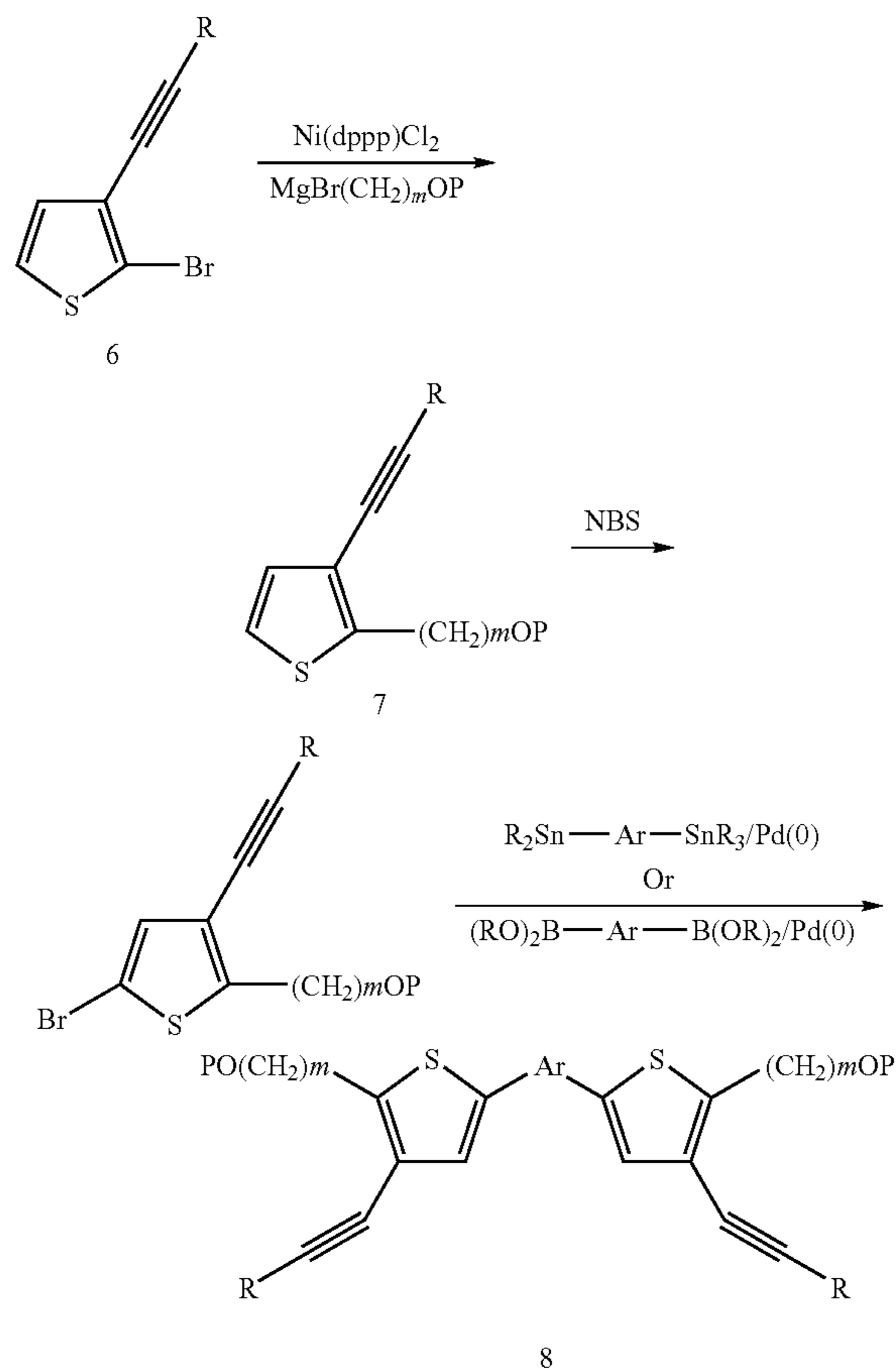
Scheme 5:
