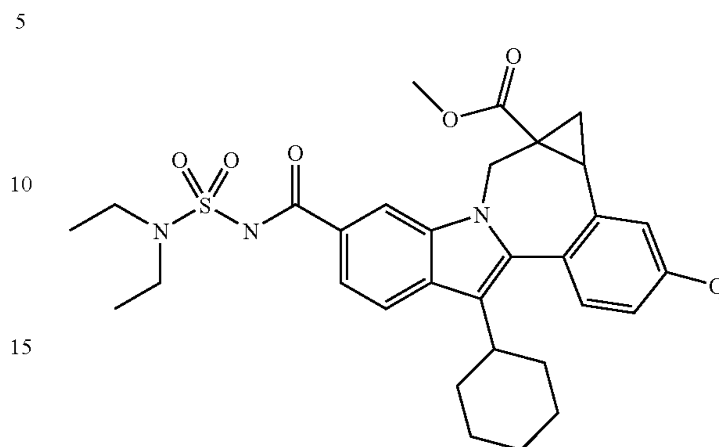
Intermediate 59
