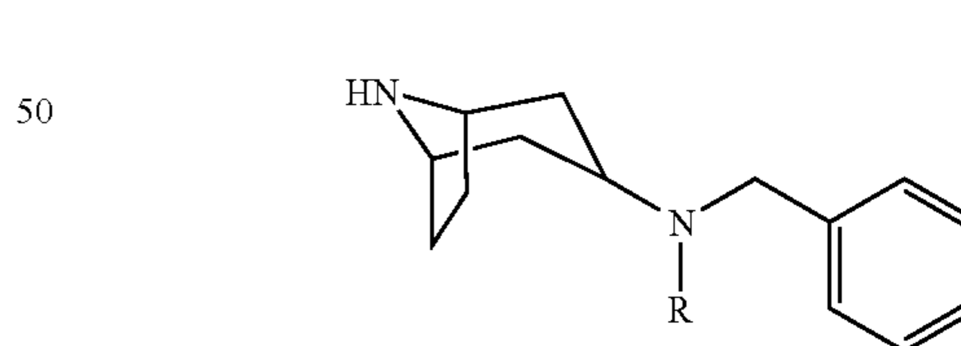
Intermediate 61
