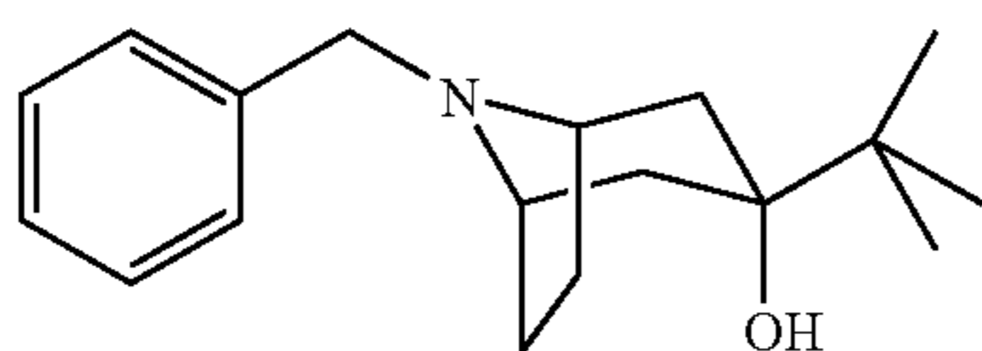
Intermediate 71
