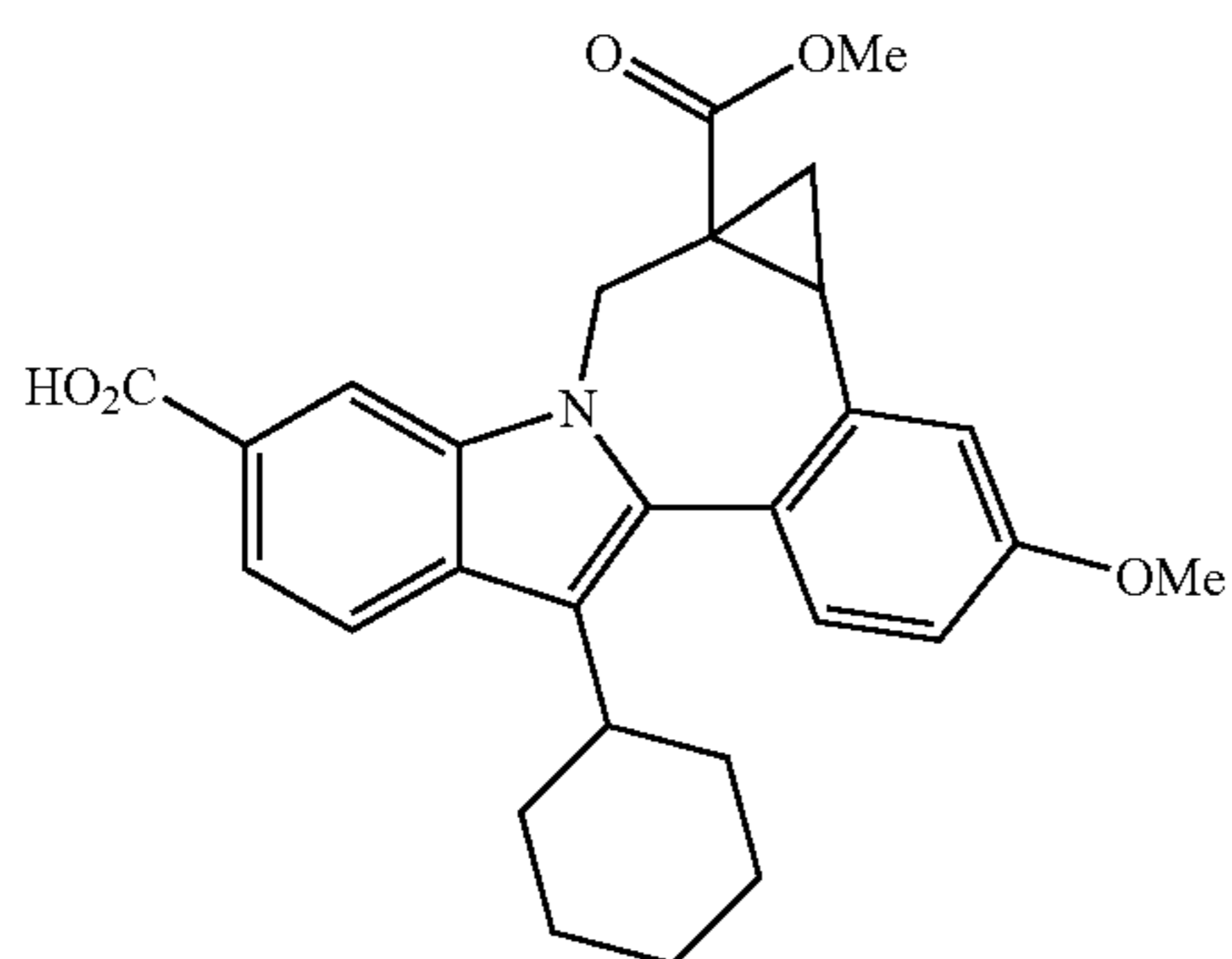
Intermediate 41
