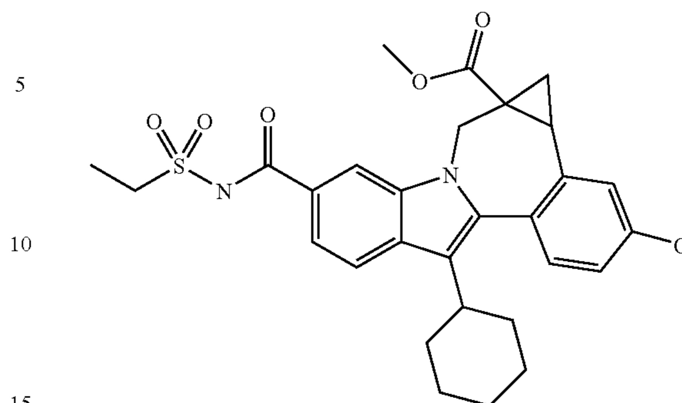
Intermediate 53
