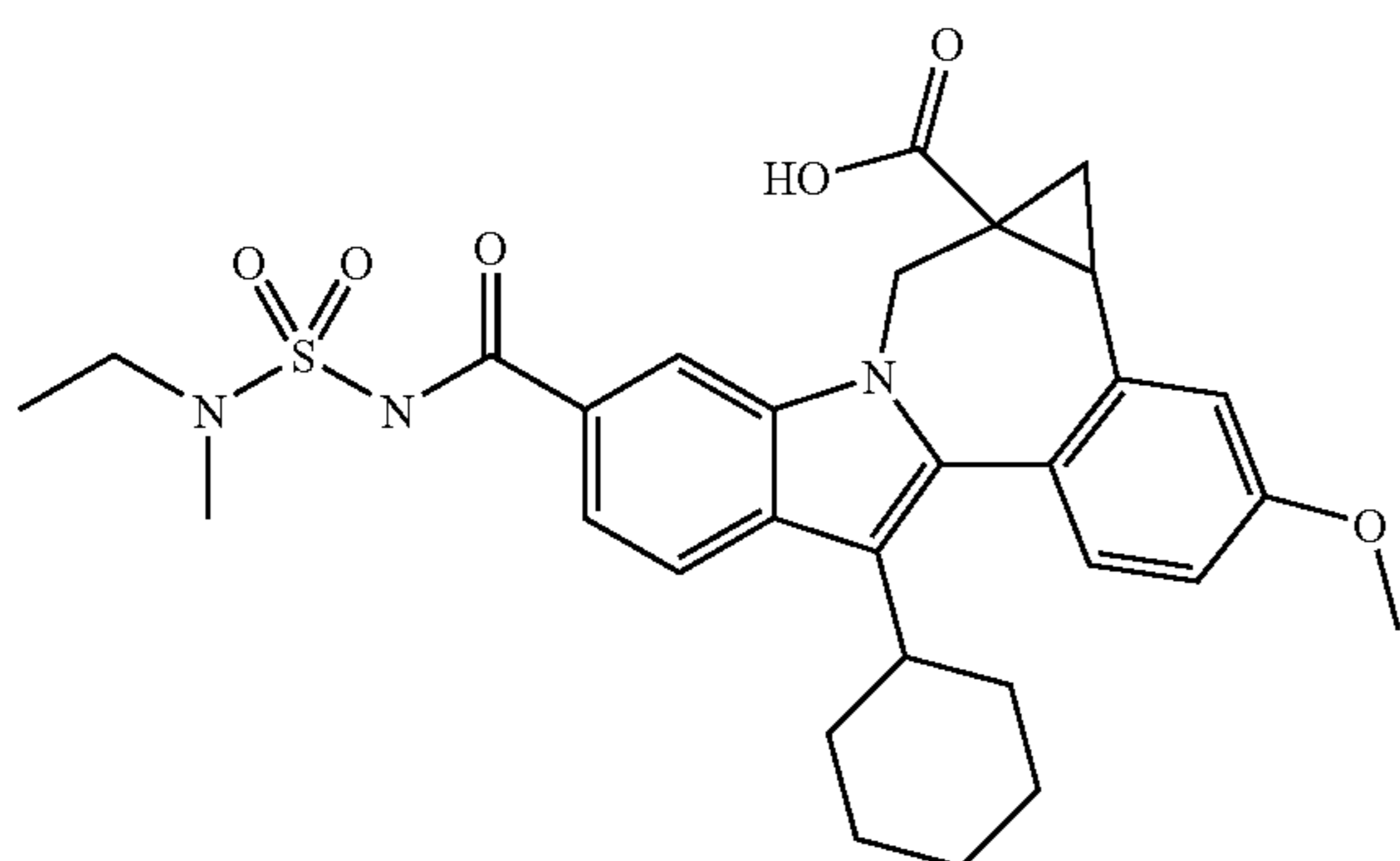
Intermediate 58
