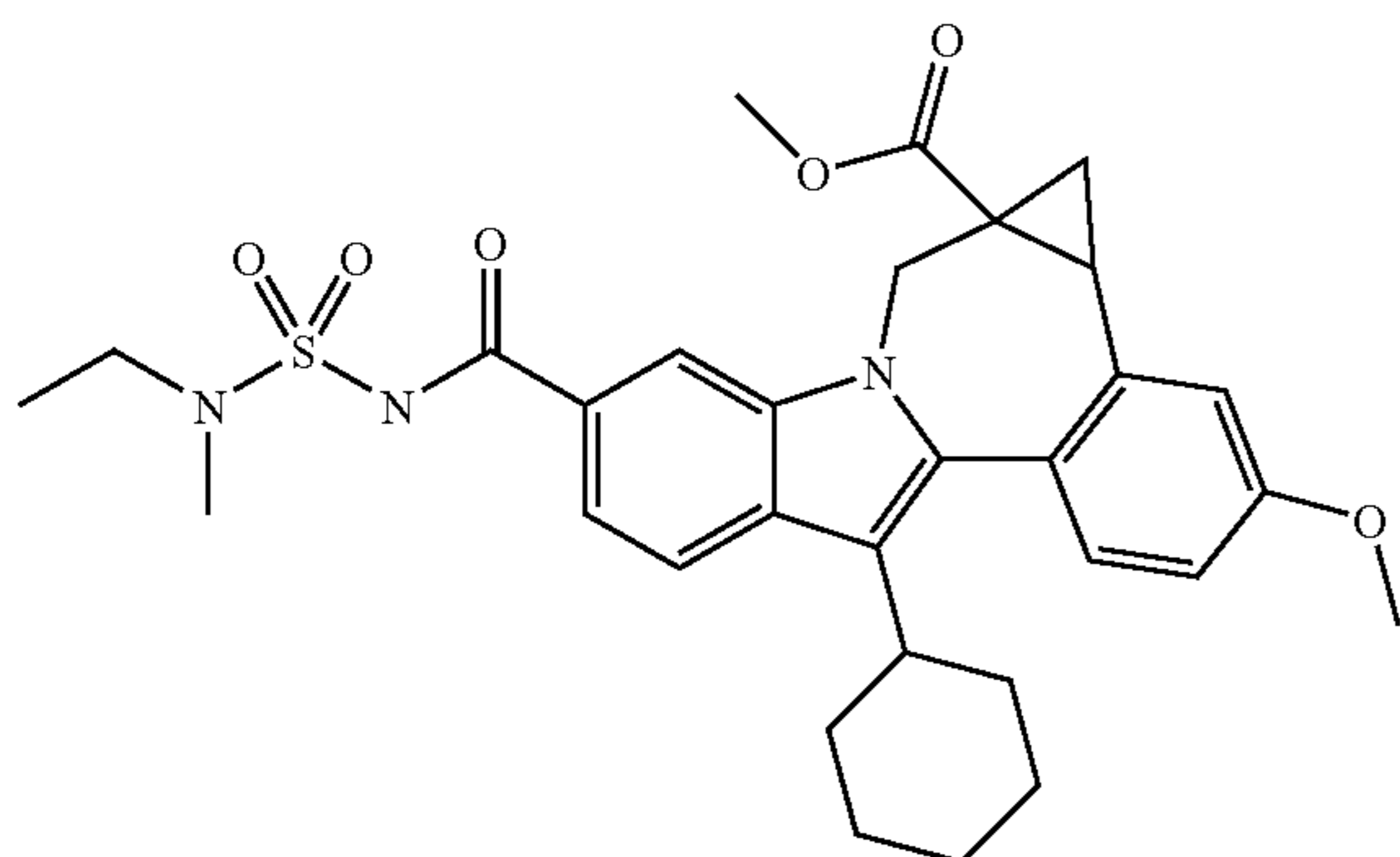
Intermediate 57
