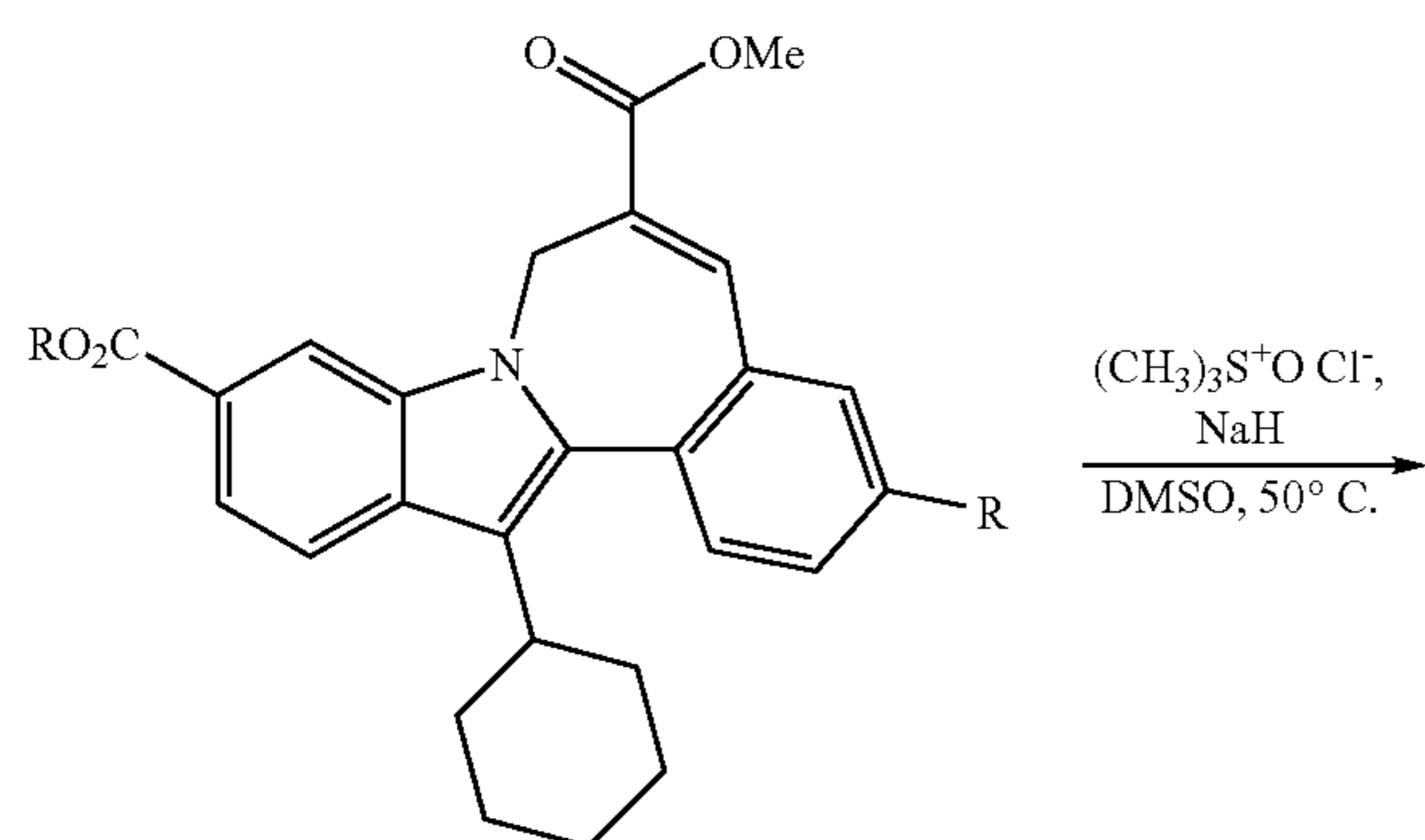
Scheme 4.
