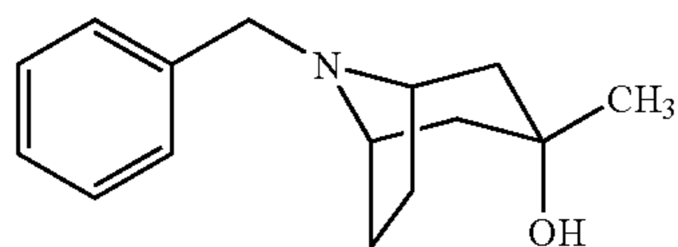
Intermediate 69
