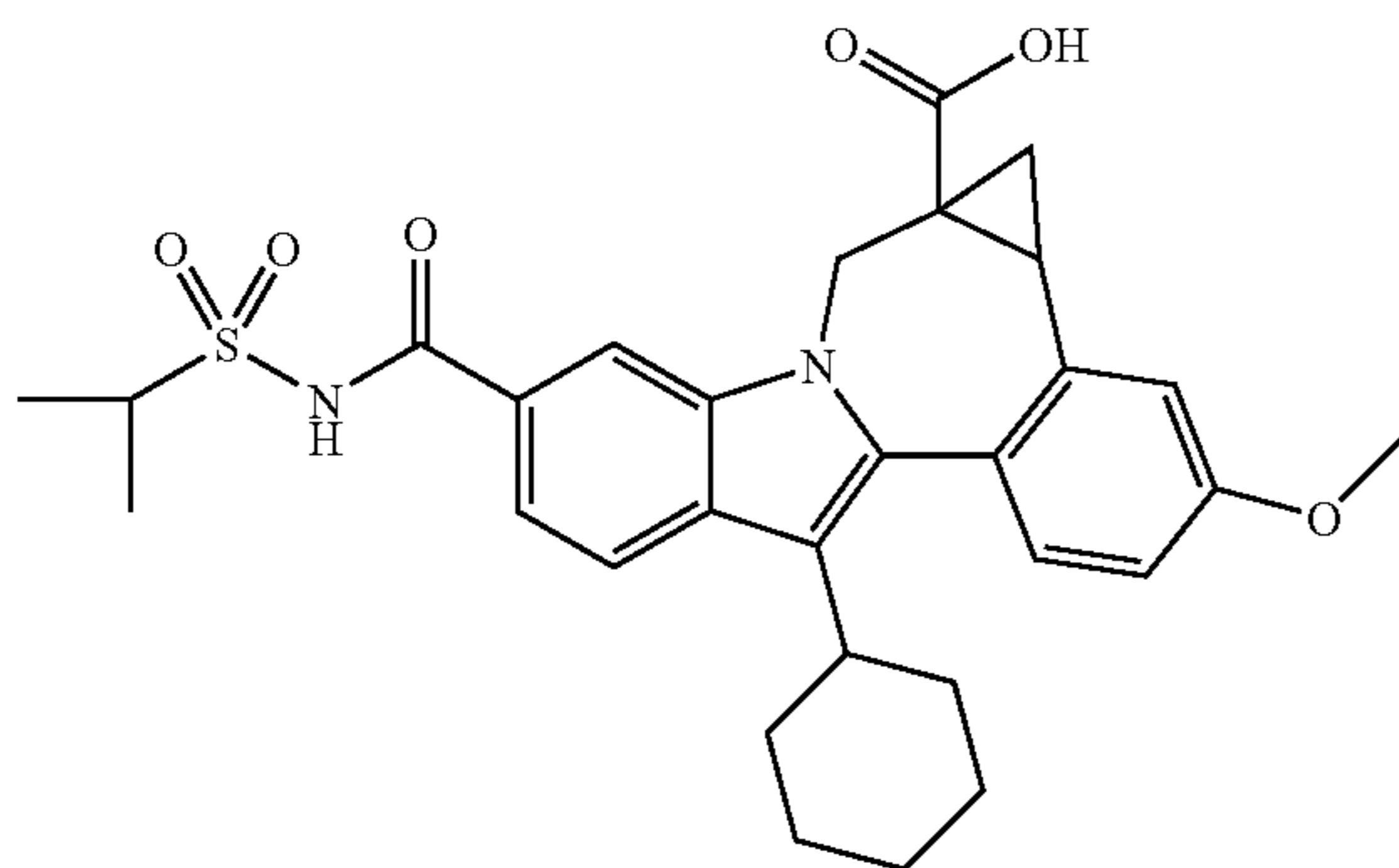
Intermediate 35
