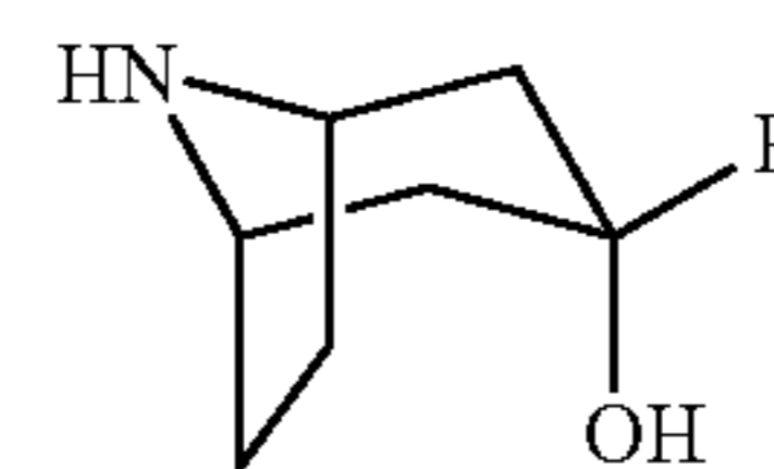
Intermediate 68
