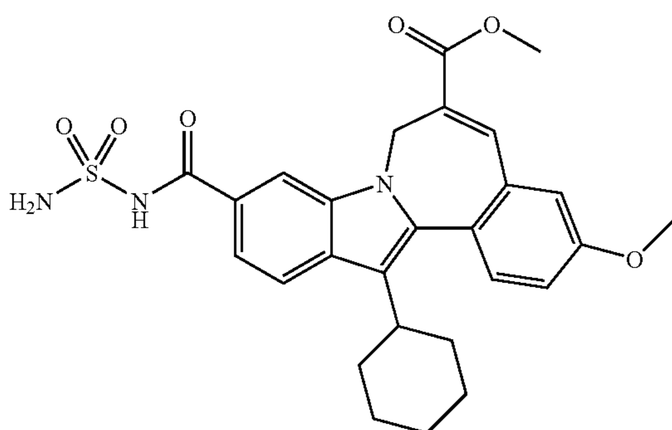
Intermediate 36
