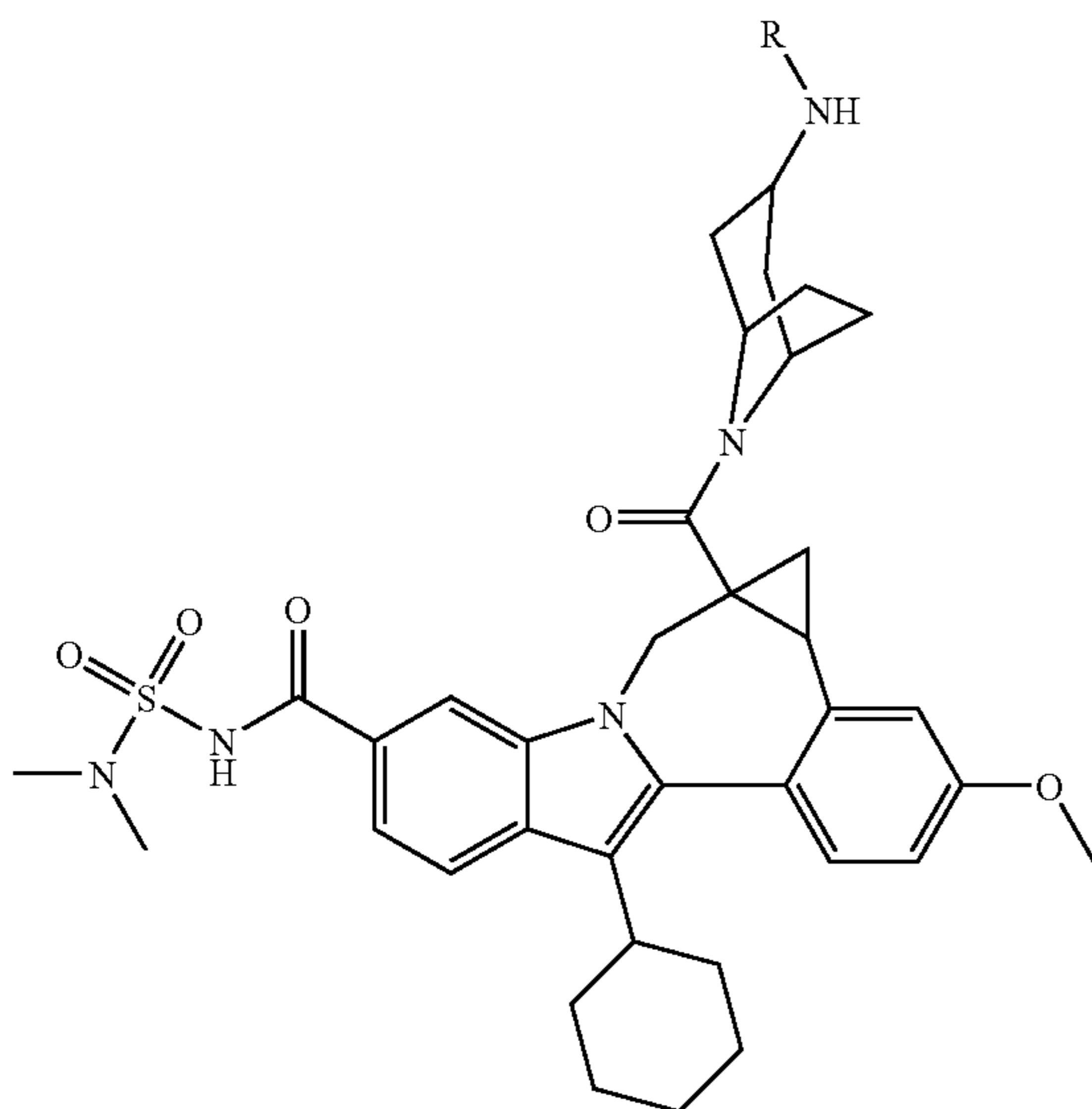
Intermediate 75
