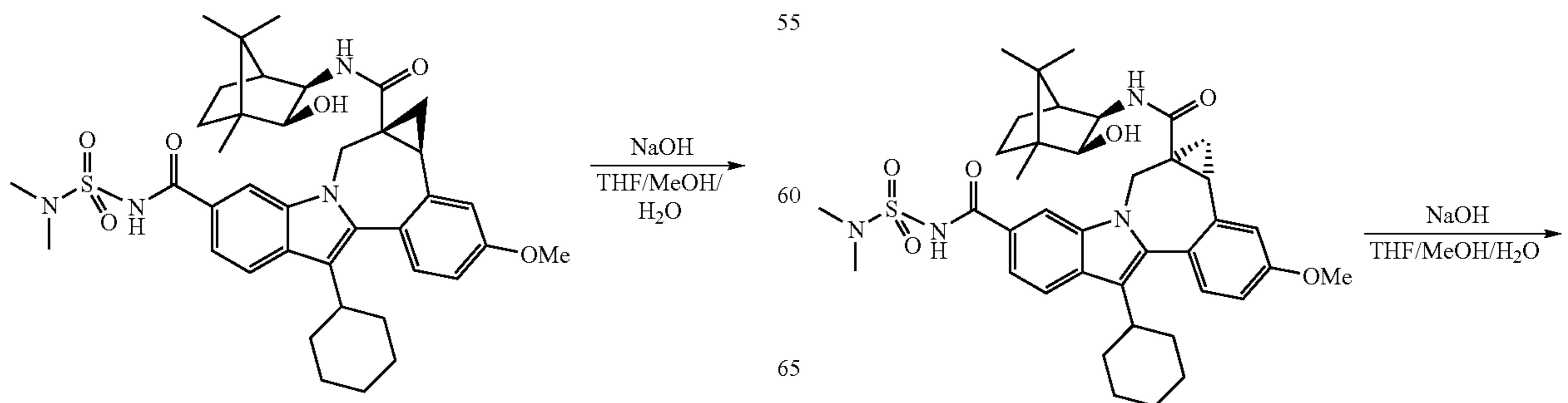
Scheme 6.
