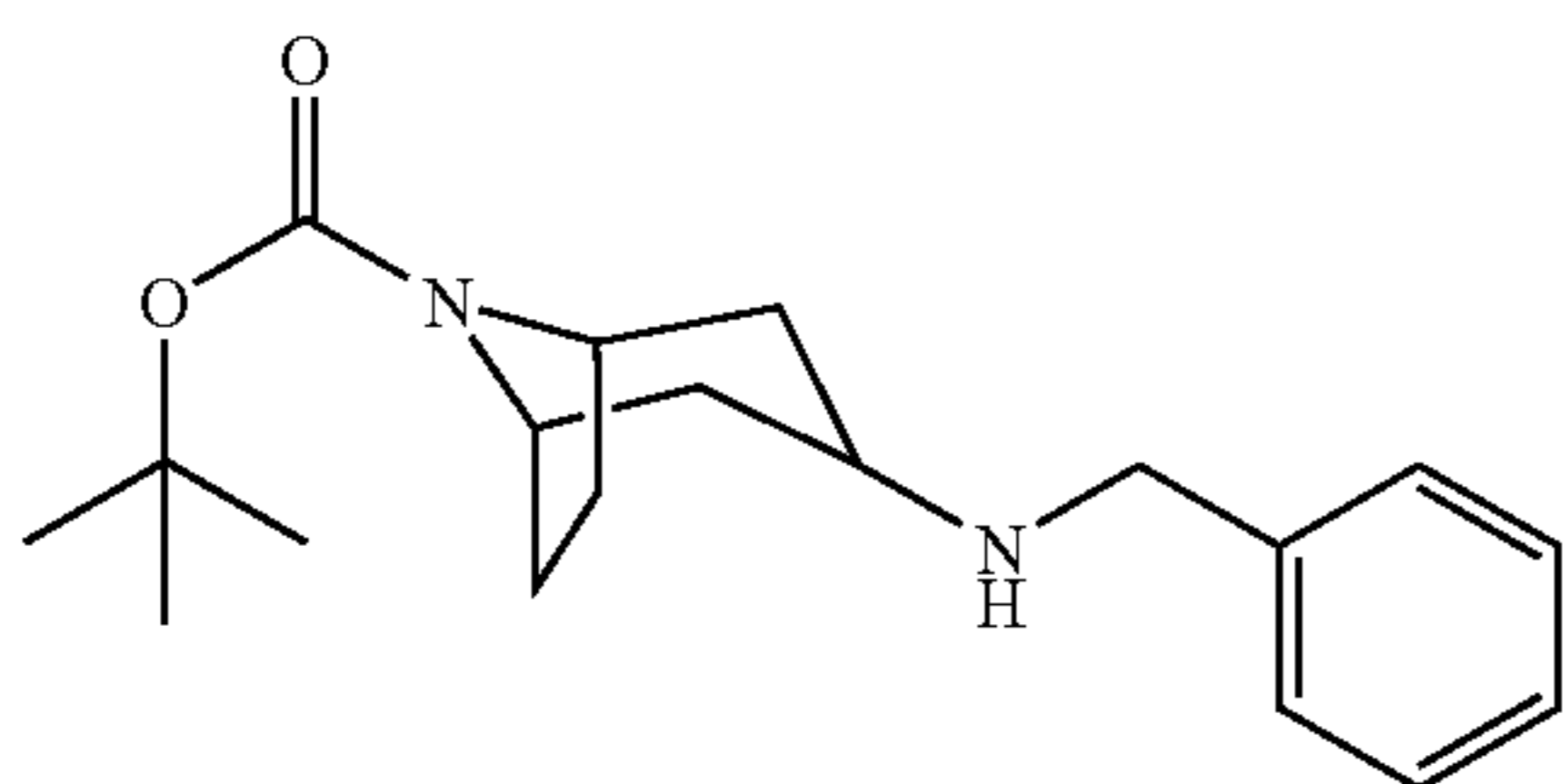
Intermediate 62
