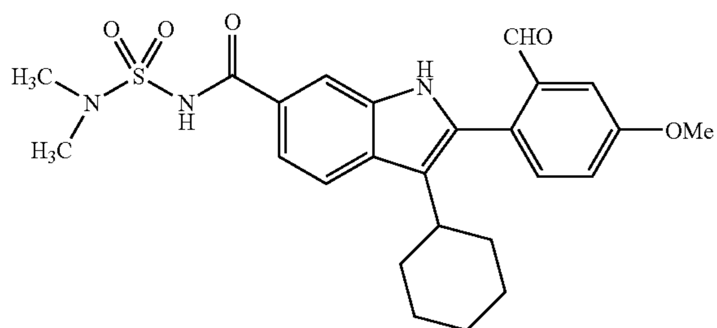
67 Intermediate 4
