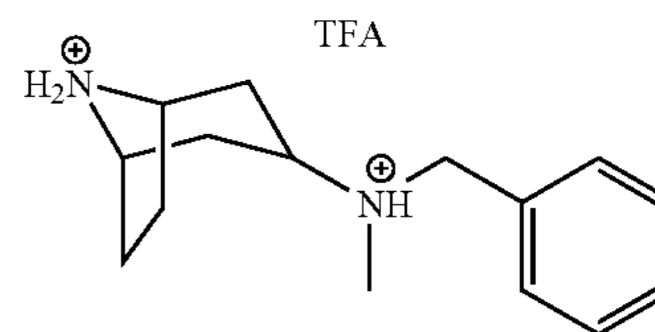
Intermediate 65
