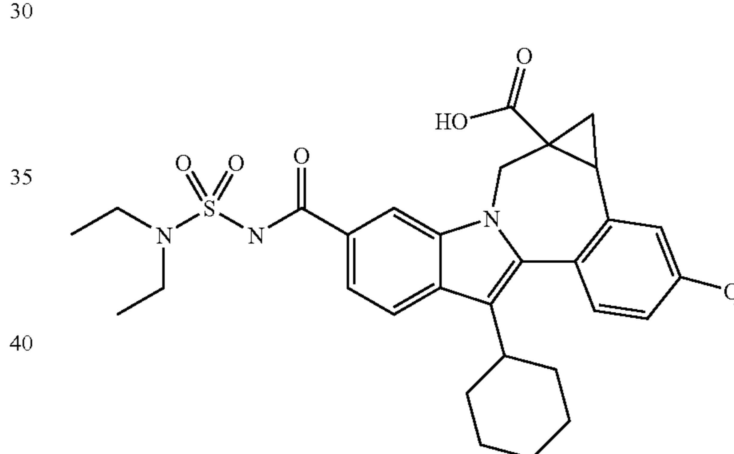
Intermediate 60
