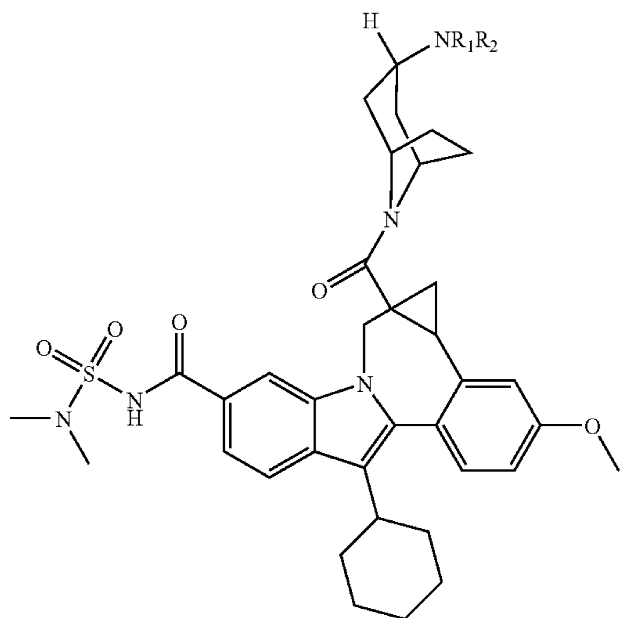
Intermediate 74
