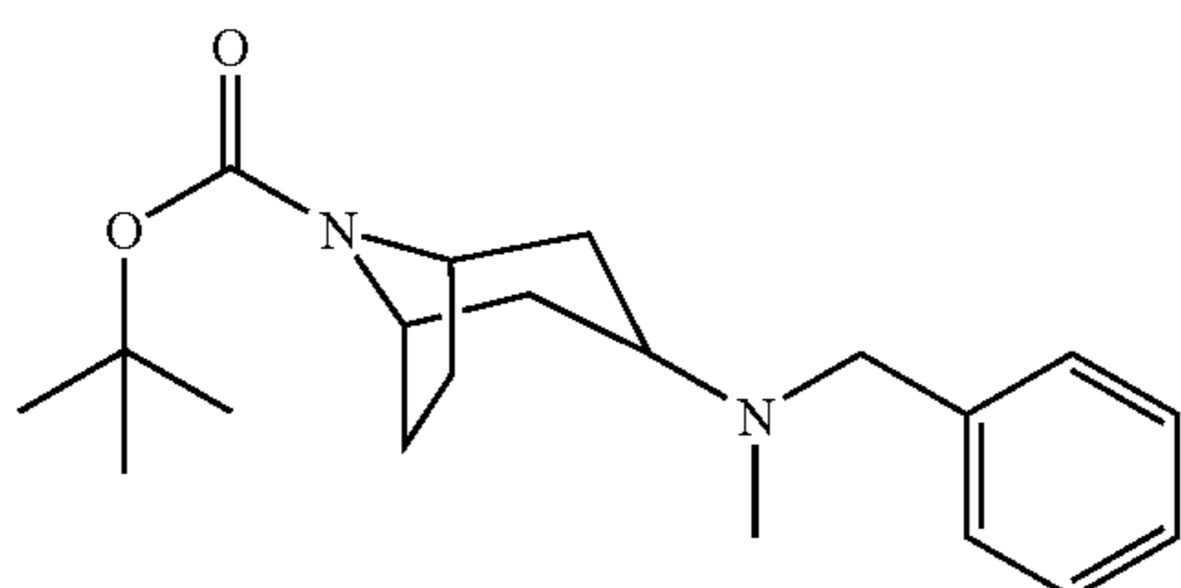
Intermediate 64
