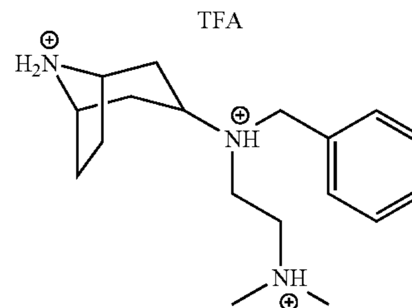
Intermediate 67
