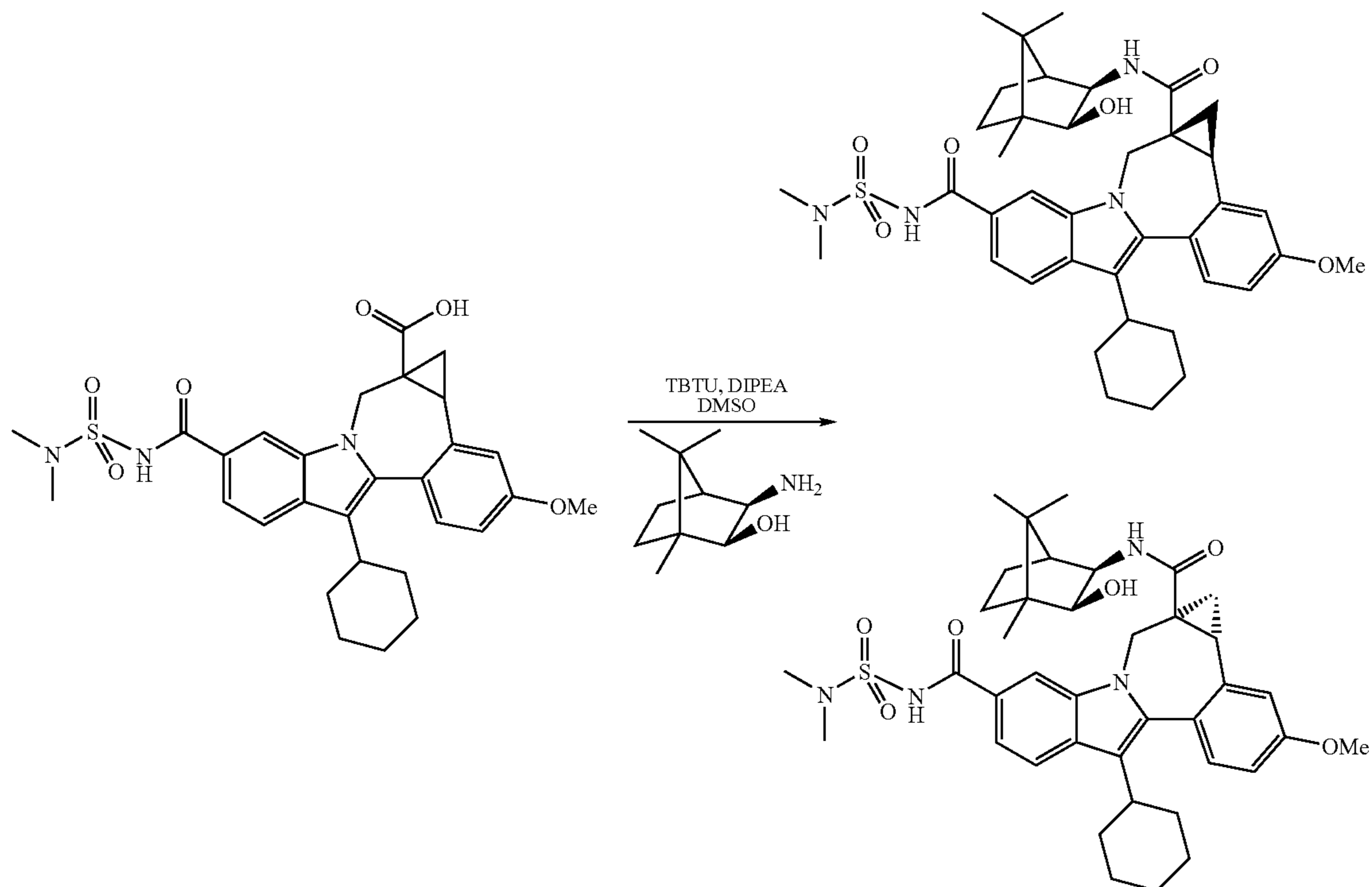
Scheme 6.
