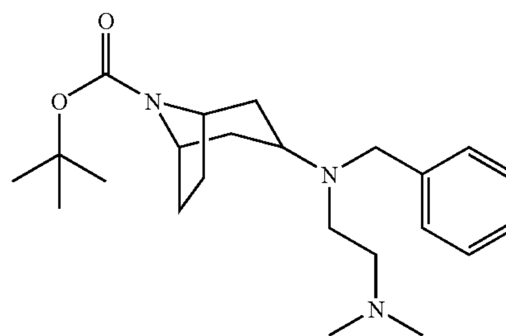
Intermediate 66
