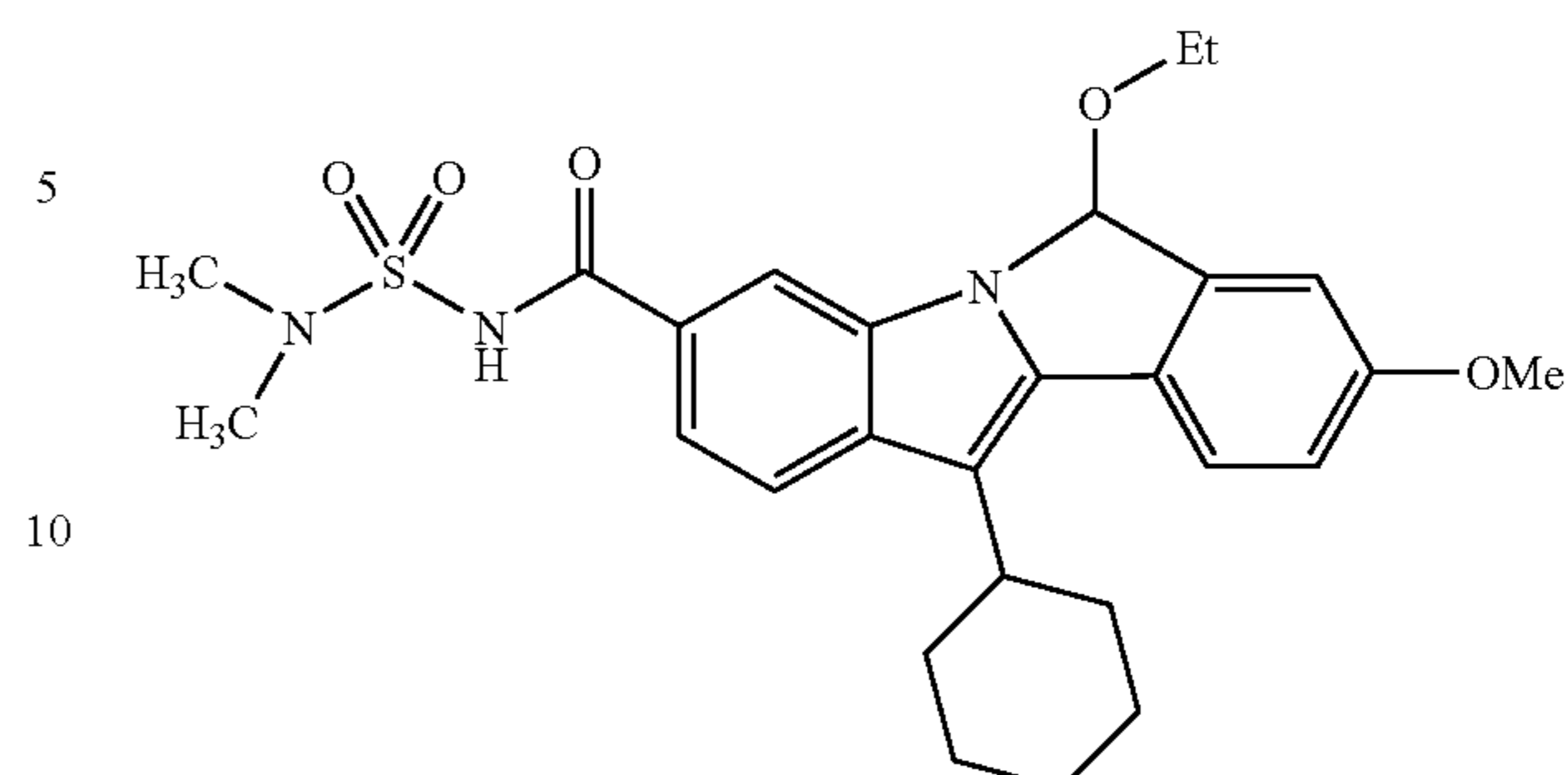
68 Intermediate 5
