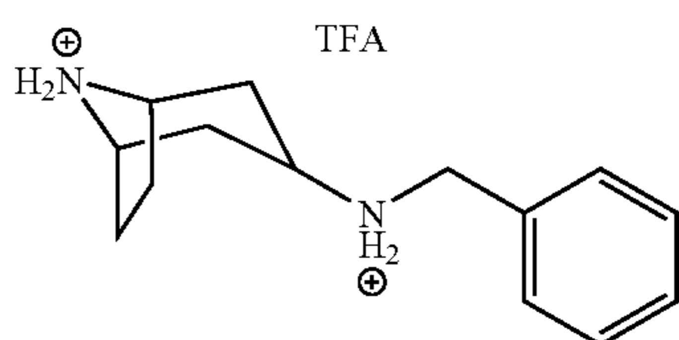
Intermediate 63
