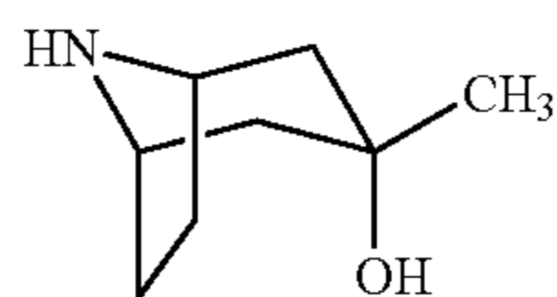
Intermediate 70
