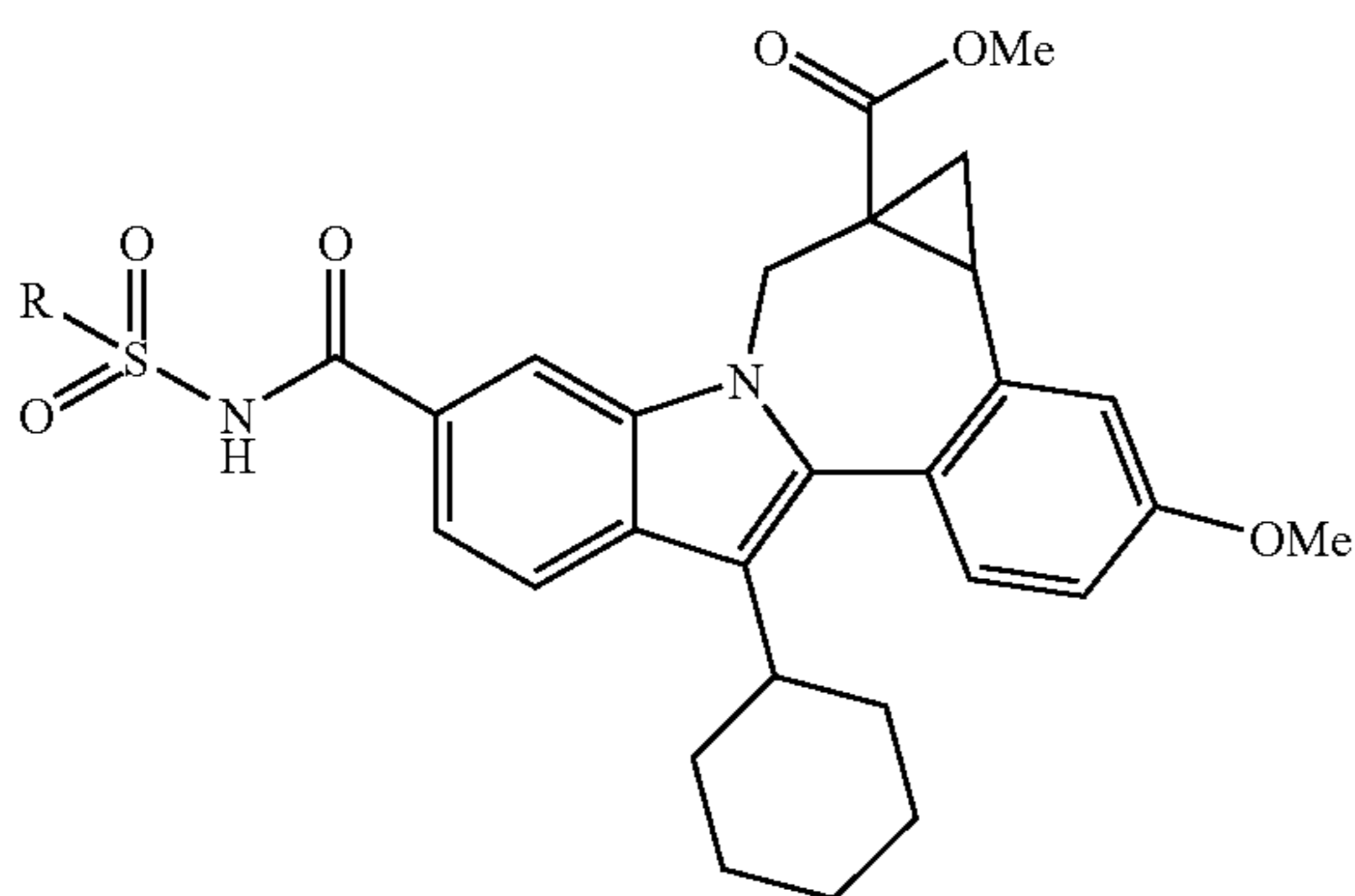
Intermediate 42
