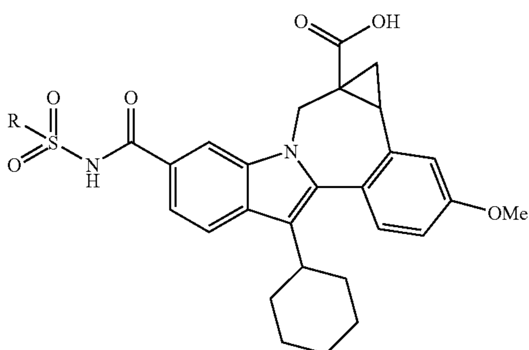
Intermediate 43
