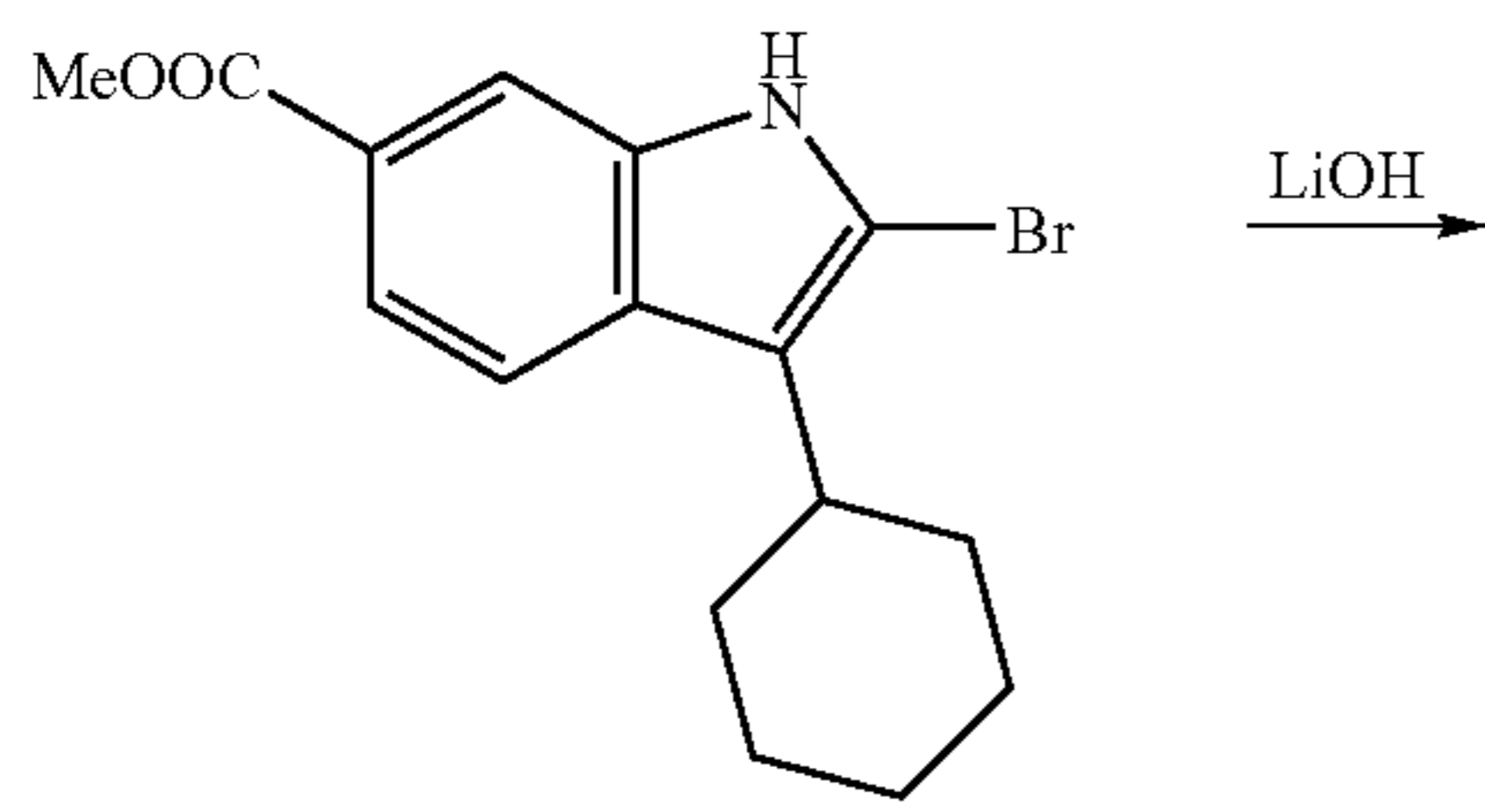
Scheme 3.
