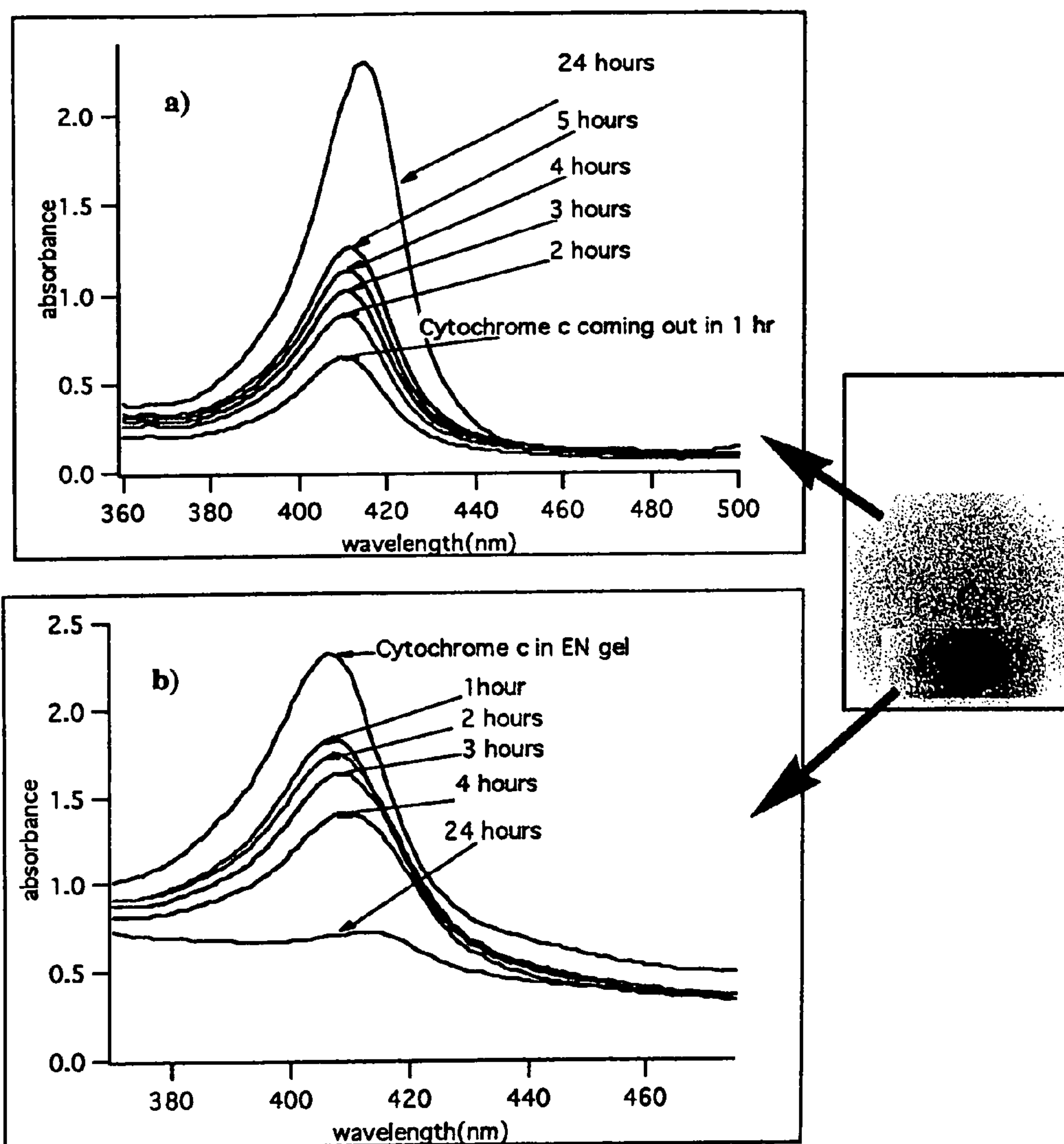
Fig.6 a) shows the release of Cyt c with time from the enTMOS gel in acetate solution. b) shows the release of Cyt c with time from the enTMOS gel.
