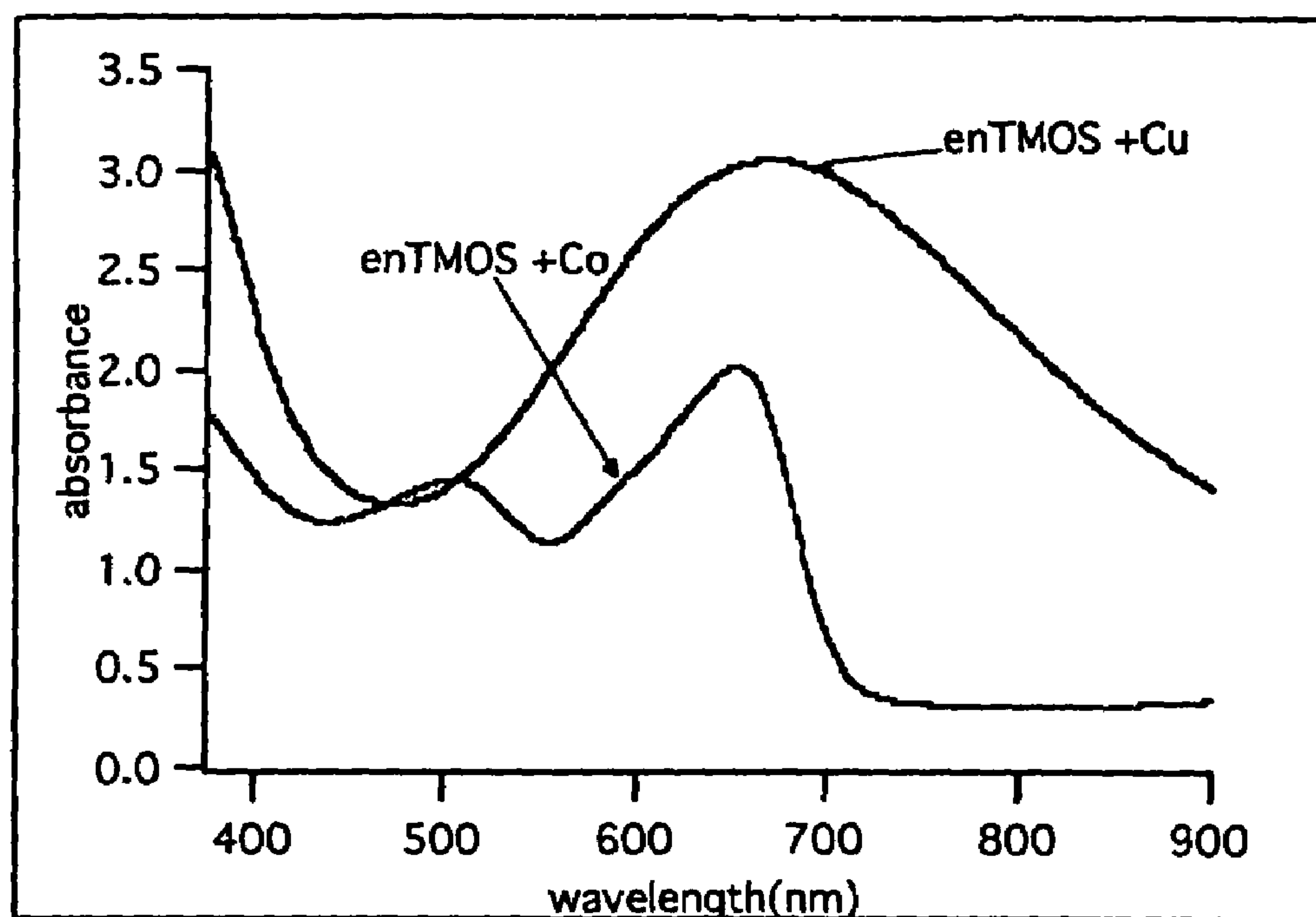
Fig.12 shows the intake of \text{Cu}^{(+2)} and \text{Co}^{(+2)} ions by enTMOS gel
