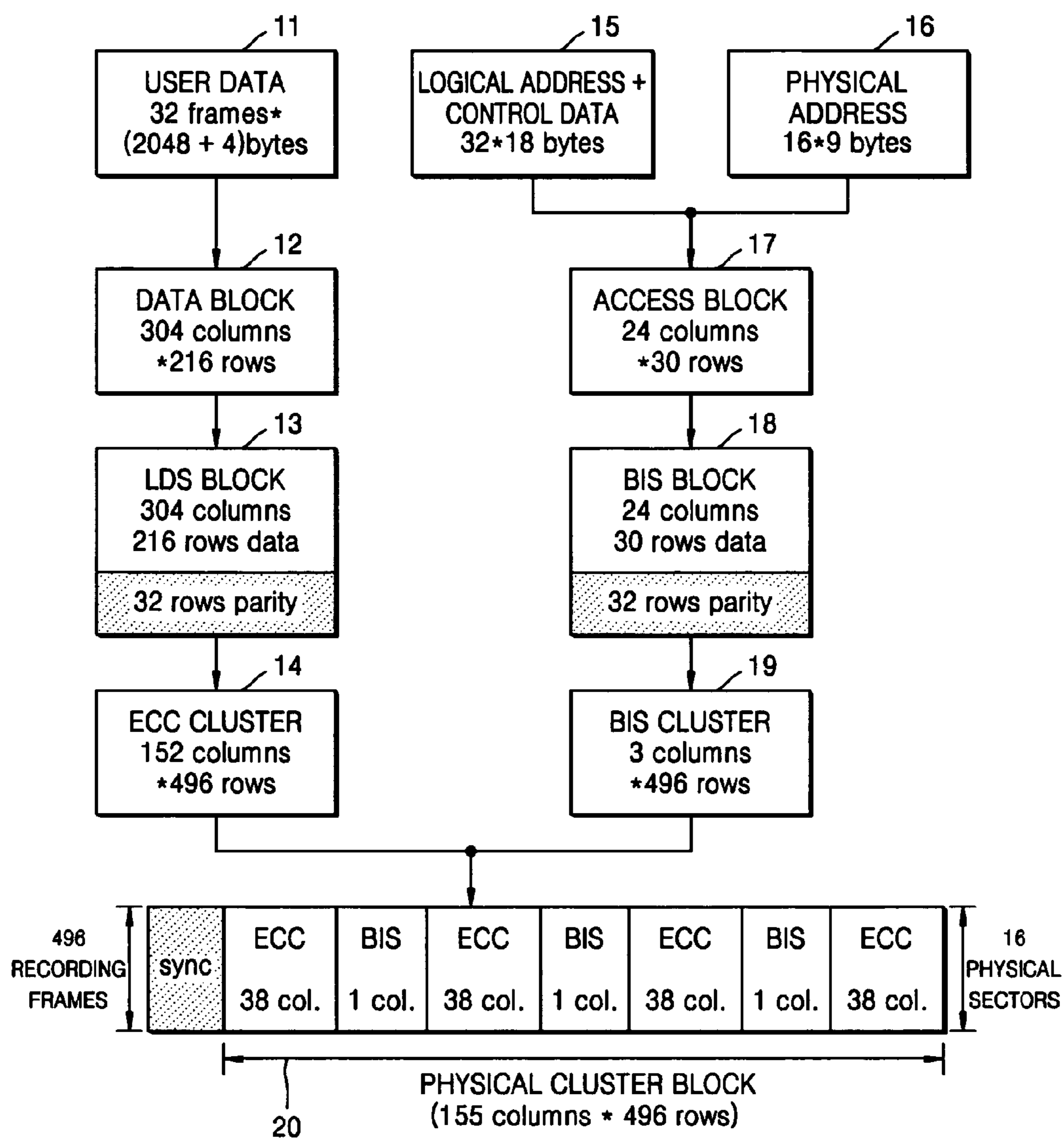
FIG. 1 (PRIOR ART)
