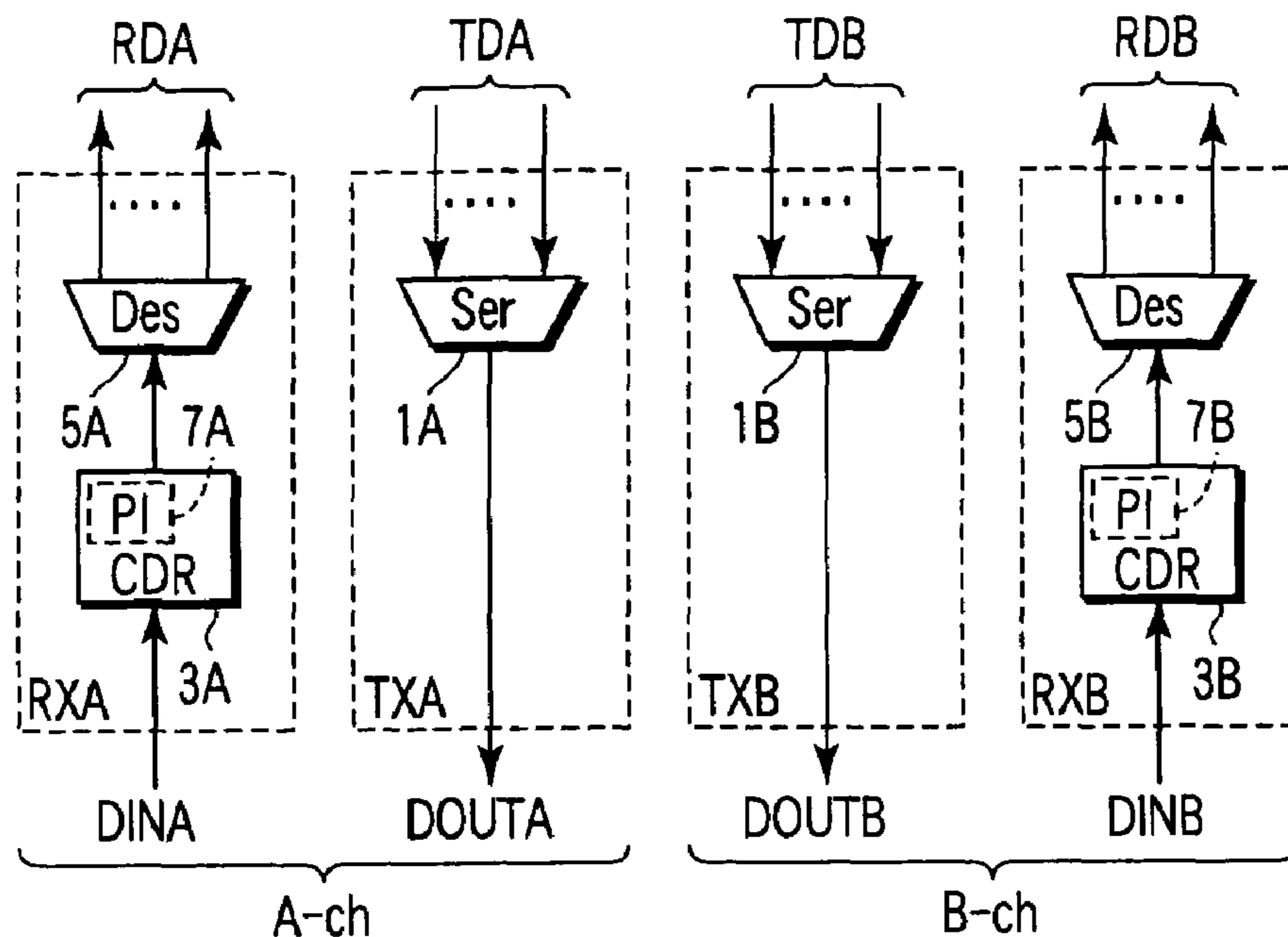
High-speed serial data interface
