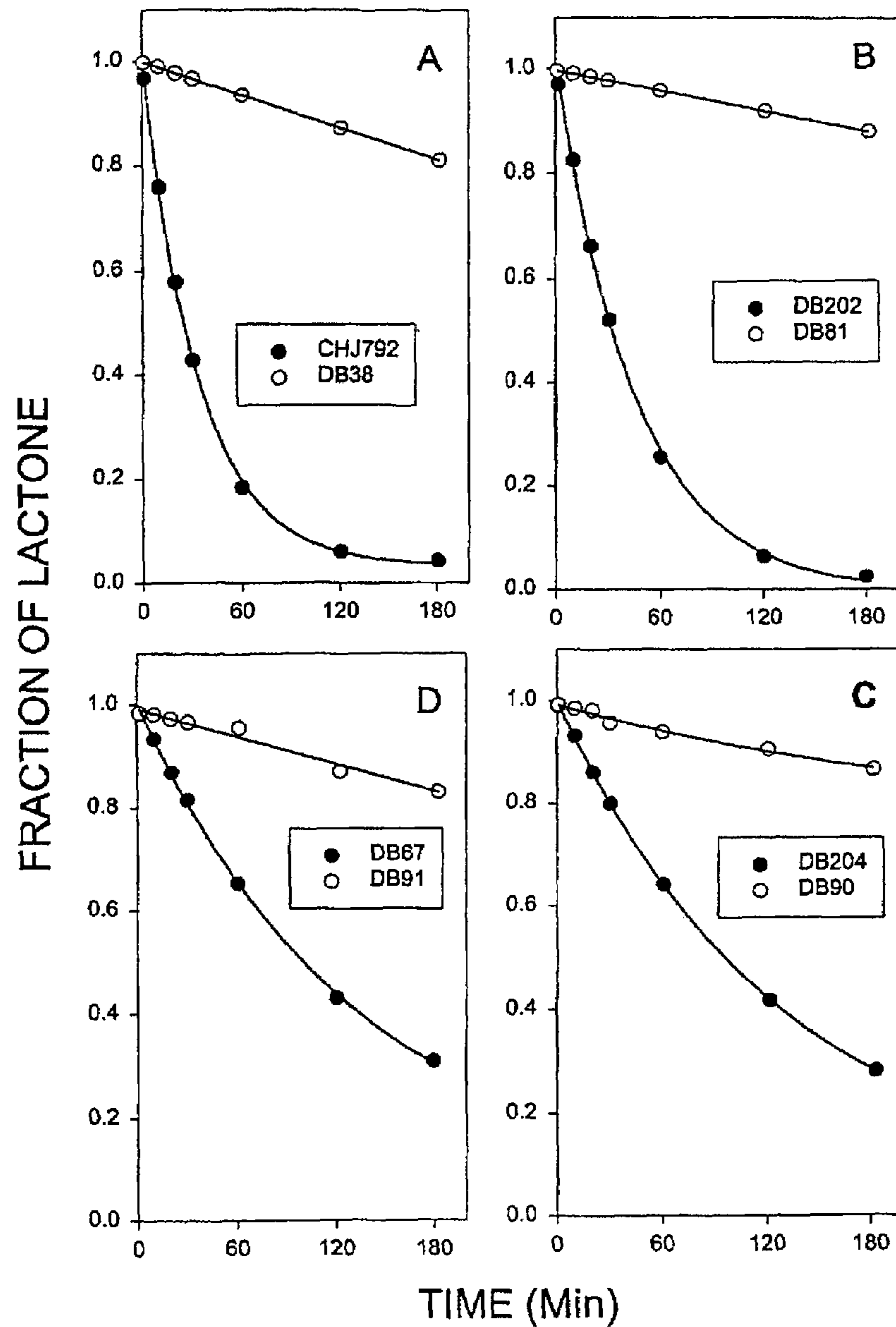
Figure 13. Comparison of the Stabilities of \alpha -Lactone Silatecans with their corresponding Homosilatecans in PBS/HSA at 37°C
