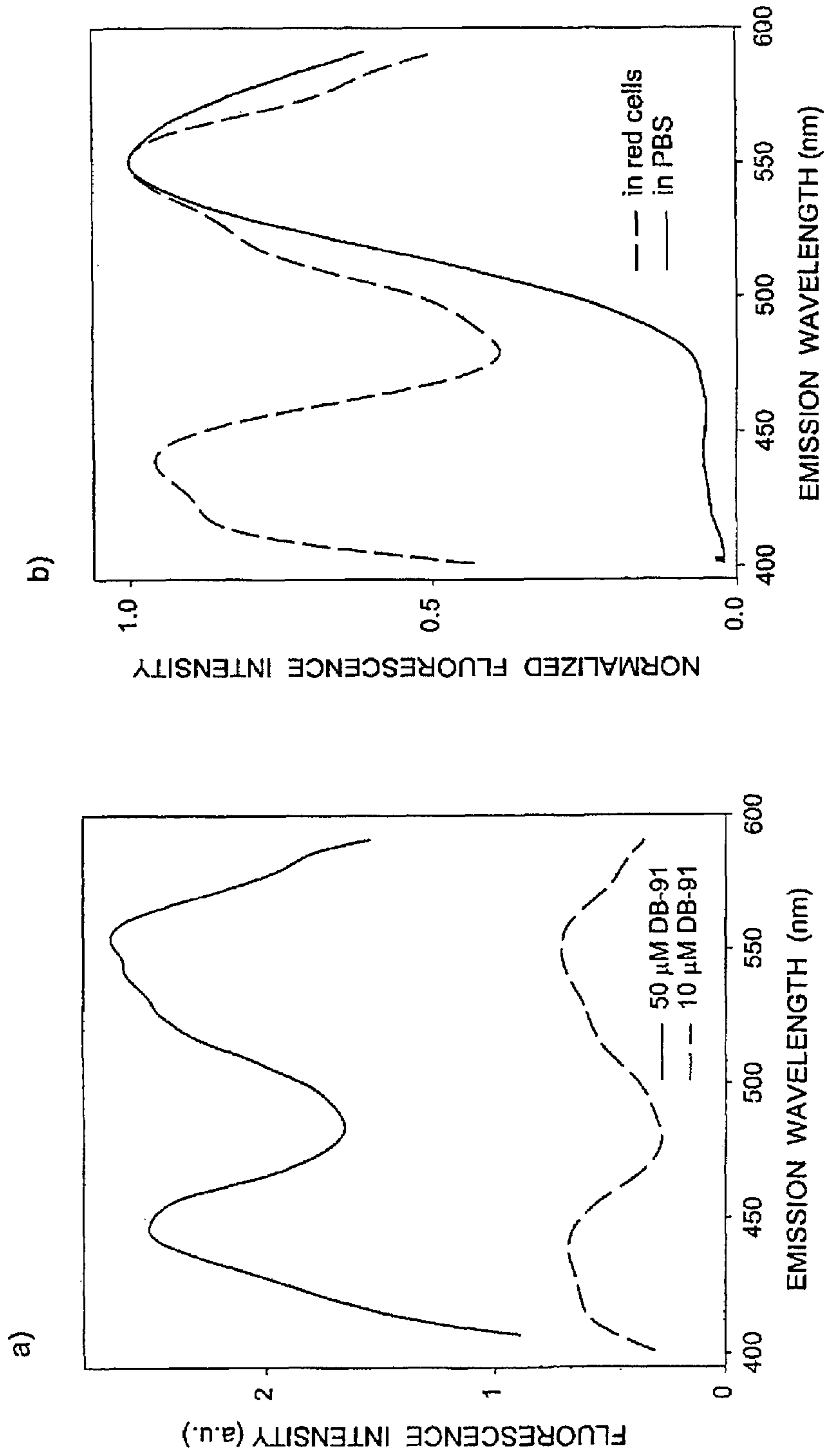
Figure 6. Fluorescence emission spectra of DB-91 in red cells (a) and normalized fluorescence emission spectra of 10 \mu\text{M} DB-91 in red cells and in PBS (b). Spectra was obtained by using front face method. \lambda_{\text{ex}} = 370 \text{ nm} , EX resol. 8 nm, EM resol. 4 nm, without EM polarizer, HV = 1260 V
