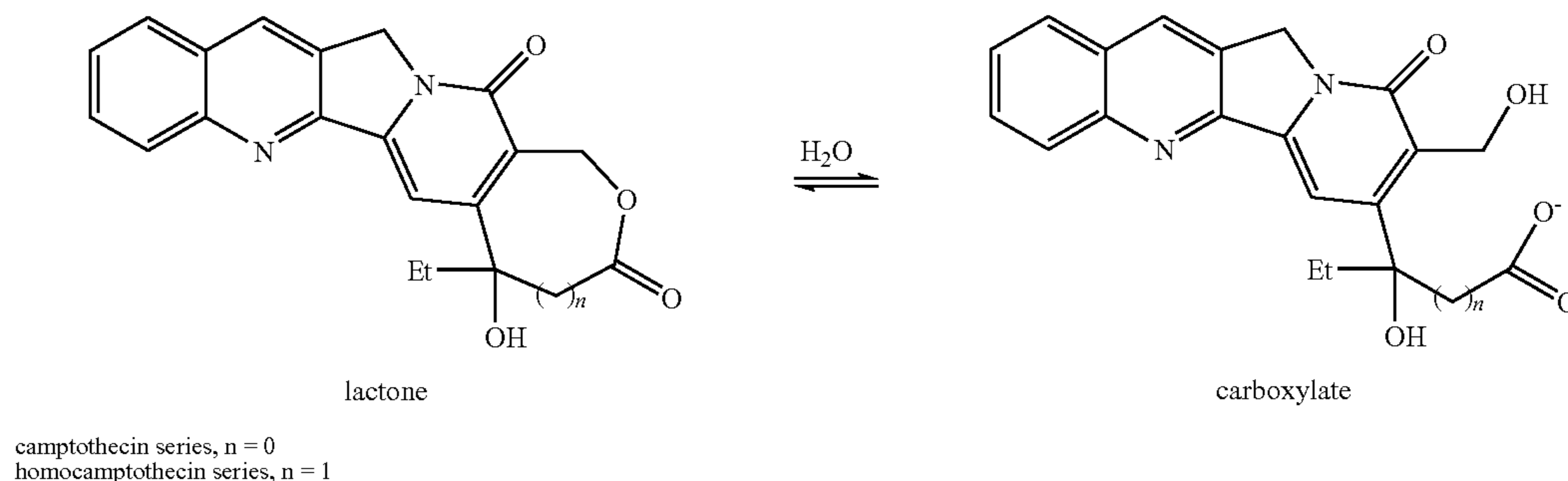
Lactone/Carboxylate Equilibrium
