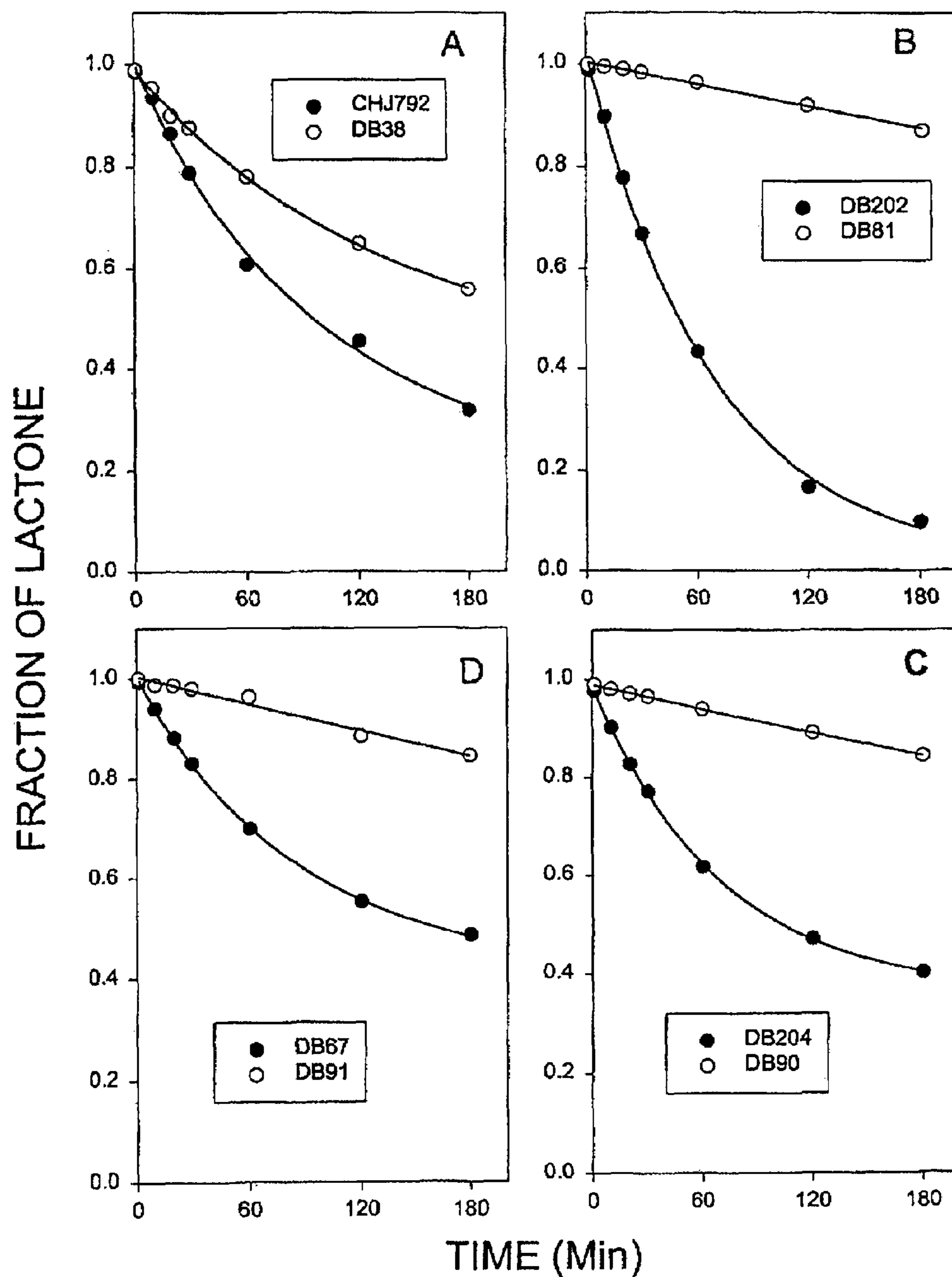
Figure 16. Comparison of the Stabilities of \alpha -Lactone Silatecans with their corresponding Homosilatecans in Whole Blood at 37°C
