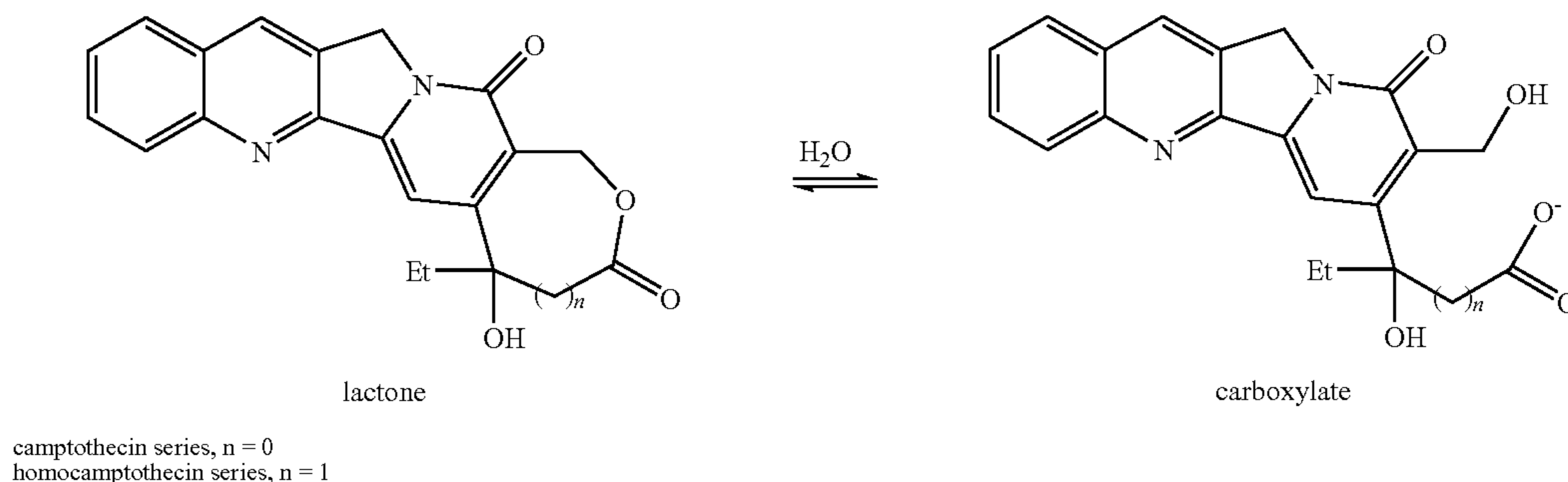
Lactone/Carboxylate Equilibrium
