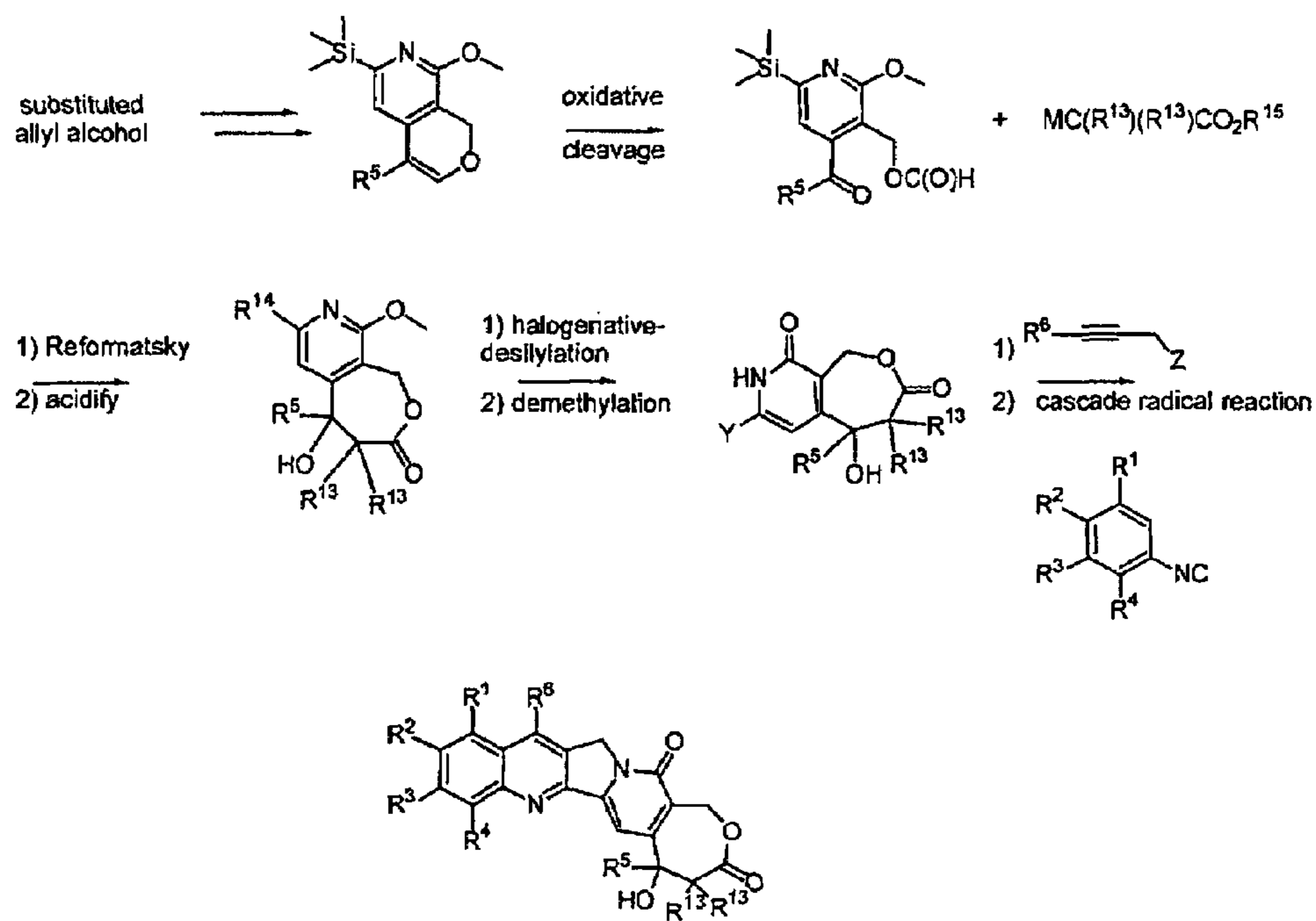
Figure 2b. General Route to A-, B-, and A/B Substituted Homocamptothecins
