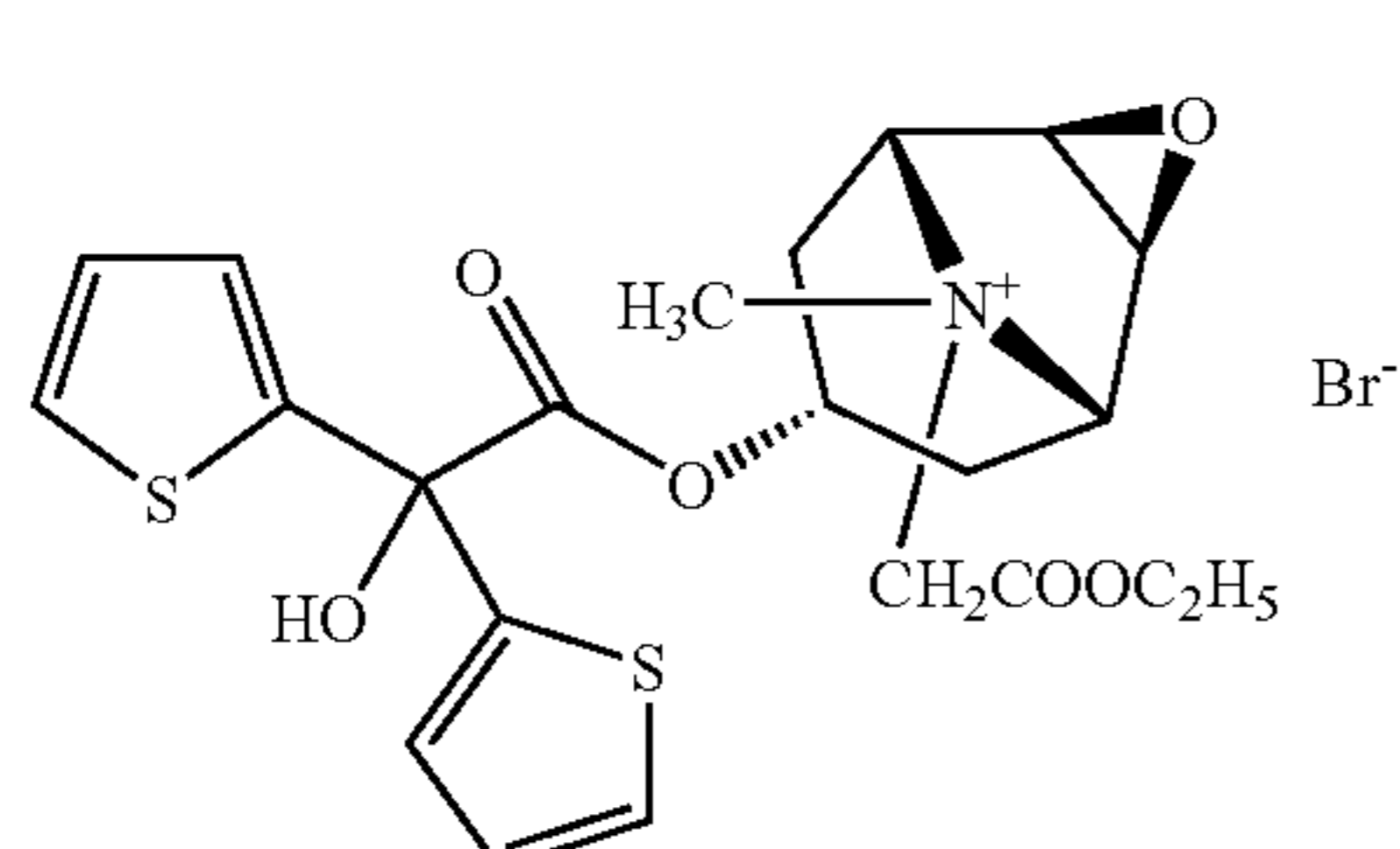
Tiotropium ethyl ester derivative derivative
