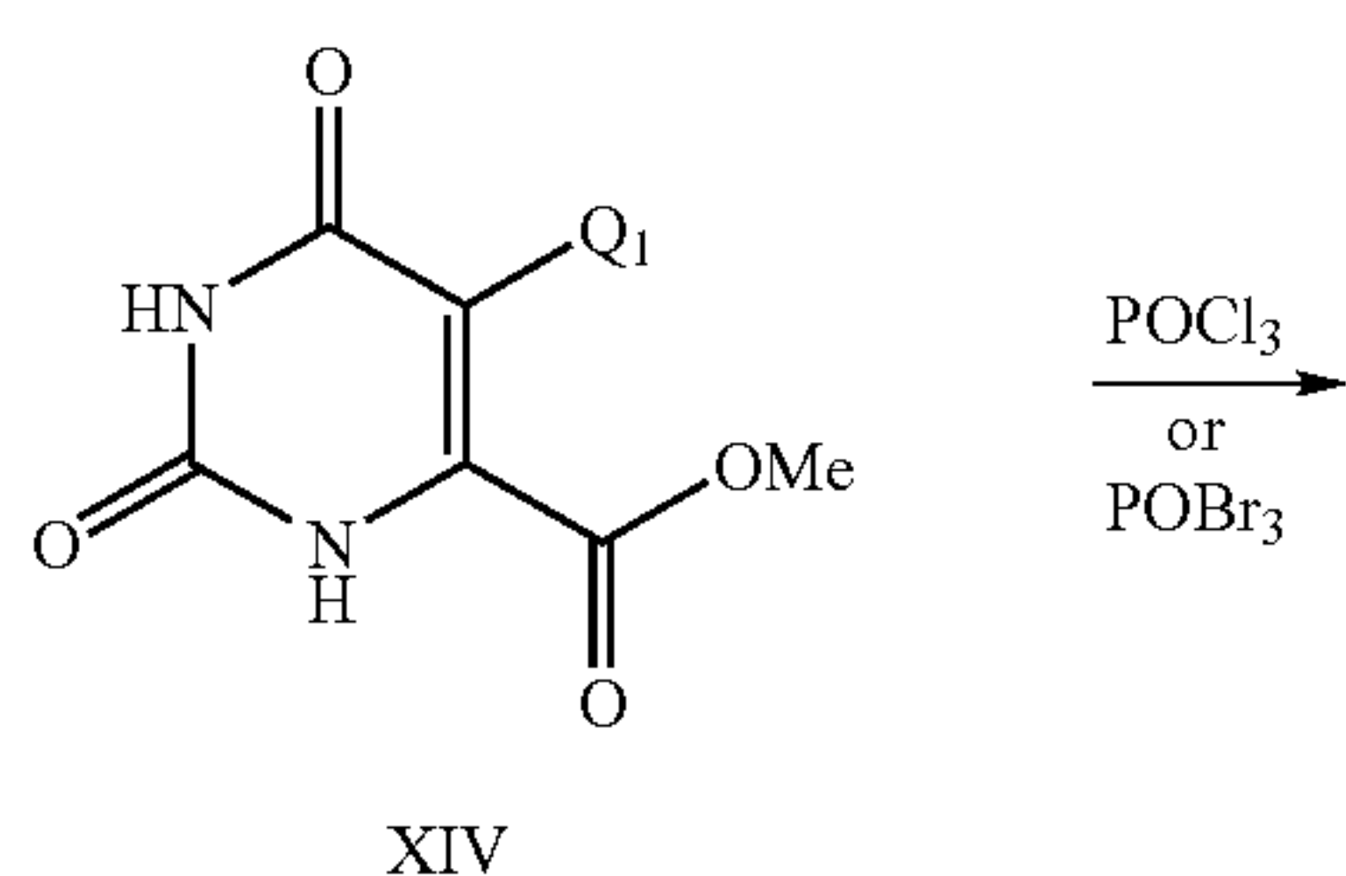
Scheme 6
