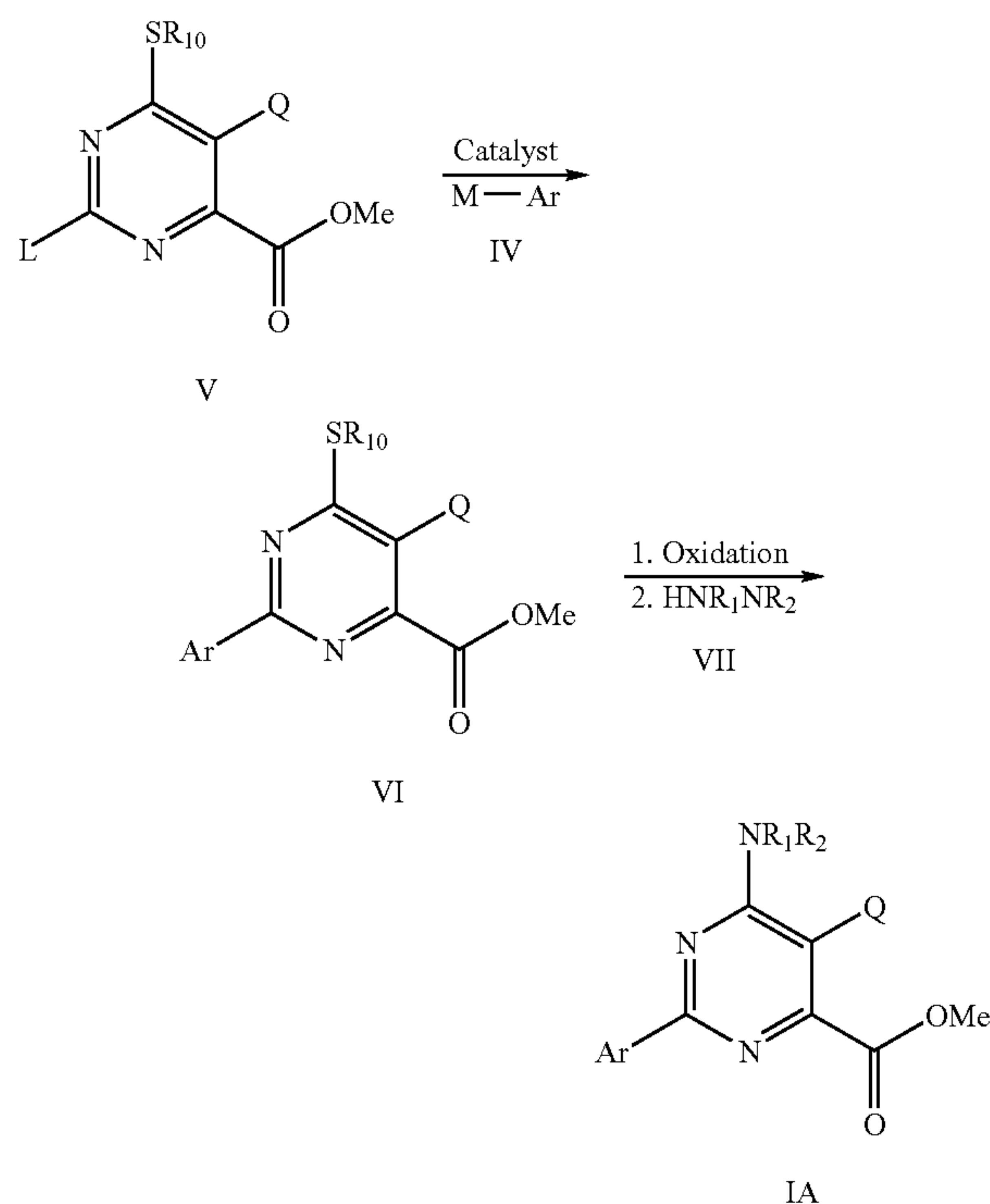
Scheme 3
