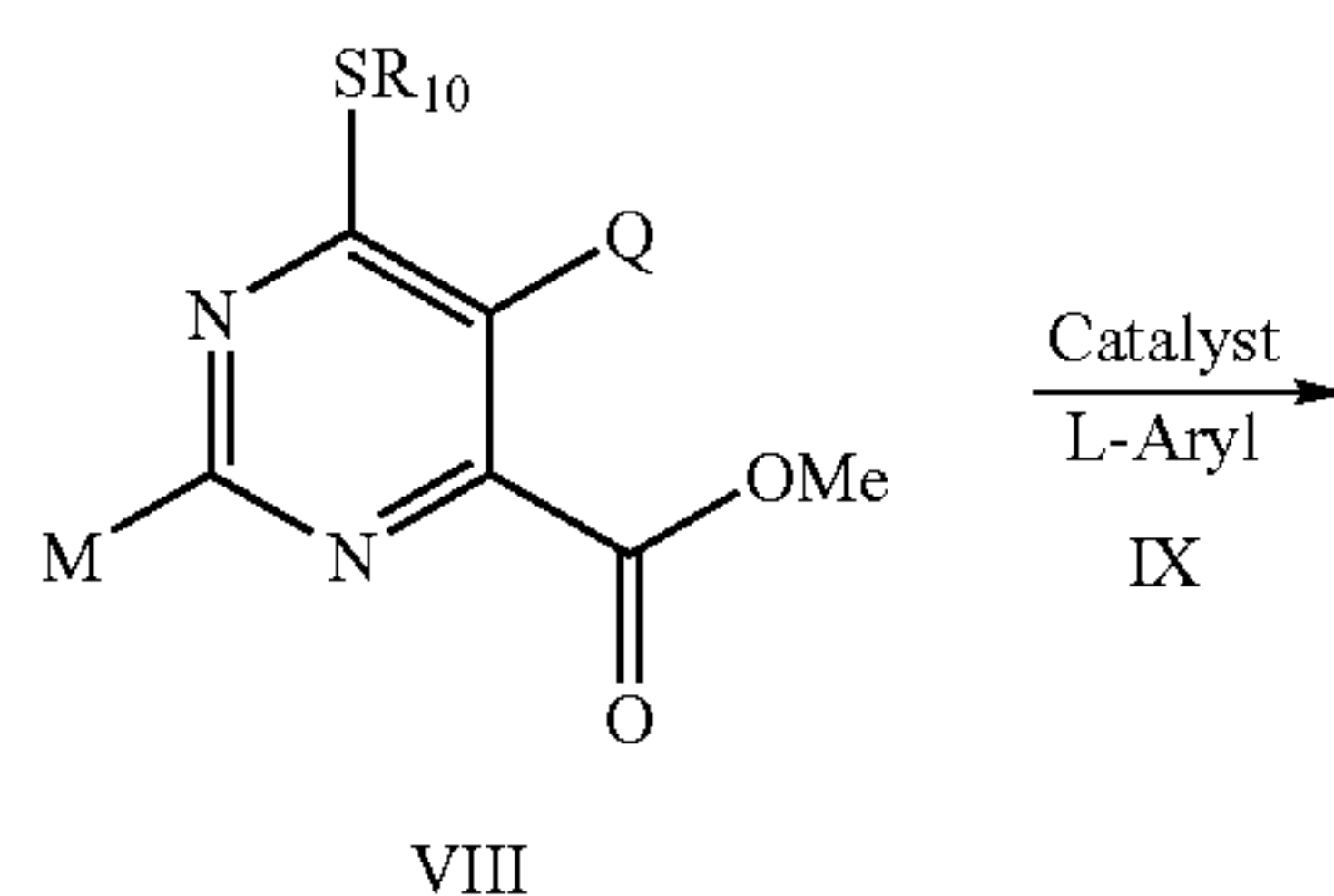
Scheme 4
