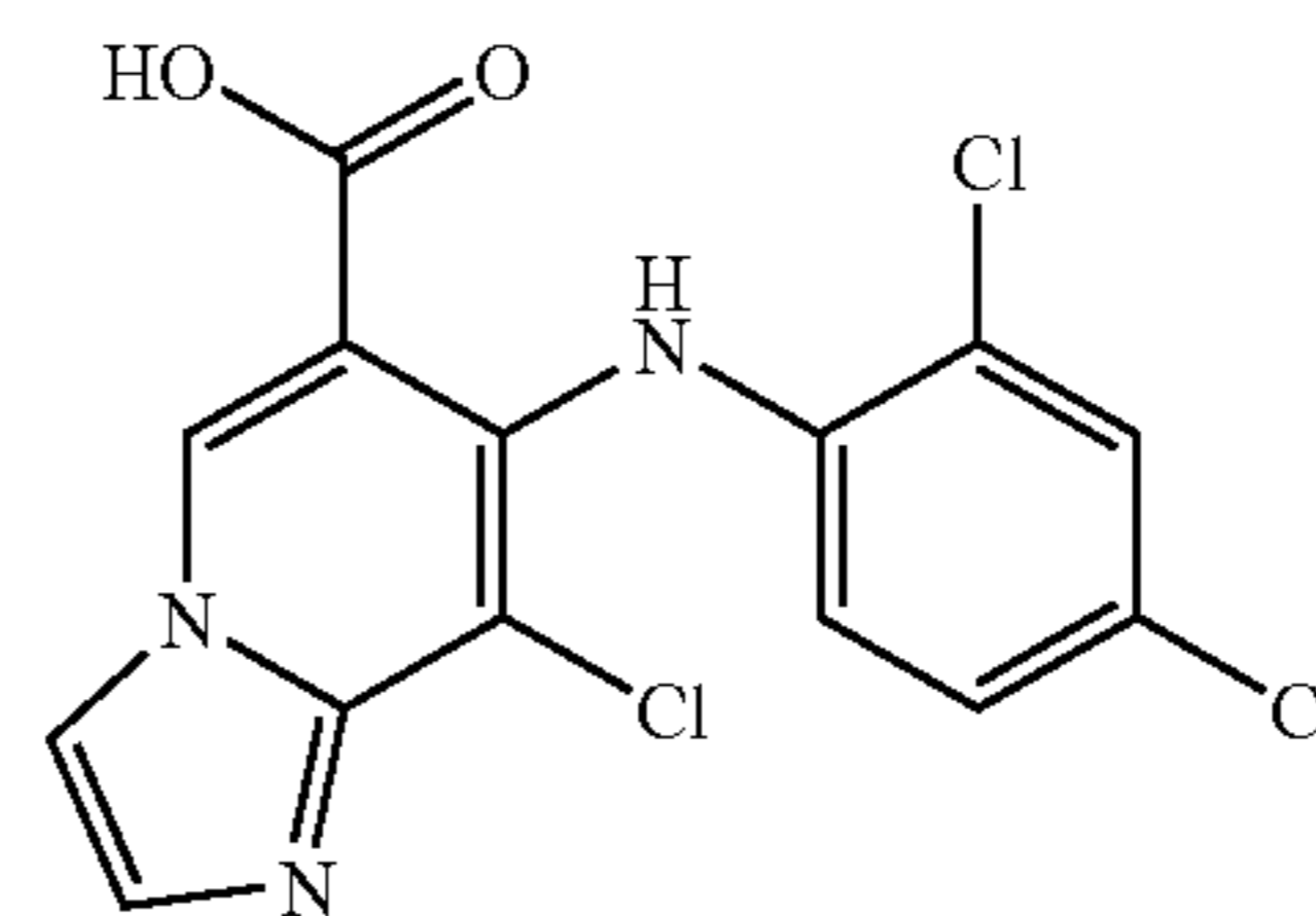
8-Chloro-7-(2,4-dichlorophenylamino)-imidazo[1,2-a]pyridine-6-carboxylic acid
