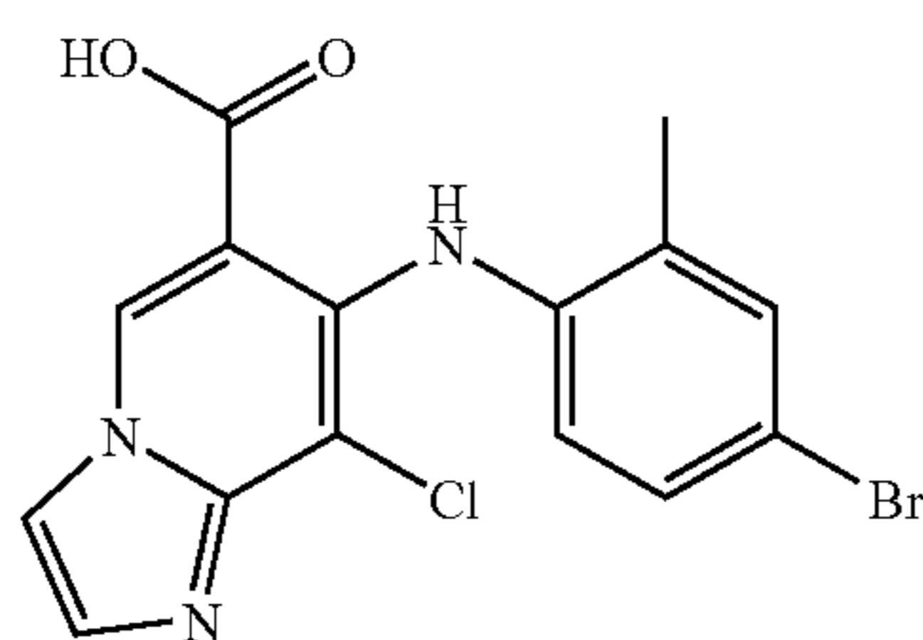
7-(4-Bromo-2-methylphenylamino)-8-chloroimidazo[1,2-a]pyridine-6-carboxylic acid
