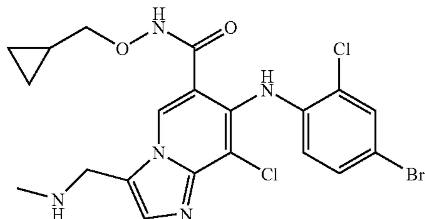
Synthesis of 7-(4-bromo-2-chlorophenylamino)-8-chloro-3-methylaminomethyl-imidazo[1,2-a]pyridine-6-carboxylic acid cyclopropylmethoxyamide (63)
