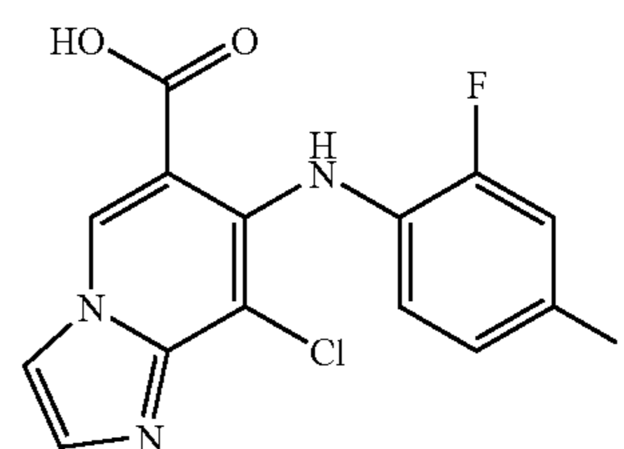
8-Chloro-7-(2-fluoro-4-iodophenylamino)-imidazo[1,2-a]pyridine-6-carboxylic acid
