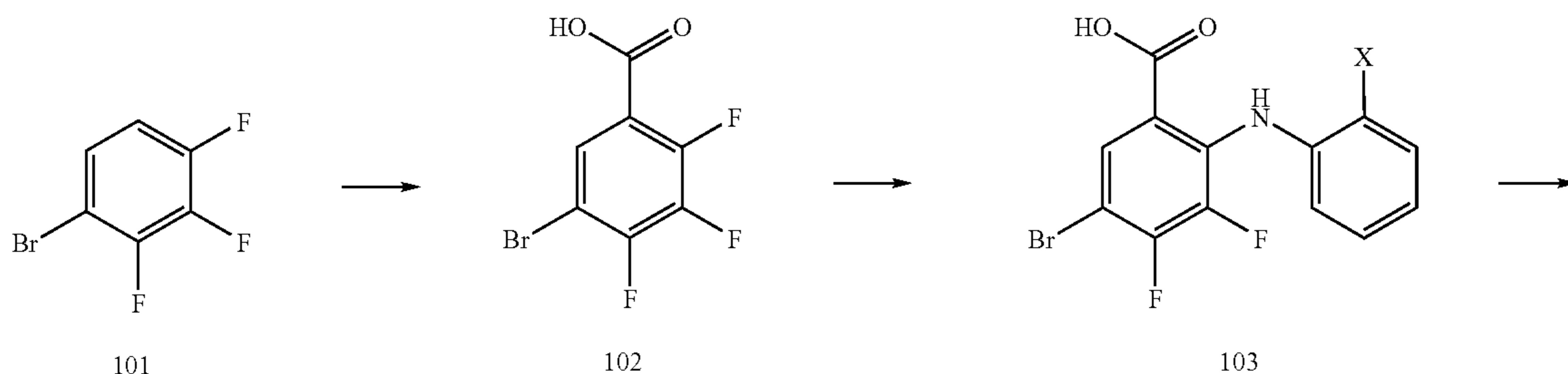
SCHEME 1
