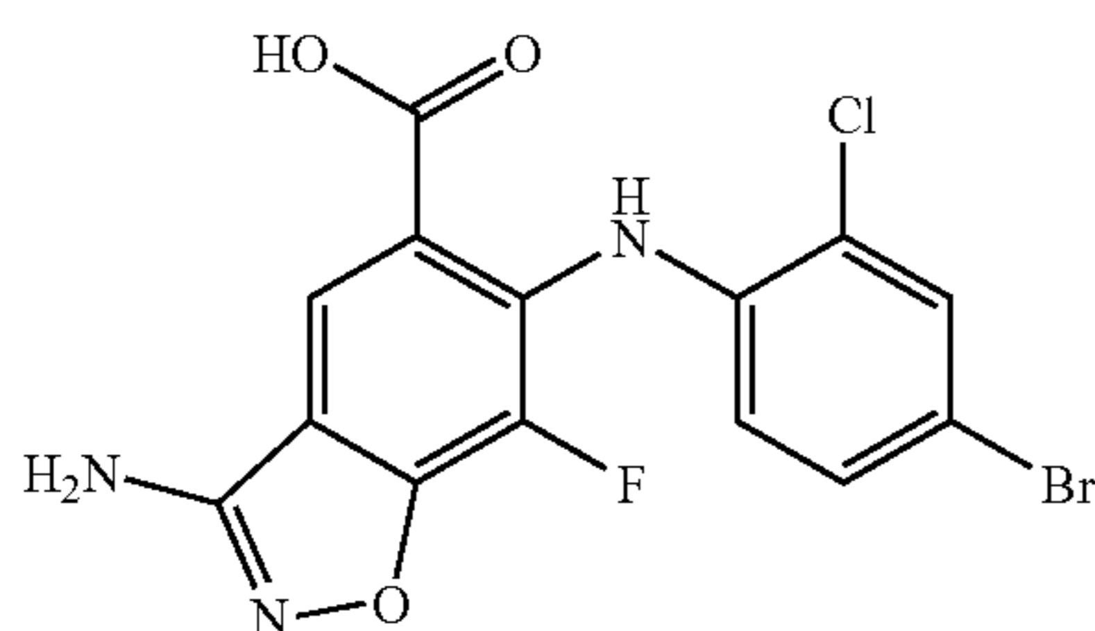
Synthesis of 3-amino-6-(4-bromo-2-chlorophenylamino)-7-fluorobenzo[d]isoxazole-5-carboxylic acid (19)
