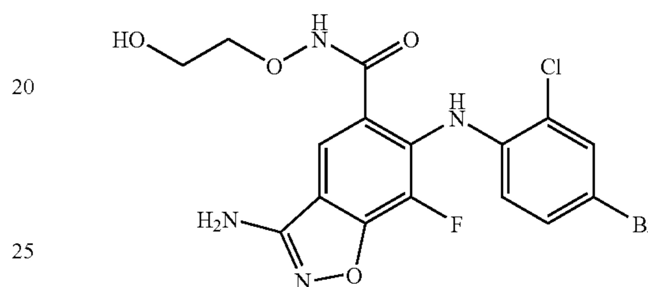
Synthesis of 3-amino-6-(4-bromo-2-chlorophenylamino)-7-fluorobenzo[d]isoxazole-5-carboxylic acid (2-hydroxyethoxy)-amide (21).
