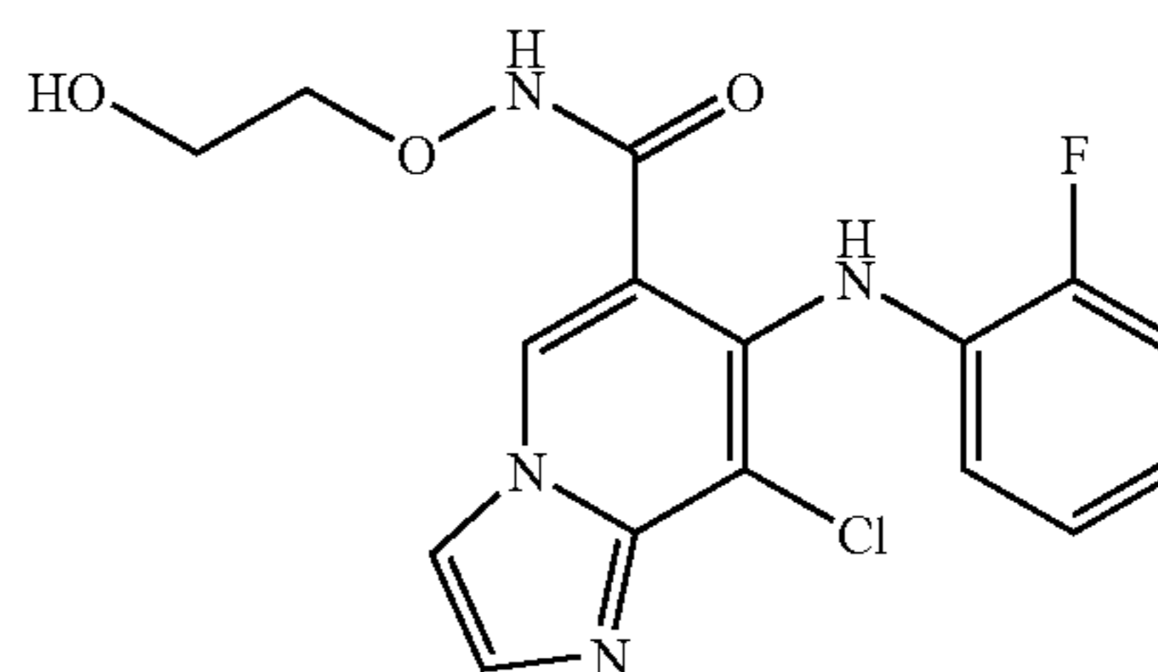
8-Chloro-7-(2-fluorophenylamino)-imidazo[1,2-a]pyridine-6-carboxylic acid (2-hydroxyethoxy)-amide
