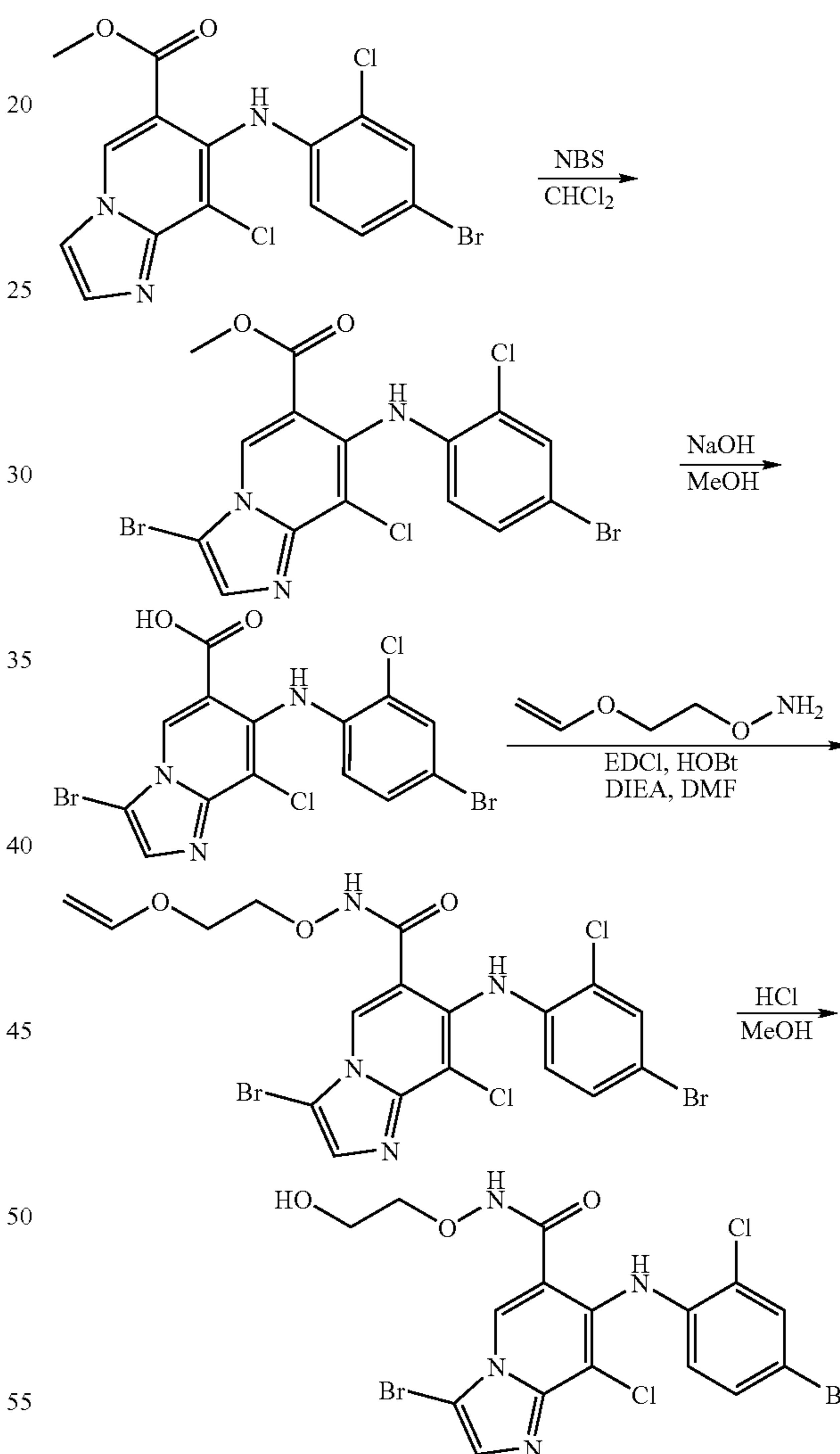
1-[7-(4-Bromo-2-chlorophenylamino)-8-chloroimidazo[1,2-a]pyridin-6-yl]-ethanone
