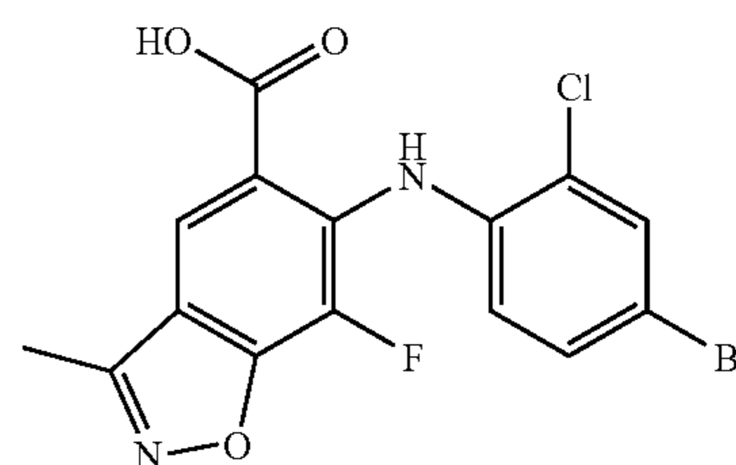
Synthesis of 6-(4-bromo-2-chlorophenylamino)-7-fluoro-3-methylbenzo[d]isoxazole-5-carboxylic acid (9a)
