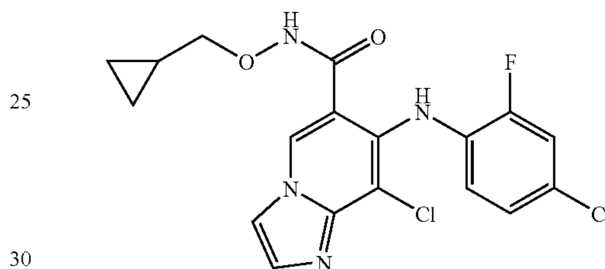
8-Chloro-7-(4-chloro-2-fluorophenylamino)-imidazo[1,2-a]pyridine-6-carboxylic acid cyclopropylmethoxyamide
