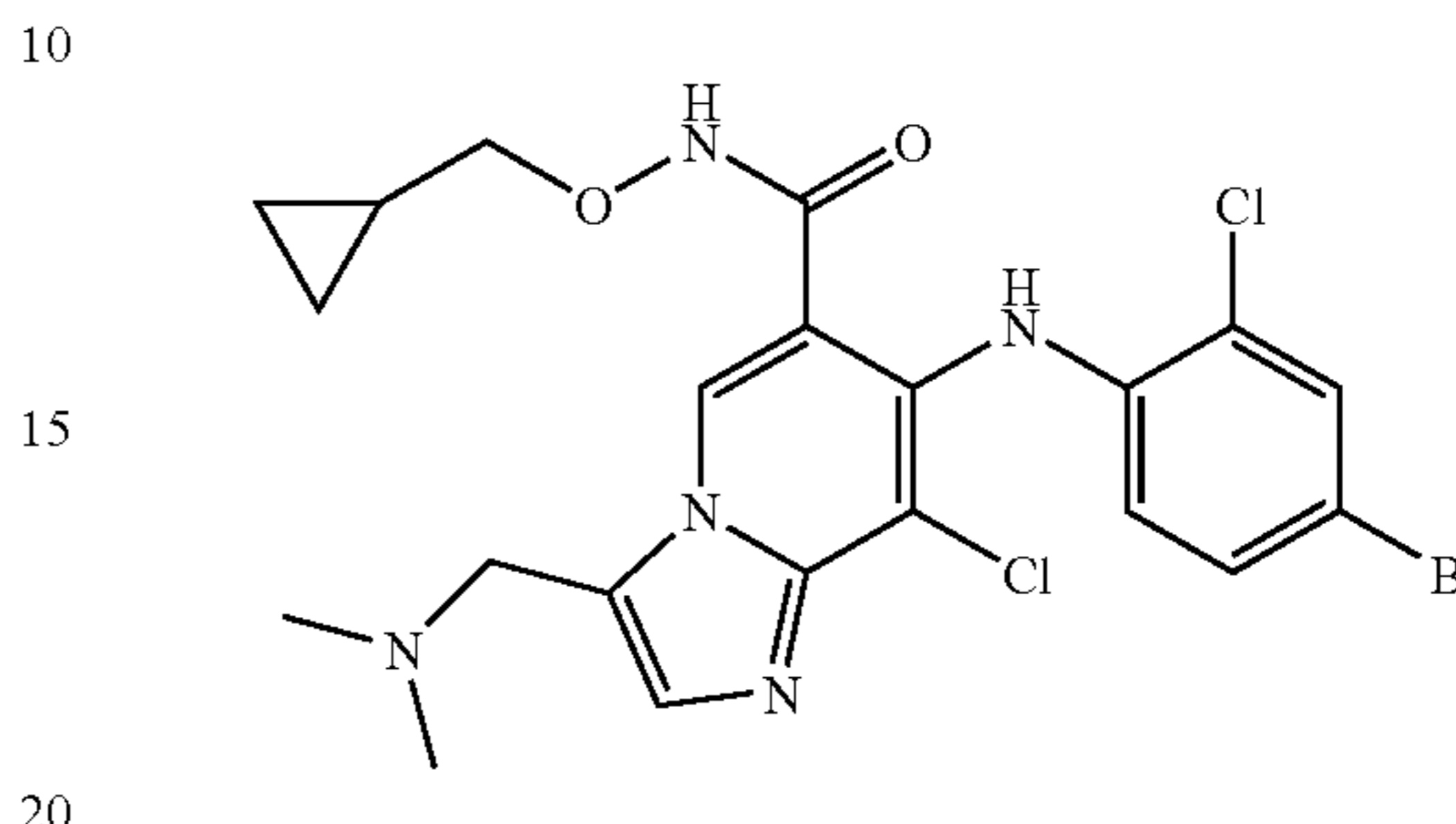
7-(4-Bromo-2-chlorophenylamino)-8-chloro-3-dimethylaminomethylimidazo[1,2-a]pyridine-6-carboxylic acid cyclopropylmethoxyamide
