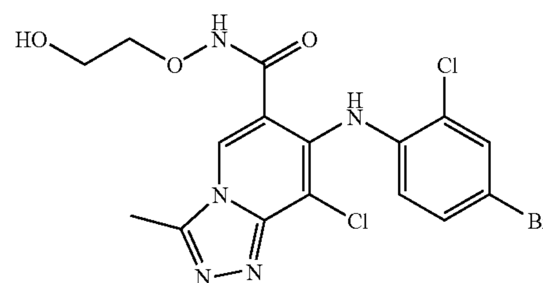
Synthesis of 7-(4-bromo-2-chlorophenylamino)-8-chloro-3-methyl-[1,2,4]triazolo[4,3-a]pyridine-6-carboxylic acid (2-hydroxyethoxy)-amide (54a)
