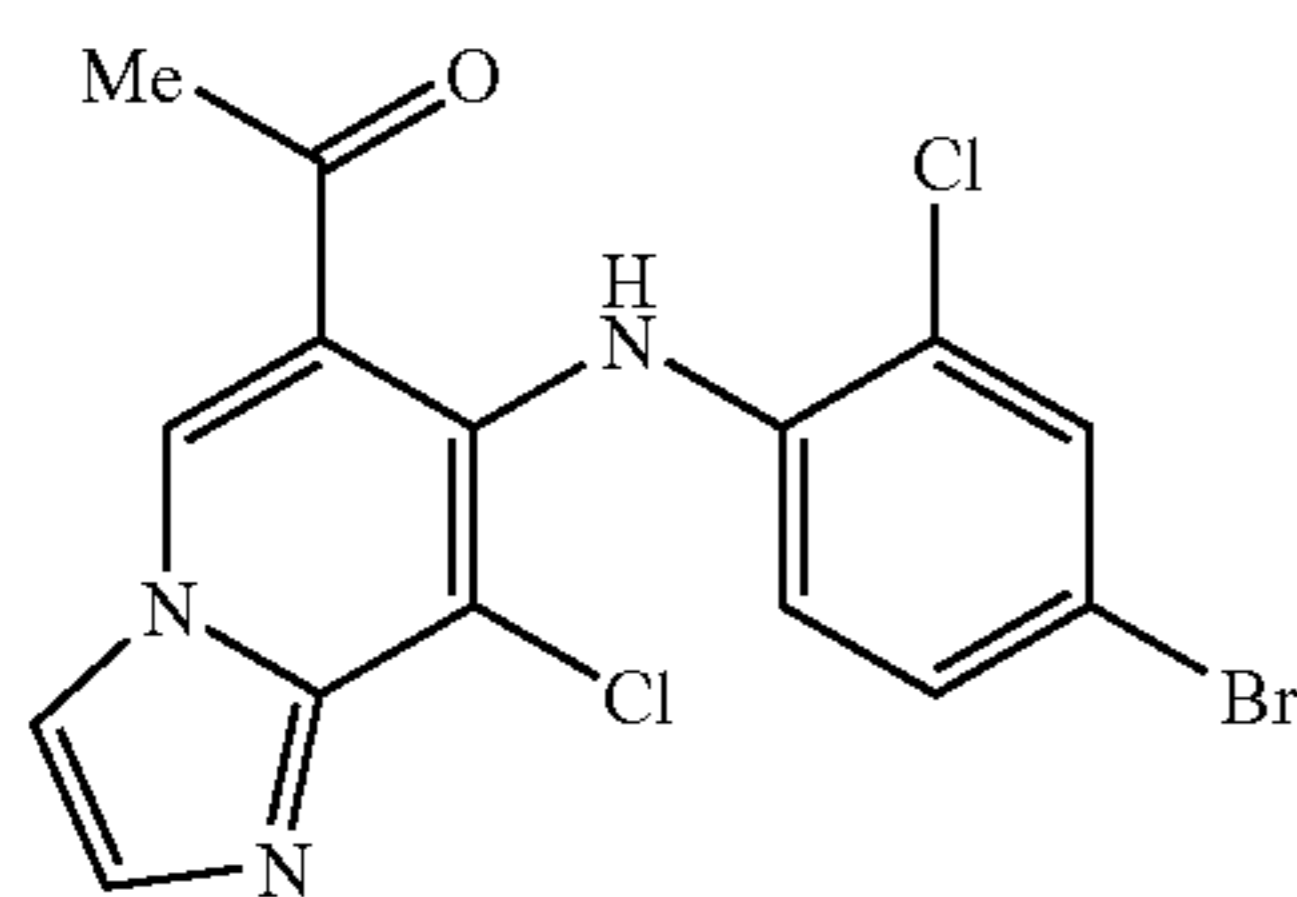
1-[7-(4-Bromo-2-chlorophenylamino)-8-chloroimidazo[1,2-a]pyridin-6-yl]-ethanone
