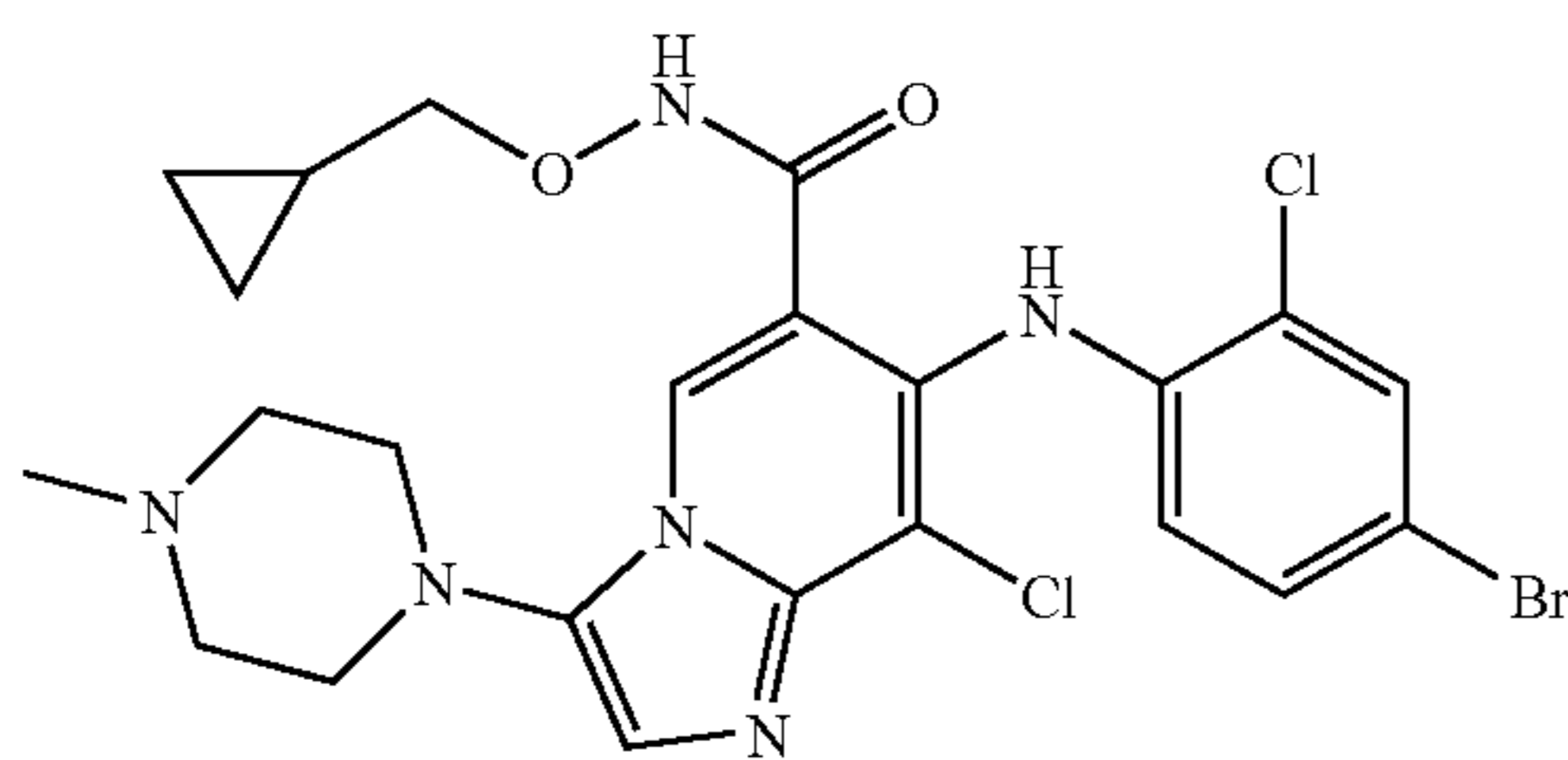
Synthesis of 7-(4-bromo-2-chlorophenylamino)-8-chloro-3-(4-methylpiperazin-1-yl)-imidazo[1,2-a]pyridine-6-carboxylic acid cyclopropylmethoxyamide (36)
