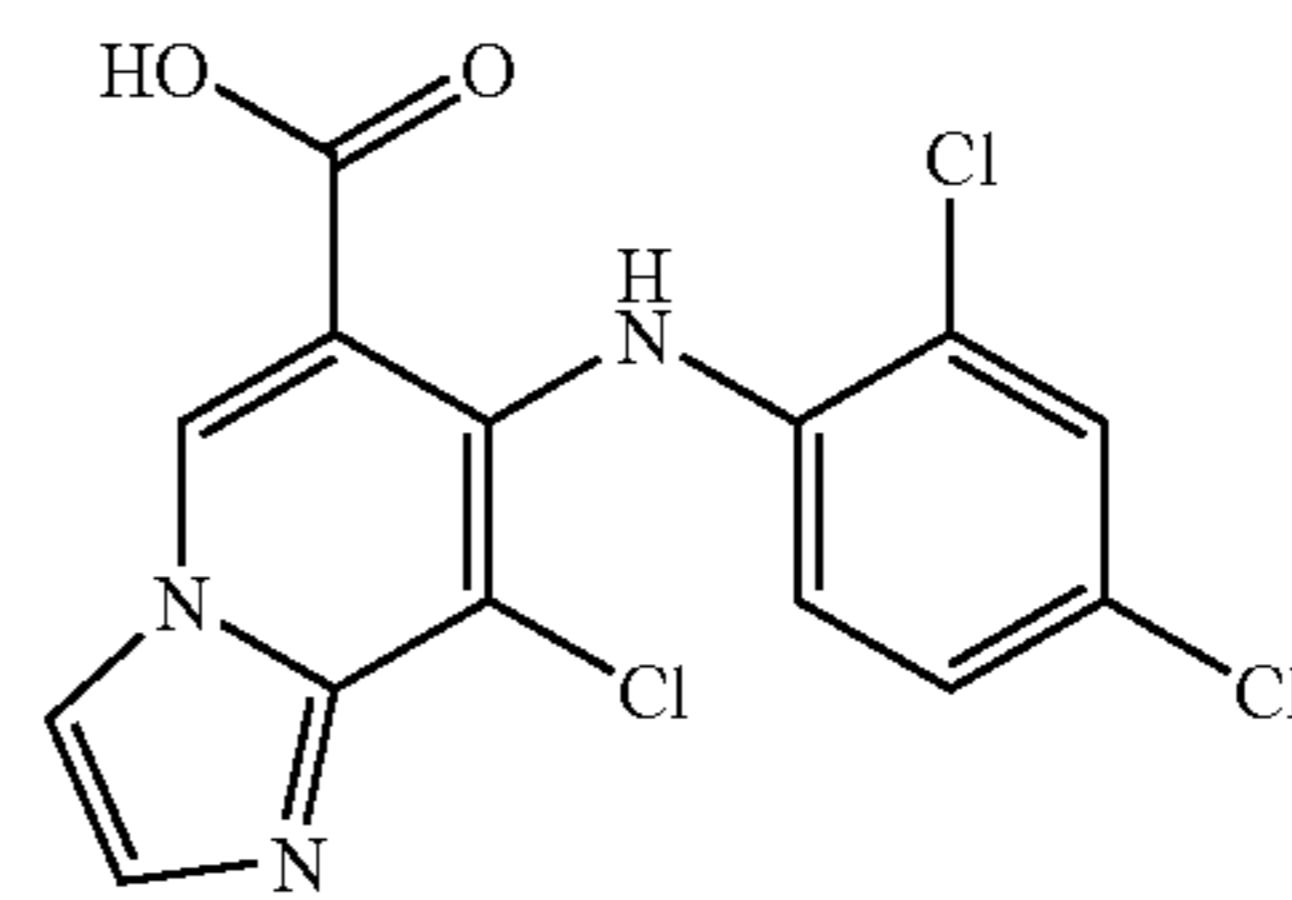
8-Chloro-7-(2,4-dichlorophenylamino)-imidazo[1,2-a]pyridine-6-carboxylic acid
