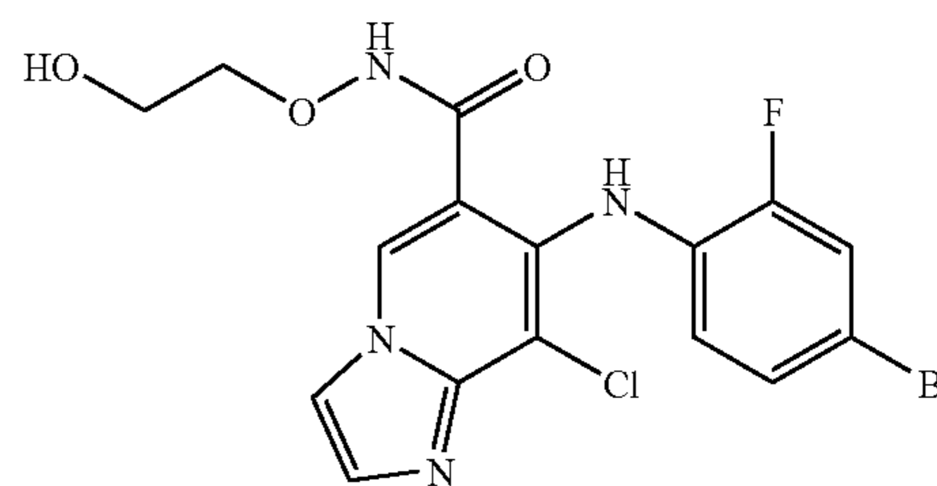
7-(4-bromo-2-fluorophenylamino)-8-chloroimidazo[1,2-a]pyridine-6-carboxylic acid (2-hydroxyethoxy)-amide
