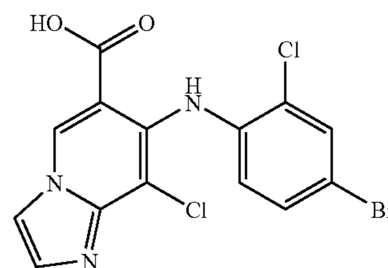
Synthesis of 7-(4-bromo-2-chlorophenylamino)-8-chloroimidazo[1,2-a]pyridine-6-carboxylic acid (30)
