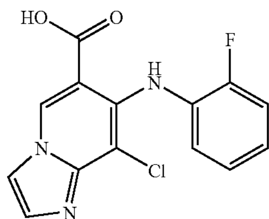
8-Chloro-7-(2-fluorophenylamino)-imidazo[1,2-a]pyridine-6-carboxylic acid
