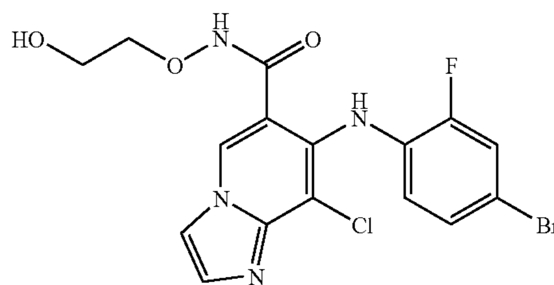
7-(4-bromo-2-fluorophenylamino)-8-chloroimidazo[1,2-a]pyridine-6-carboxylic acid (2-hydroxyethoxy)-amide
