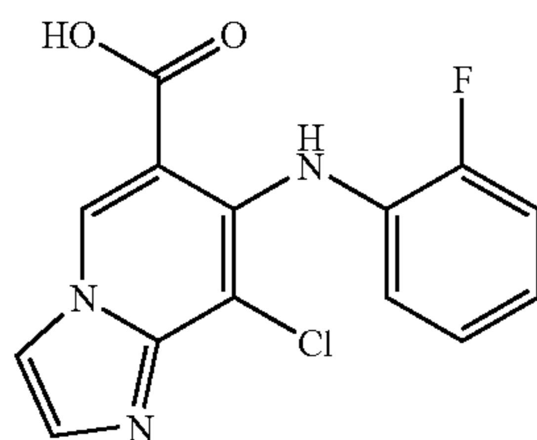
8-Chloro-7-(2-fluorophenylamino)-imidazo[1,2-a]pyridine-6-carboxylic acid
