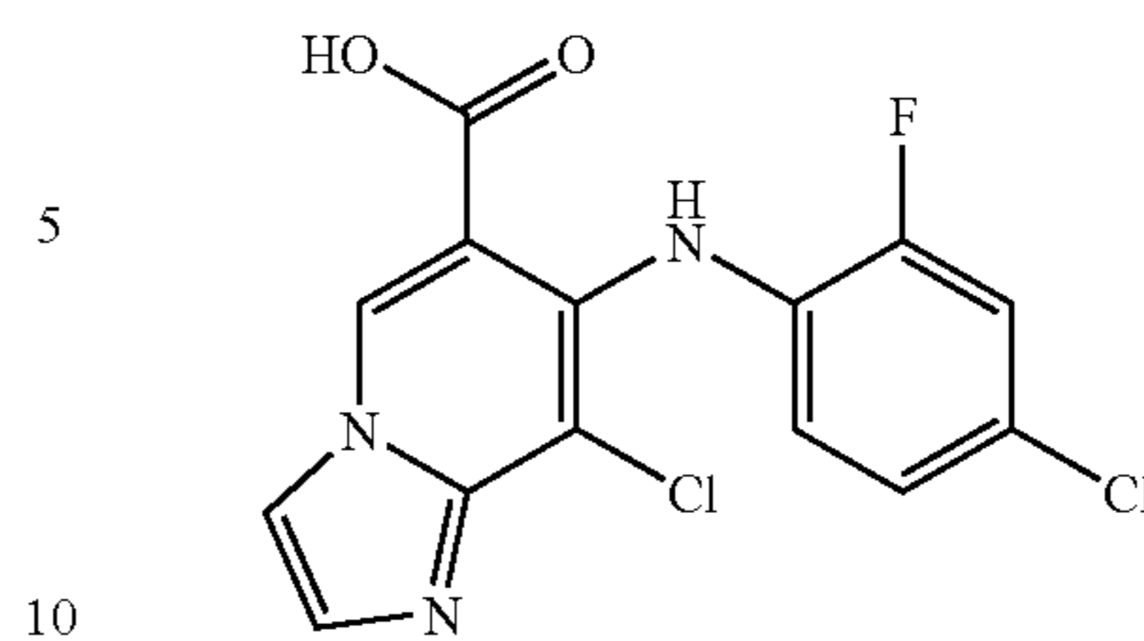
8-Chloro-7-(4-chloro-2-fluorophenylamino)-imidazo[1,2-a]pyridine-6-carboxylic acid
