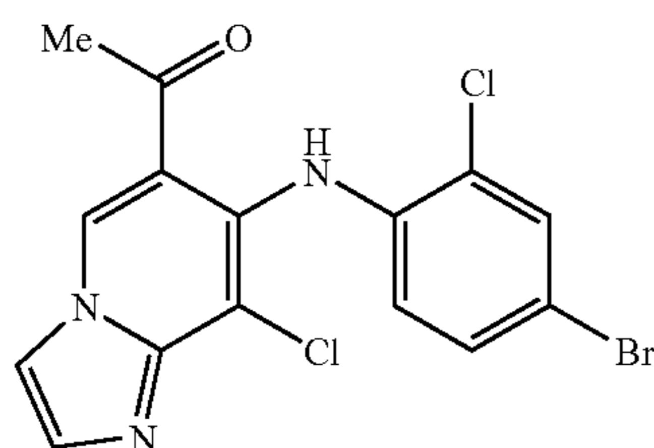
1-[7-(4-Bromo-2-chlorophenylamino)-8-chloroimidazo[1,2-a]pyridin-6-yl]-ethanone
