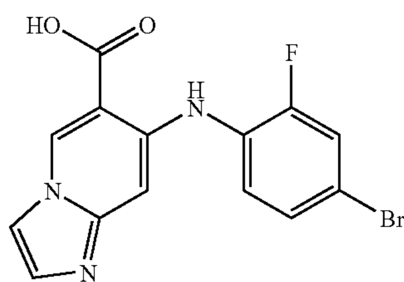
7-(4-Bromo-2-fluorophenylamino)-imidazo[1,2-a]pyridine-6-carboxylic acid
