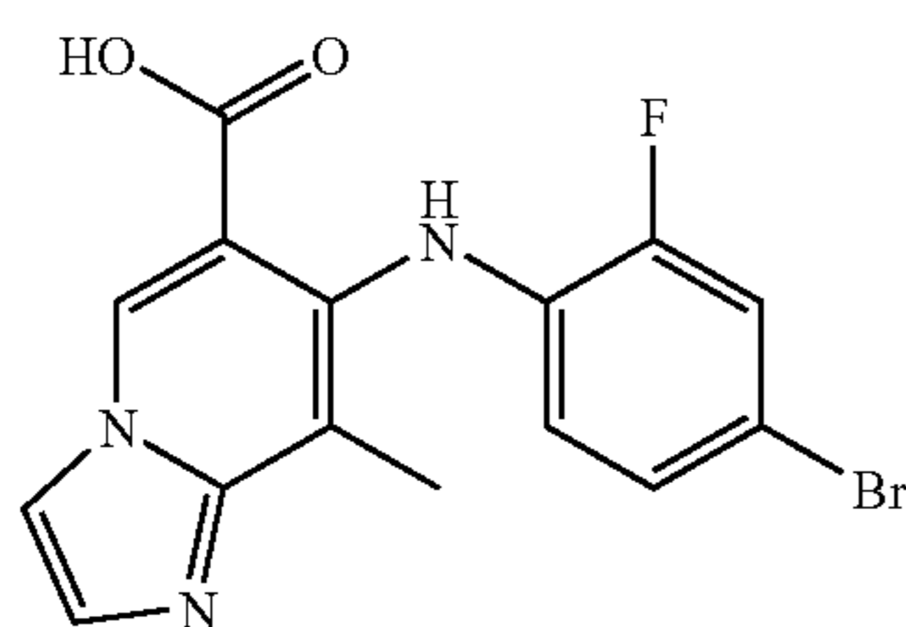
7-(4-Bromo-2-fluorophenylamino)-8-methylimidazo[1,2-a]pyridine-6-carboxylic acid
