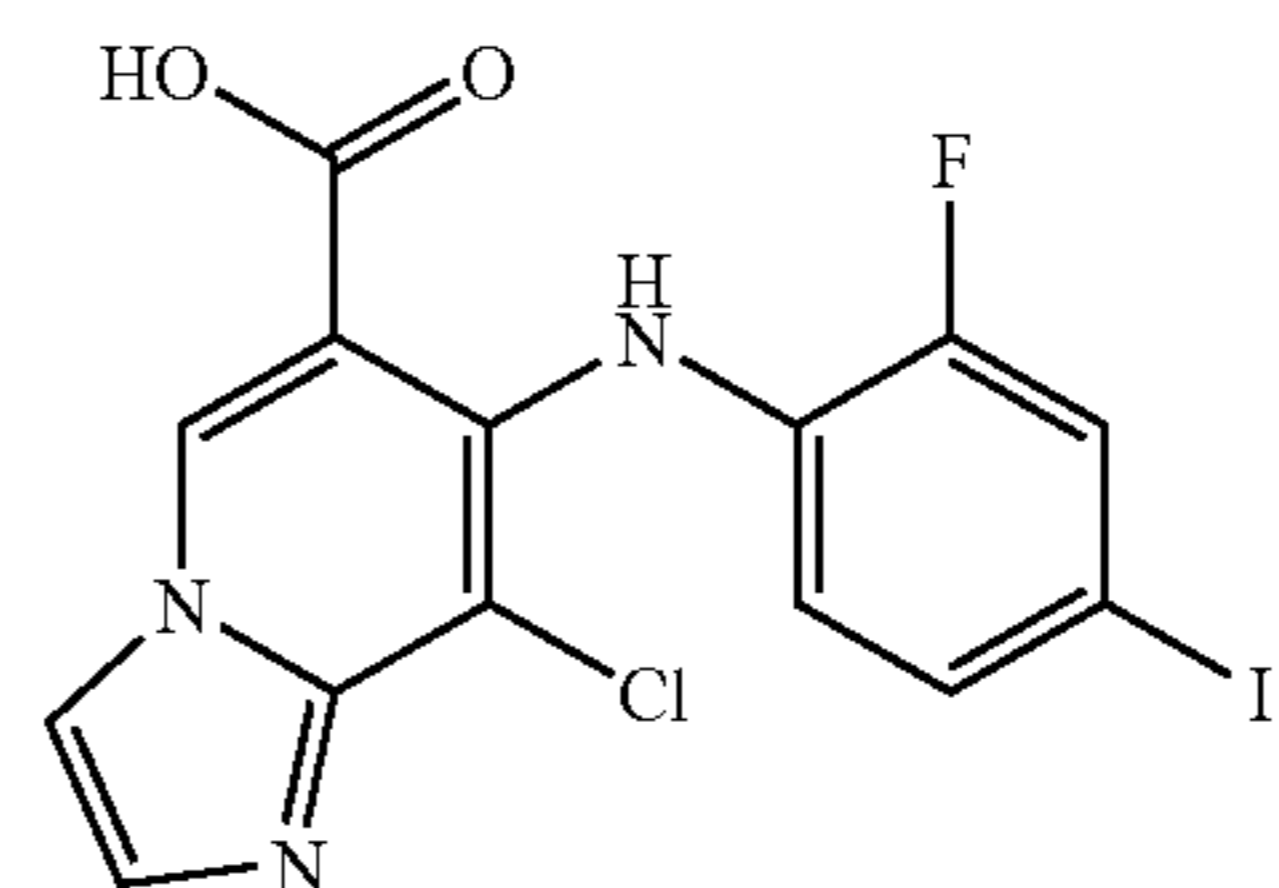
8-Chloro-7-(2-fluoro-4-iodophenylamino)-imidazo[1,2-a]pyridine-6-carboxylic acid
