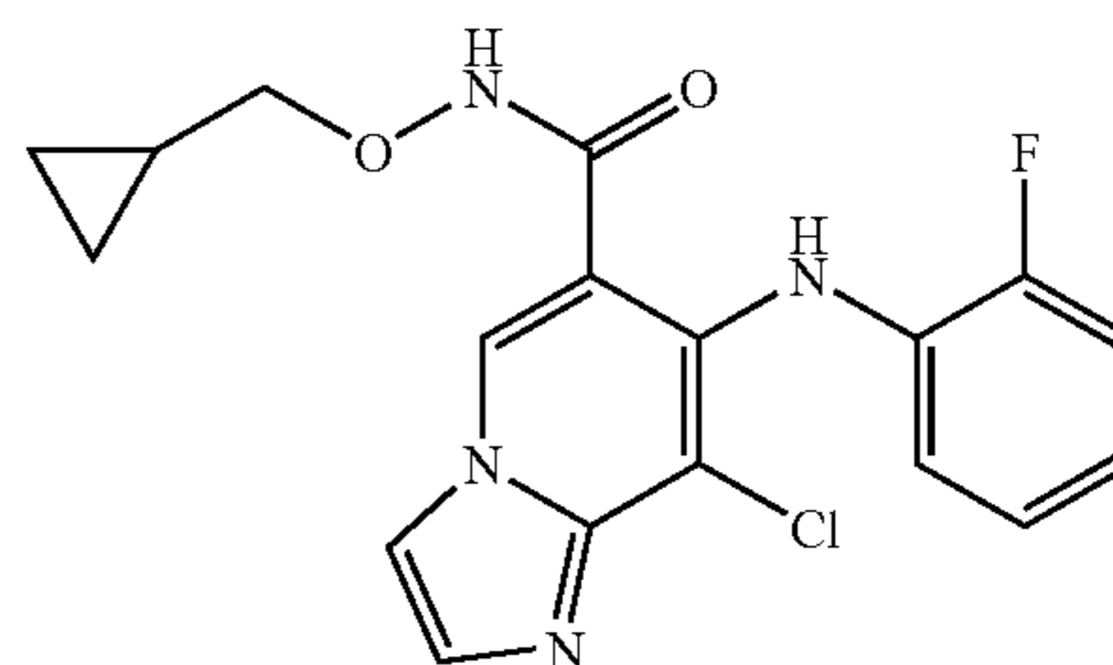
8-chloro-7-(2-fluorophenylamino)-imidazo[1,2-a]pyridine-6-carboxylic acid cyclopropylmethoxyamide
