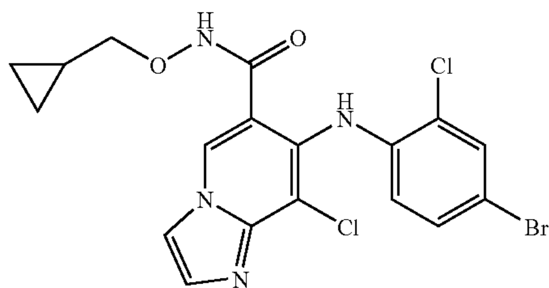
7-(4-bromo-2-chlorophenylamino)-8-chloroimidazo[1,2-a]pyridine-6-carboxylic acid cyclopropylmethoxyamide (31)
