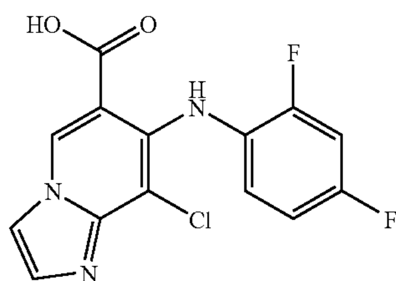
8-Chloro-7-(2,4-difluorophenylamino)-imidazo[1,2-a]pyridine-6-carboxylic acid
