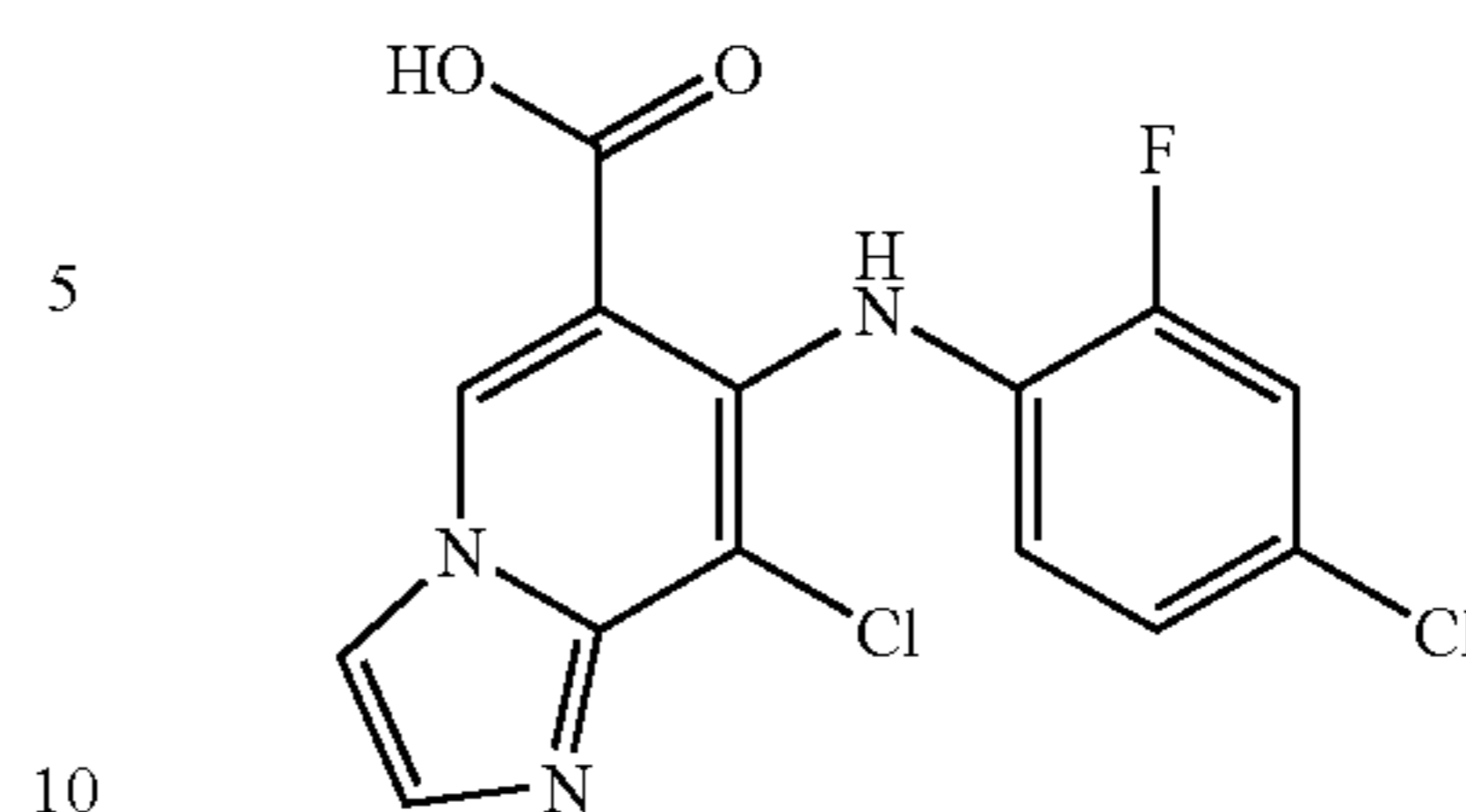
8-Chloro-7-(4-chloro-2-fluorophenylamino)-imidazo[1,2-a]pyridine-6-carboxylic acid
