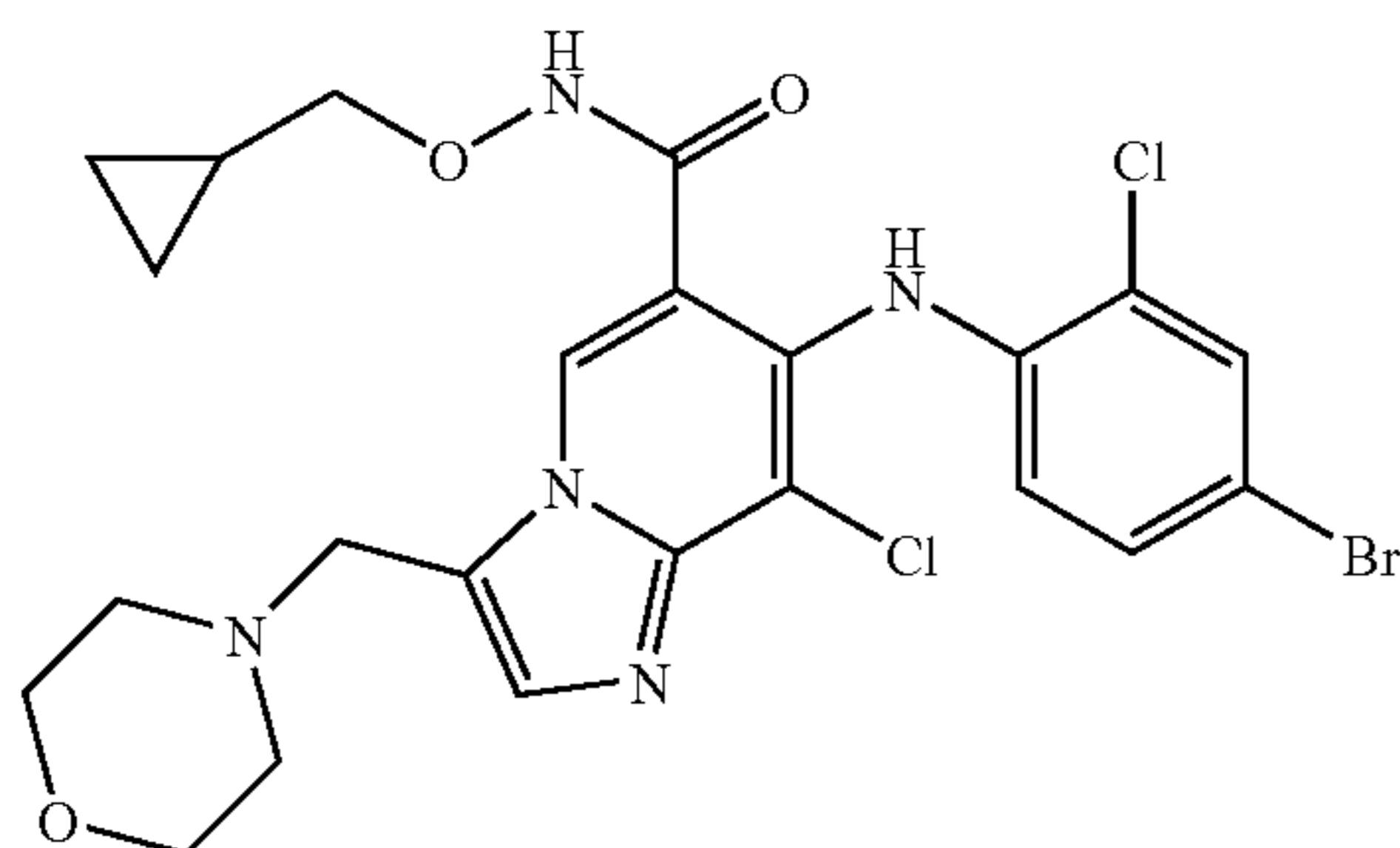
7-(4-Bromo-2-chlorophenylamino)-8-chloro-3-morpholin-4-ylmethyl-imidazo[1,2-a]pyridine-6-carboxylic acid cyclopropylmethoxyamide
