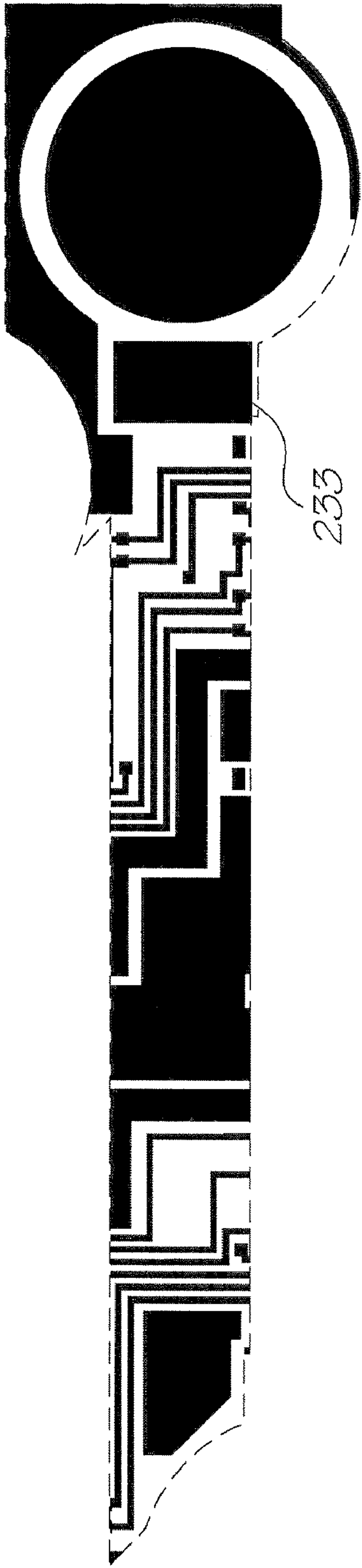
Metal 2 mask
