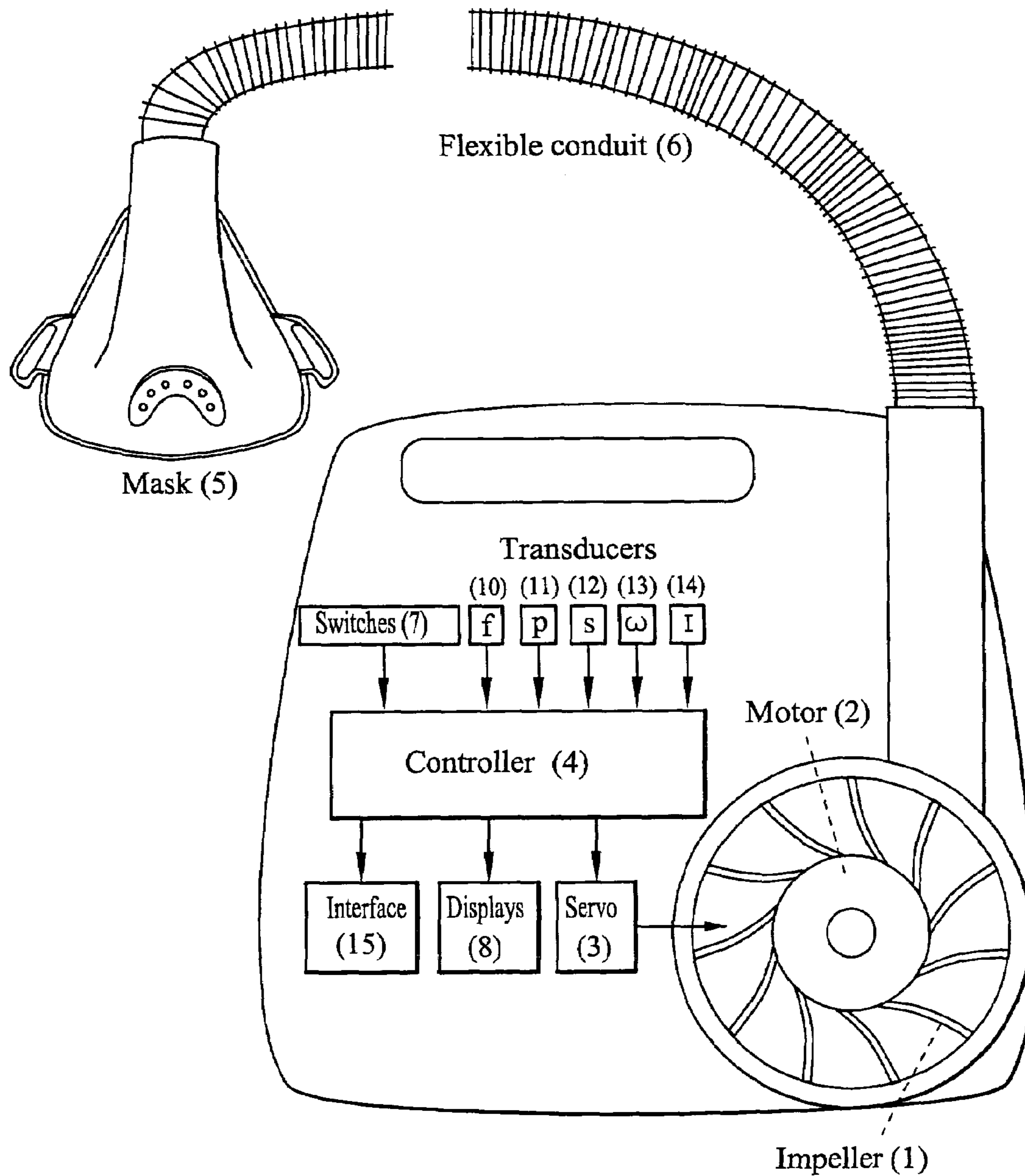
Figure 2: CPAP apparatus
